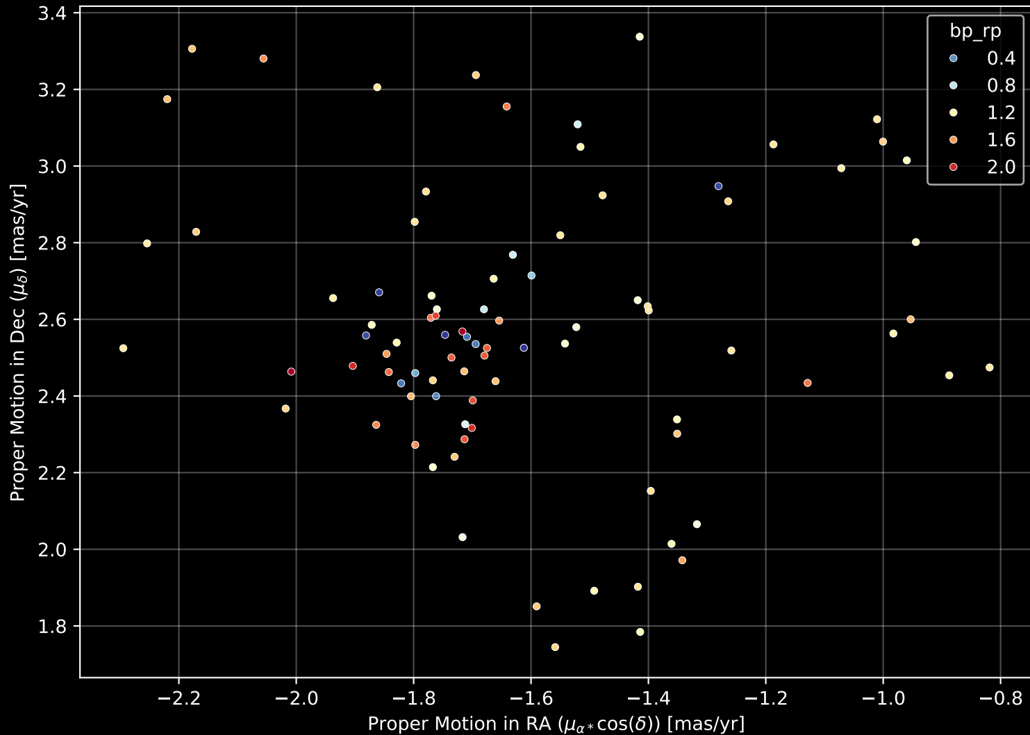
Gaia Cluster: [NGC_2367] Proper Motion Diagram (n= 89)
