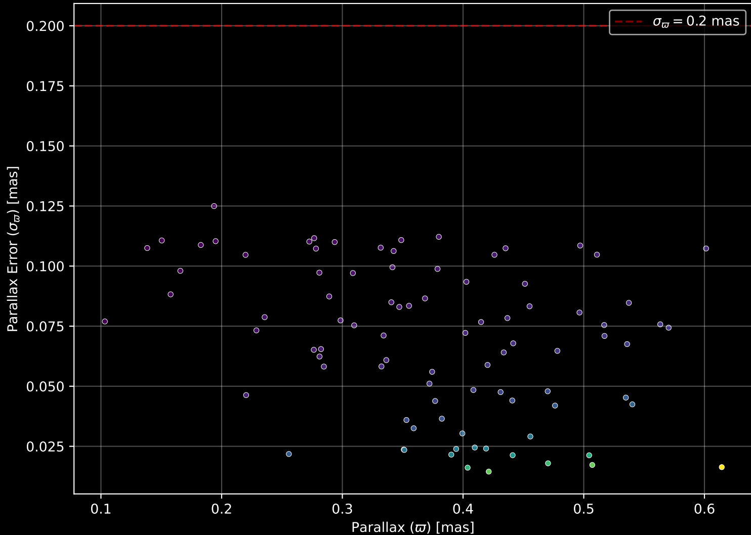
Gaia Cluster: [NGC_2367] Parallax Quality (n= 89)
