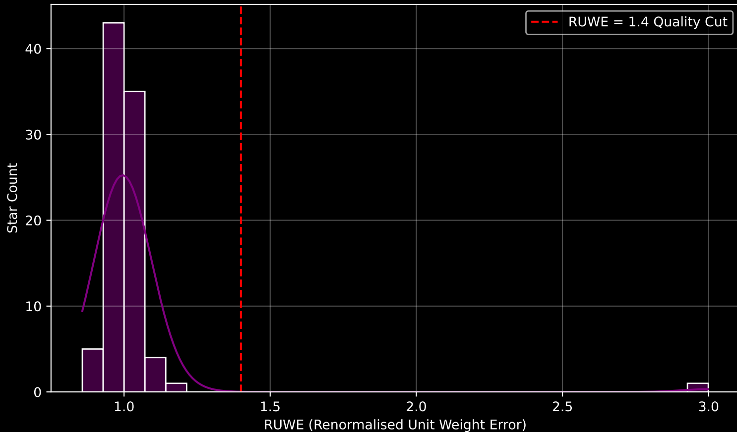
Gaia Cluster: [NGC_2367] RUWE Distribution (n= 89)
