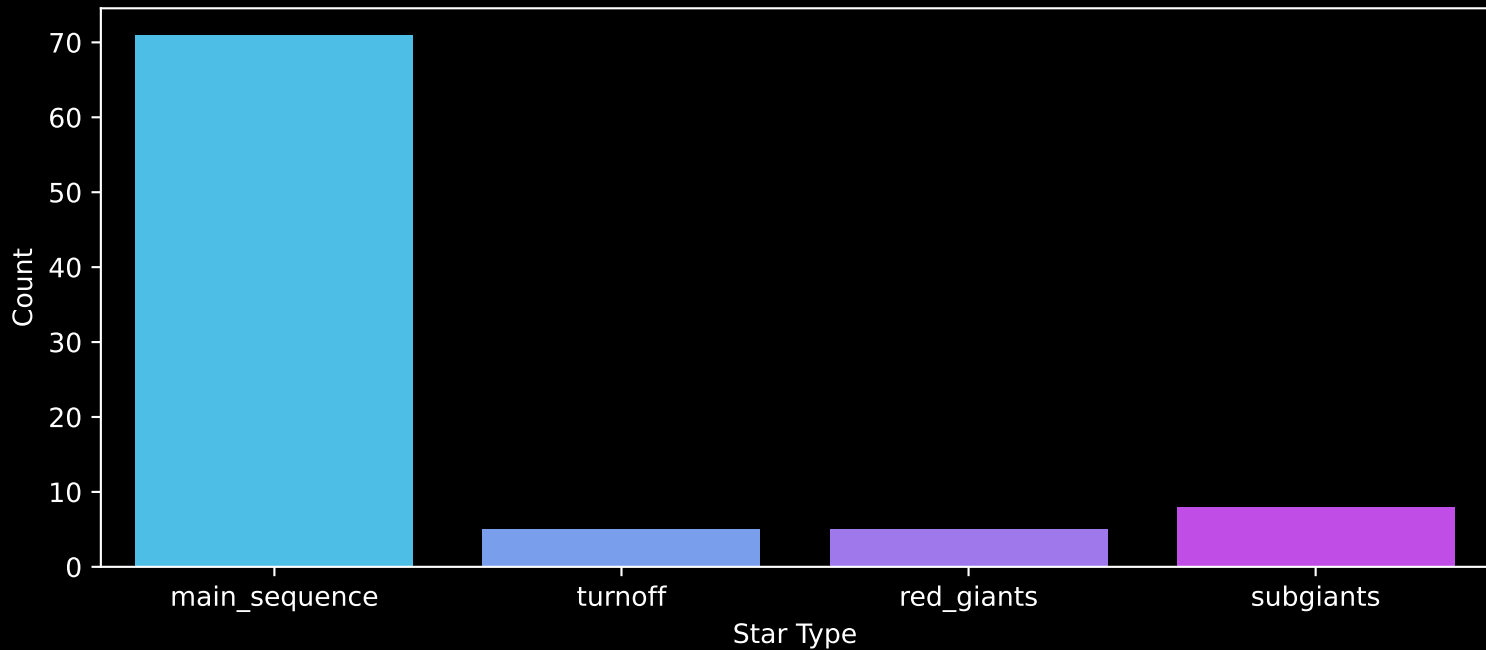
Gaia Cluster: [NGC_2367] Count plot of Star Type
