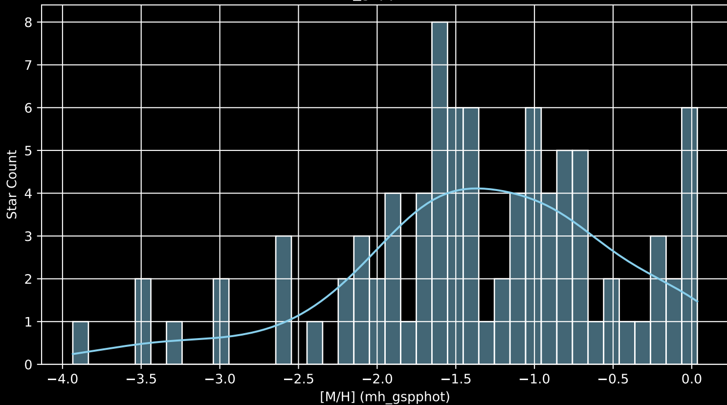
Gaia Cluster: [NGC_2367 [M/H] (mh_gspphot) (n= 89)
