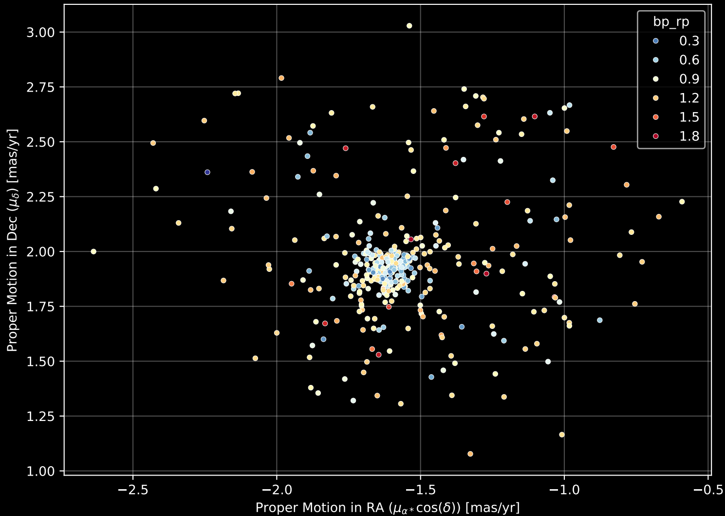
Gaia Cluster: [NGC_2383] Proper Motion Diagram (n= 387)
