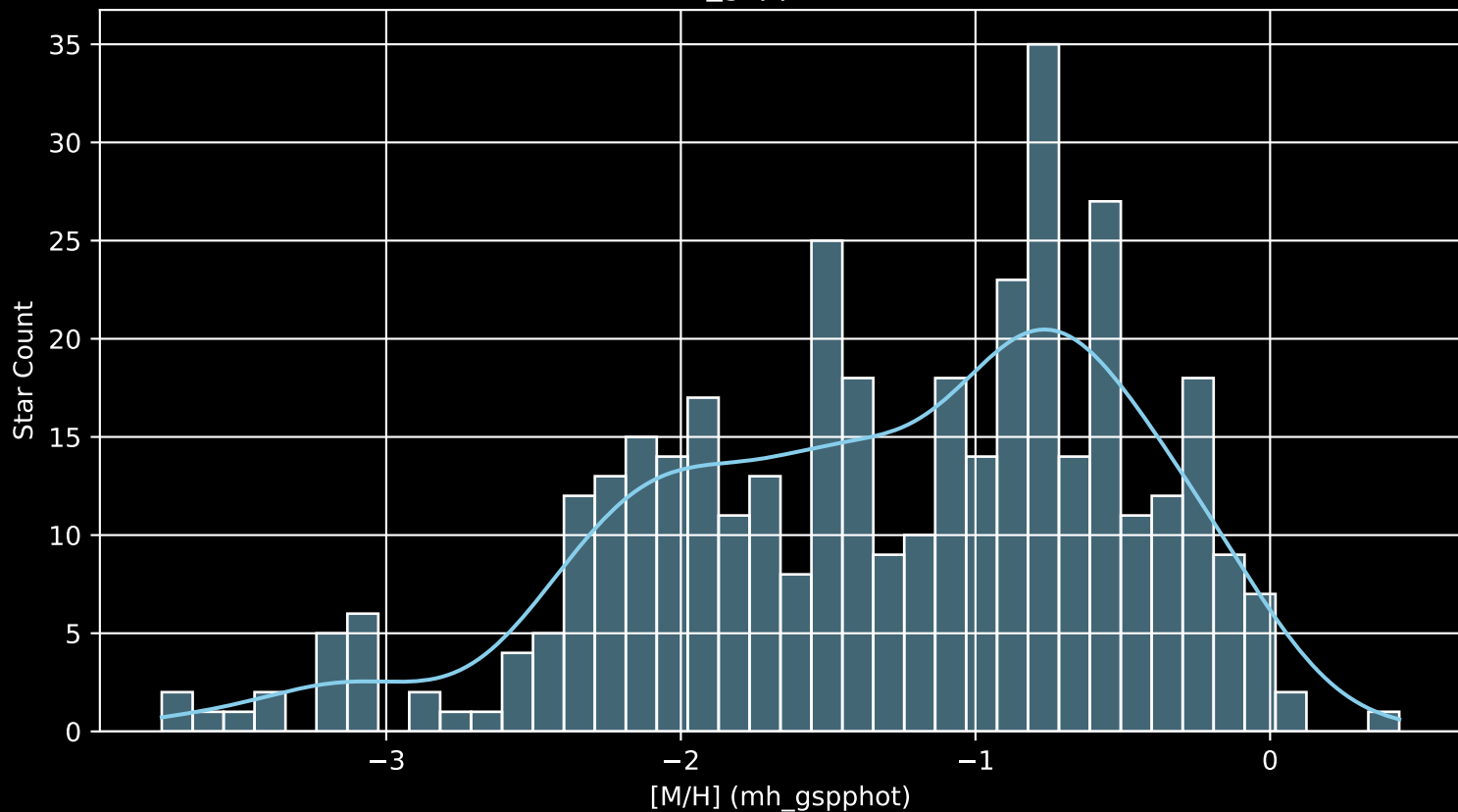
Gaia Cluster: [NGC_2383 [M/H] (mh_gspphot) (n= 386)
