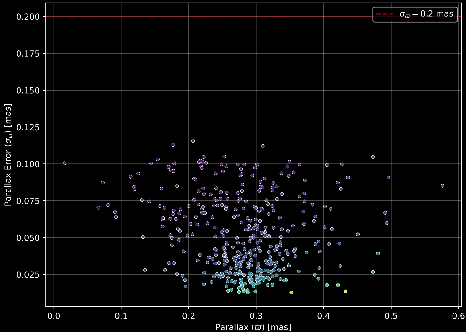
Gaia Cluster: [NGC_2383] Parallax Quality (n= 387)
