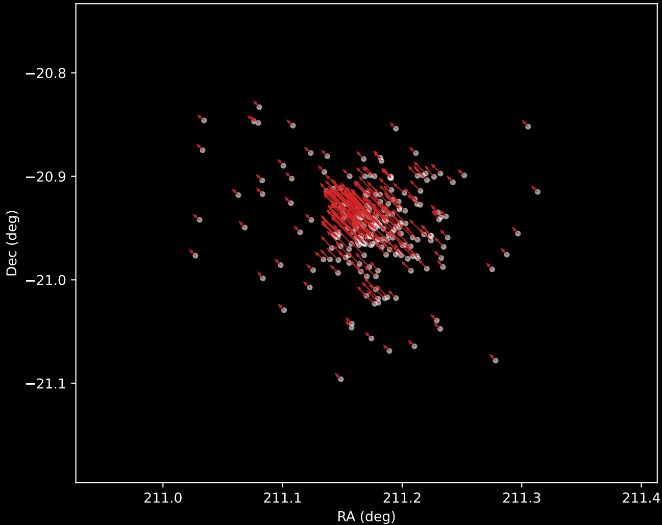
Gaia DR3 Cluster 6 Proper Motion Vectors (n=217)
