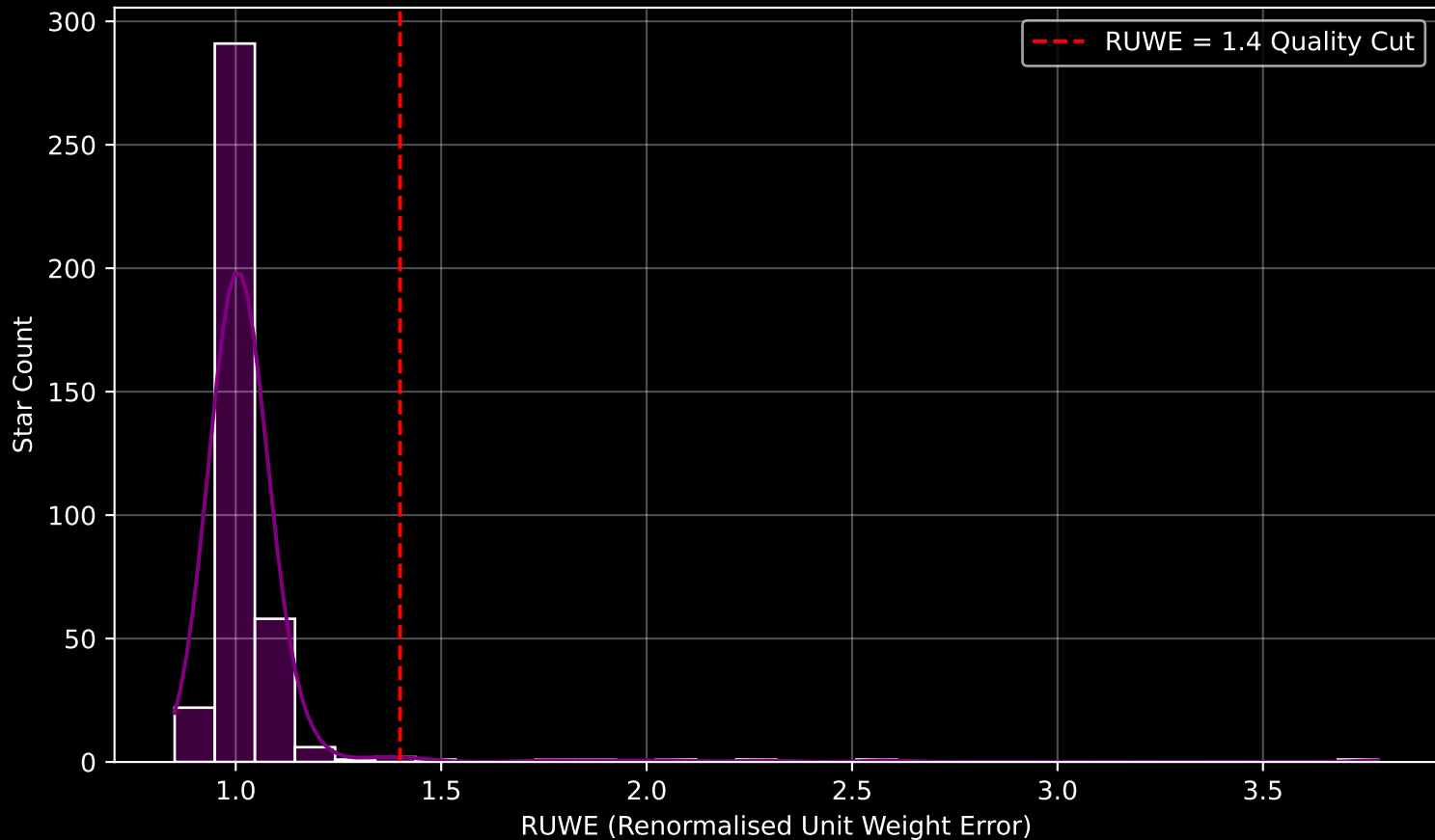
Gaia Cluster: [NGC_2383] RUWE Distribution (n= 387)
