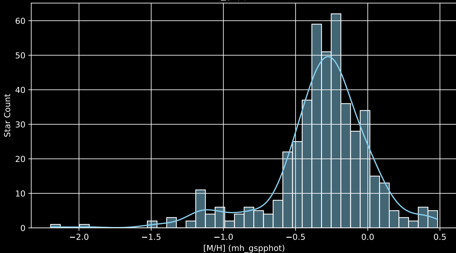
Gaia Cluster: [NGC_2423 [M/H] (mh_gspphot) (n= 462)
