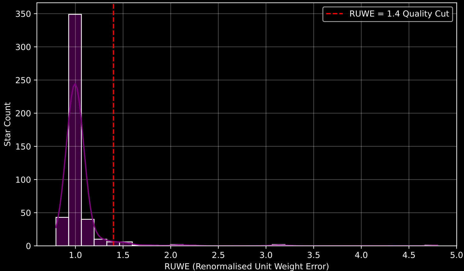
Gaia Cluster: [NGC_2423] RUWE Distribution (n= 462)
