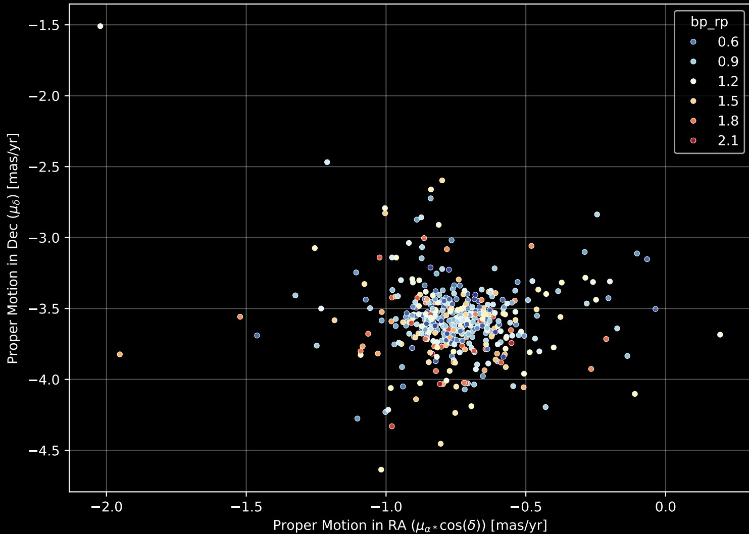
Gaia Cluster: [NGC_2423] Proper Motion Diagram (n= 462)
