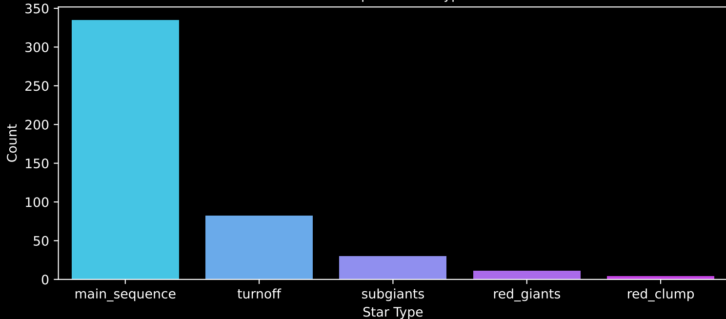
Gaia Cluster: [NGC_2423] Count plot of Star Type
