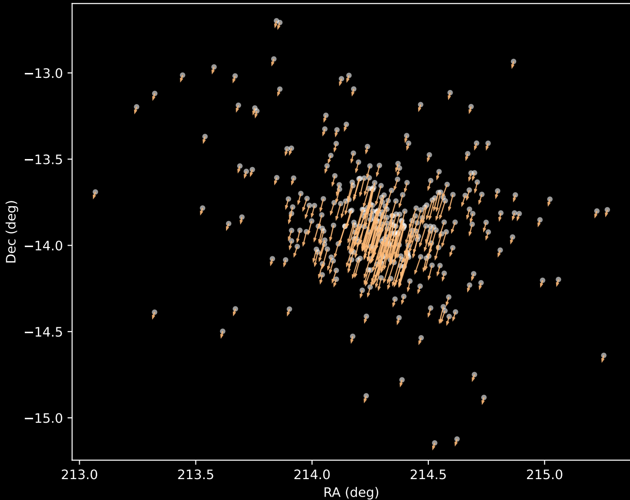
Gaia DR3 Cluster 3 Proper Motion Vectors (n=305)
