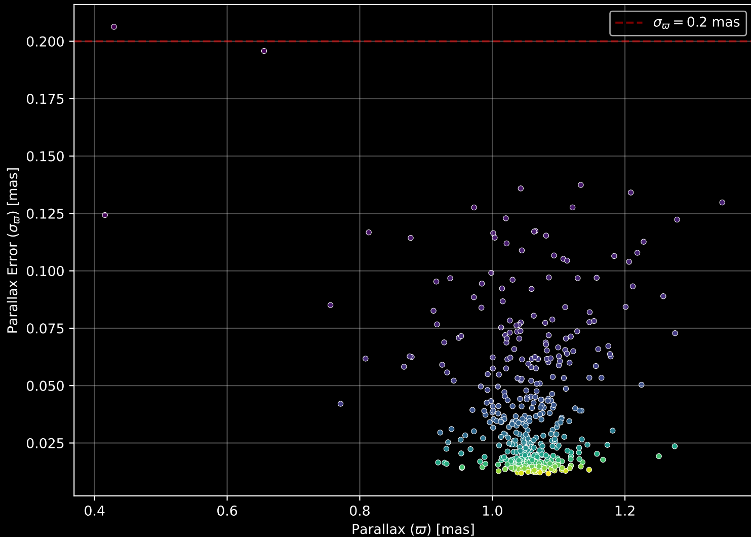
Gaia Cluster: [NGC_2423] Parallax Quality (n= 462)
