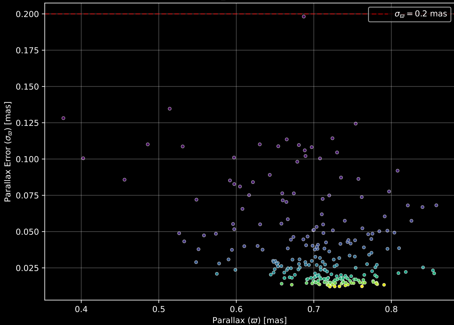
Gaia Cluster: [NGC_2428] Parallax Quality (n= 234)
