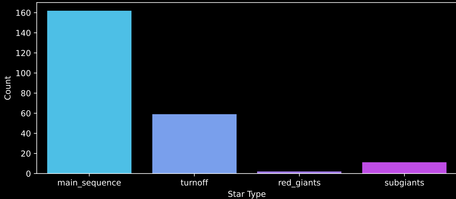
Gaia Cluster: [NGC_2428] Count plot of Star Type
