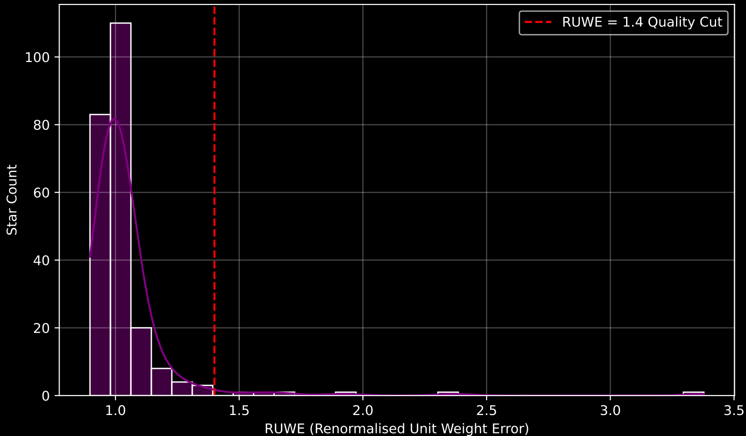
Gaia Cluster: [NGC_2428] RUWE Distribution (n= 234)
