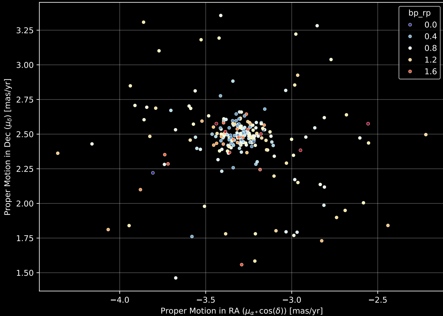
Gaia Cluster: [NGC_2428] Proper Motion Diagram (n= 234)
