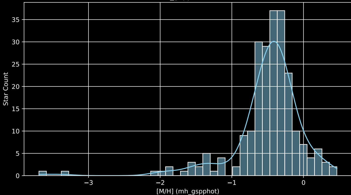
Gaia Cluster: [NGC_2428 [M/H] (mh_gspphot) (n= 231)
