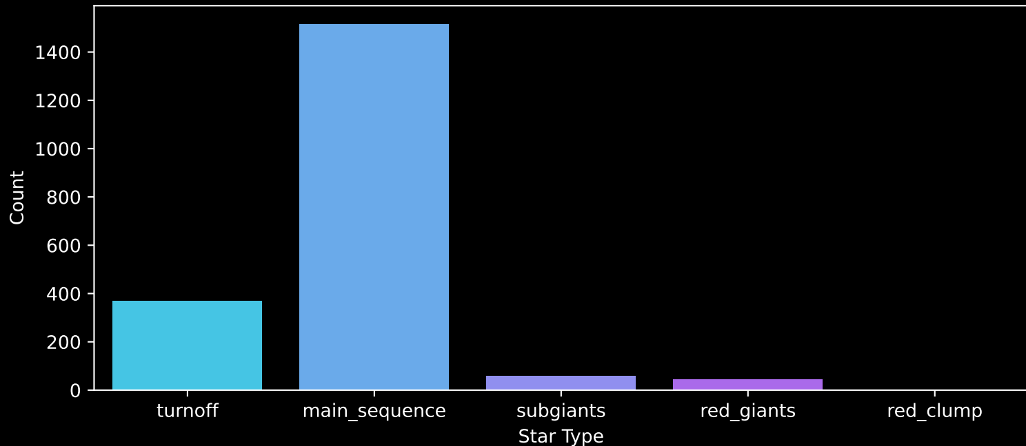
Gaia Cluster: [NGC_2437] Count plot of Star Type
