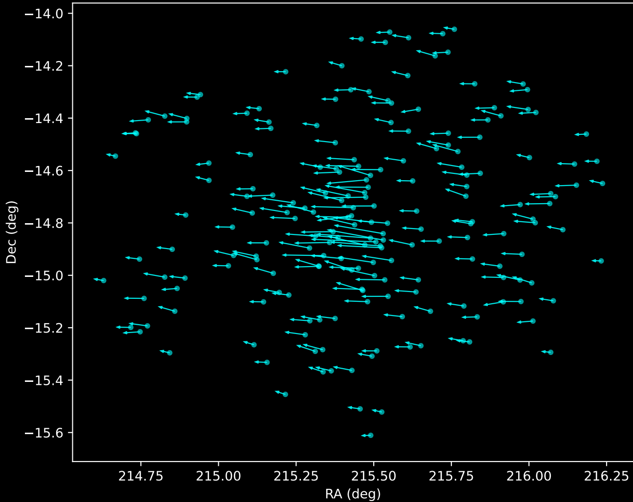
Gaia DR3 Noise Stream Proper Motion Vectors (n=196)
