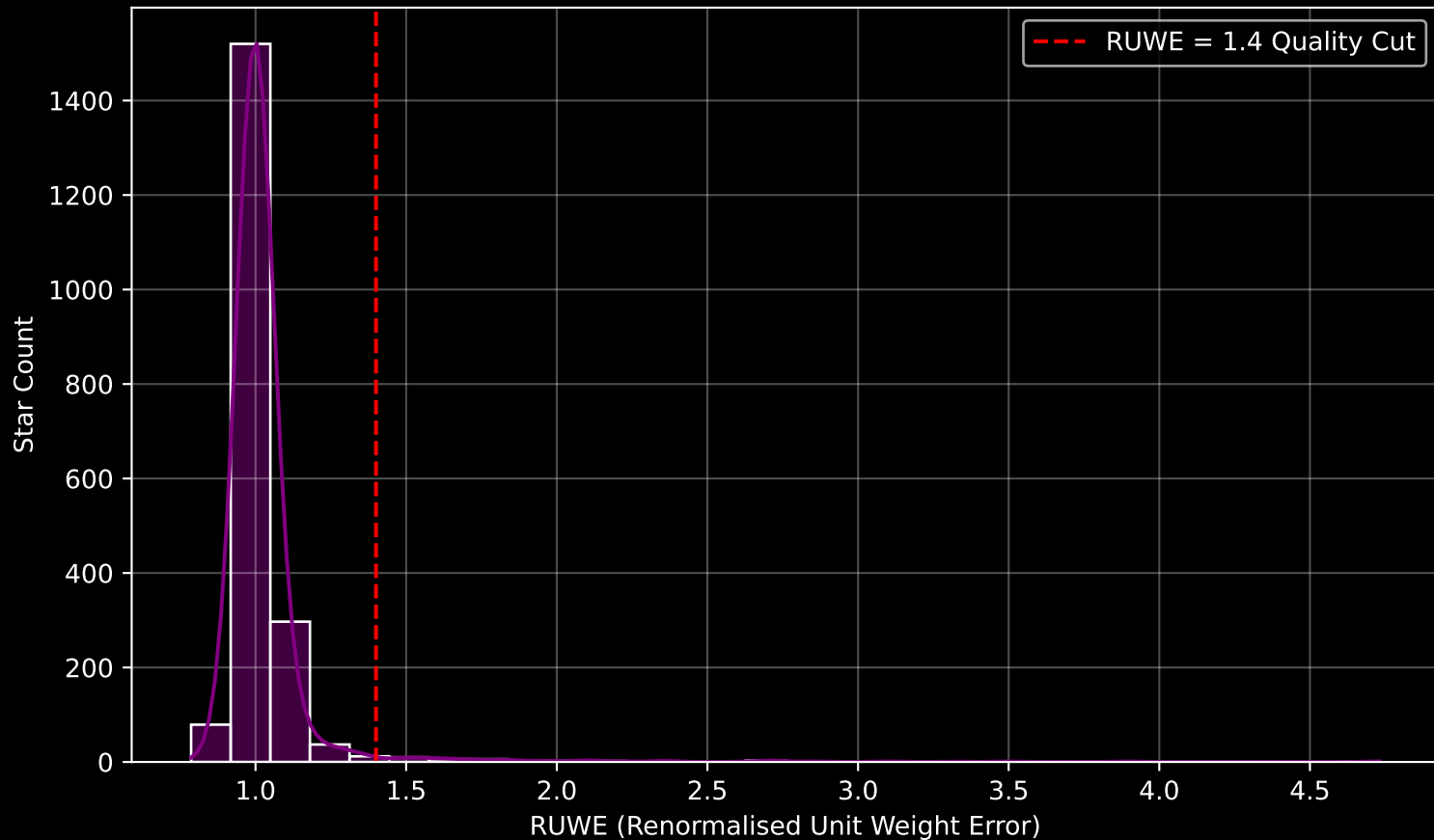
Gaia Cluster: [NGC_2437] RUWE Distribution (n= 1985)
