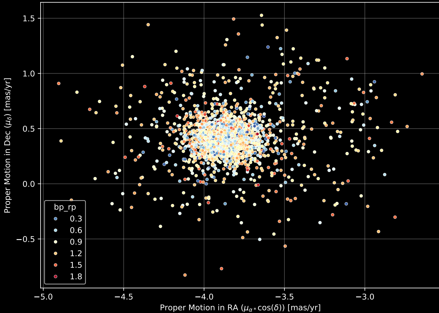
Gaia Cluster: [NGC_2437] Proper Motion Diagram (n= 1988)
