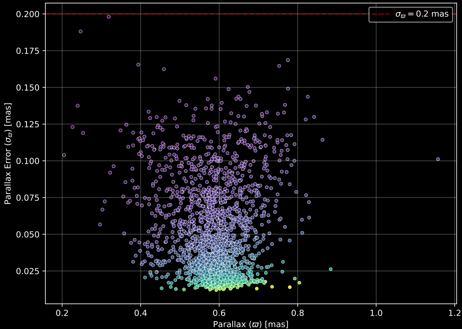
Gaia Cluster: [NGC_2437] Parallax Quality (n= 1988)
