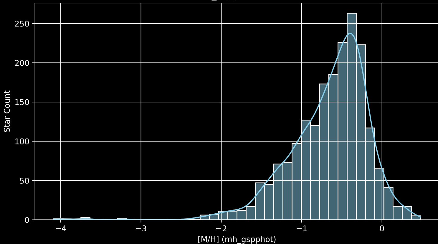
Gaia Cluster: [NGC_2437 [M/H] (mh_gspphot) (n= 1986)
