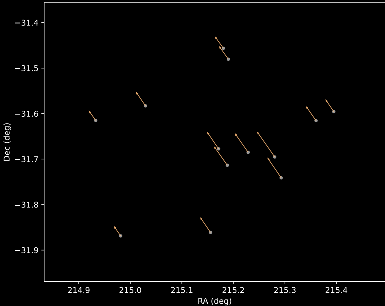
Gaia DR3 Cluster 23 Proper Motion Vectors (n=13)
