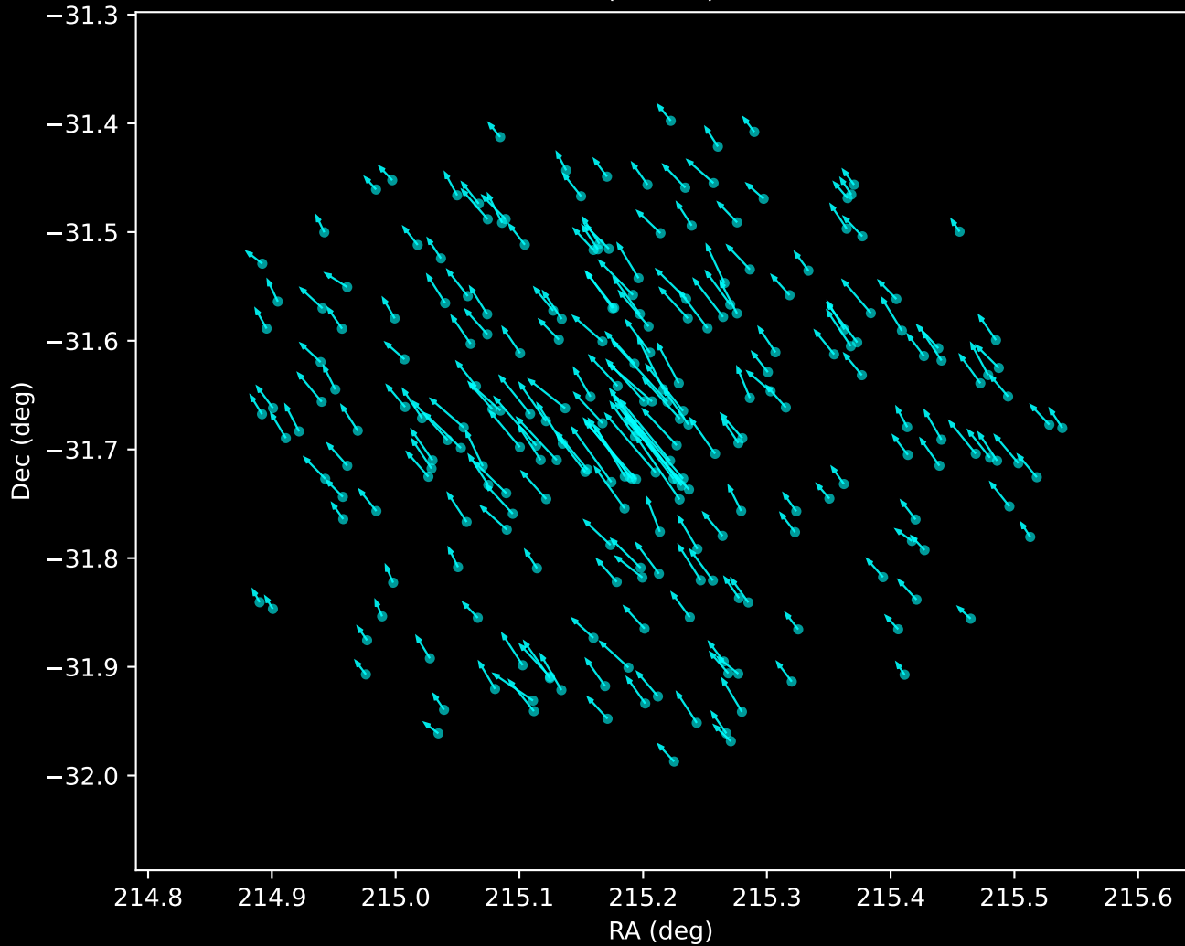
Gaia DR3 Noise Stream Proper Motion Vectors (n=239)
