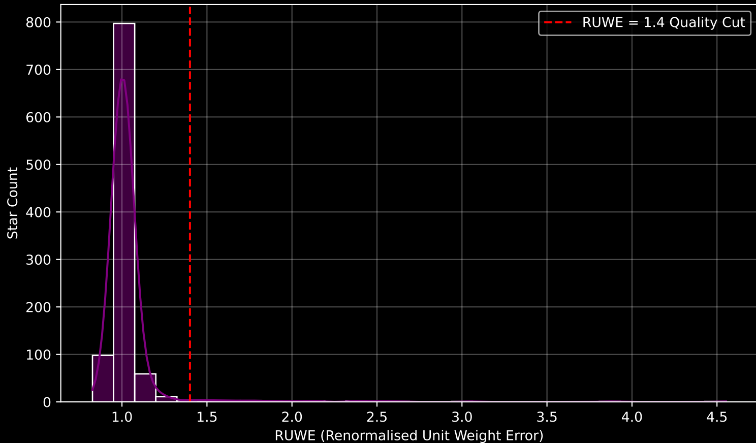
Gaia Cluster: [NGC_2439] RUWE Distribution (n= 989)
