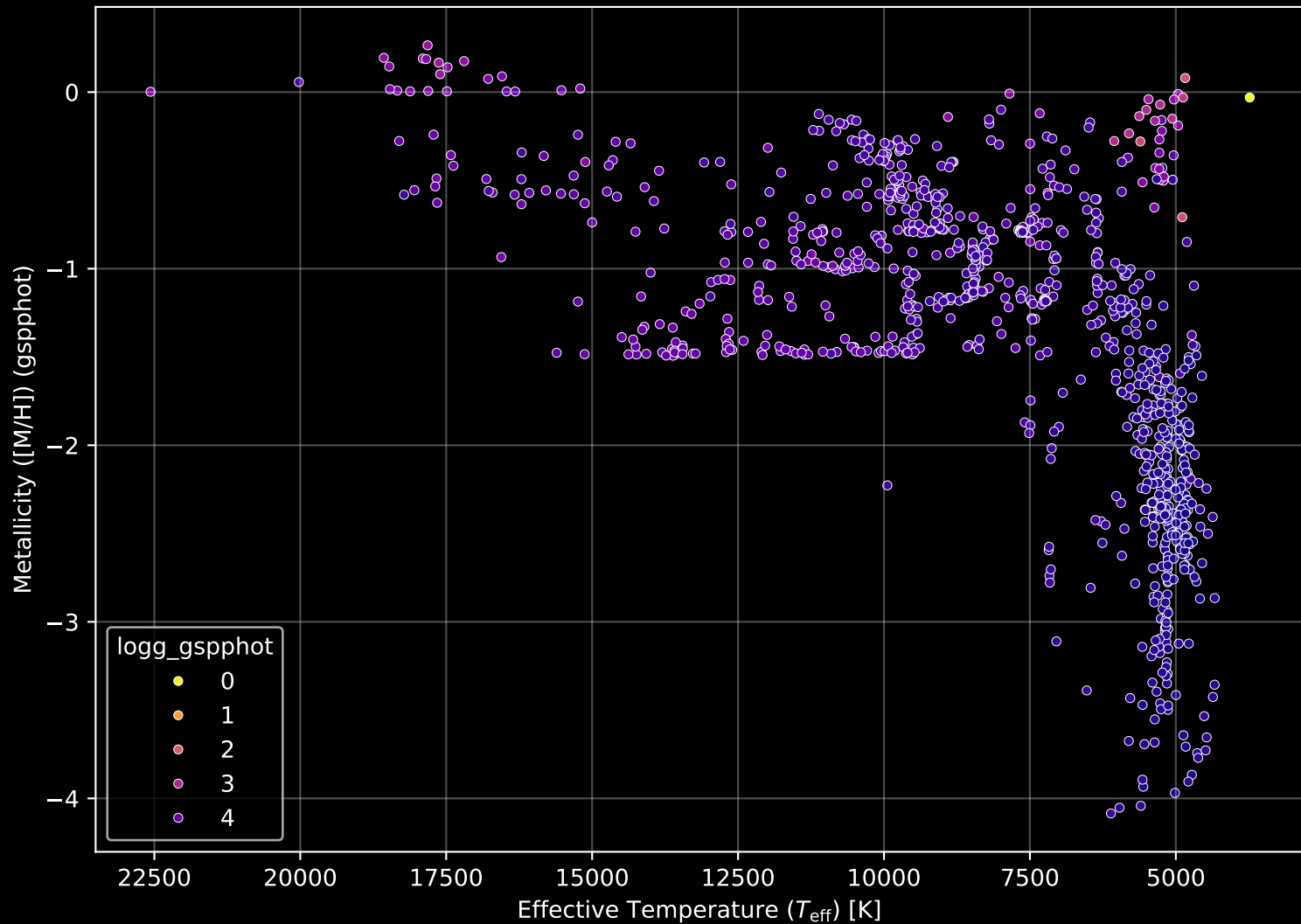
Gaia Cluster: [NGC_2439] Stellar Population Parameters (n= 991)
