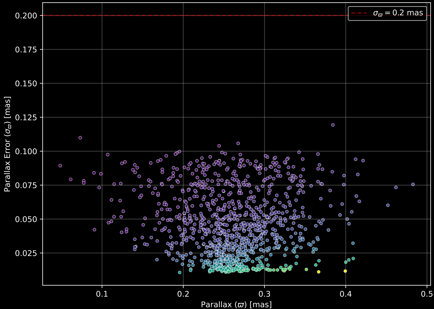
Gaia Cluster: [NGC_2439] Parallax Quality (n= 991)
