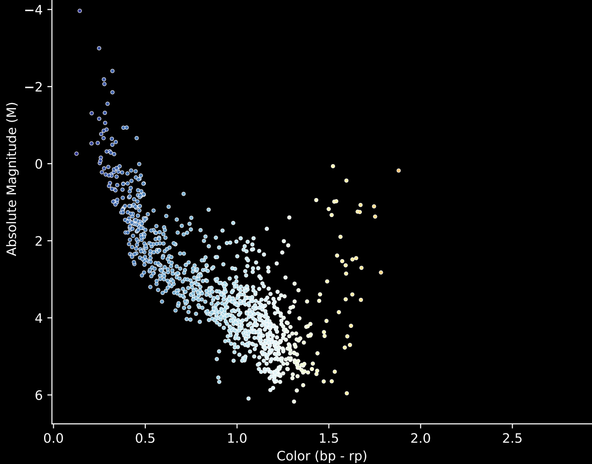
Gaia Cluster: [NGC_2439] Stars (n= 991) Hertzsprung-Russel Diagram
