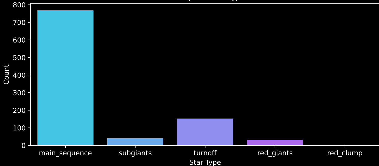
Gaia Cluster: [NGC_2439] Count plot of Star Type
