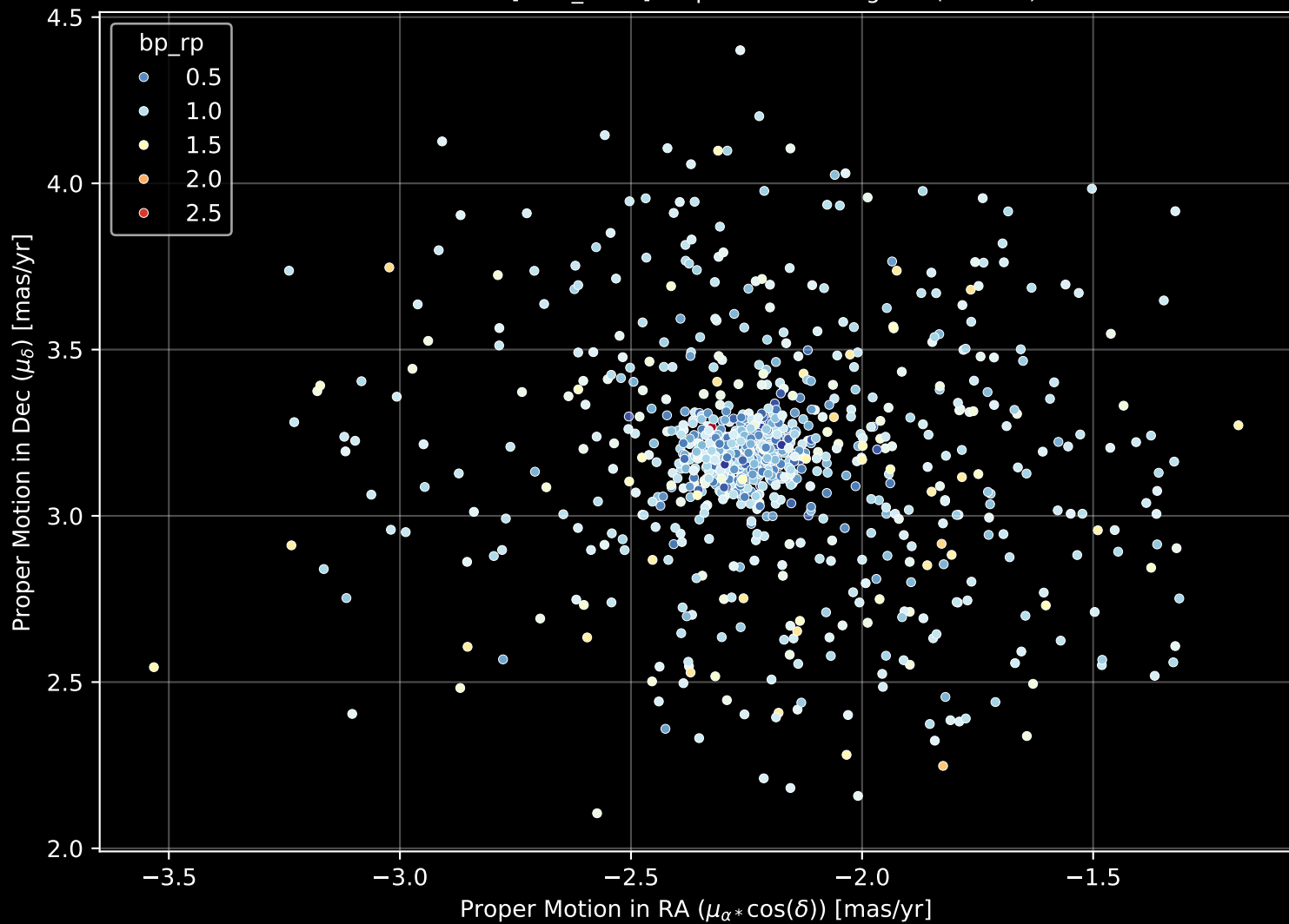
Gaia Cluster: [NGC_2439] Proper Motion Diagram (n= 991)
