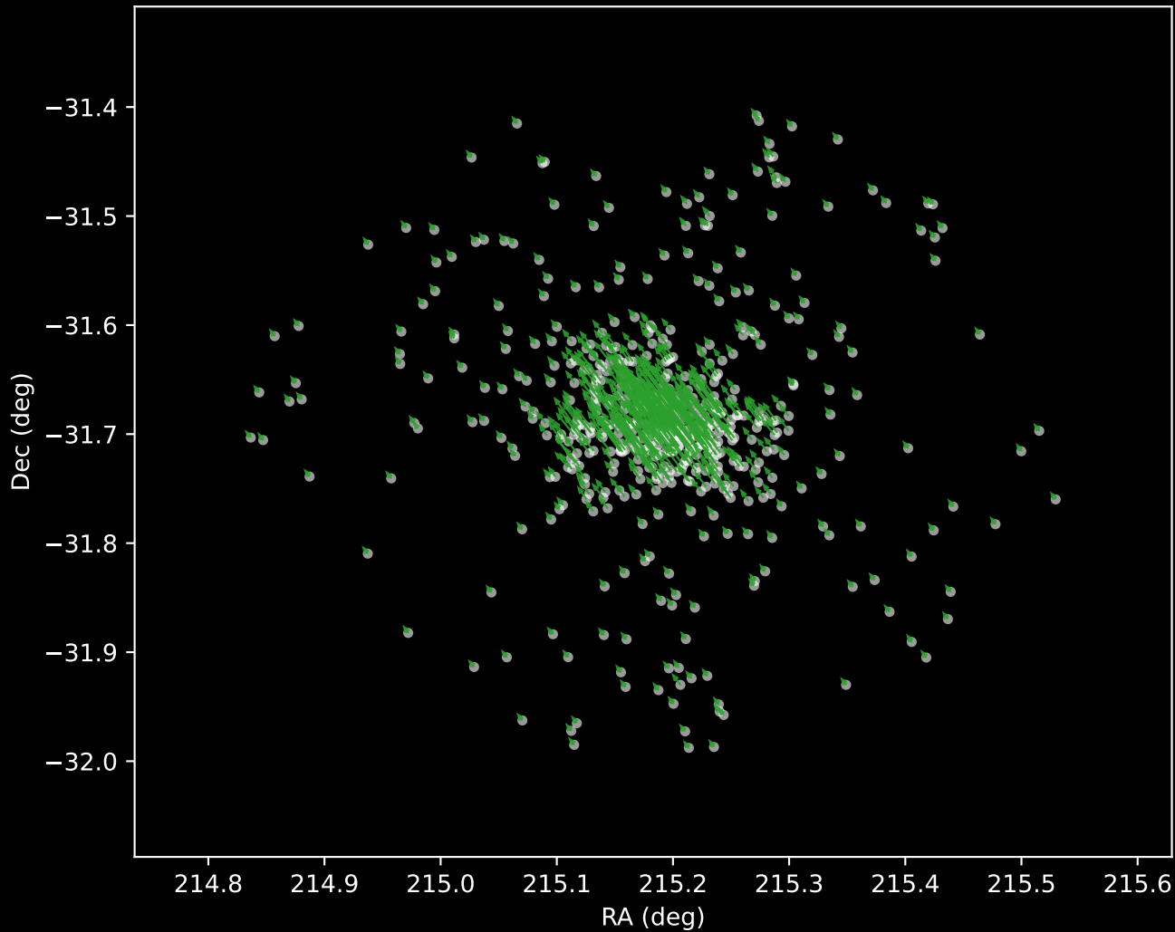
Gaia DR3 Cluster 24 Proper Motion Vectors (n=560)
