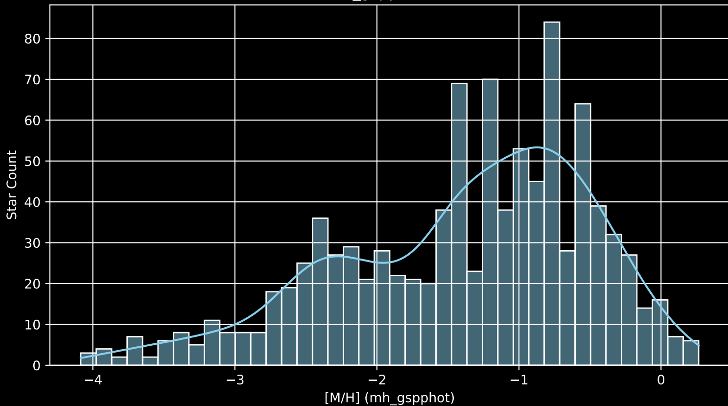
Gaia Cluster: [NGC_2439 [M/H] (mh_gspphot) (n= 991)
