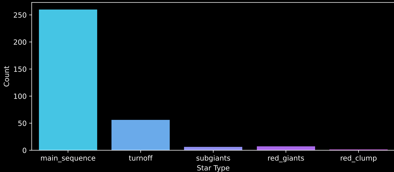
Gaia Cluster: [NGC_2527] Count plot of Star Type
