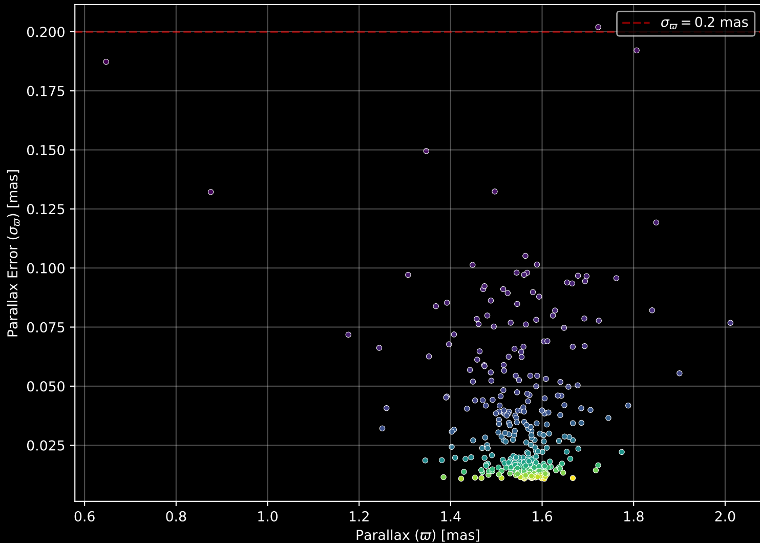
Gaia Cluster: [NGC_2527] Parallax Quality (n= 330)
