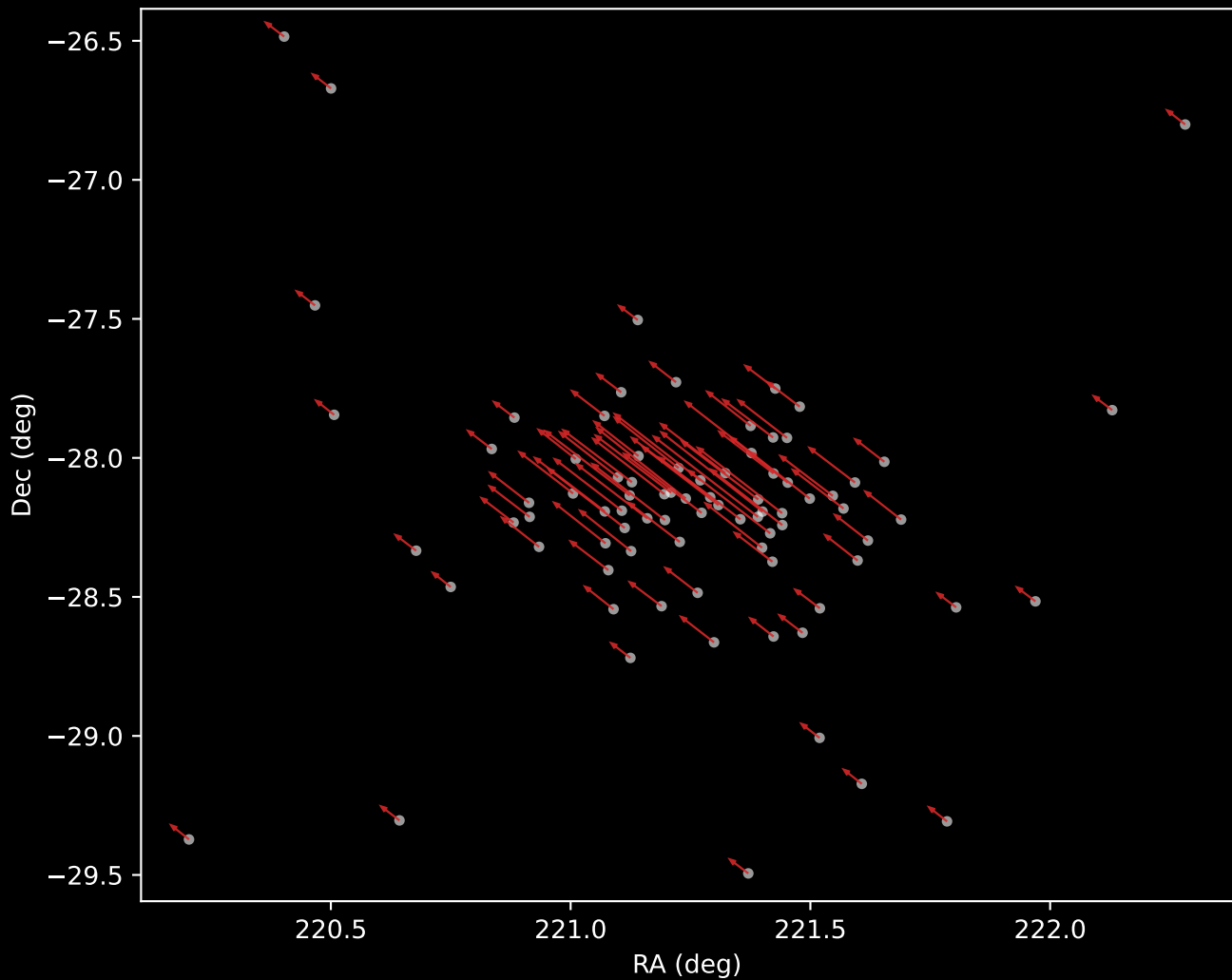
Gaia DR3 Cluster 6 Proper Motion Vectors (n=83)
