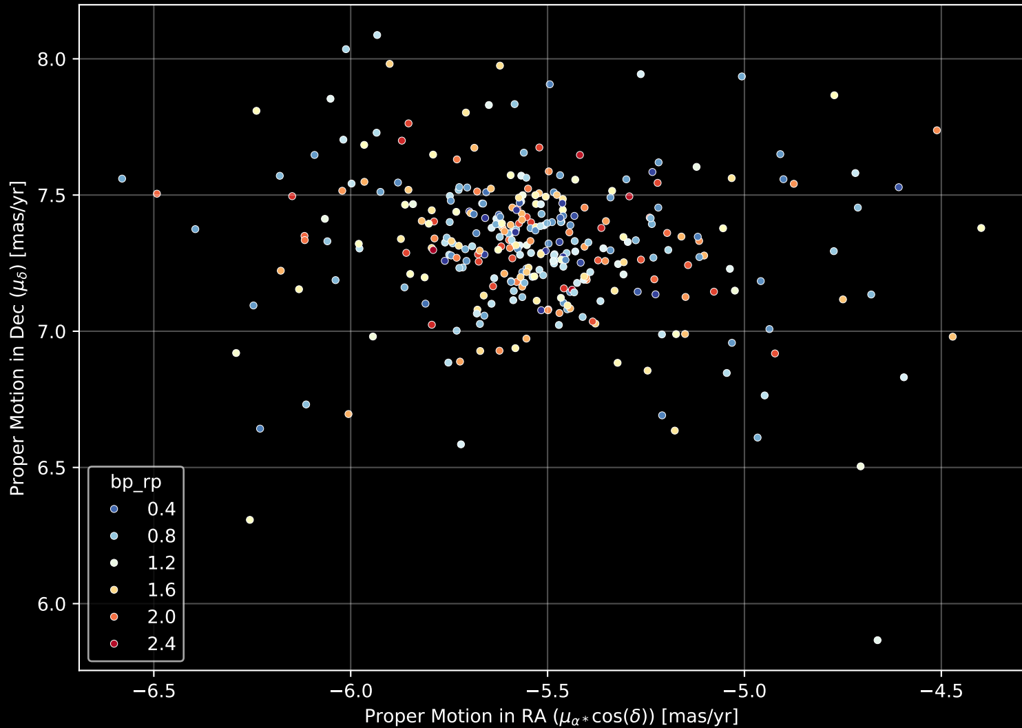
Gaia Cluster: [NGC_2527] Proper Motion Diagram (n= 330)
