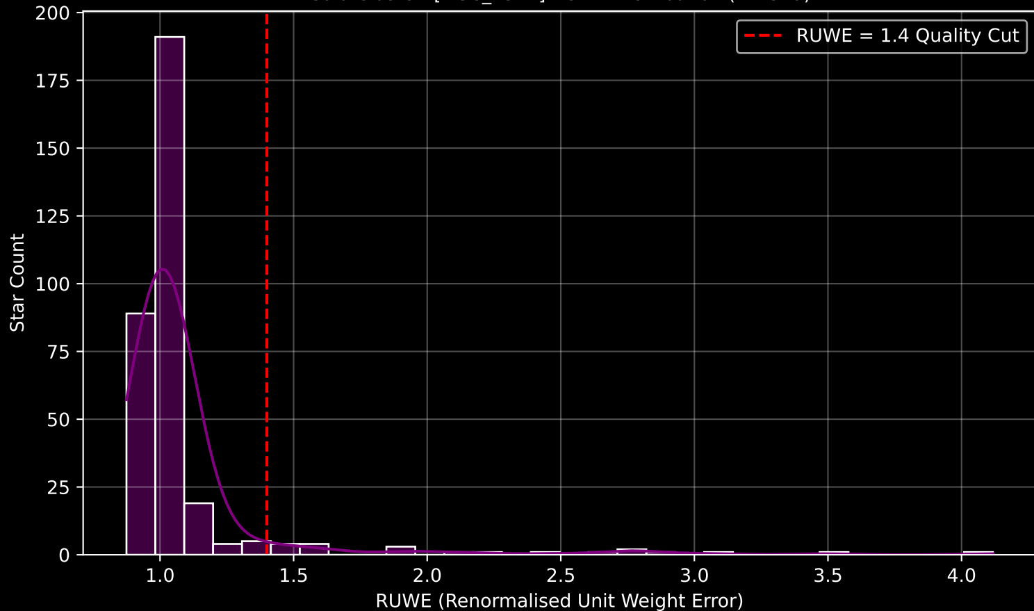
Gaia Cluster: [NGC_2527] RUWE Distribution (n= 329)
