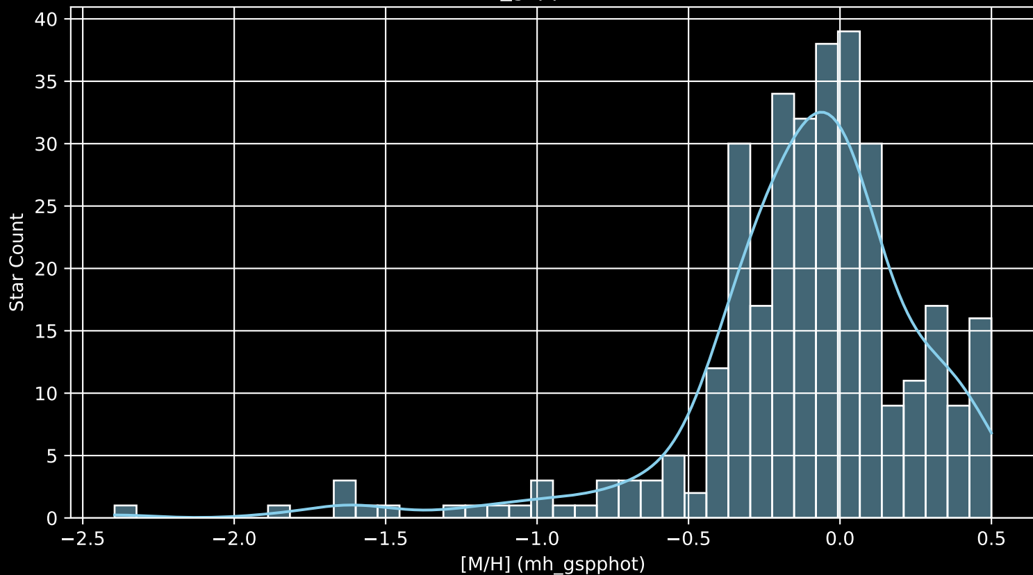
Gaia Cluster: [NGC_2527 [M/H] (mh_gspphot) (n= 326)
