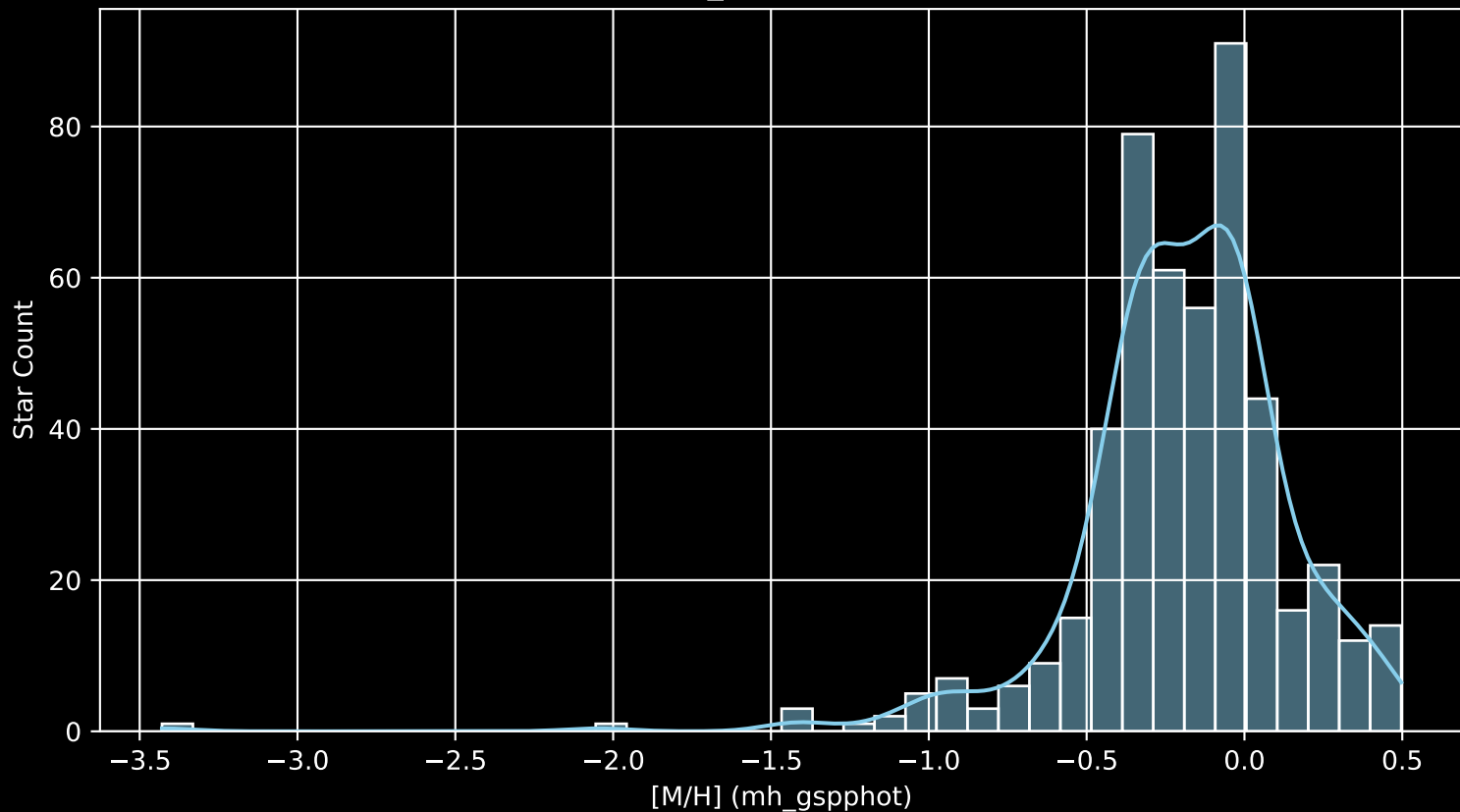
Gaia Cluster: [NGC_2548 [M/H] (mh_gspphot) (n= 488)
