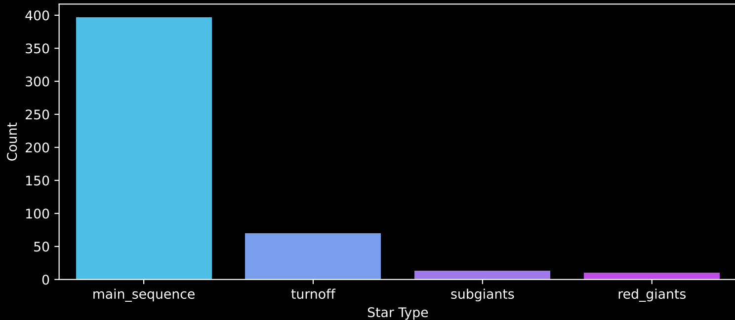
Gaia Cluster: [NGC_2548] Count plot of Star Type
