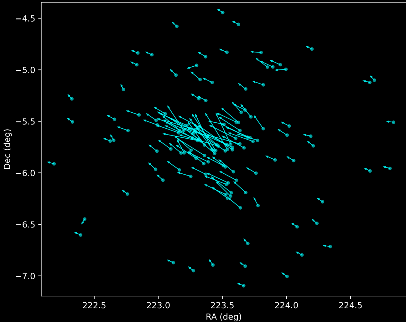
Gaia DR3 Noise Stream Proper Motion Vectors (n=129)
