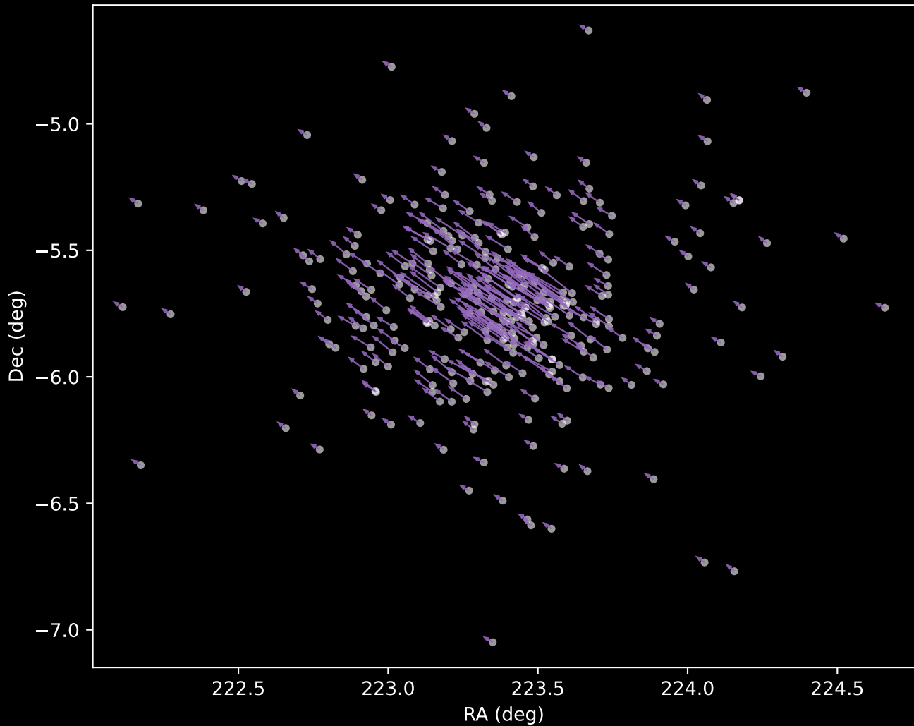
Gaia DR3 Cluster 8 Proper Motion Vectors (n=299)
