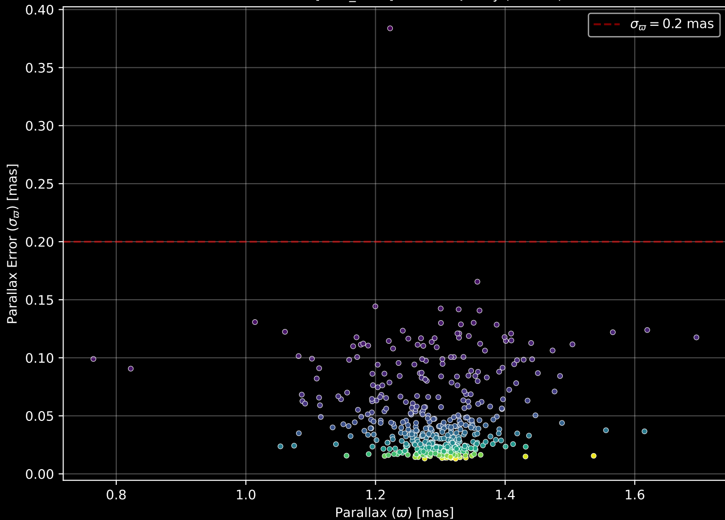
Gaia Cluster: [NGC_2548] Parallax Quality (n= 490)
