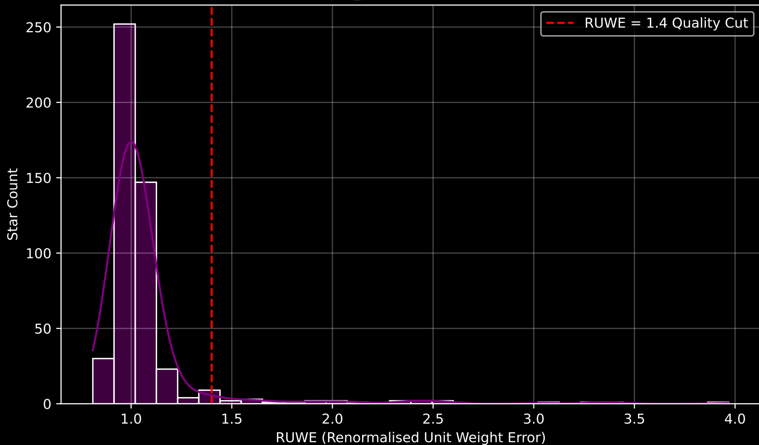
Gaia Cluster: [NGC_2548] RUWE Distribution (n= 487)
