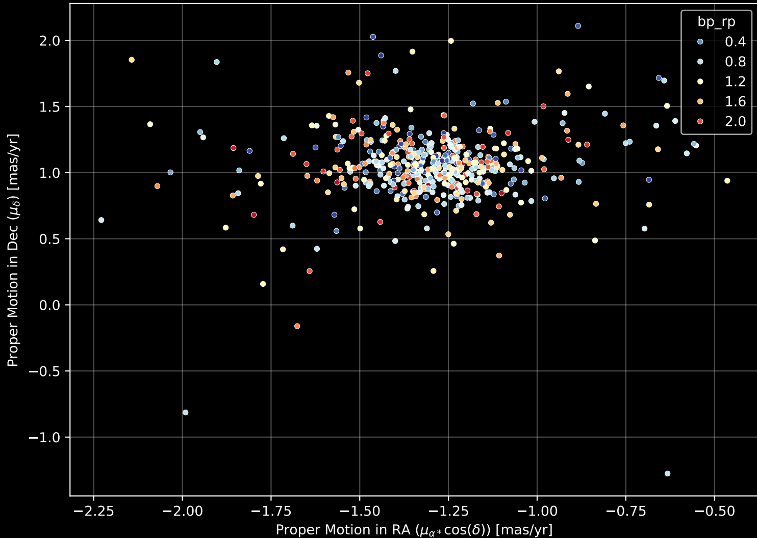
Gaia Cluster: [NGC_2548] Proper Motion Diagram (n= 490)
