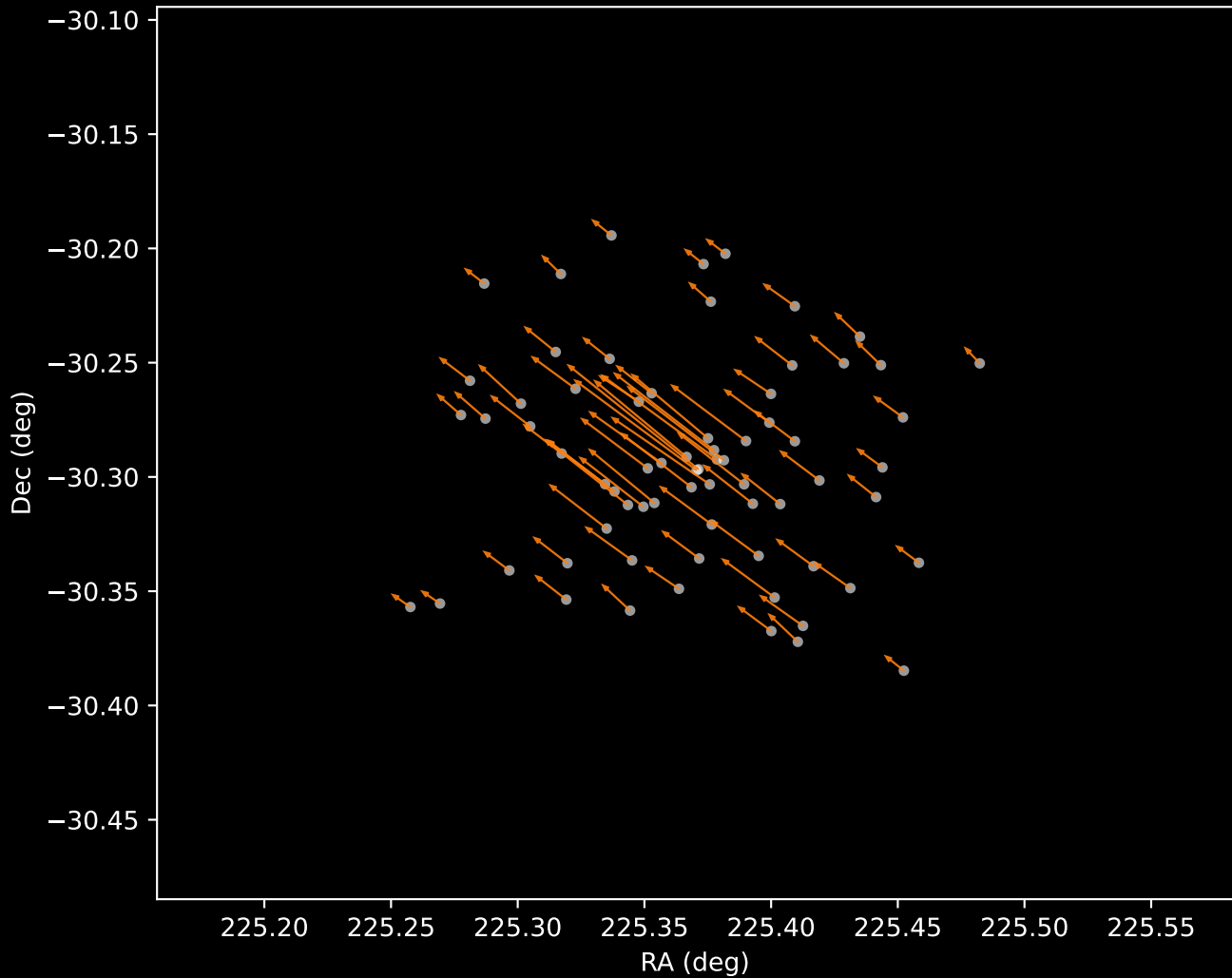
Gaia DR3 Cluster 2 Proper Motion Vectors (n=70)
