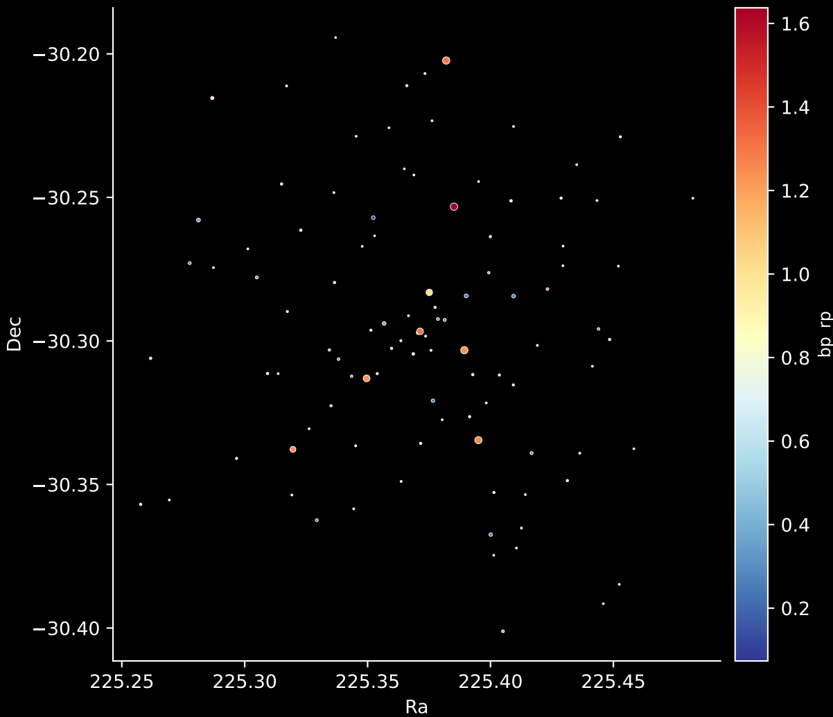
Gaia Cluster: [NGC_2580] Stars: 101
