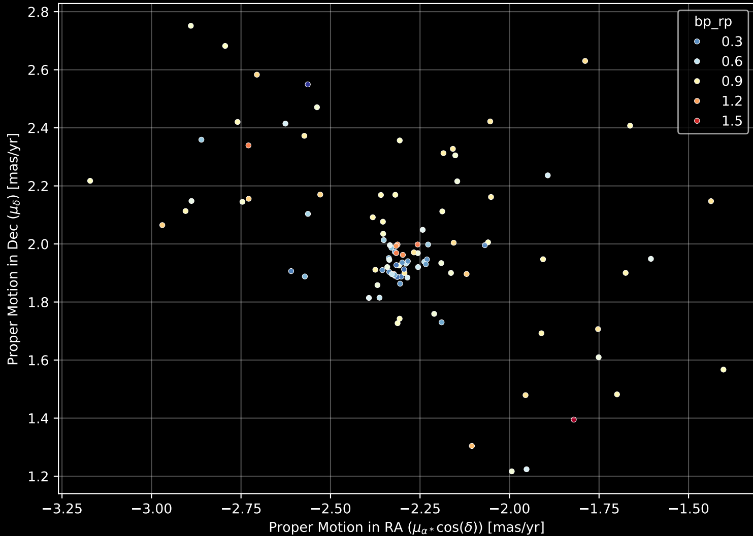
Gaia Cluster: [NGC_2580] Proper Motion Diagram (n= 101)
