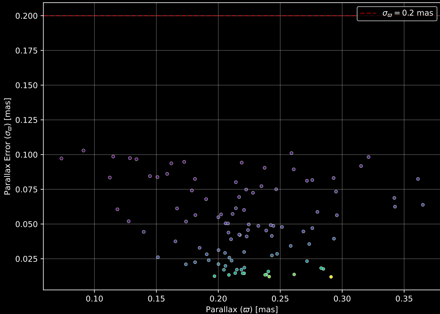
Gaia Cluster: [NGC_2580] Parallax Quality (n= 101)
