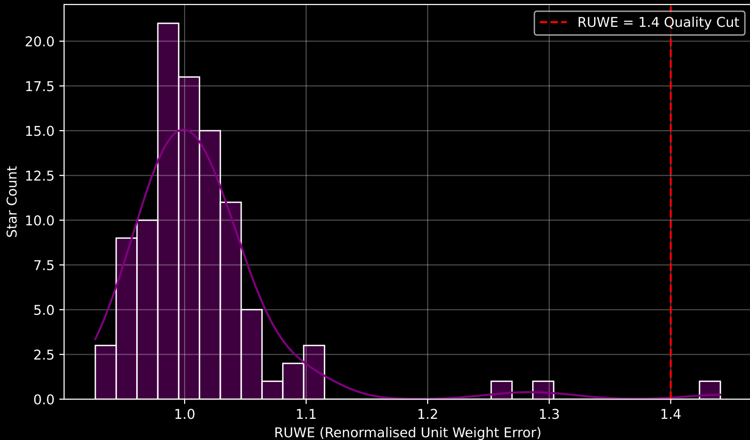
Gaia Cluster: [NGC_2580] RUWE Distribution (n= 101)
