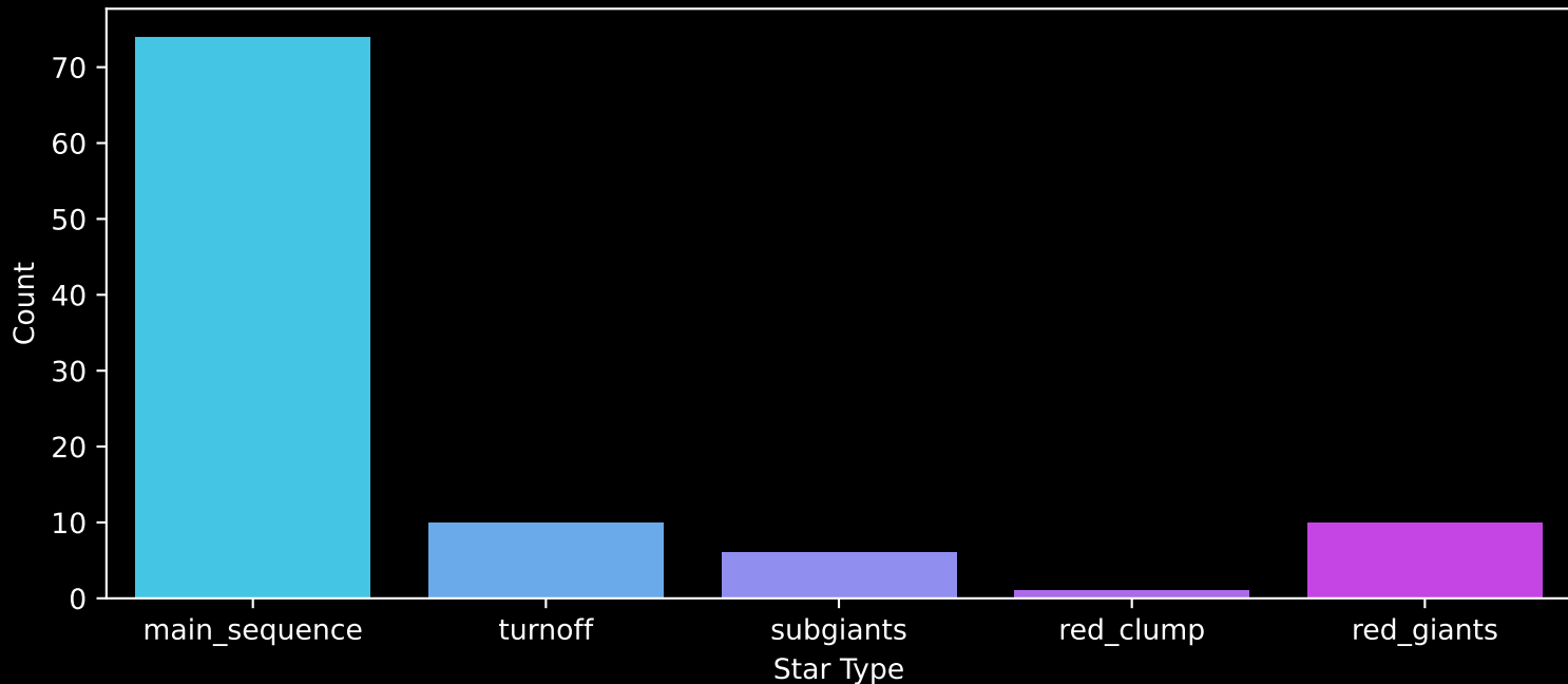
Gaia Cluster: [NGC_2580] Count plot of Star Type
