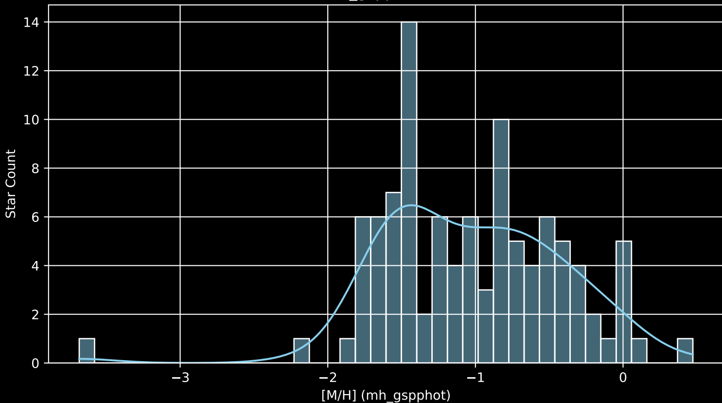
Gaia Cluster: [NGC_2580 [M/H] (mh_gspphot) (n= 101)
