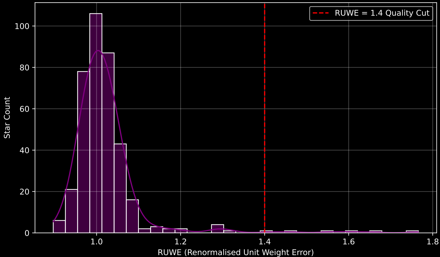
Gaia Cluster: [NGC_2587] RUWE Distribution (n= 377)
