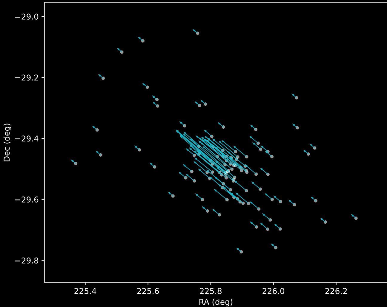
Gaia DR3 Cluster 18 Proper Motion Vectors (n=101)
