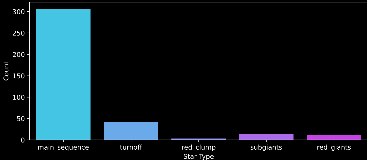
Gaia Cluster: [NGC_2587] Count plot of Star Type
