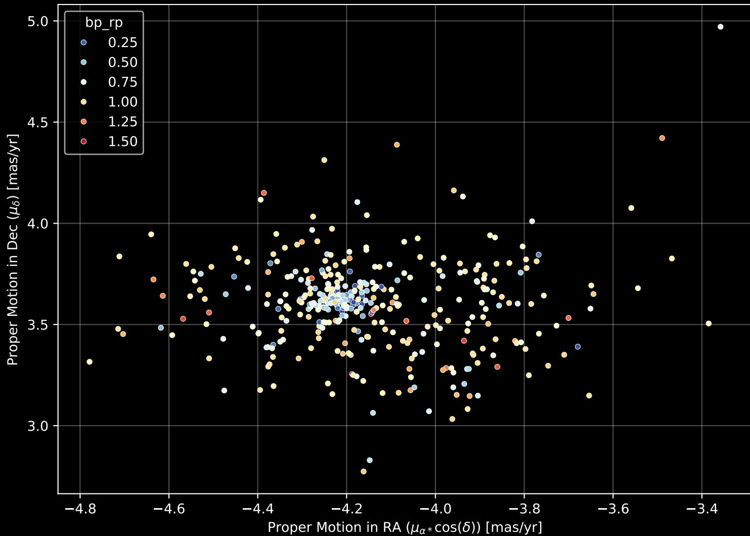
Gaia Cluster: [NGC_2587] Proper Motion Diagram (n= 377)
