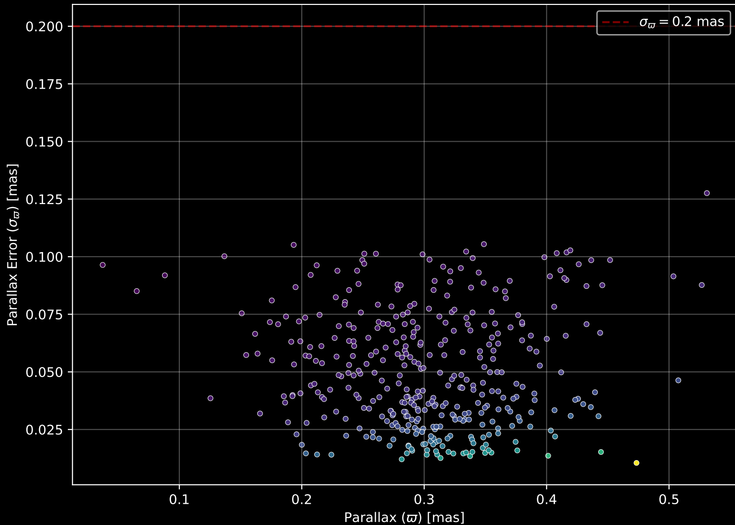
Gaia Cluster: [NGC_2587] Parallax Quality (n= 377)
