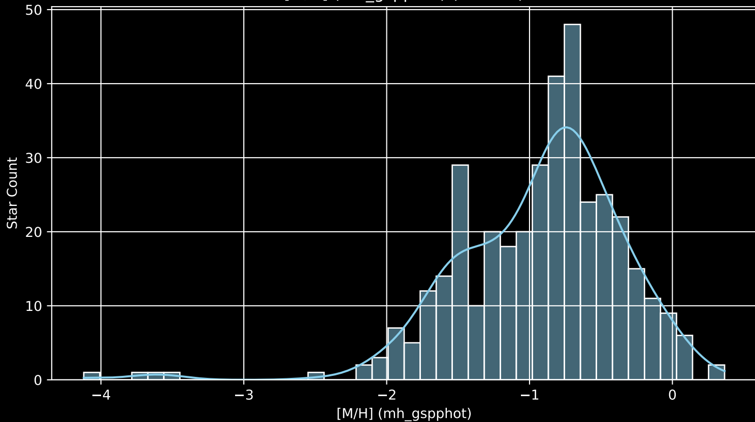
Gaia Cluster: [NGC_2587 [M/H] (mh_gspphot) (n= 377)
