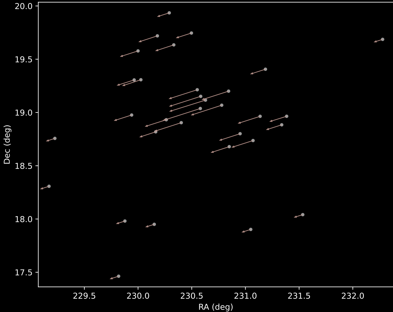
Gaia DR3 Cluster 11 Proper Motion Vectors (n=32)
