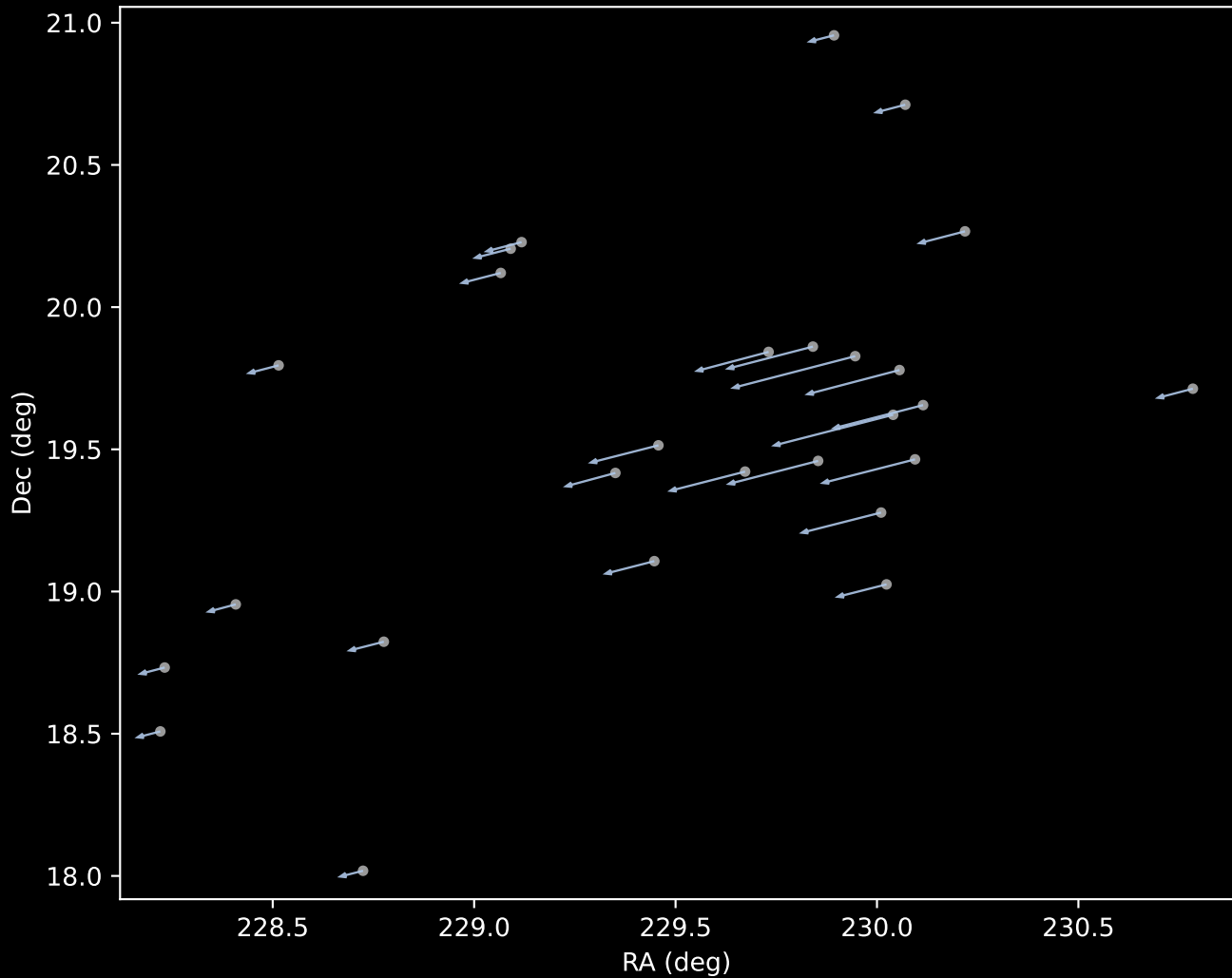
Gaia DR3 Cluster 21 Proper Motion Vectors (n=27)
