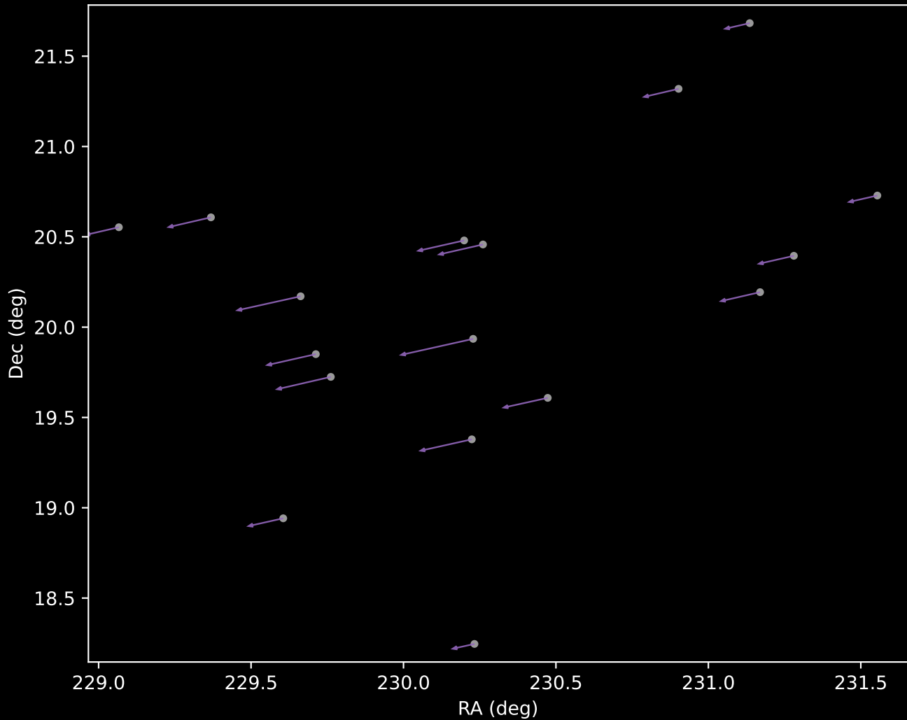
Gaia DR3 Cluster 8 Proper Motion Vectors (n=17)
