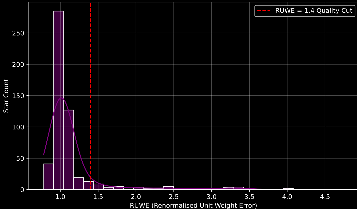
Gaia Cluster: [NGC_2632] RUWE Distribution (n= 537)
