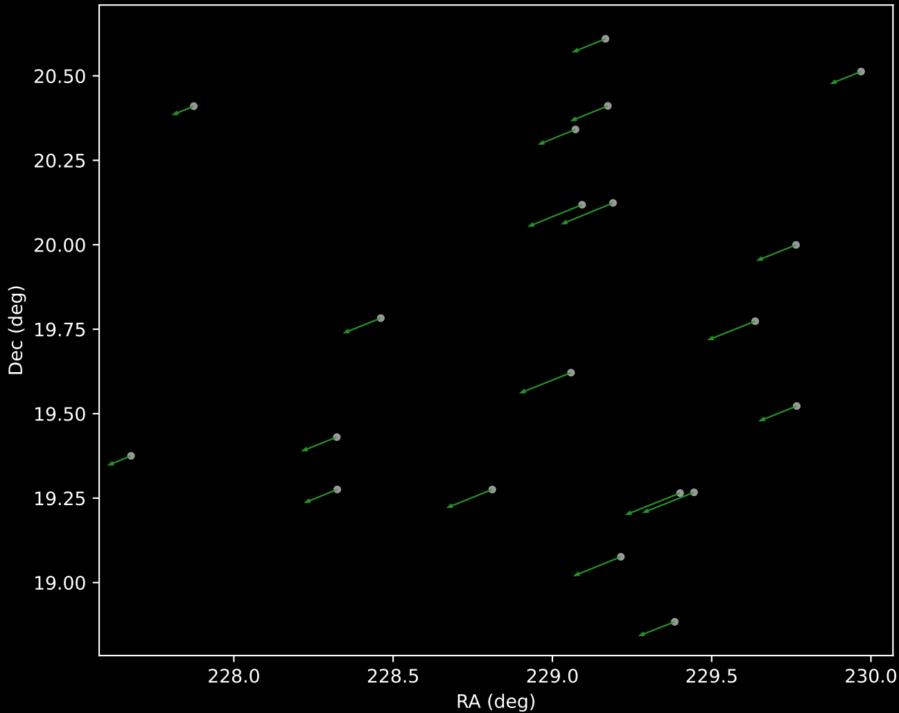
Gaia DR3 Cluster 4 Proper Motion Vectors (n=20)
