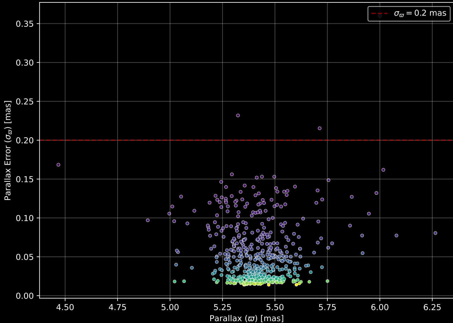
Gaia Cluster: [NGC_2632] Parallax Quality (n= 545)
