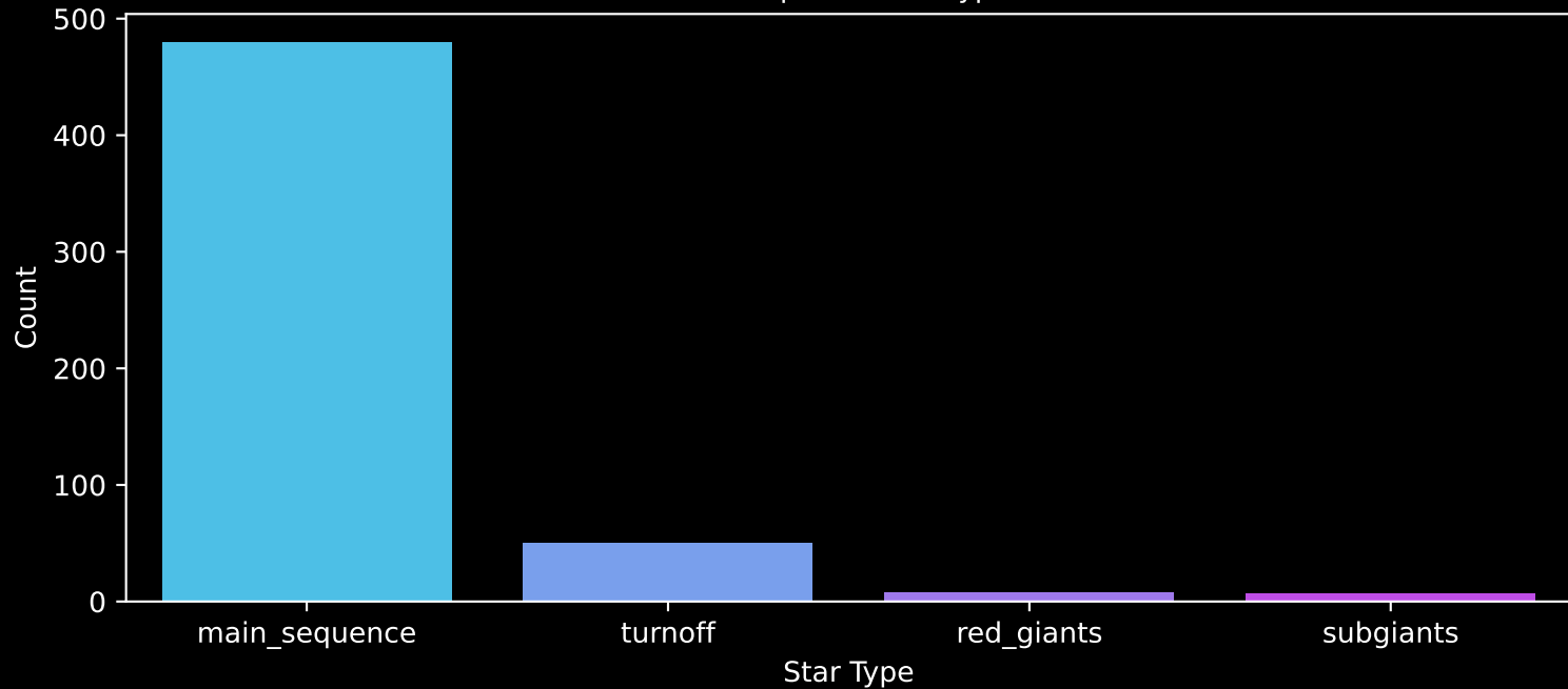
Gaia Cluster: [NGC_2632] Count plot of Star Type
