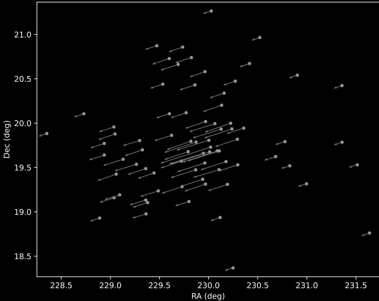
Gaia DR3 Cluster 14 Proper Motion Vectors (n=75)
