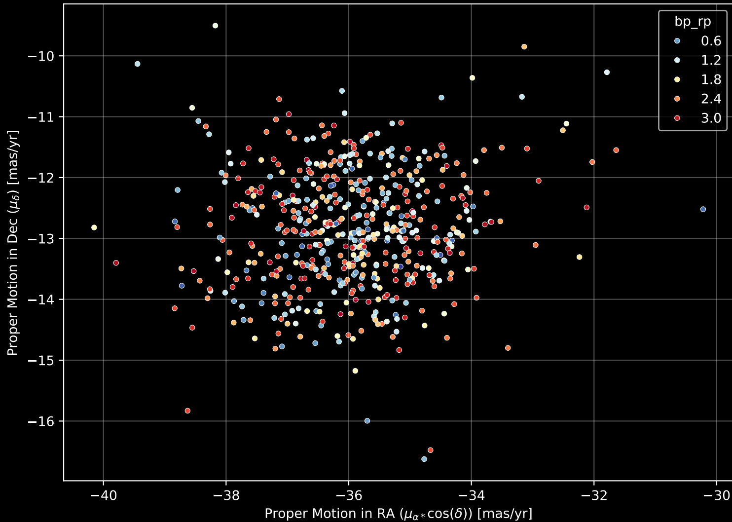
Gaia Cluster: [NGC_2632] Proper Motion Diagram (n= 545)
