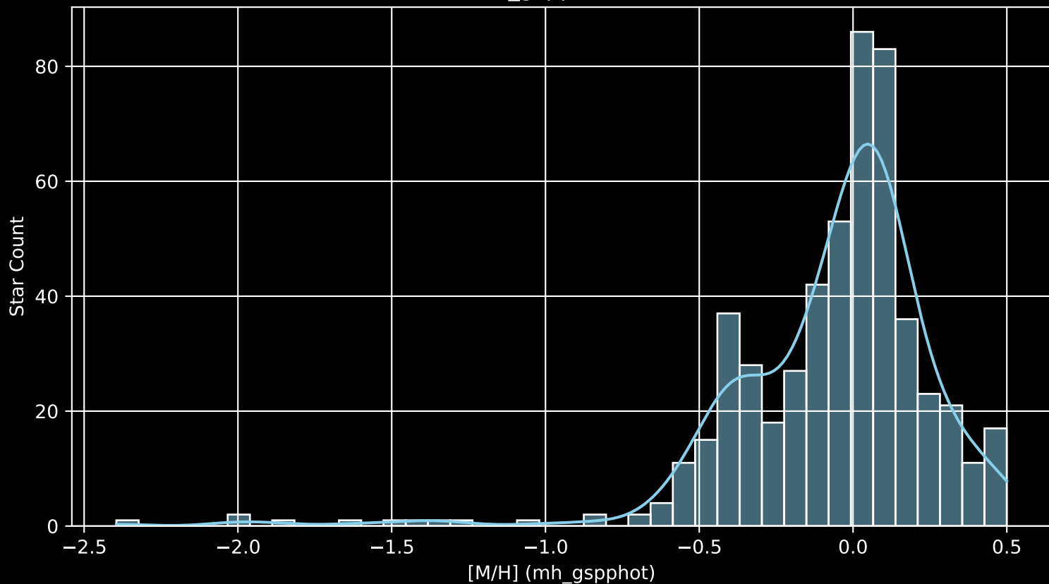
Gaia Cluster: [NGC_2632 [M/H] (mh_gspphot) (n= 526)
