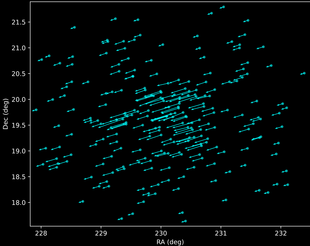
Gaia DR3 Noise Stream Proper Motion Vectors (n=215)
