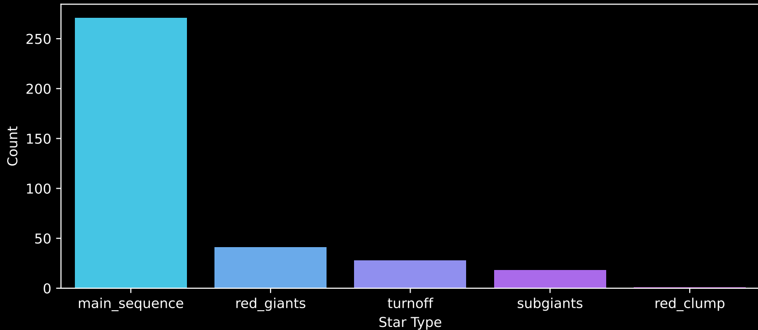
Gaia Cluster: [NGC_2635] Count plot of Star Type
