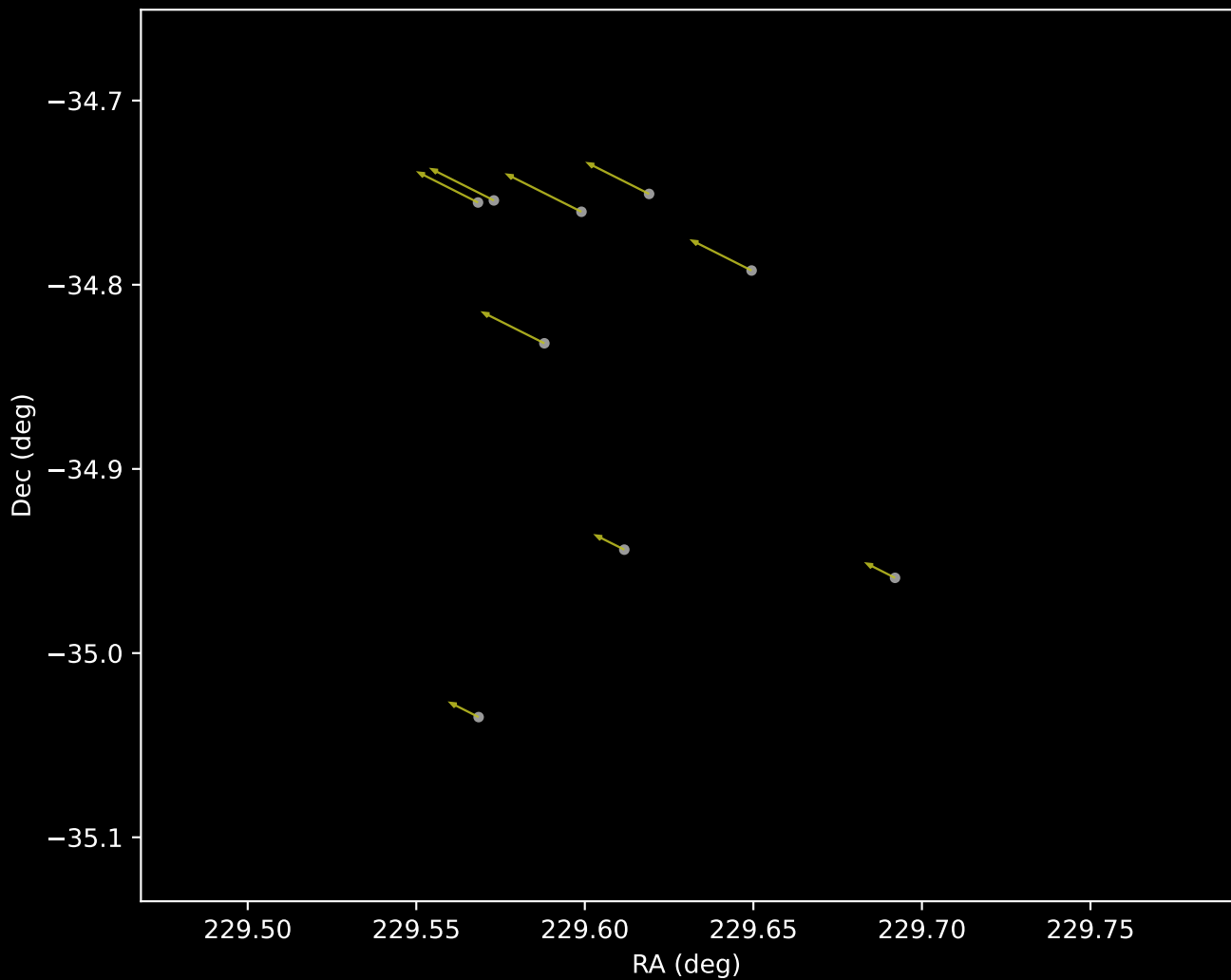
Gaia DR3 Cluster 16 Proper Motion Vectors (n=9)
