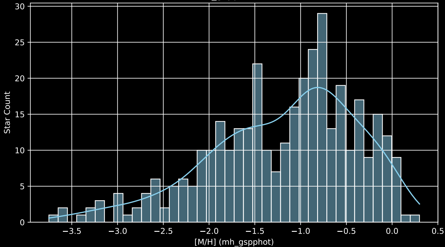
Gaia Cluster: [NGC_2635 [M/H] (mh_gspphot) (n= 359)
