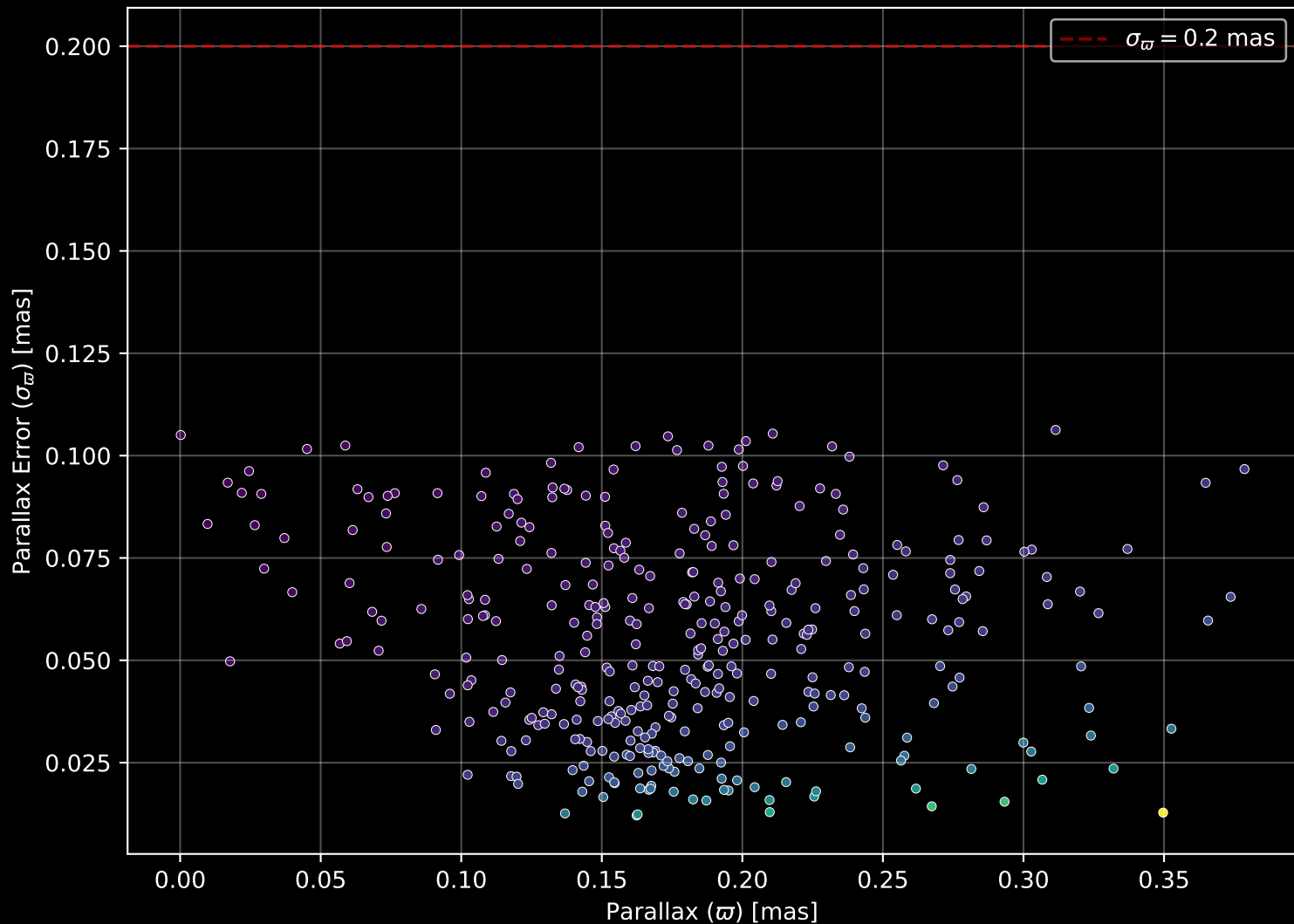
Gaia Cluster: [NGC_2635] Parallax Quality (n= 359)
