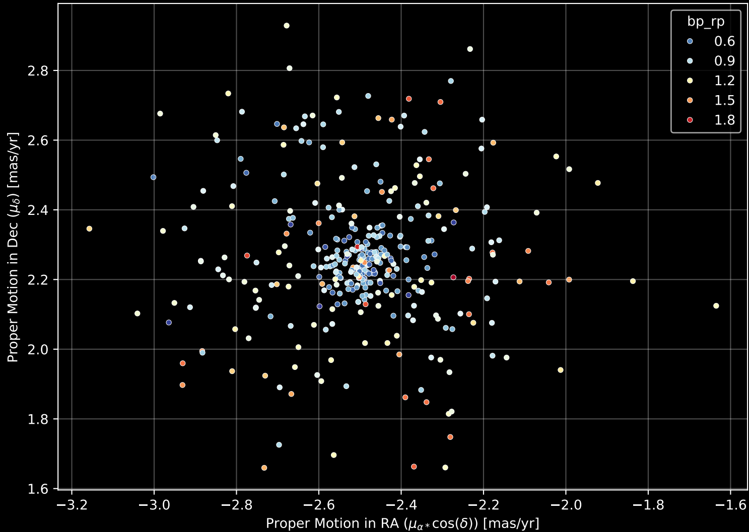
Gaia Cluster: [NGC_2635] Proper Motion Diagram (n= 359)
