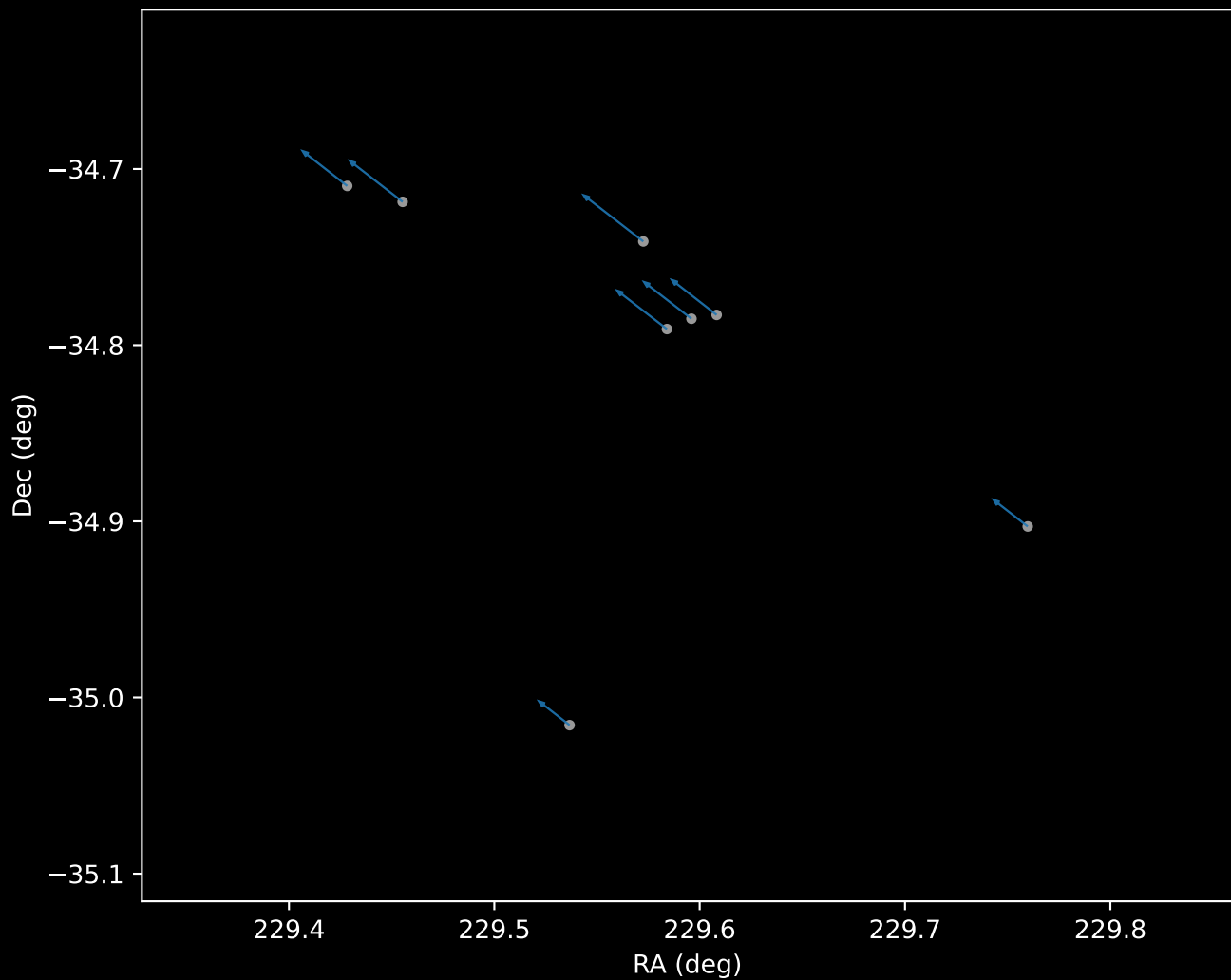
Gaia DR3 Cluster 20 Proper Motion Vectors (n=8)
