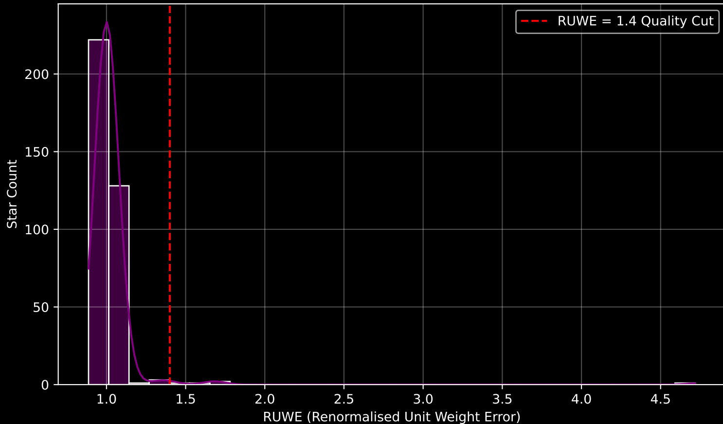
Gaia Cluster: [NGC_2635] RUWE Distribution (n= 359)
