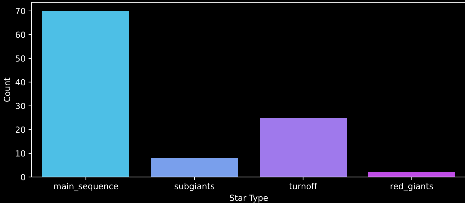
Gaia Cluster: [NGC_2645] Count plot of Star Type
