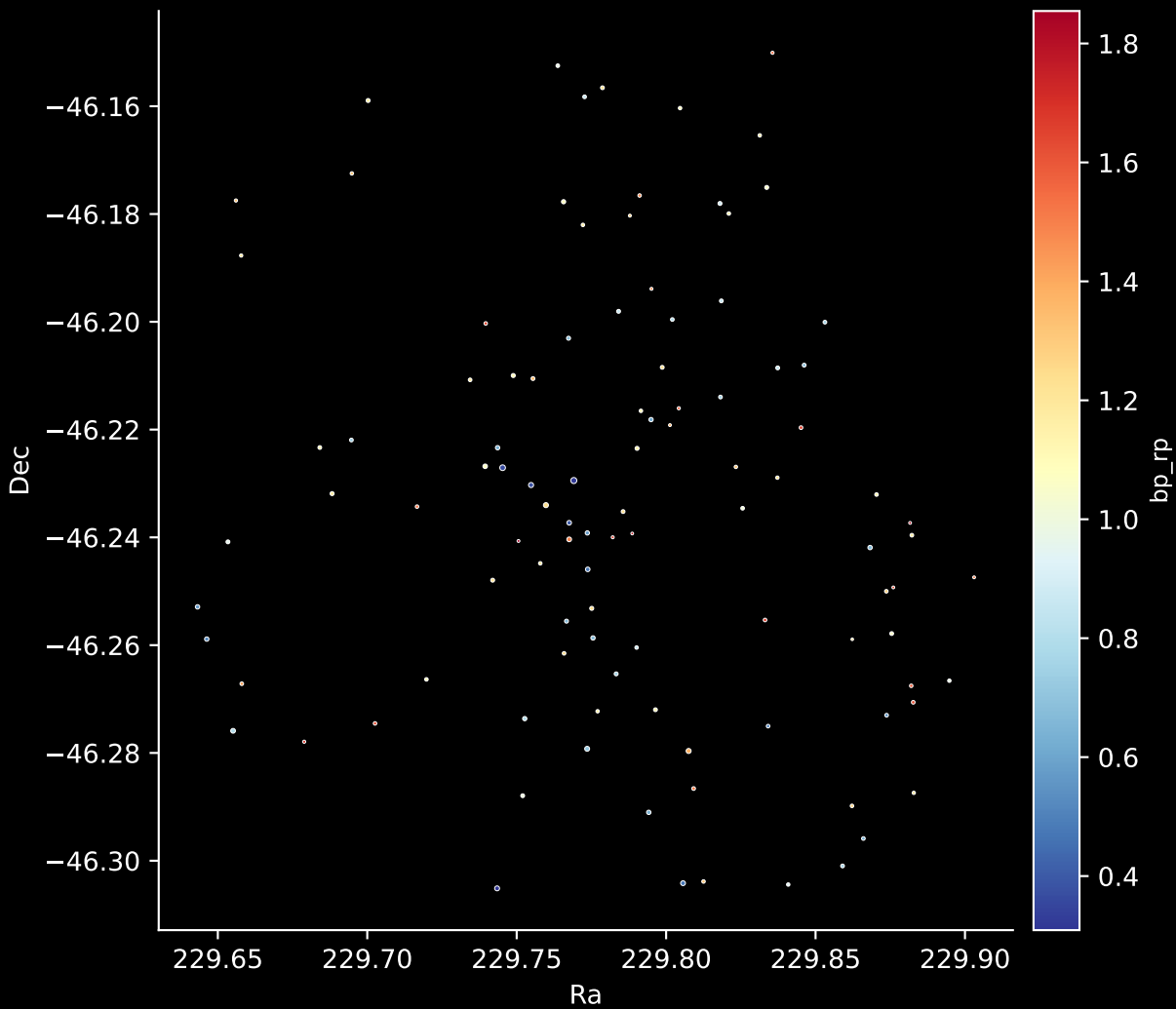
Gaia Cluster: [NGC_2645] Stars: 105
