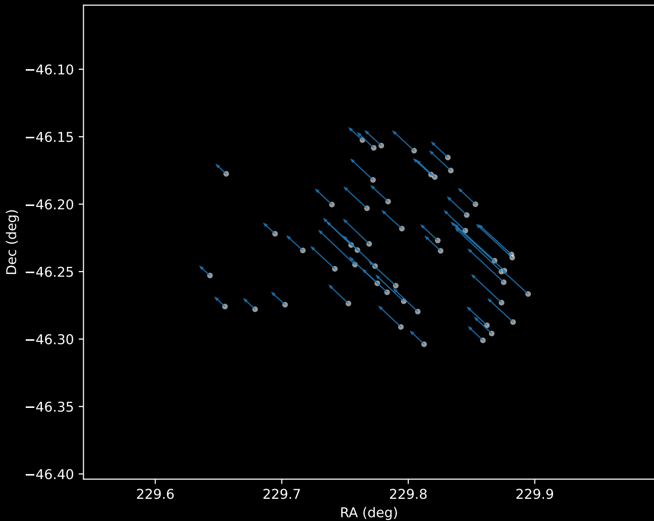
Gaia DR3 Cluster 0 Proper Motion Vectors (n=51)
