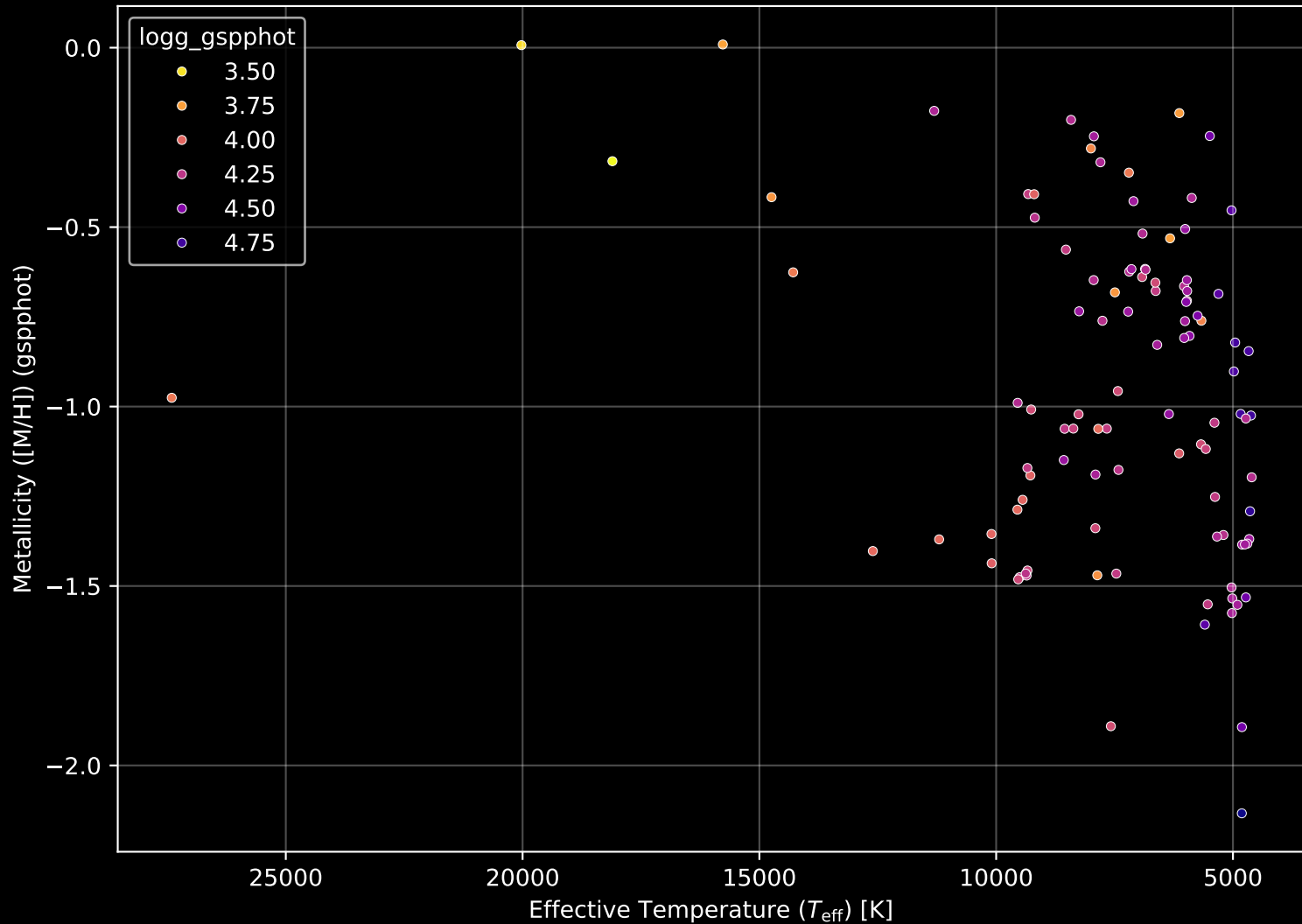
Gaia Cluster: [NGC_2645] Stellar Population Parameters (n= 105)
