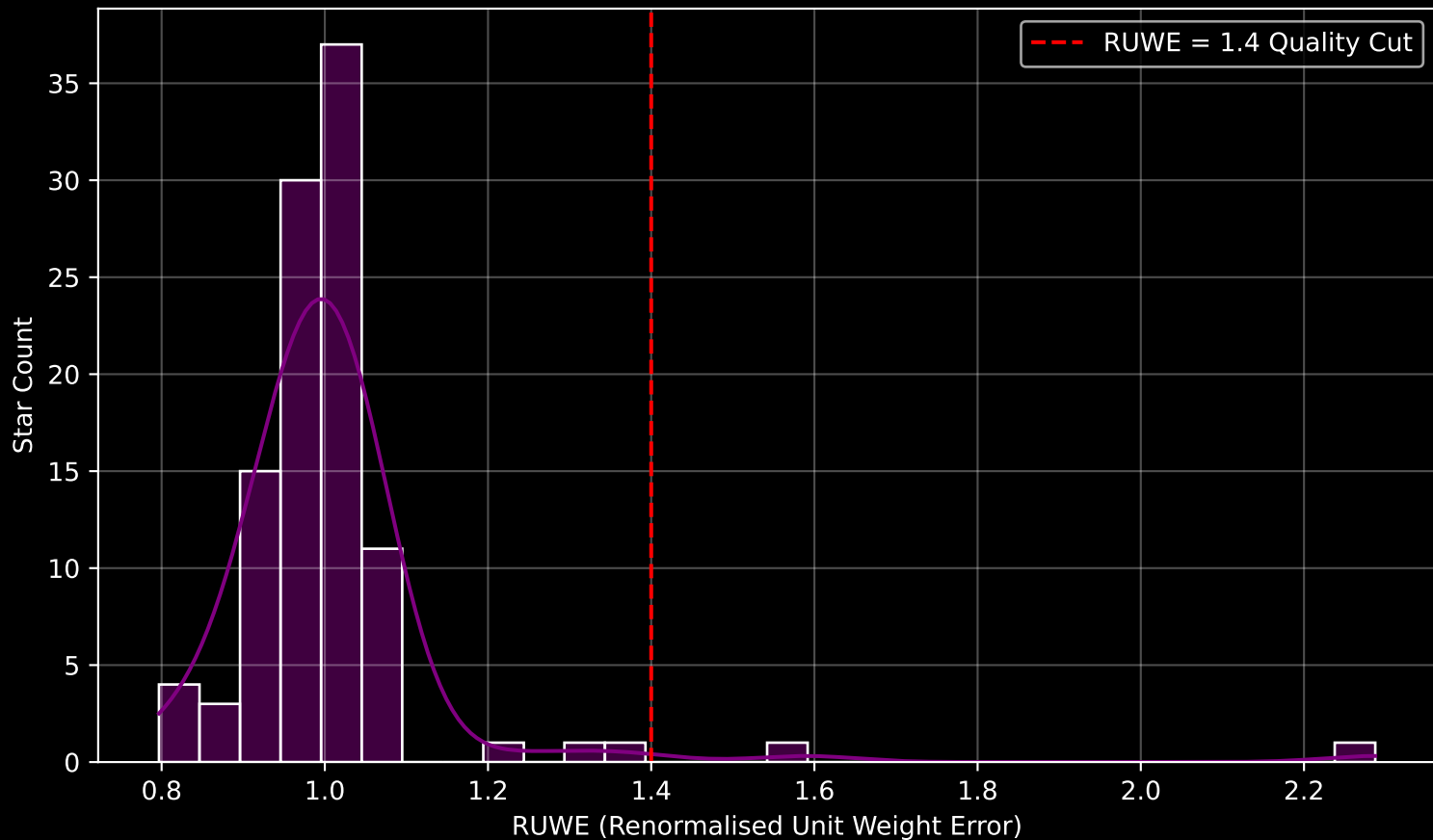
Gaia Cluster: [NGC_2645] RUWE Distribution (n= 105)
