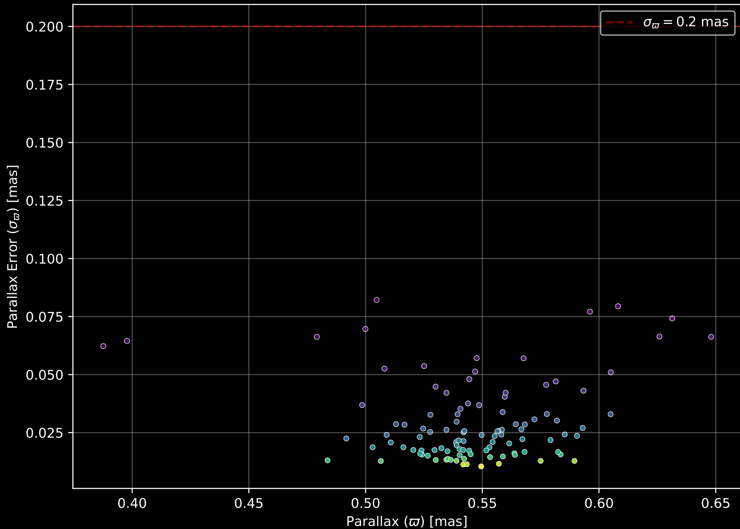
Gaia Cluster: [NGC_2645] Parallax Quality (n= 105)
