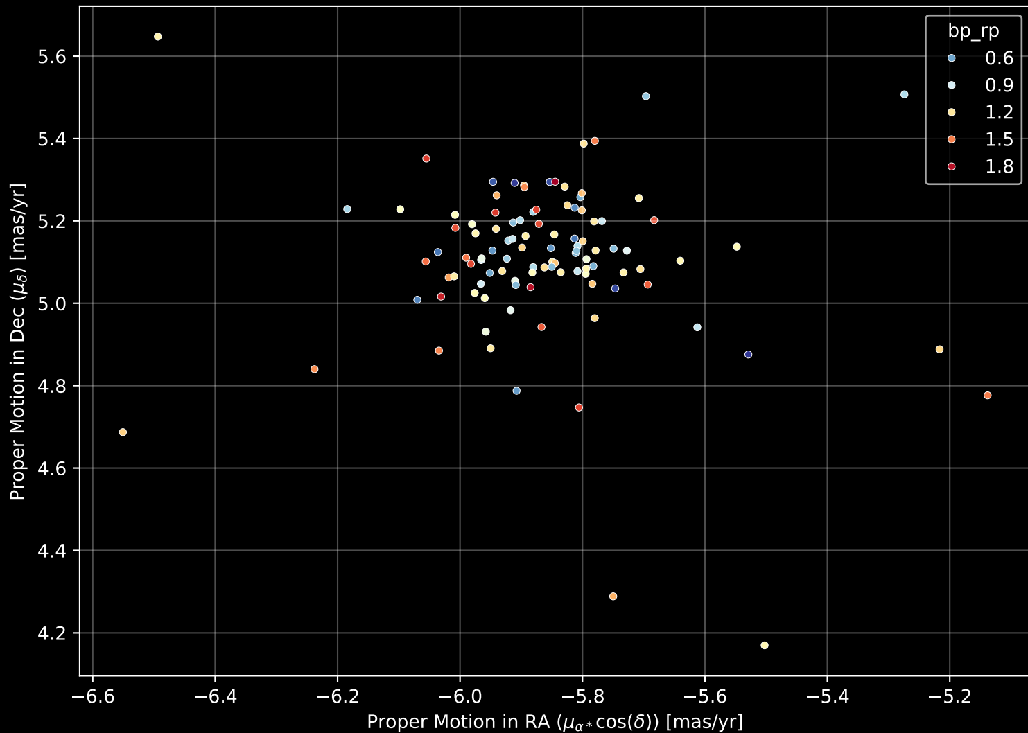
Gaia Cluster: [NGC_2645] Proper Motion Diagram (n= 105)
