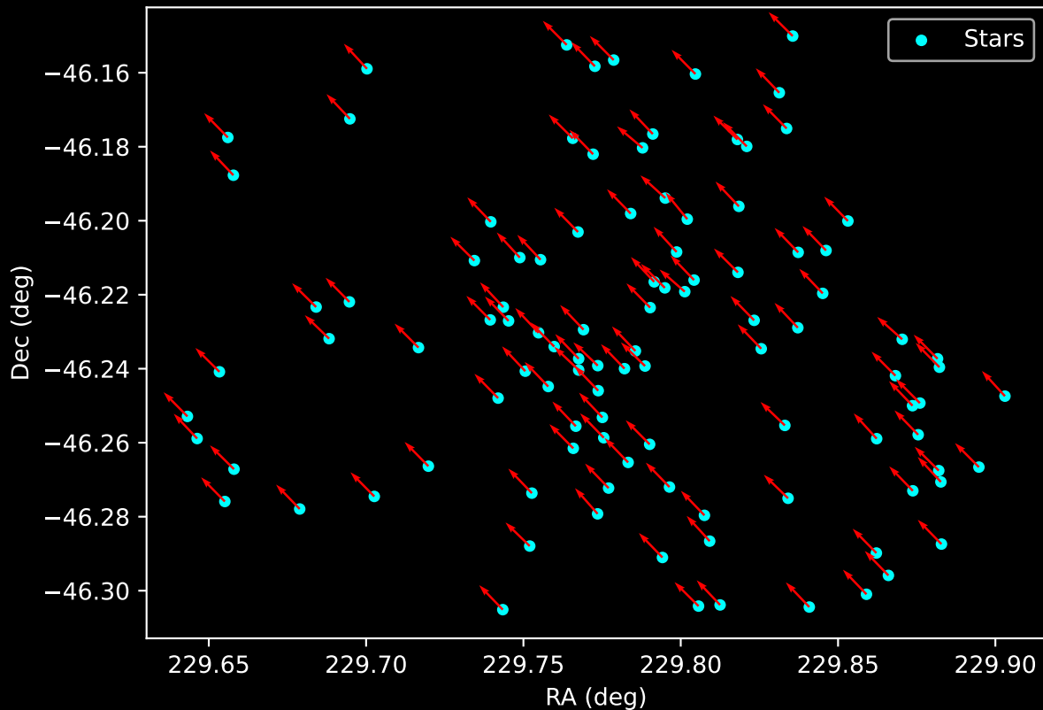
Gaia Cluster: [NGC_2645] Proper Motion Vectors for Gaia Star Field (n= 105)
