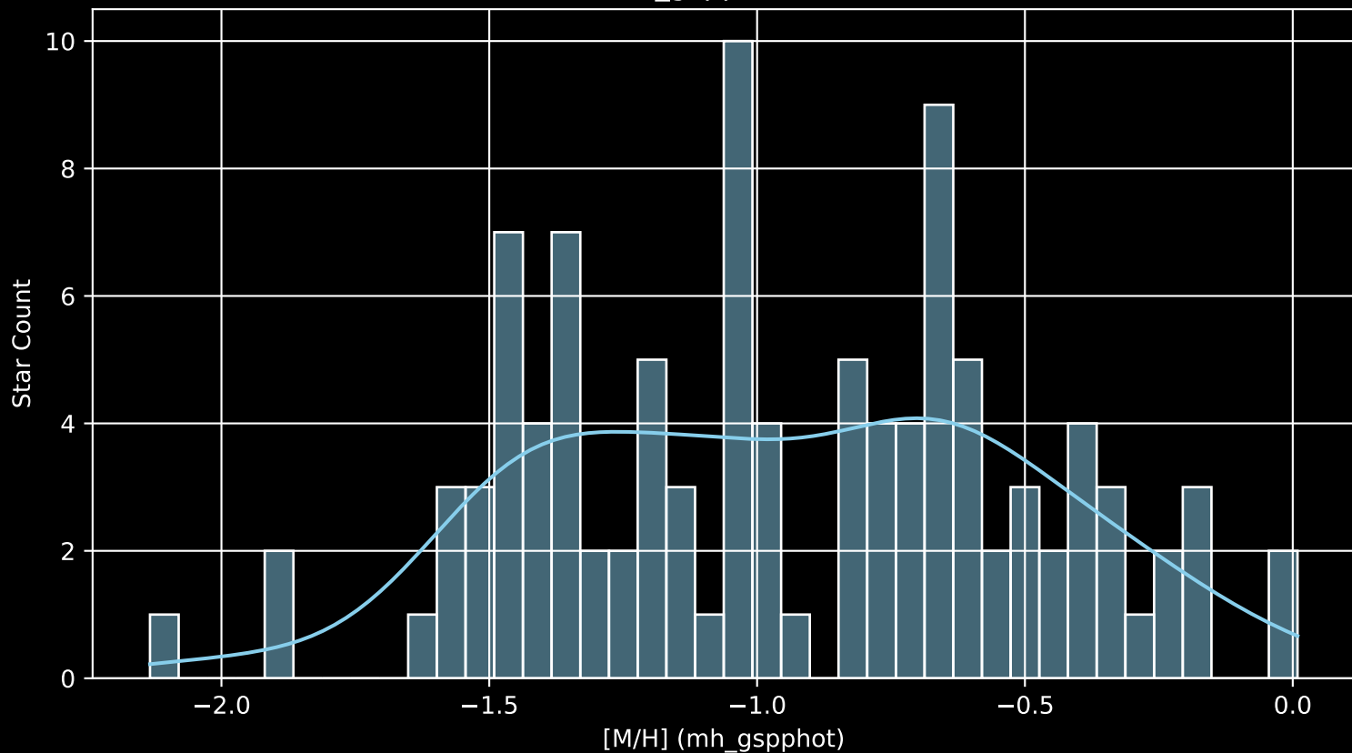
Gaia Cluster: [NGC_2645 [M/H] (mh_gspphot) (n= 105)
