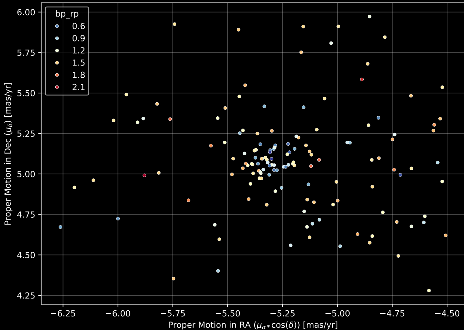
Gaia Cluster: [NGC_2659] Proper Motion Diagram (n= 145)
