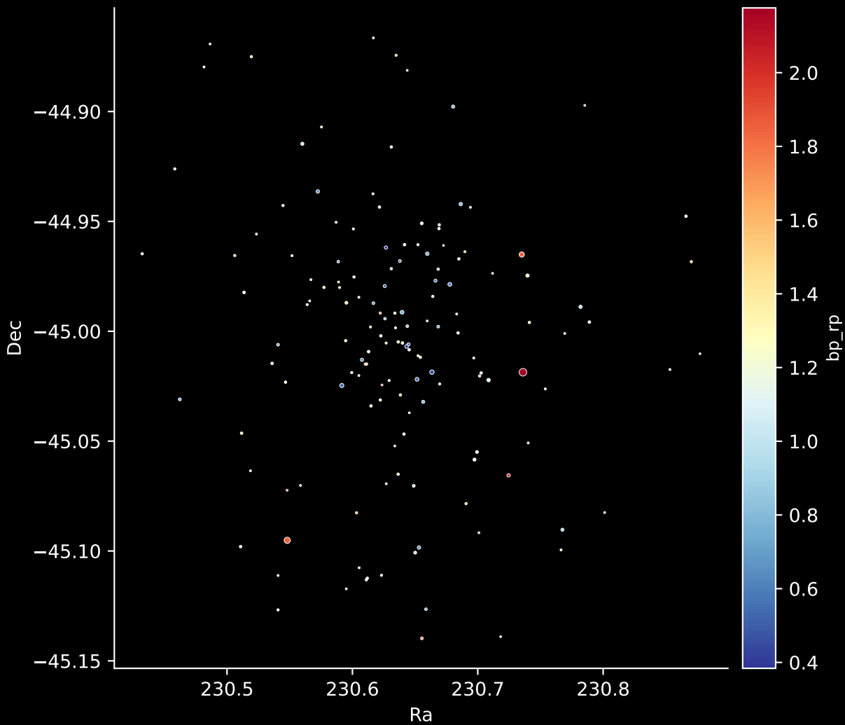
Gaia Cluster: [NGC_2659] Stars: 145
