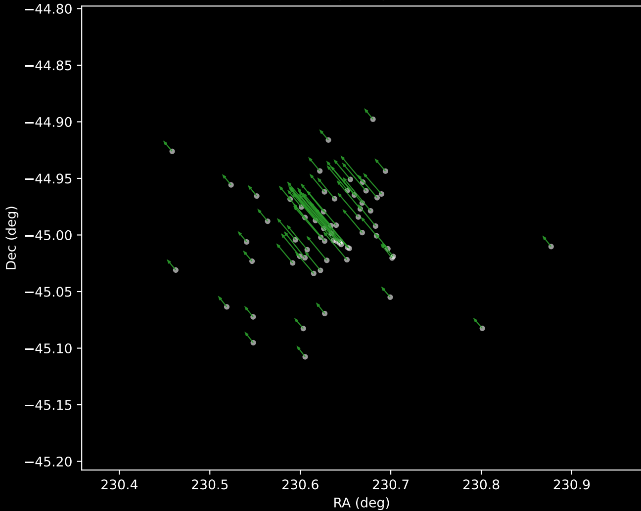
Gaia DR3 Cluster 4 Proper Motion Vectors (n=66)
