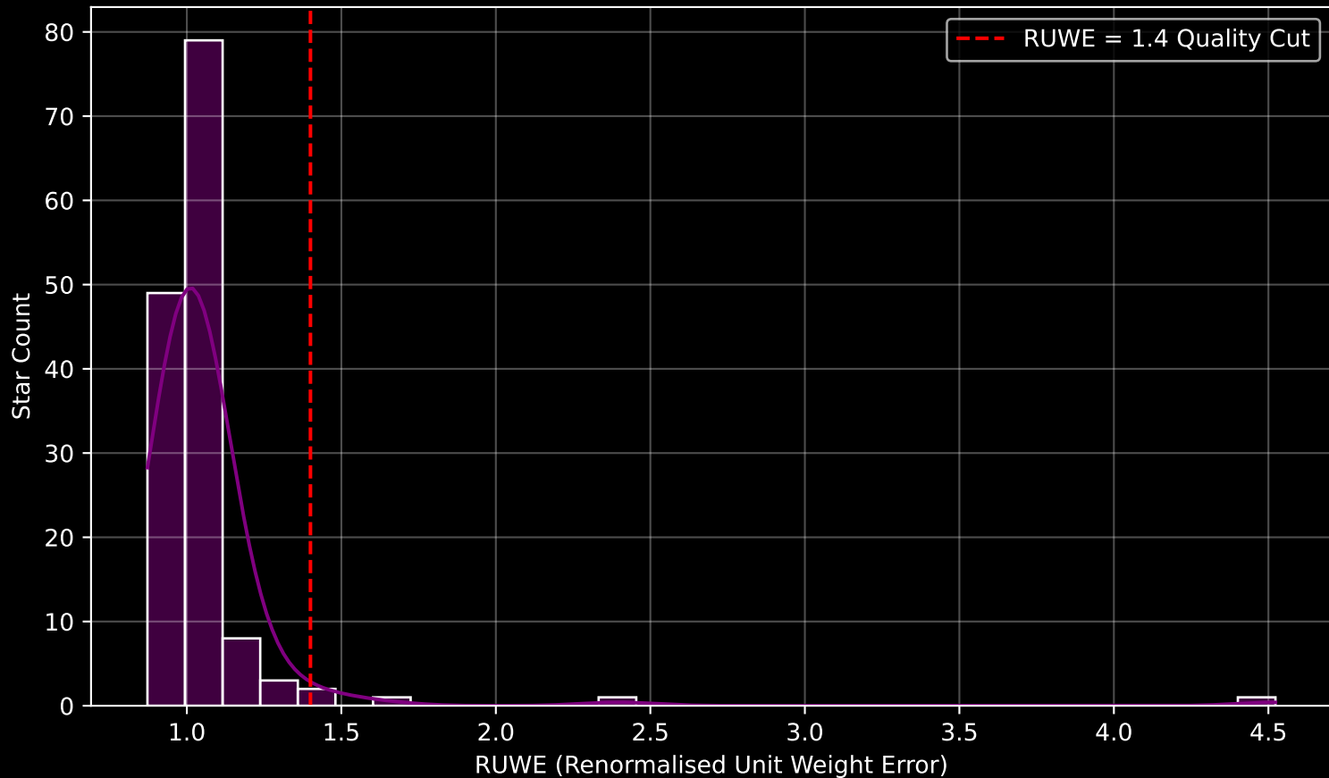
Gaia Cluster: [NGC_2659] RUWE Distribution (n= 144)
