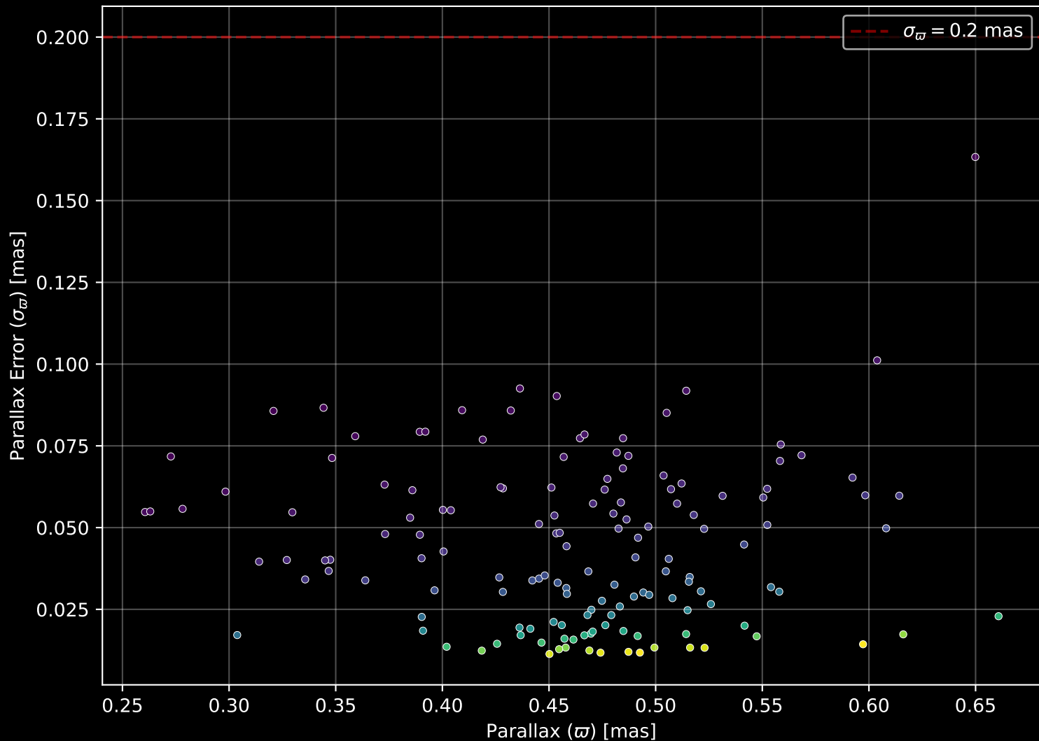
Gaia Cluster: [NGC_2659] Parallax Quality (n= 145)
