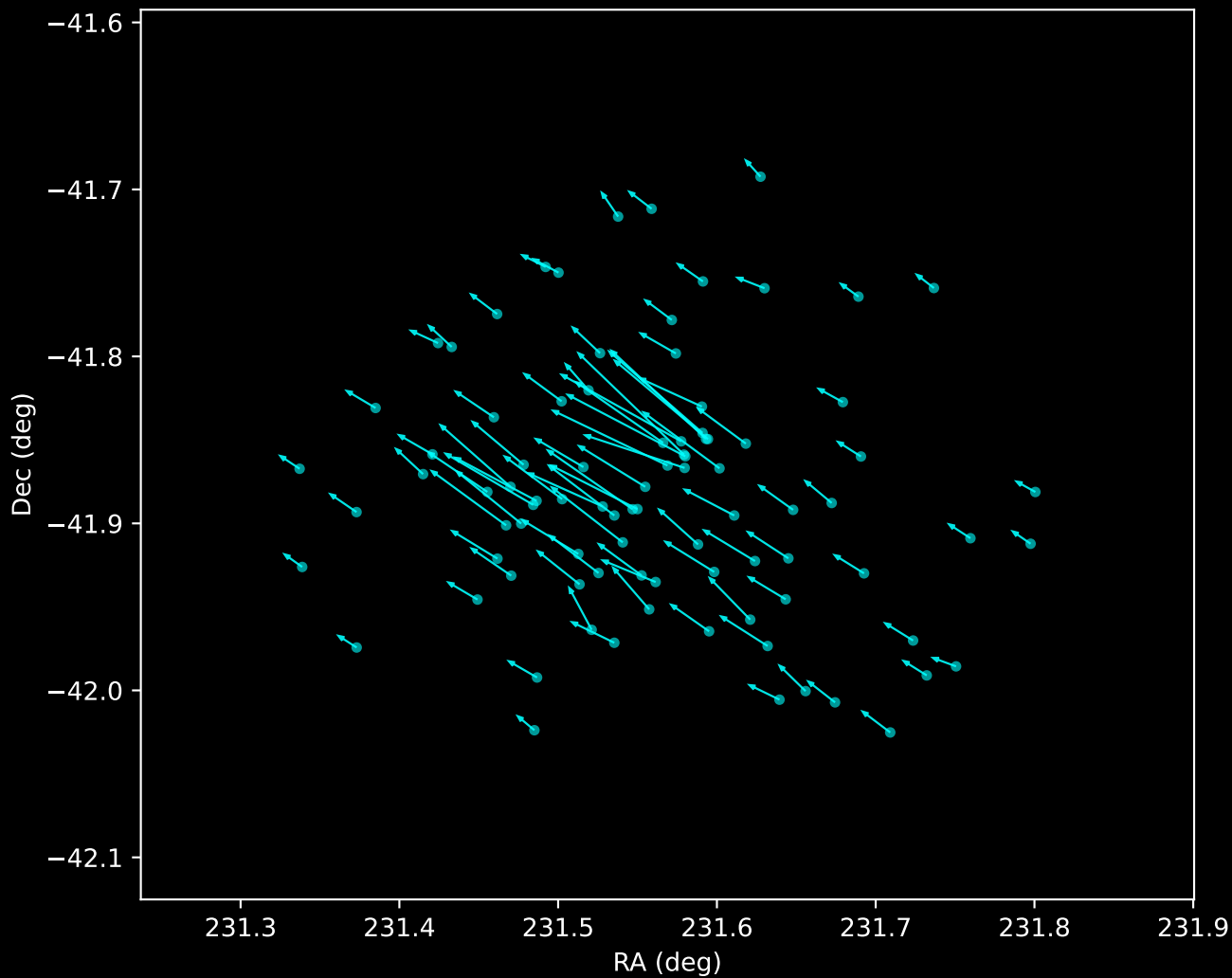
Gaia DR3 Noise Stream Proper Motion Vectors (n=89)
