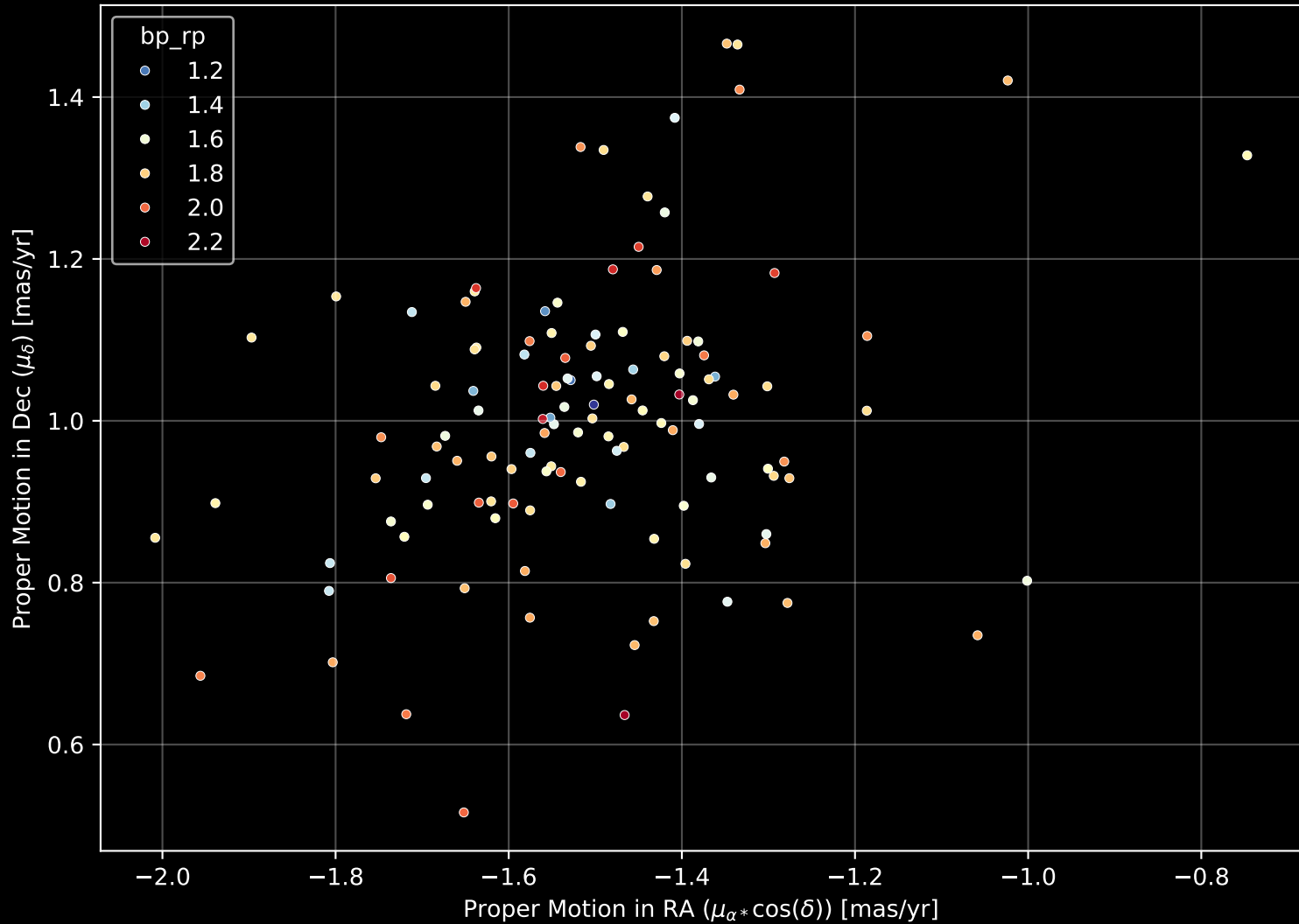
Gaia Cluster: [NGC_2671] Proper Motion Diagram (n= 121)
