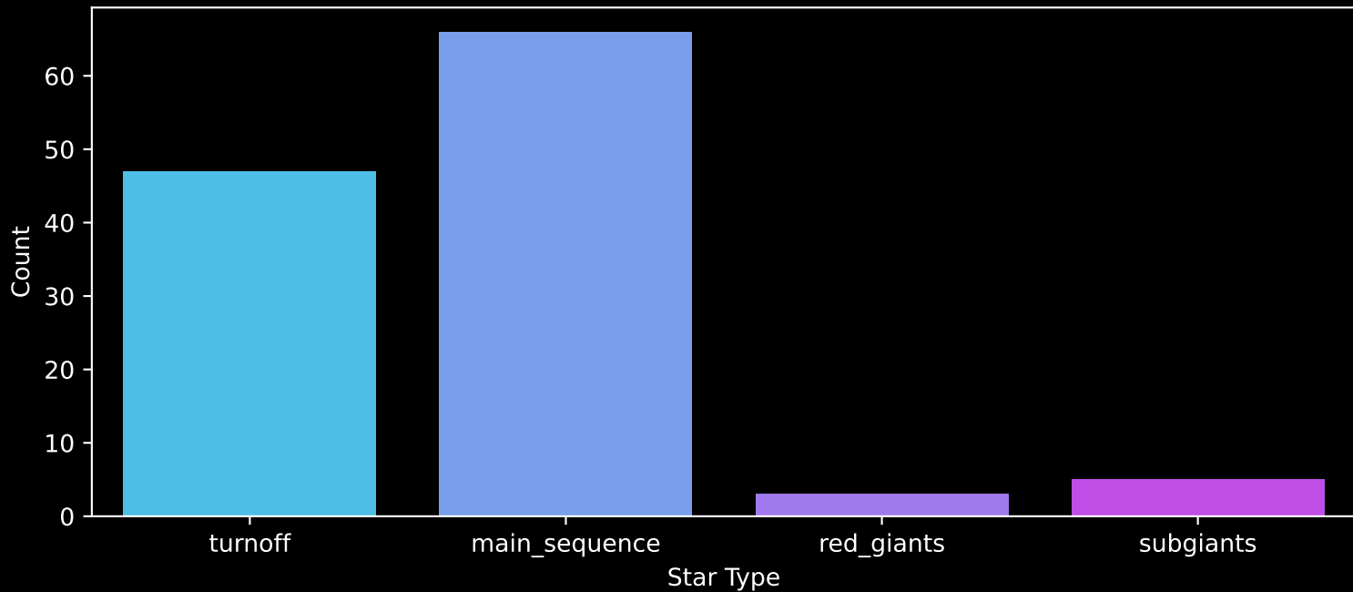
Gaia Cluster: [NGC_2671] Count plot of Star Type
