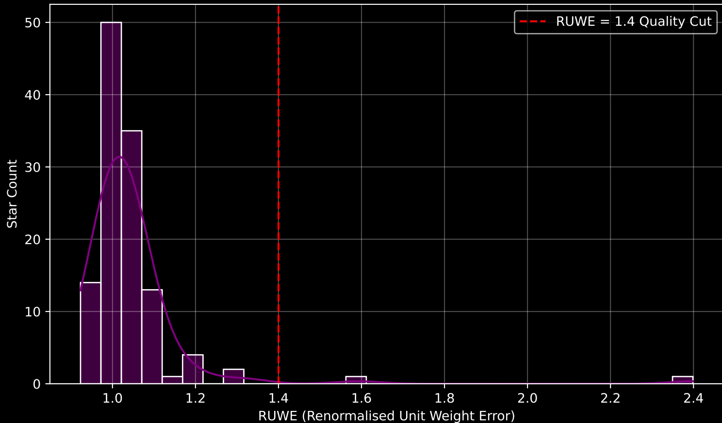
Gaia Cluster: [NGC_2671] RUWE Distribution (n= 121)
