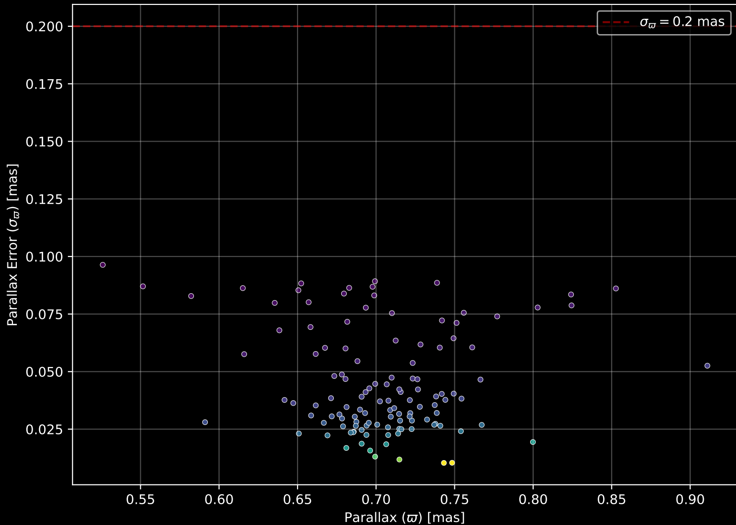
Gaia Cluster: [NGC_2671] Parallax Quality (n= 121)
