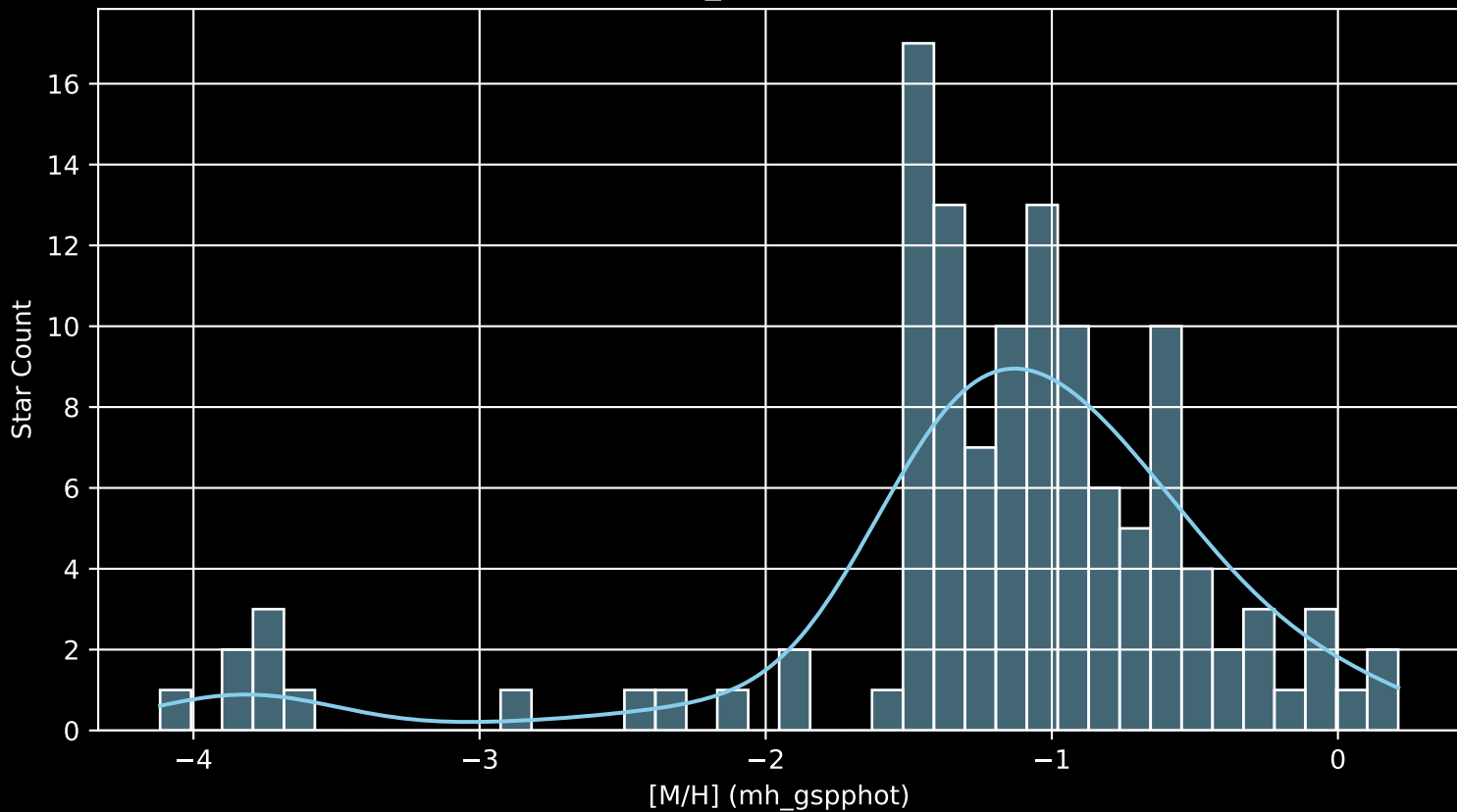
Gaia Cluster: [NGC_2671 [M/H] (mh_gspphot) (n= 121)
