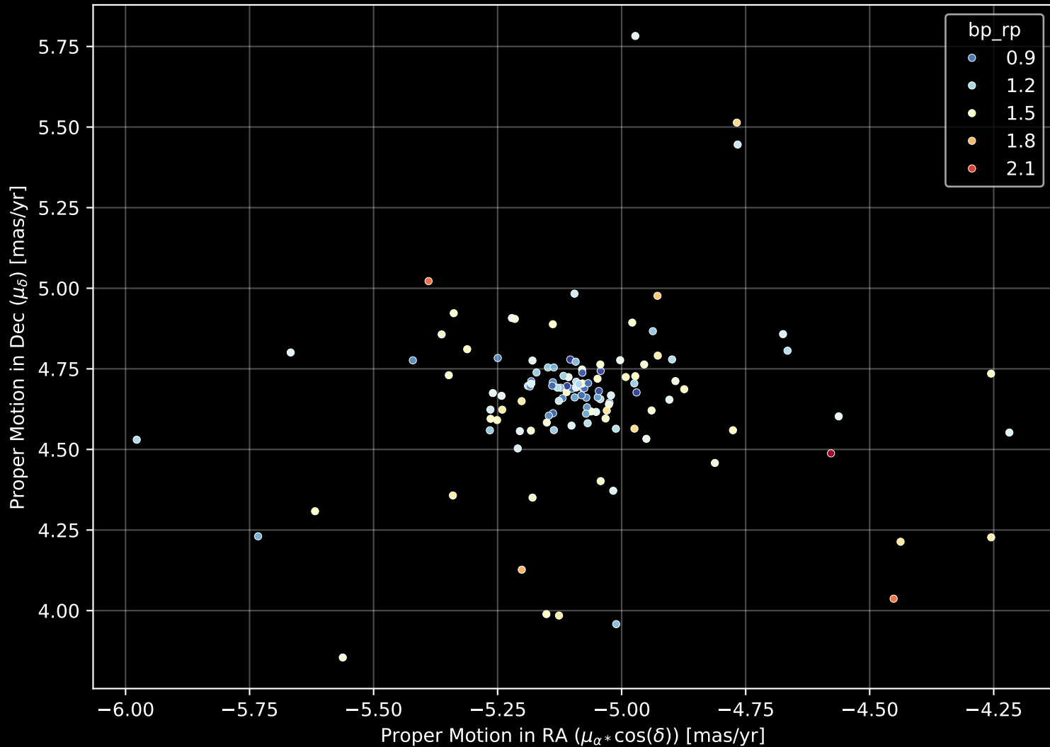
Gaia Cluster: [NGC_2866] Proper Motion Diagram (n= 121)
