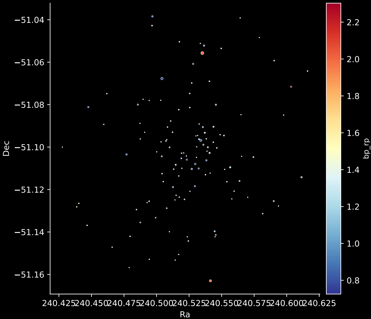
Gaia Cluster: [NGC_2866] Stars: 121
