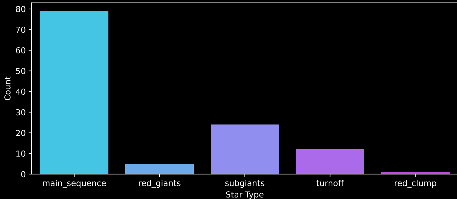
Gaia Cluster: [NGC_2866] Count plot of Star Type
