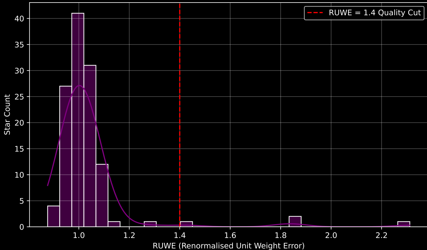
Gaia Cluster: [NGC_2866] RUWE Distribution (n= 121)
