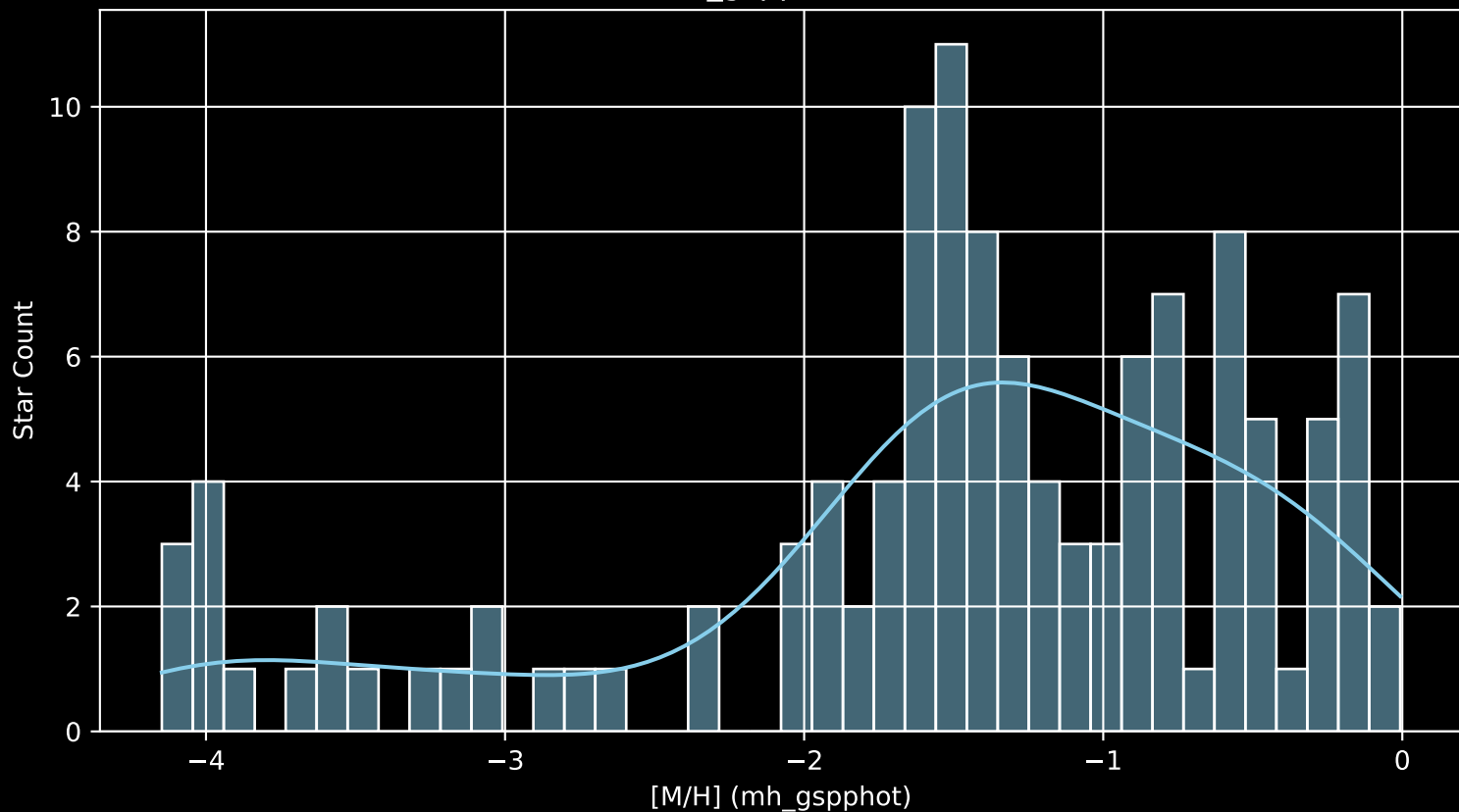
Gaia Cluster: [NGC_2866 [M/H] (mh_gspphot) (n= 121)
