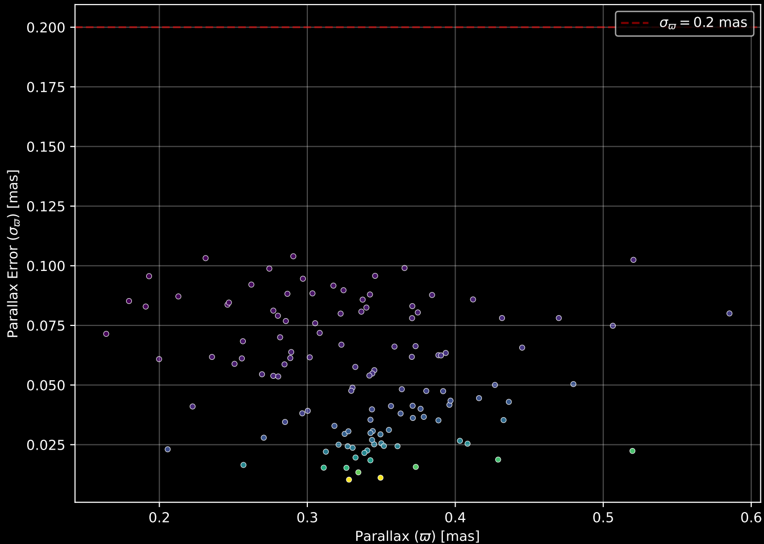
Gaia Cluster: [NGC_2866] Parallax Quality (n= 121)
