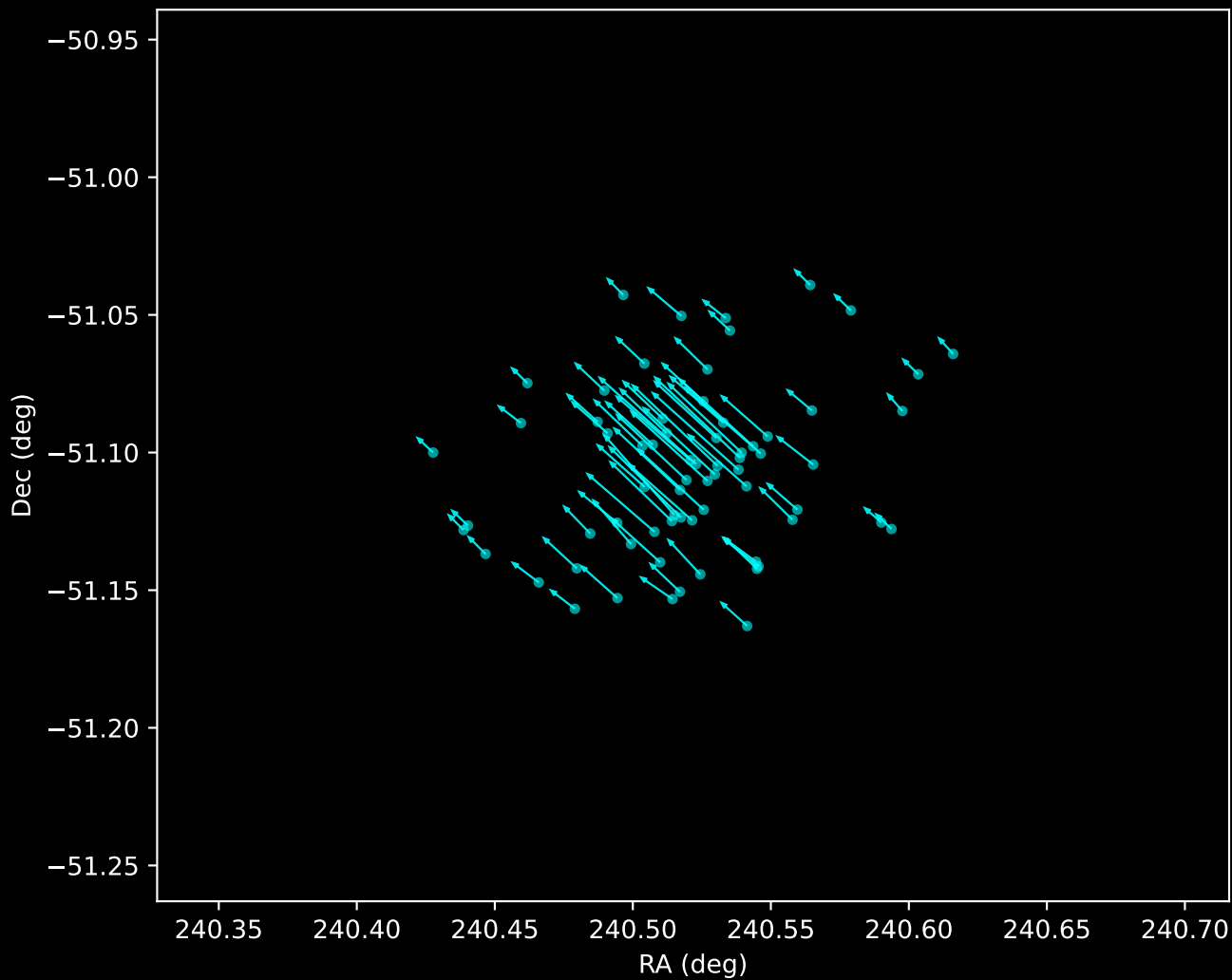
Gaia DR3 Noise Stream Proper Motion Vectors (n=69)
