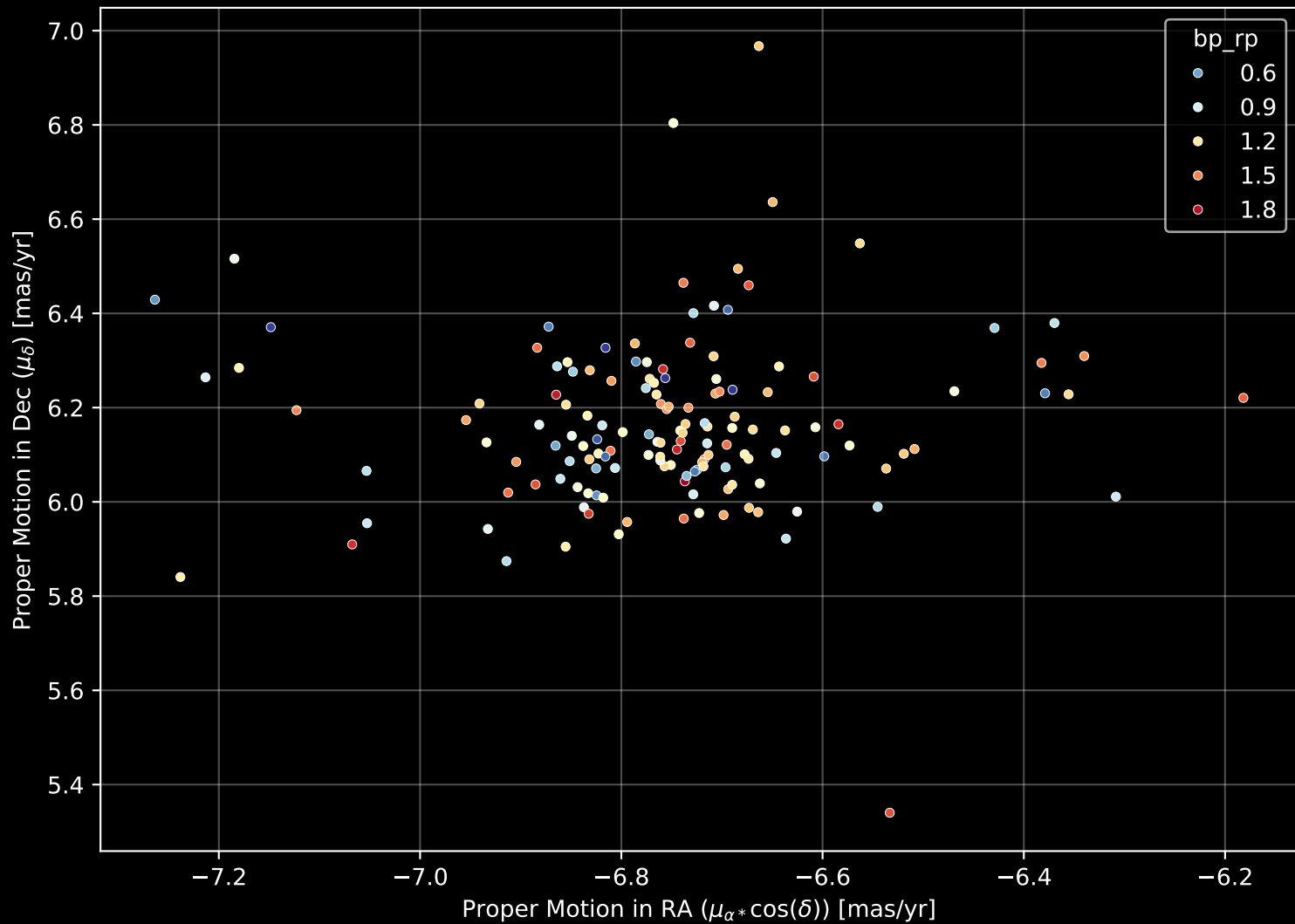
Gaia Cluster: [NGC_2910] Proper Motion Diagram (n= 147)
