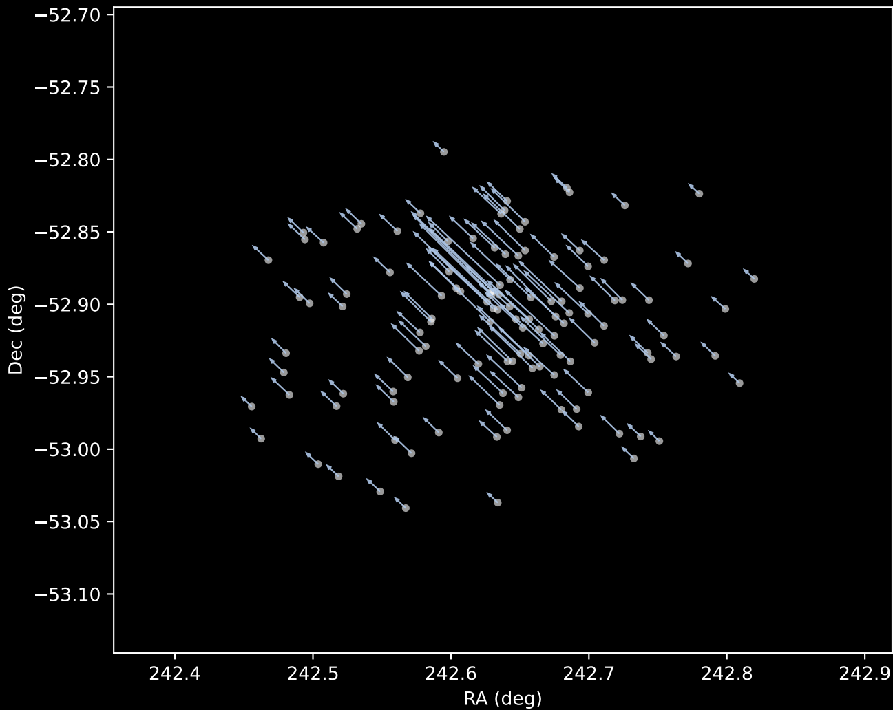
Gaia DR3 Cluster 1 Proper Motion Vectors (n=124)
