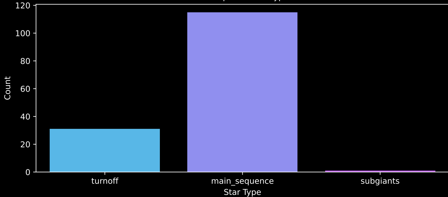
Gaia Cluster: [NGC_2910] Count plot of Star Type
