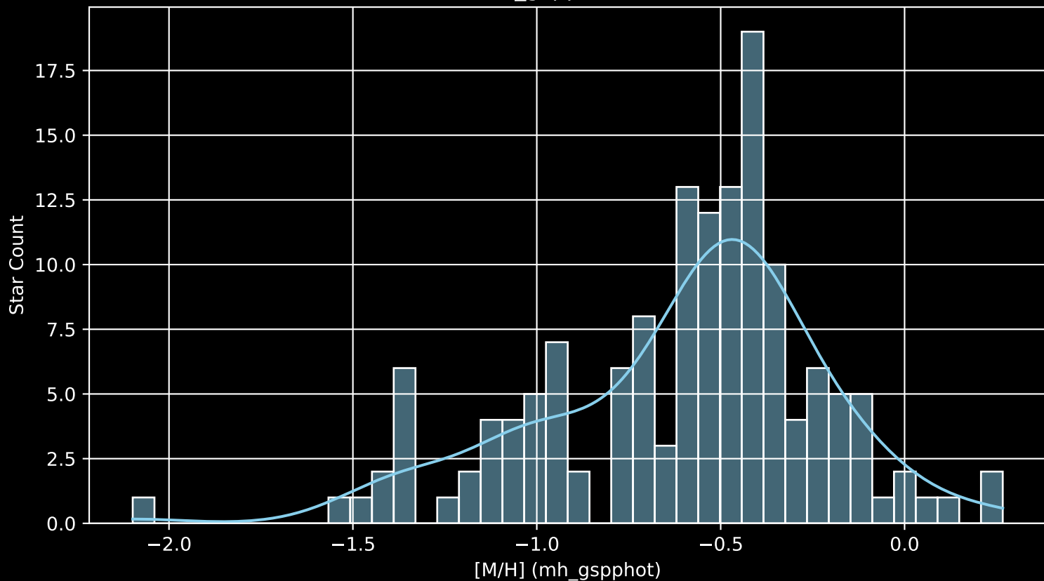
Gaia Cluster: [NGC_2910 [M/H] (mh_gspphot) (n= 147)
