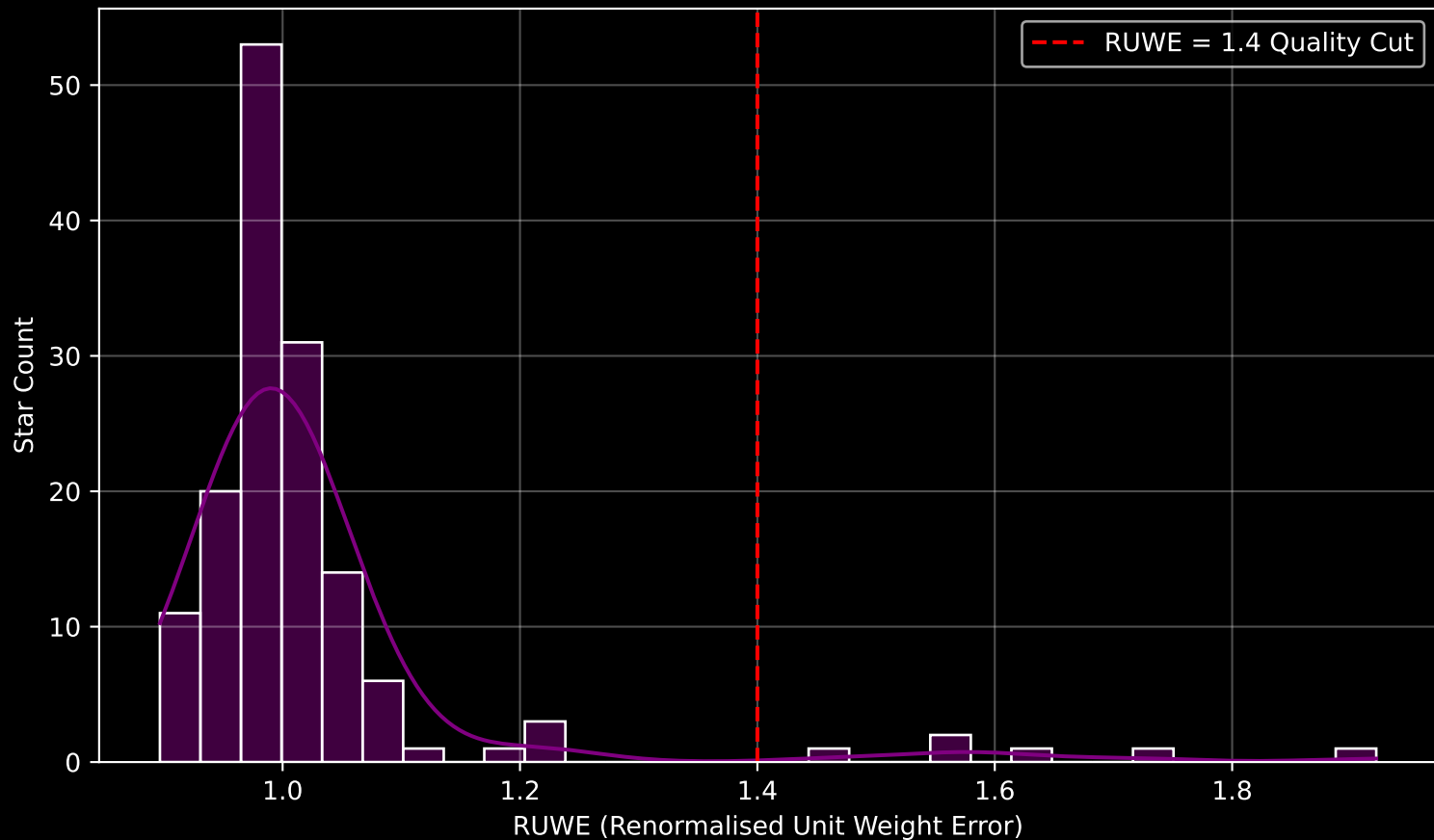
Gaia Cluster: [NGC_2910] RUWE Distribution (n= 146)
