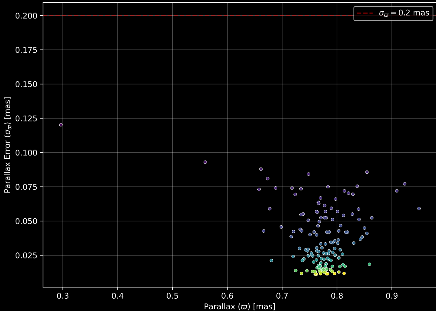
Gaia Cluster: [NGC_2910] Parallax Quality (n= 147)
