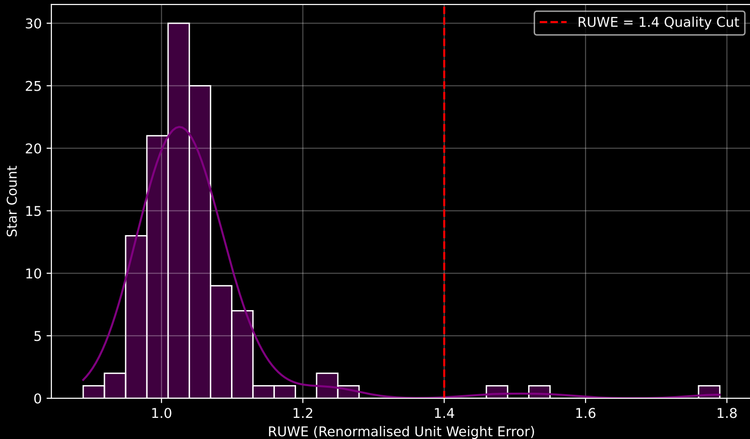
Gaia Cluster: [NGC_3105] RUWE Distribution (n= 116)
