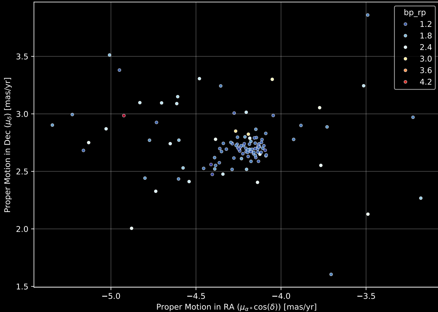
Gaia Cluster: [NGC_3105] Proper Motion Diagram (n= 116)
