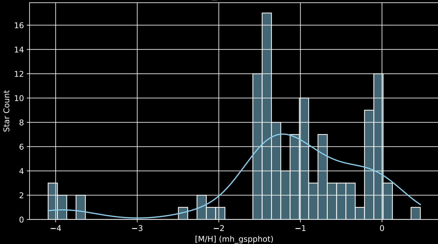
Gaia Cluster: [NGC_3105 [M/H] (mh_gspphot) (n= 115)
