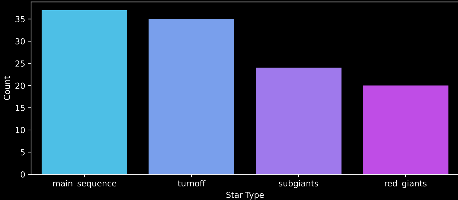
Gaia Cluster: [NGC_3105] Count plot of Star Type
