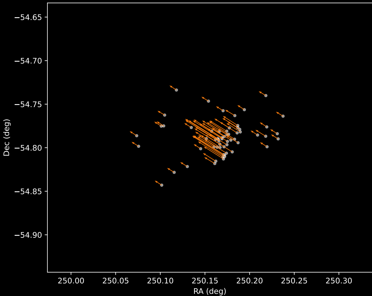
Gaia DR3 Cluster 2 Proper Motion Vectors (n=61)
