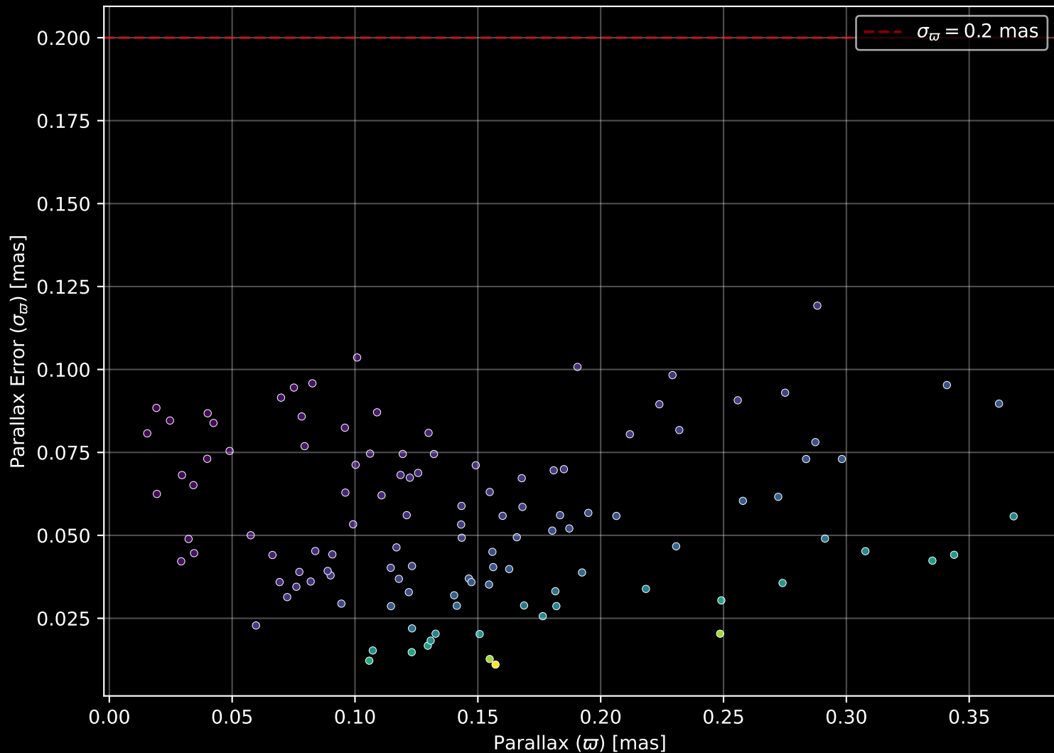
Gaia Cluster: [NGC_3105] Parallax Quality (n= 116)
