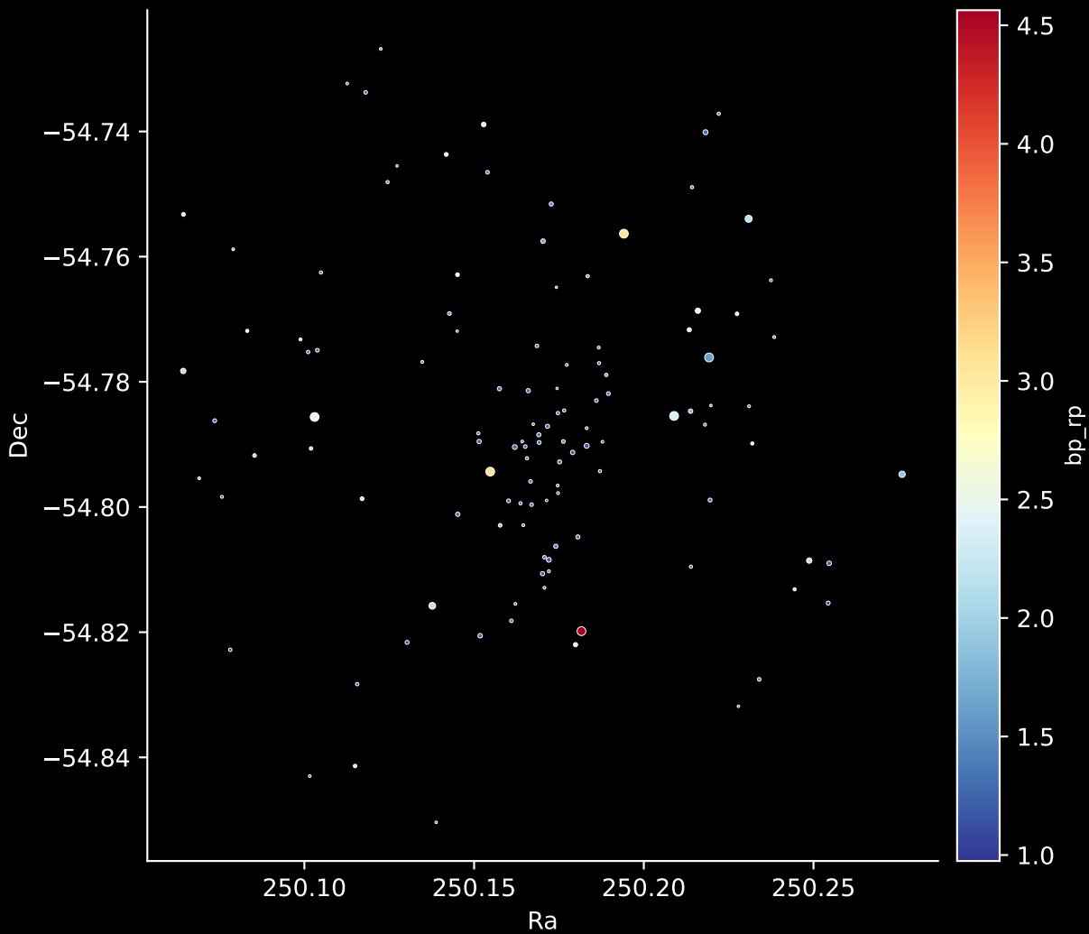
Gaia Cluster: [NGC_3105] Stars: 116
