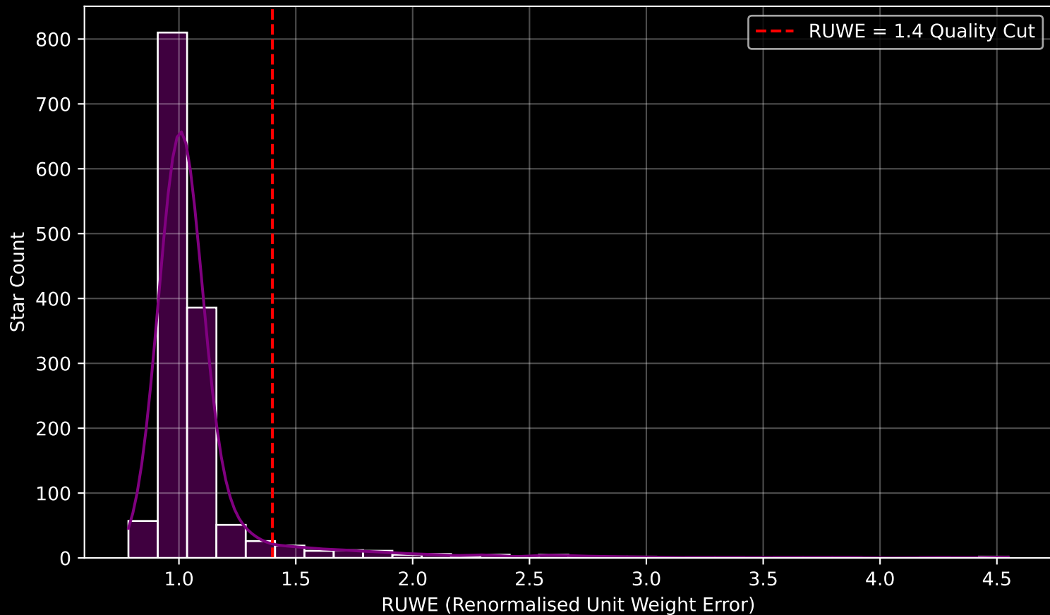
Gaia Cluster: [NGC_3114] RUWE Distribution (n= 1423)
