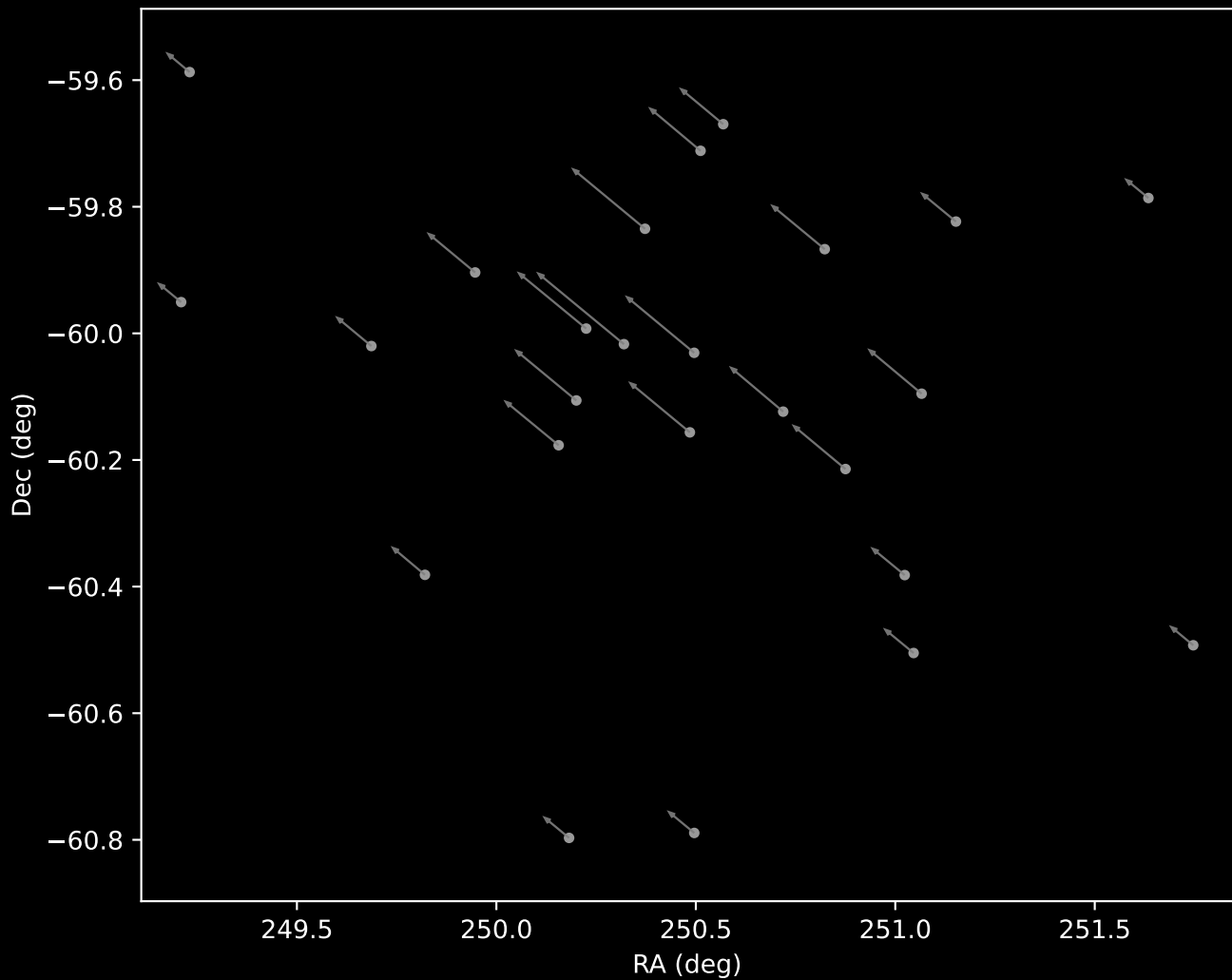
Gaia DR3 Cluster 54 Proper Motion Vectors (n=25)
