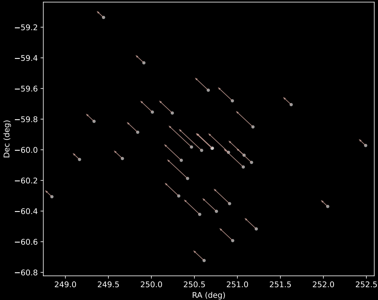
Gaia DR3 Cluster 71 Proper Motion Vectors (n=32)
