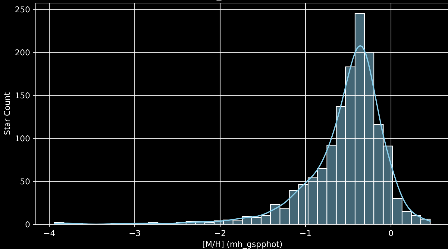
Gaia Cluster: [NGC_3114 [M/H] (mh_gspphot) (n= 1430)
