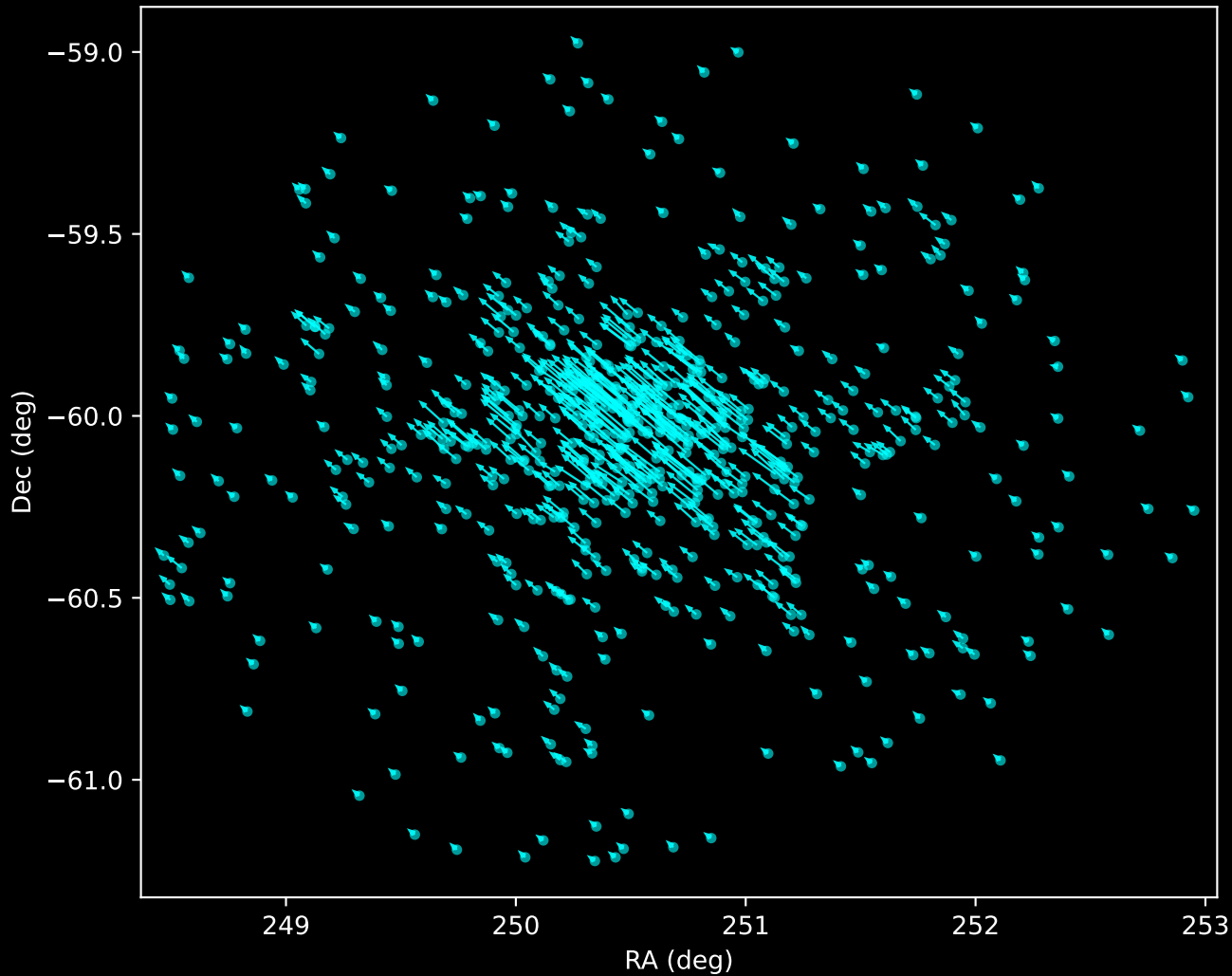
Gaia DR3 Noise Stream Proper Motion Vectors (n=613)
