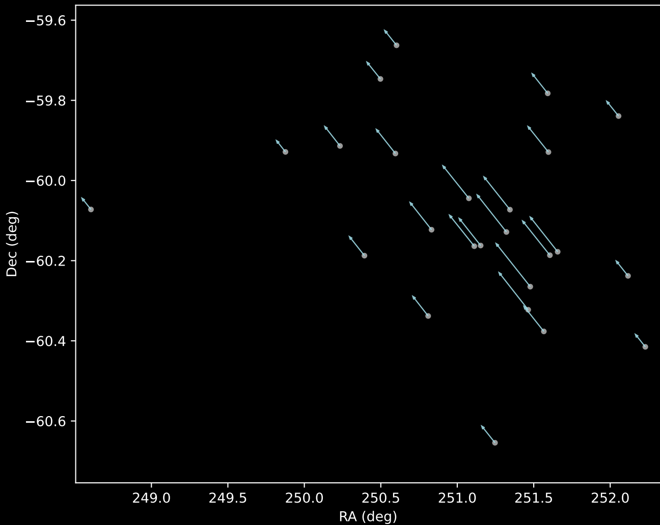
Gaia DR3 Cluster 59 Proper Motion Vectors (n=25)
