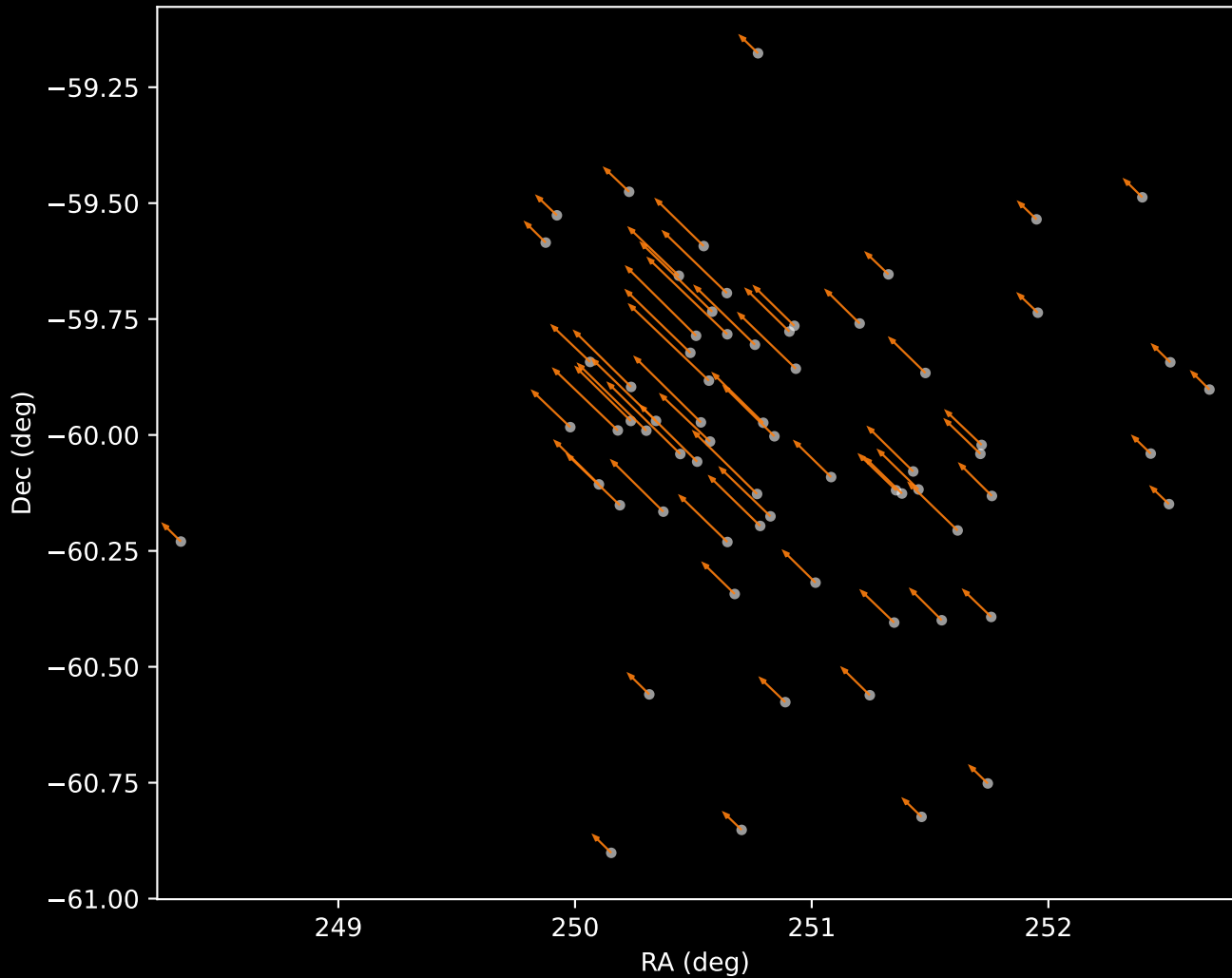
Gaia DR3 Cluster 62 Proper Motion Vectors (n=68)
