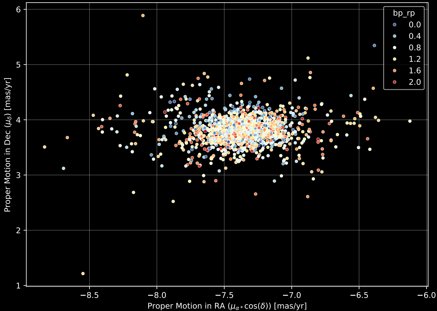
Gaia Cluster: [NGC_3114] Proper Motion Diagram (n= 1432)
