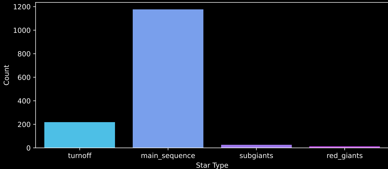
Gaia Cluster: [NGC_3114] Count plot of Star Type
