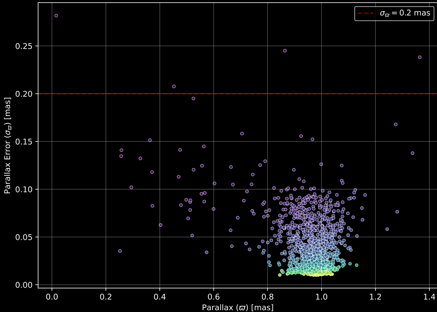
Gaia Cluster: [NGC_3114] Parallax Quality (n= 1432)
