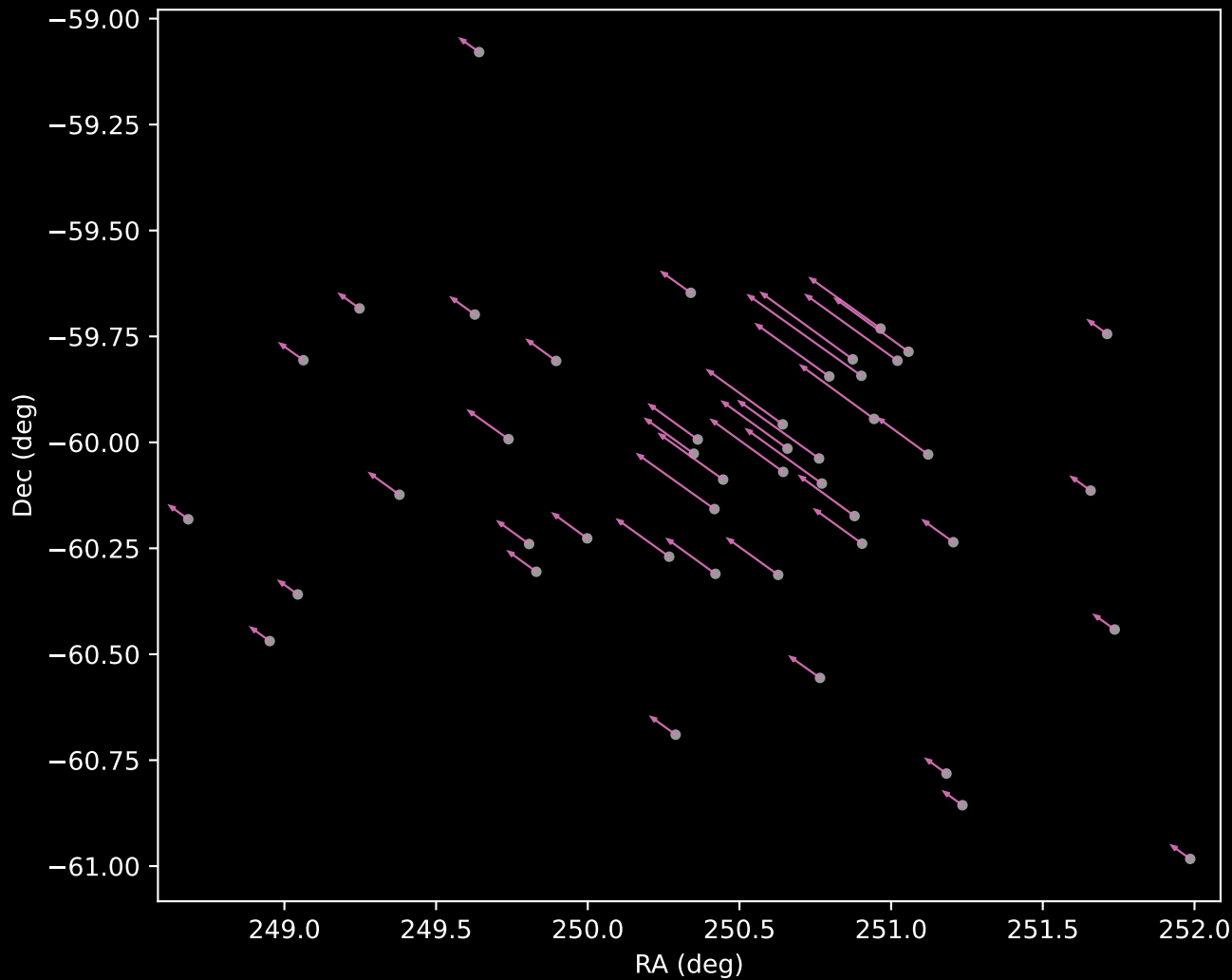
Gaia DR3 Cluster 52 Proper Motion Vectors (n=45)
