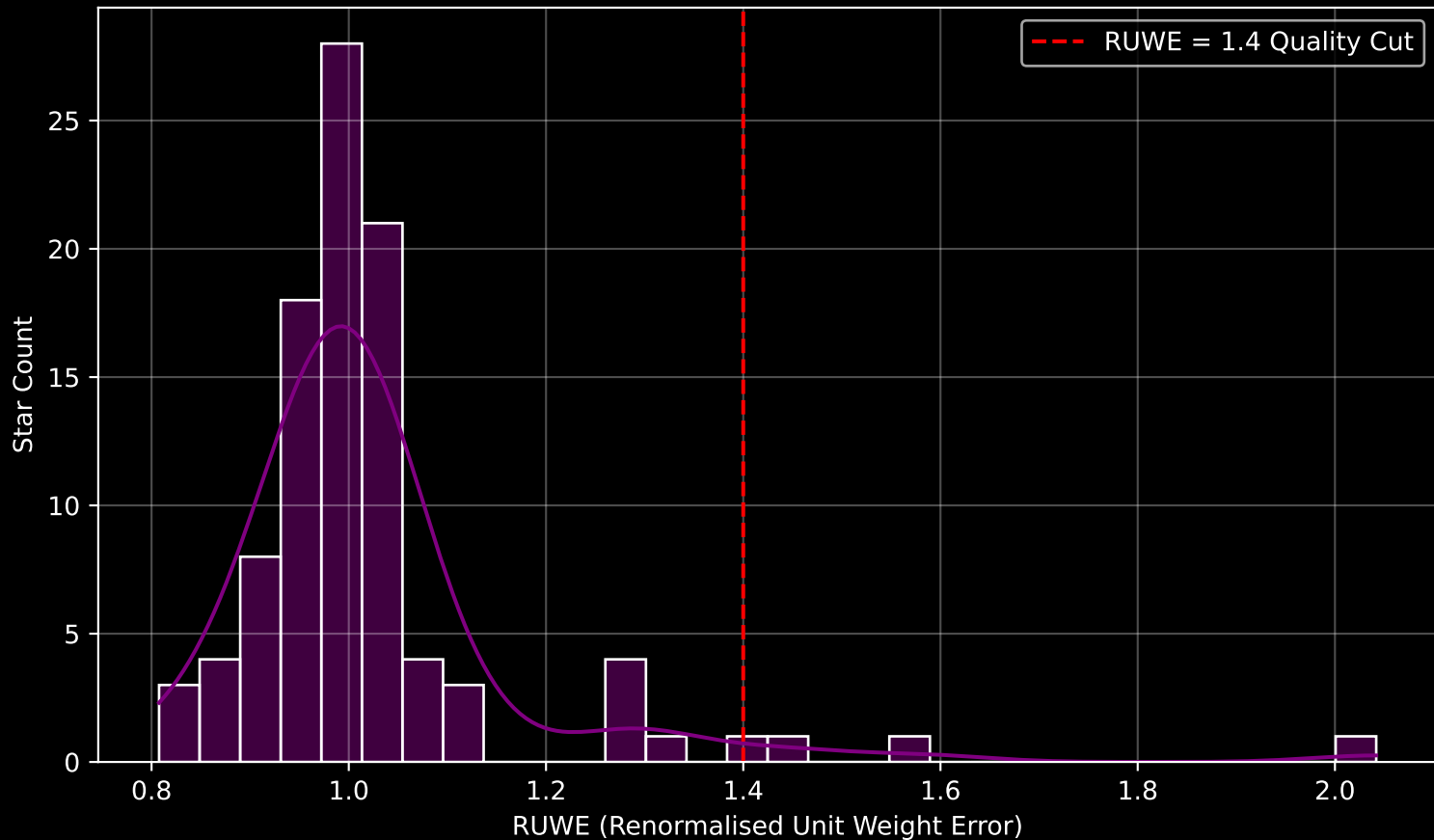
Gaia Cluster: [NGC_3228] RUWE Distribution (n= 98)
