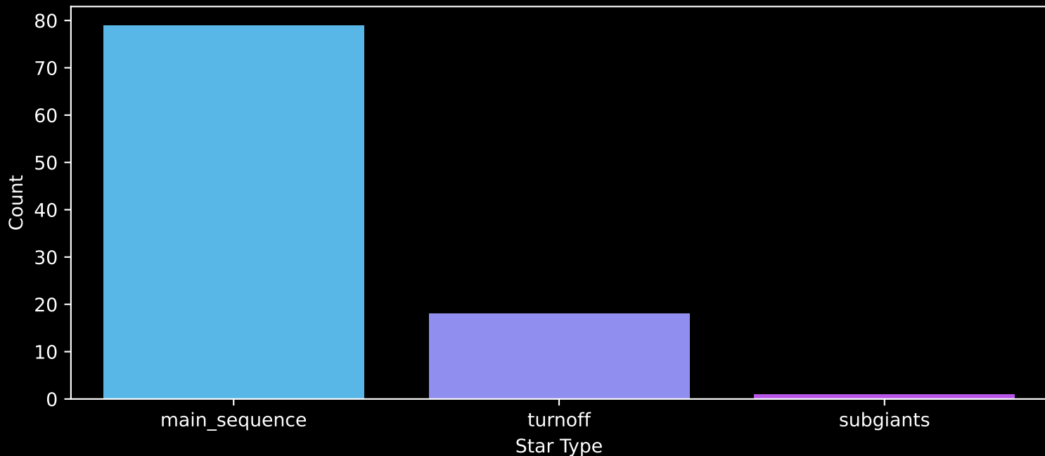
Gaia Cluster: [NGC_3228] Count plot of Star Type
