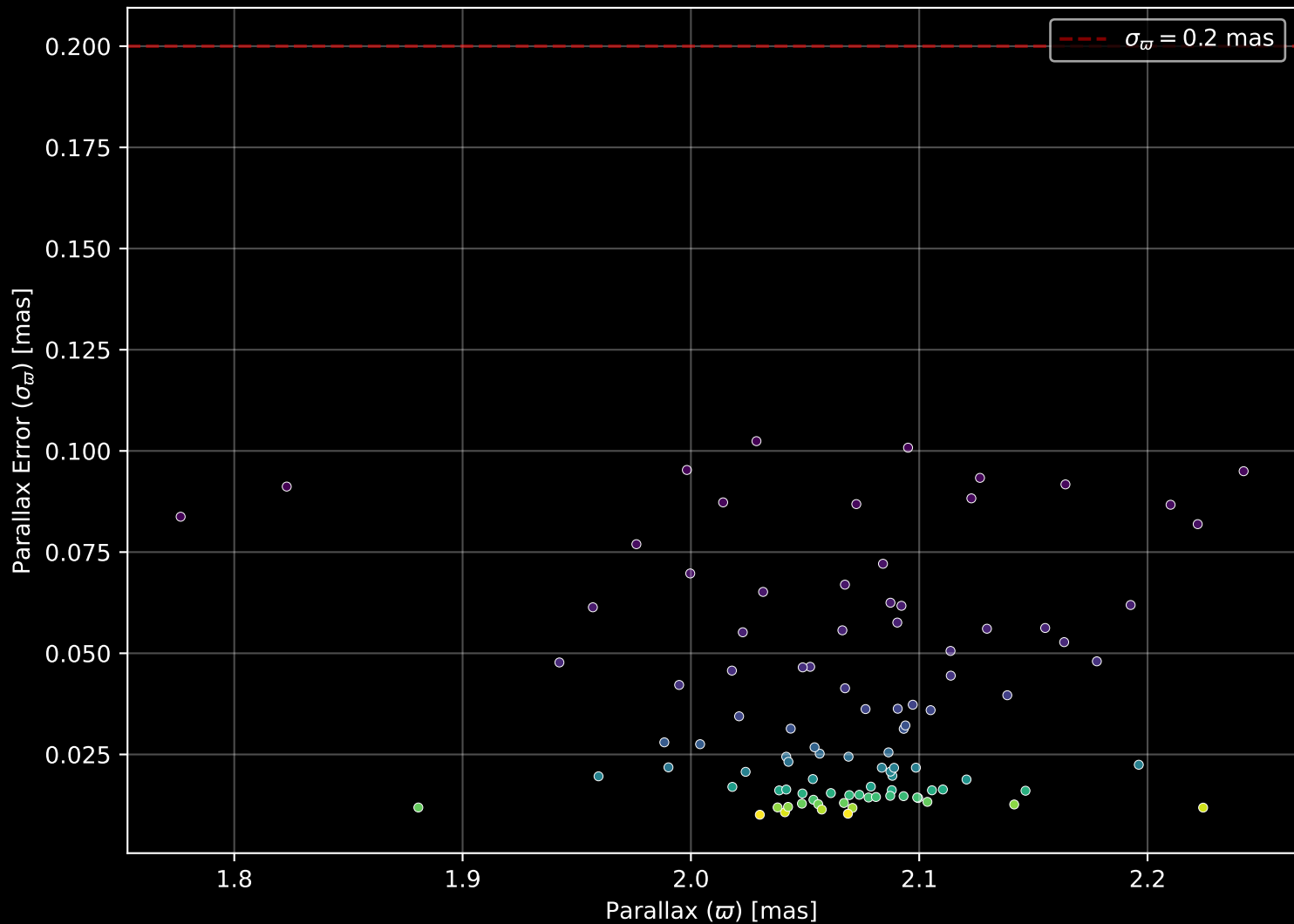
Gaia Cluster: [NGC_3228] Parallax Quality (n= 98)
