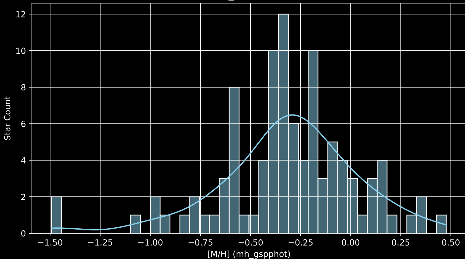
Gaia Cluster: [NGC_3228 [M/H] (mh_gspphot) (n= 98)
