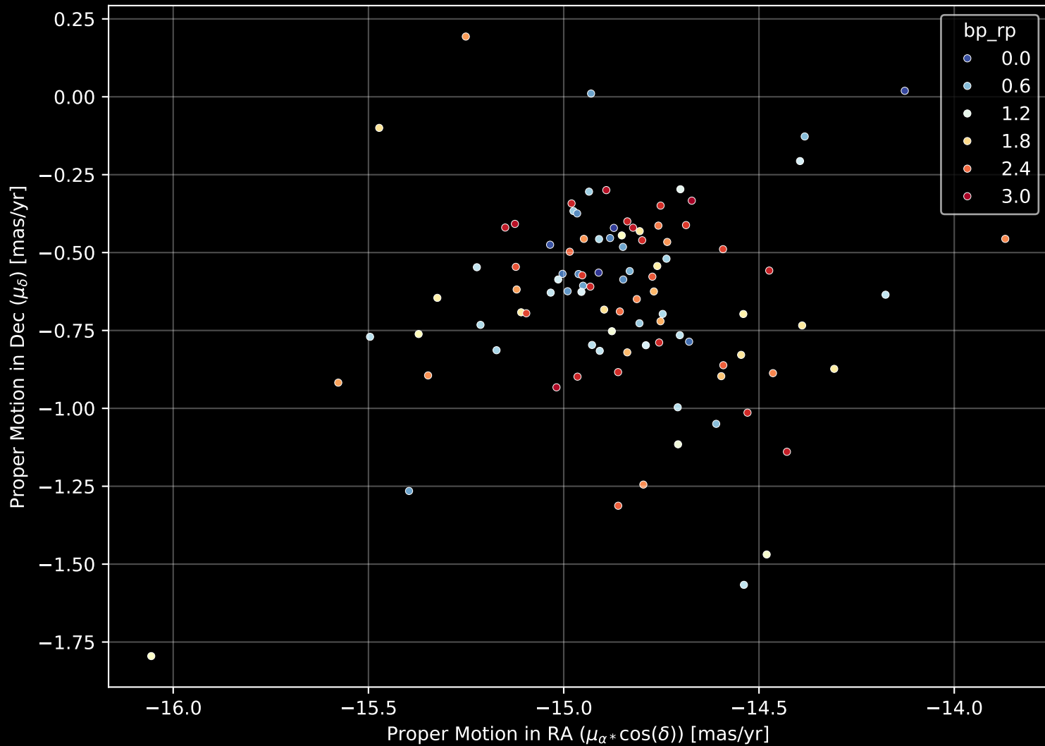
Gaia Cluster: [NGC_3228] Proper Motion Diagram (n= 98)
