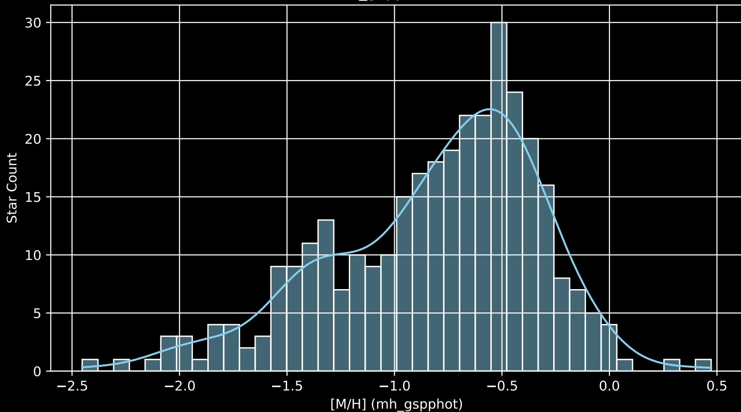
Gaia Cluster: [NGC_3330 [M/H] (mh_gspphot) (n= 331)
