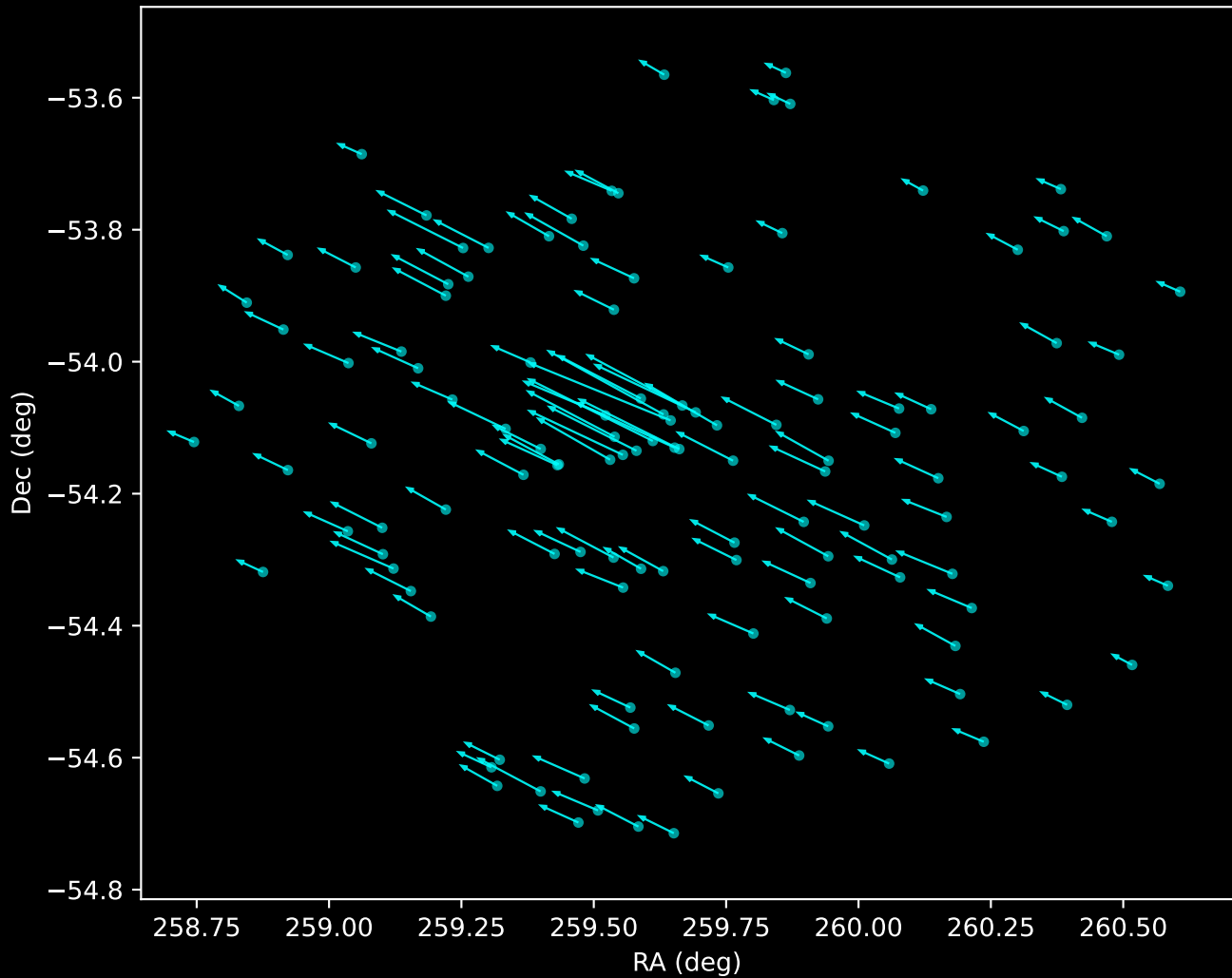
Gaia DR3 Noise Stream Proper Motion Vectors (n=126)
