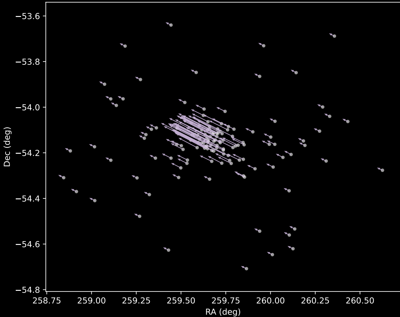
Gaia DR3 Cluster 9 Proper Motion Vectors (n=134)
