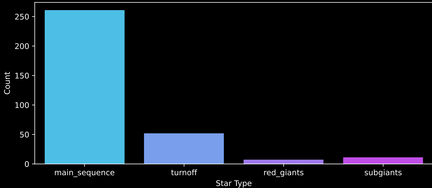
Gaia Cluster: [NGC_3330] Count plot of Star Type
