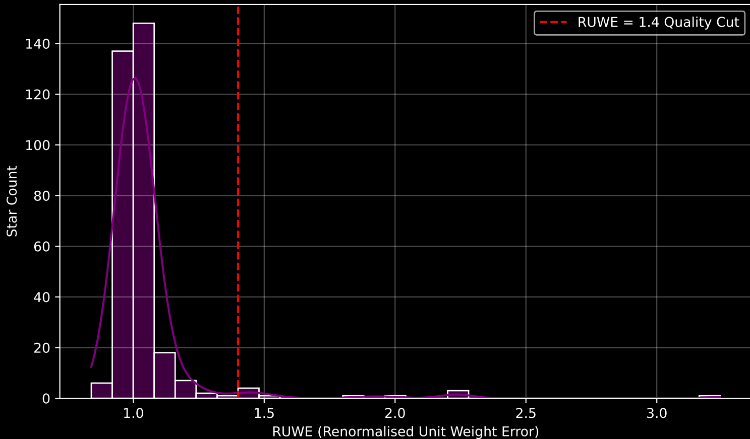
Gaia Cluster: [NGC_3330] RUWE Distribution (n= 330)
