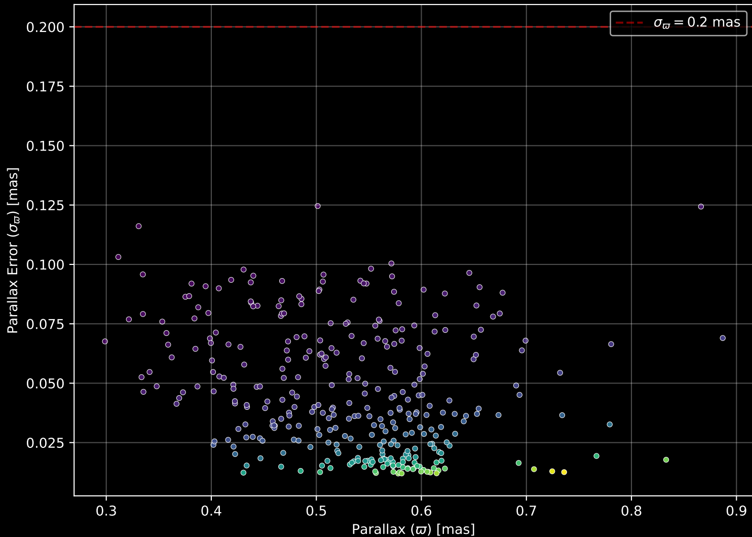
Gaia Cluster: [NGC_3330] Parallax Quality (n= 331)
