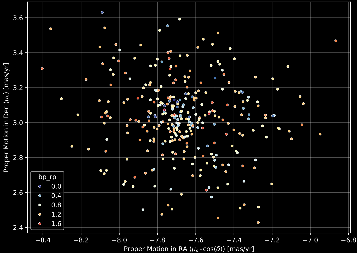
Gaia Cluster: [NGC_3330] Proper Motion Diagram (n= 331)
