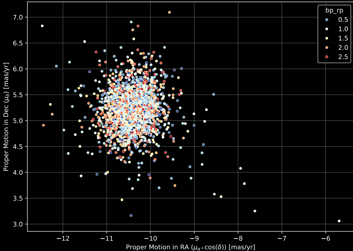
Gaia Cluster: [NGC_3532] Proper Motion Diagram (n= 1694)
