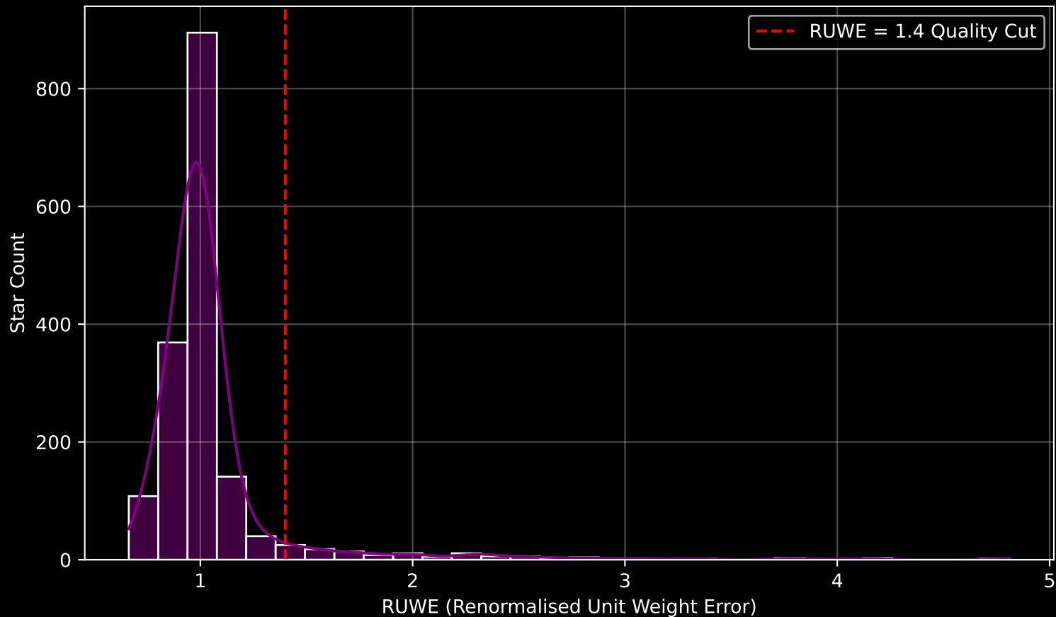
Gaia Cluster: [NGC_3532] RUWE Distribution (n= 1680)
