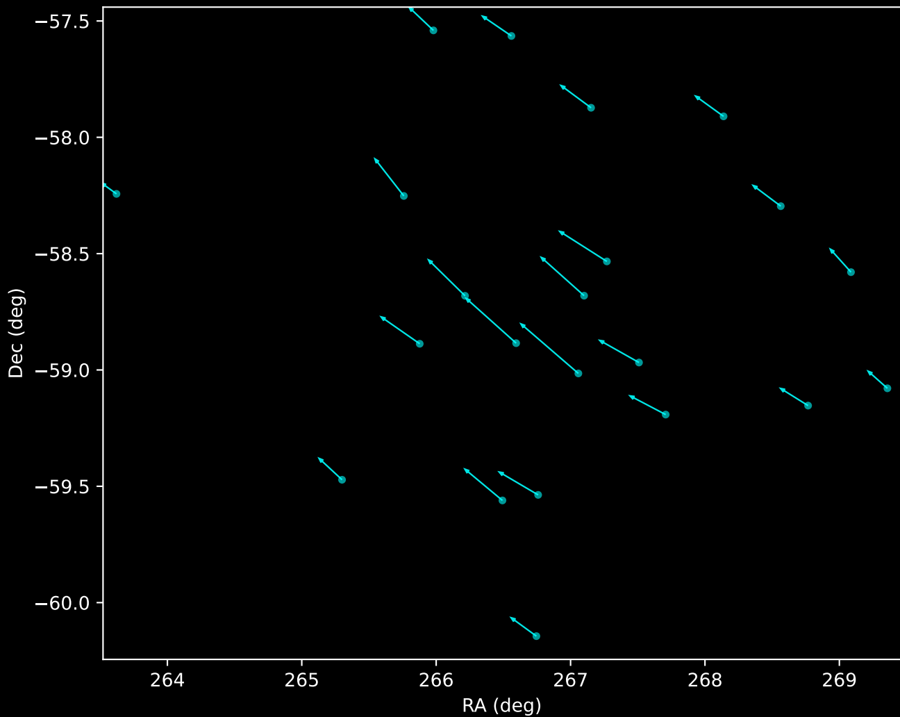
Gaia DR3 Noise Stream Proper Motion Vectors (n=22)
