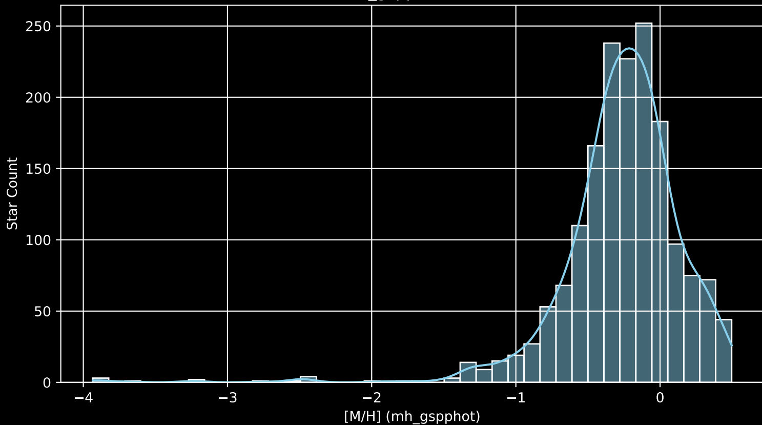
Gaia Cluster: [NGC_3532 [M/H] (mh_gspphot) (n= 1687)
