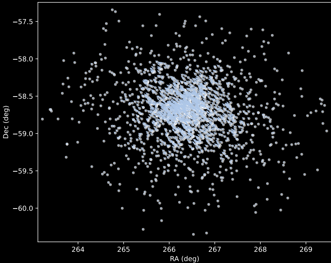
Gaia DR3 Cluster 1 Proper Motion Vectors (n=1667)
