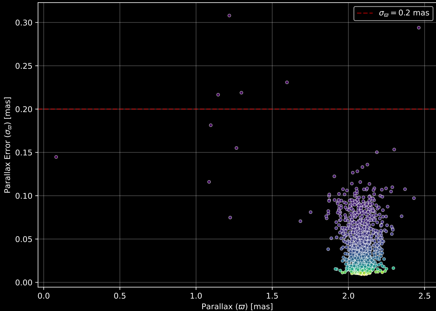
Gaia Cluster: [NGC_3532] Parallax Quality (n= 1694)
