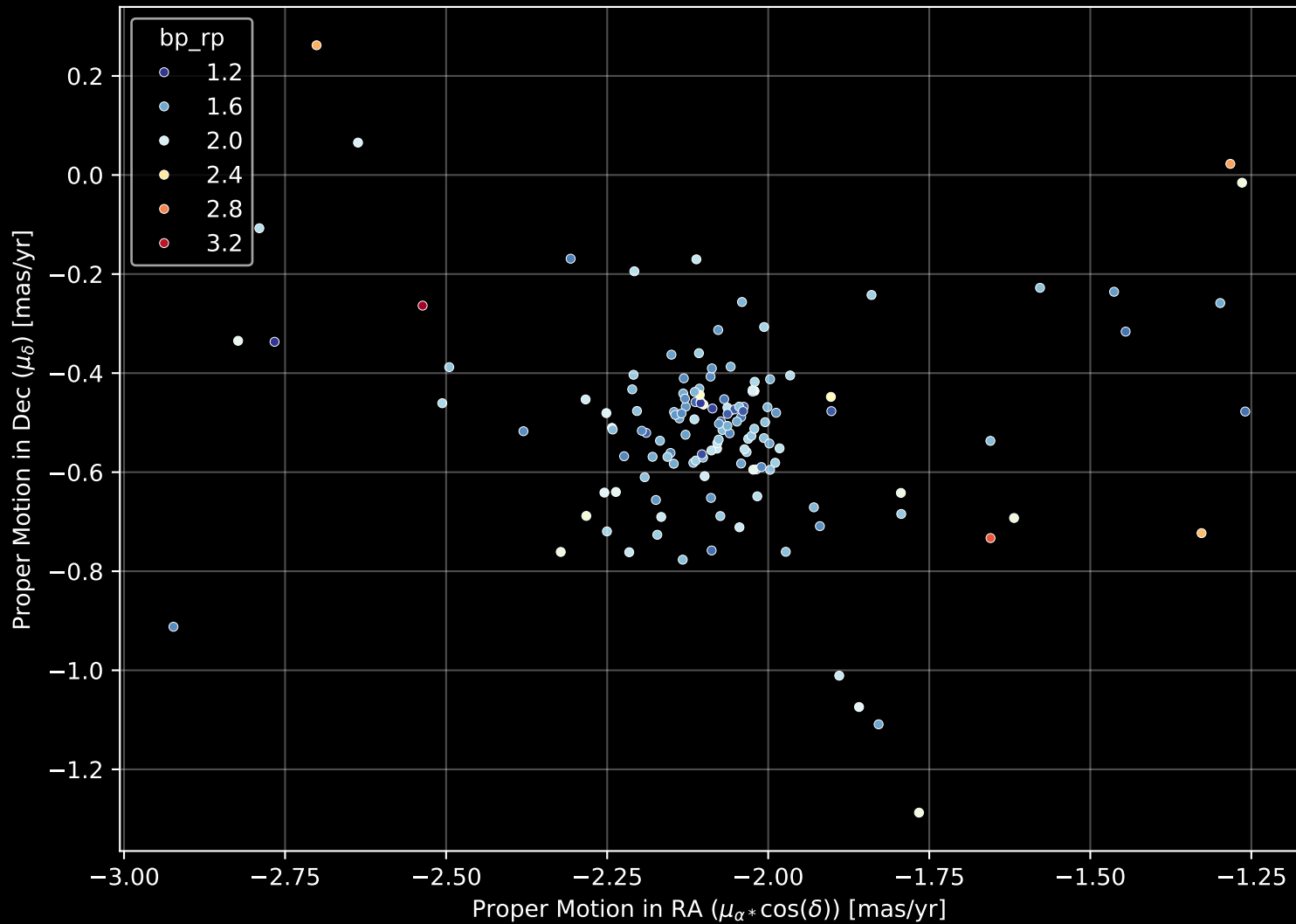
Gaia Cluster: [NGC_366] Proper Motion Diagram (n= 140)
