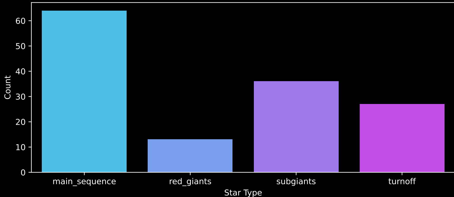
Gaia Cluster: [NGC_366] Count plot of Star Type
