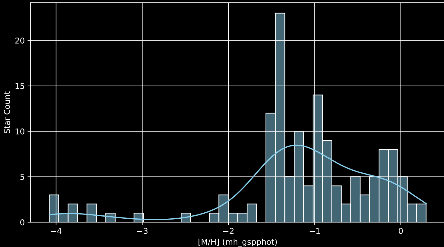
Gaia Cluster: [NGC_366 [M/H] (mh_gspphot) (n= 140)
