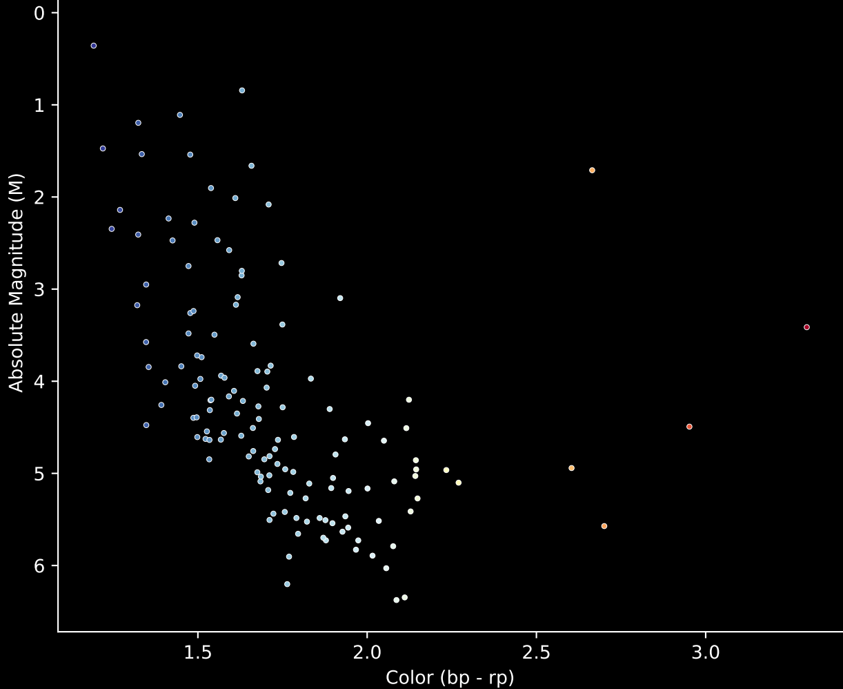
Gaia Cluster: [NGC_366] Stars (n= 140) Hertzsprung-Russel Diagram
