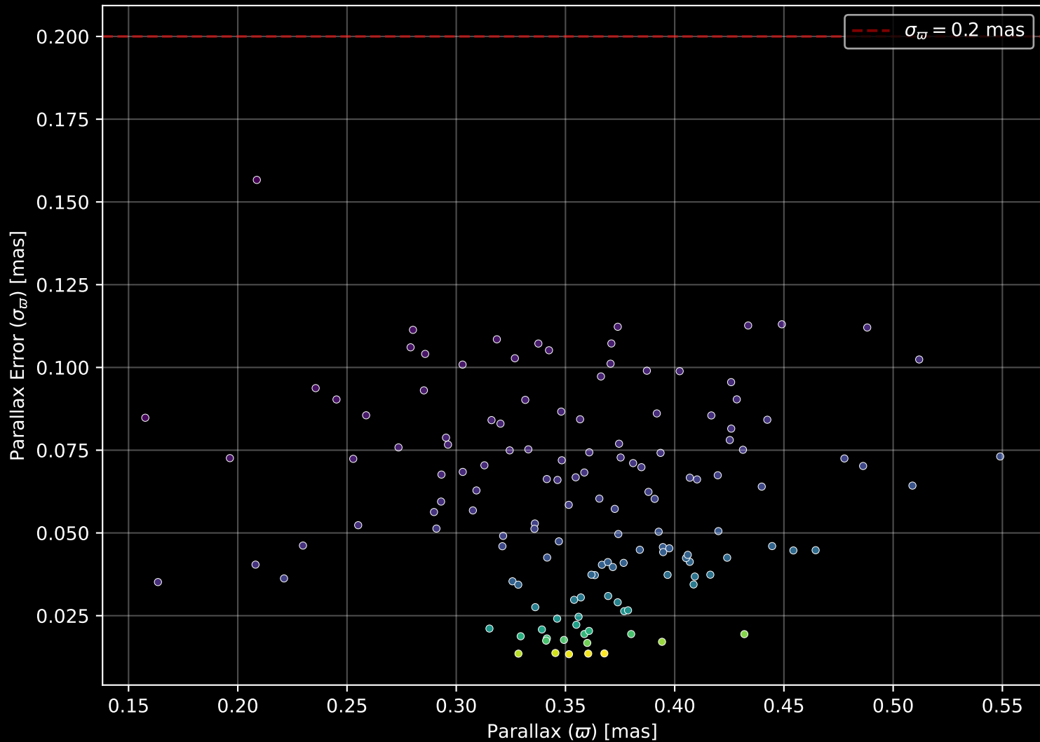
Gaia Cluster: [NGC_366] Parallax Quality (n= 140)
