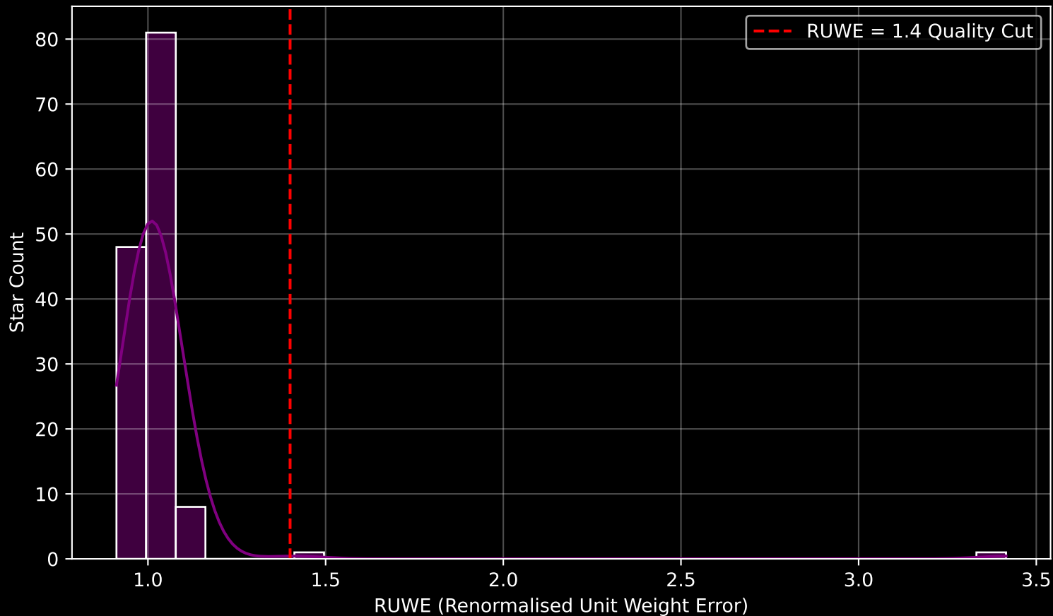
Gaia Cluster: [NGC_366] RUWE Distribution (n= 139)
