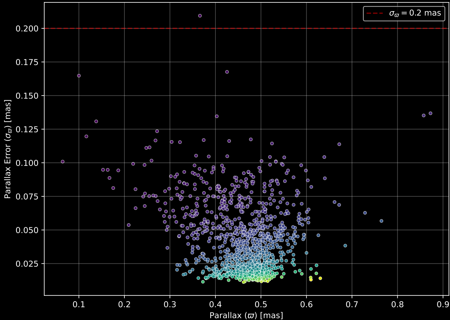
Gaia Cluster: [NGC_3766] Parallax Quality (n= 1197)
