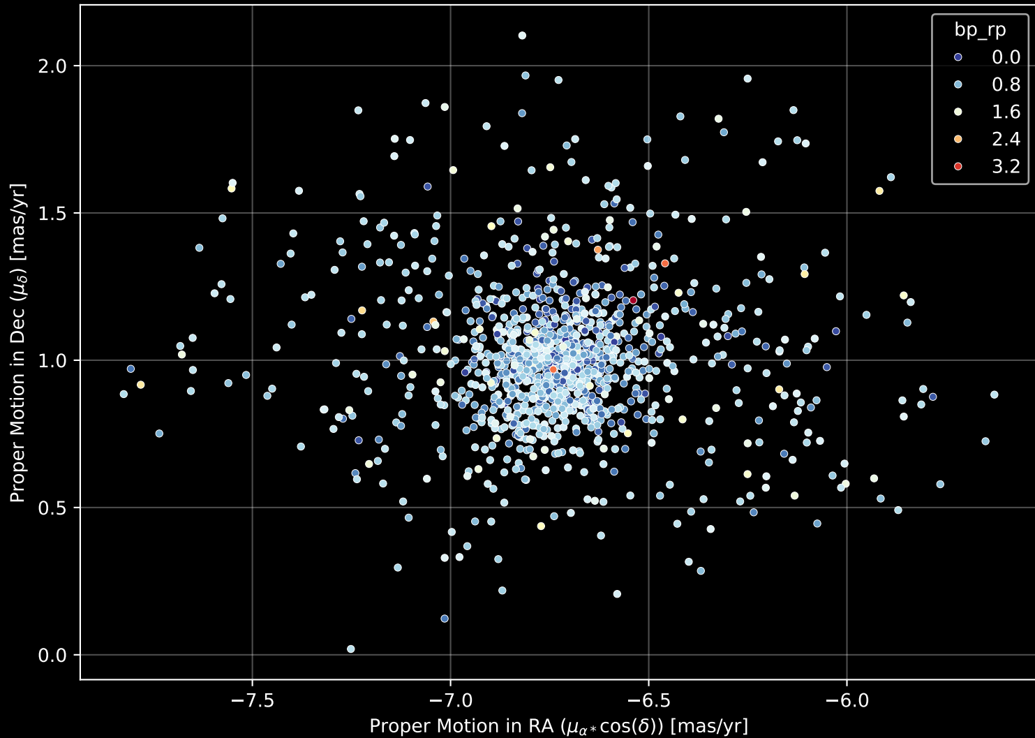
Gaia Cluster: [NGC_3766] Proper Motion Diagram (n= 1197)
