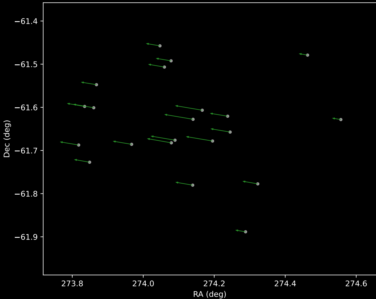
Gaia DR3 Cluster 44 Proper Motion Vectors (n=21)
