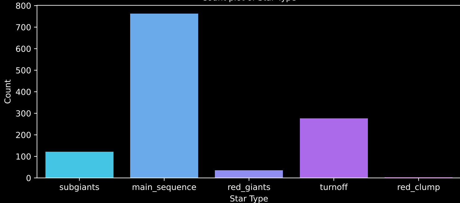
Gaia Cluster: [NGC_3766] Count plot of Star Type
