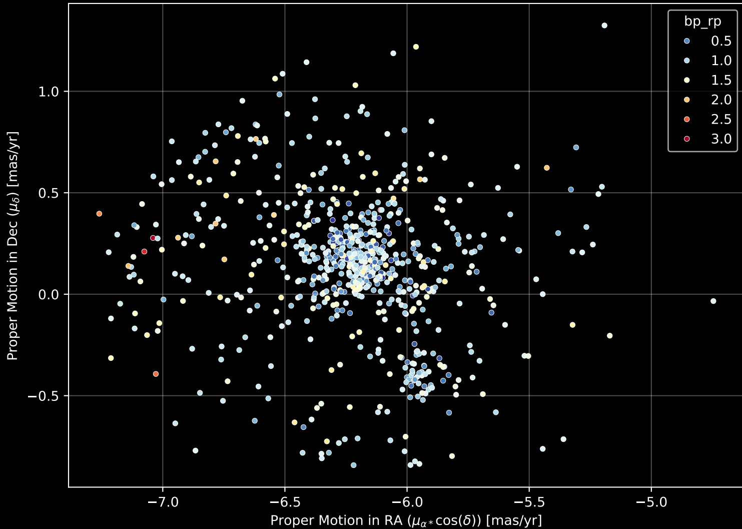
Gaia Cluster: [NGC_4103] Proper Motion Diagram (n= 729)
