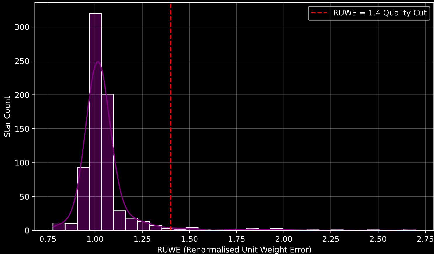
Gaia Cluster: [NGC_4103] RUWE Distribution (n= 727)
