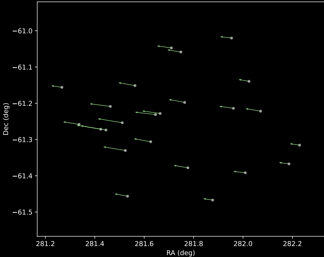
Gaia DR3 Cluster 5 Proper Motion Vectors (n=24)
