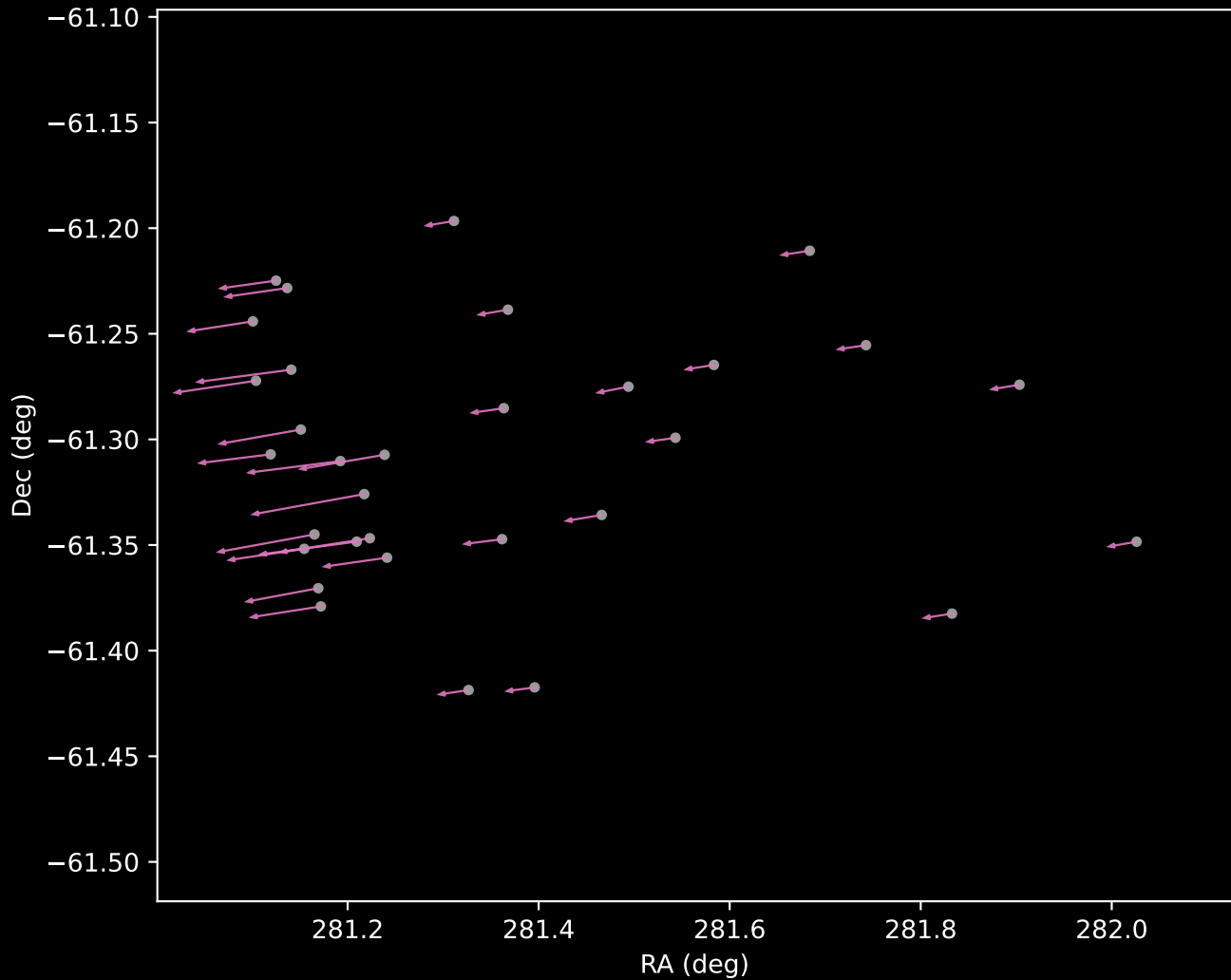
Gaia DR3 Cluster 12 Proper Motion Vectors (n=32)
