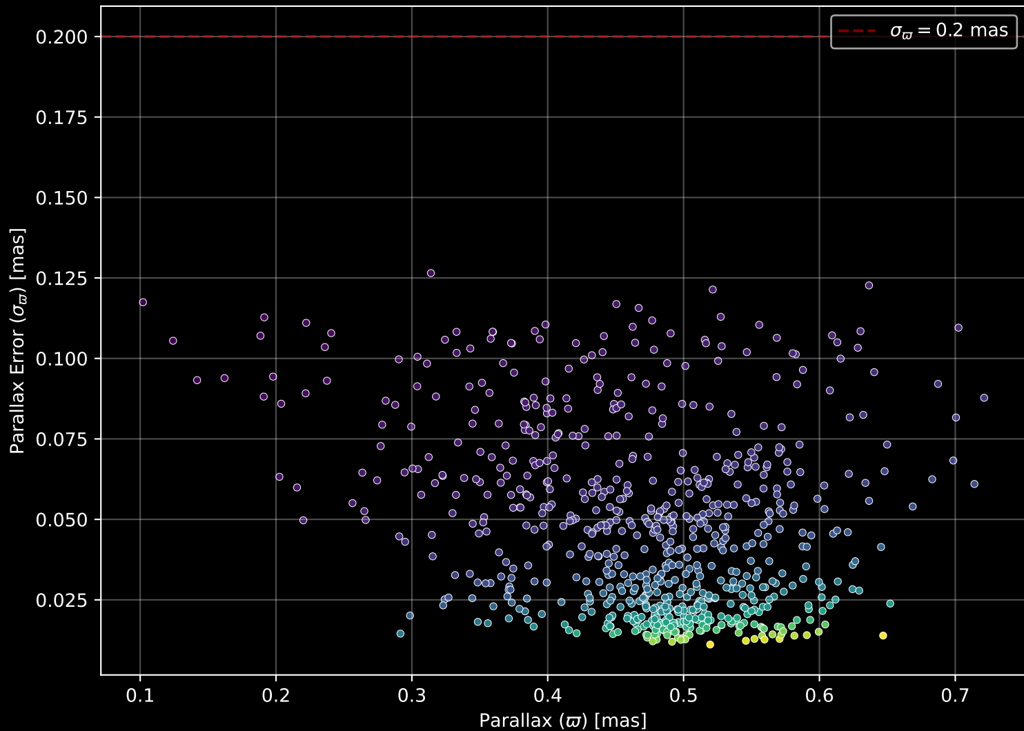
Gaia Cluster: [NGC_4103] Parallax Quality (n= 729)
