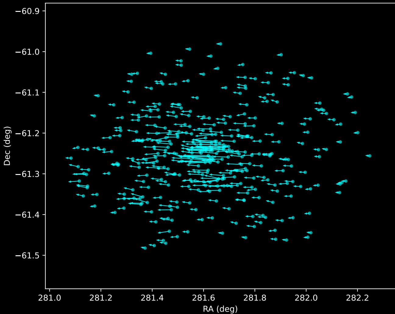
Gaia DR3 Noise Stream Proper Motion Vectors (n=336)
