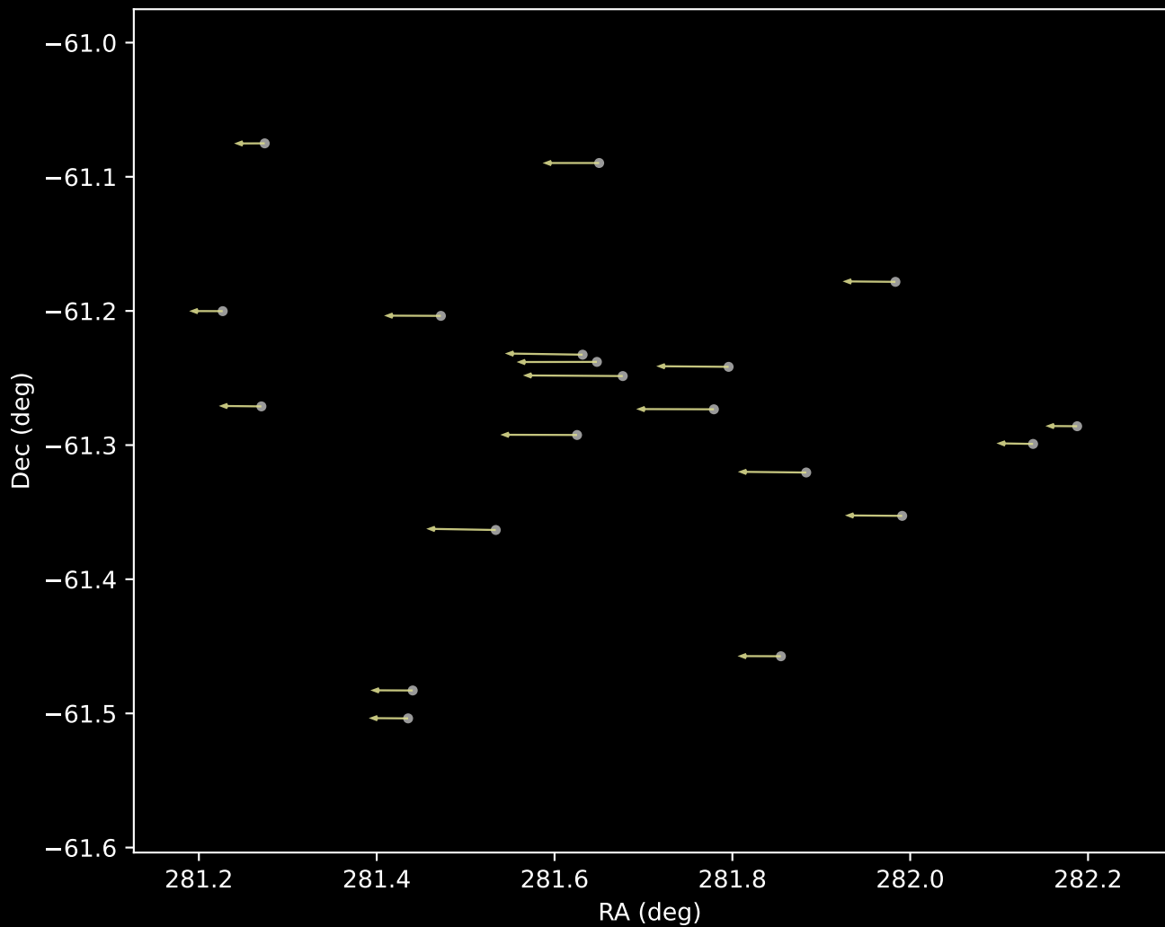
Gaia DR3 Cluster 17 Proper Motion Vectors (n=20)
