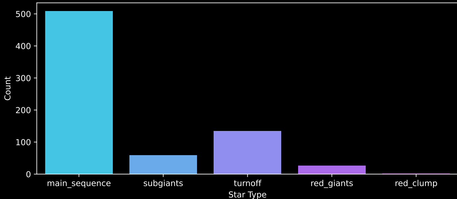
Gaia Cluster: [NGC_4103] Count plot of Star Type
