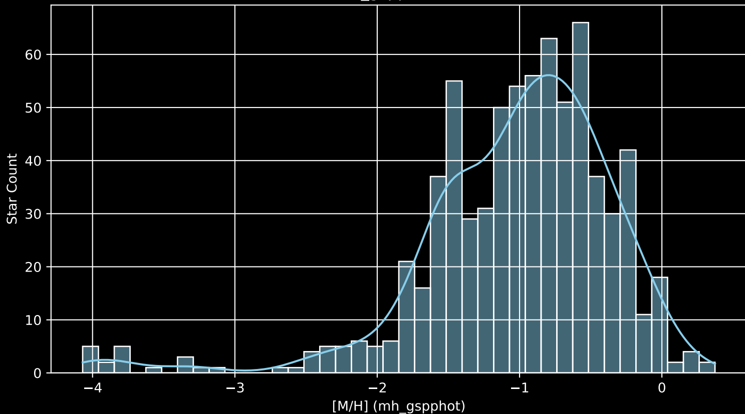
Gaia Cluster: [NGC_4103 [M/H] (mh_gspphot) (n= 726)
