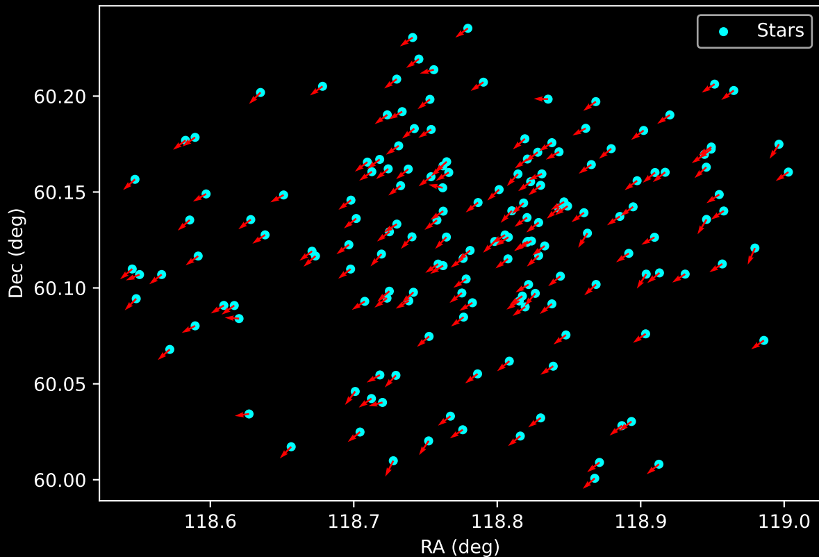
Gaia Cluster: [NGC_433] Proper Motion Vectors for Gaia Star Field (n= 162)
