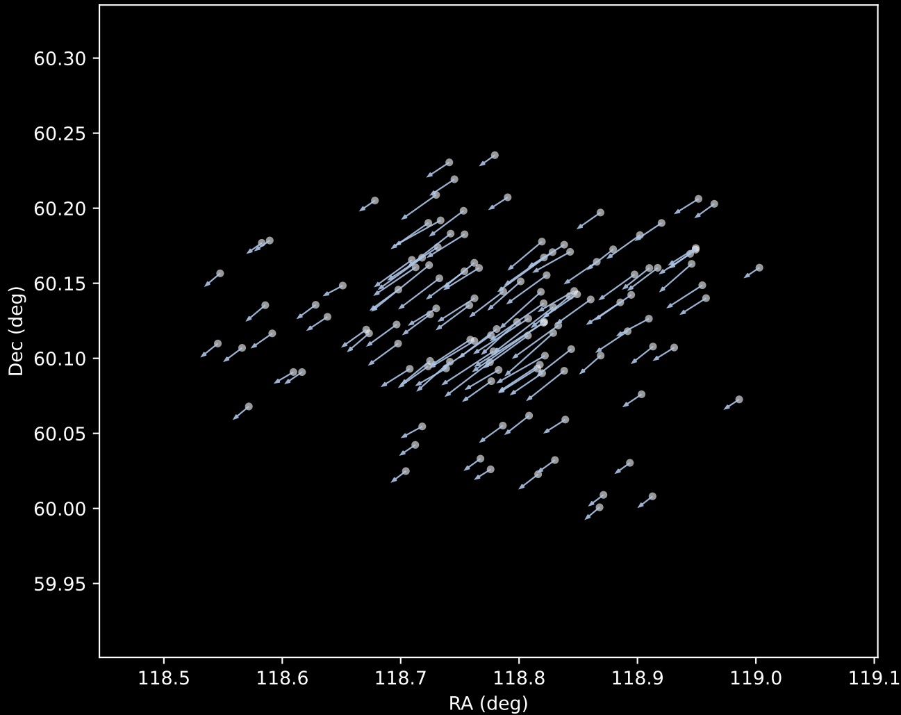
Gaia DR3 Cluster 1 Proper Motion Vectors (n=123)
