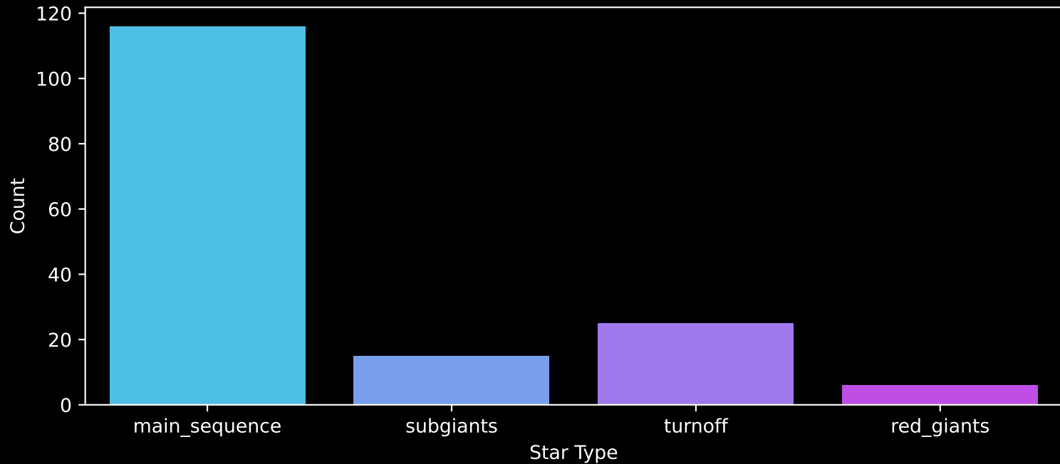
Gaia Cluster: [NGC_433] Count plot of Star Type
