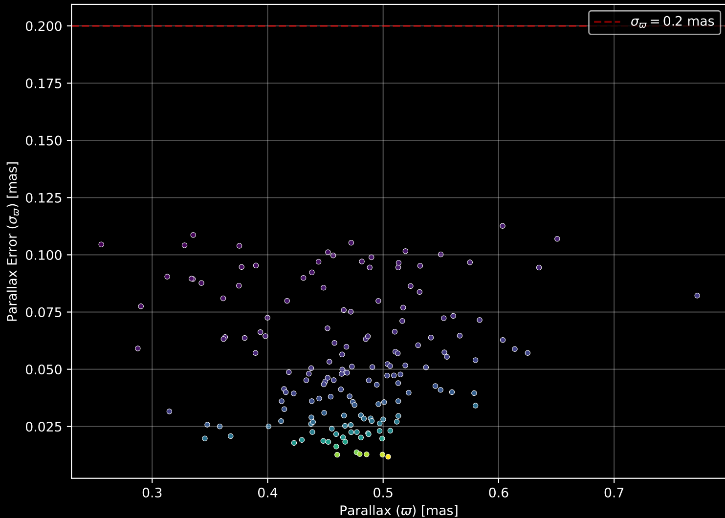
Gaia Cluster: [NGC_433] Parallax Quality (n= 162)
