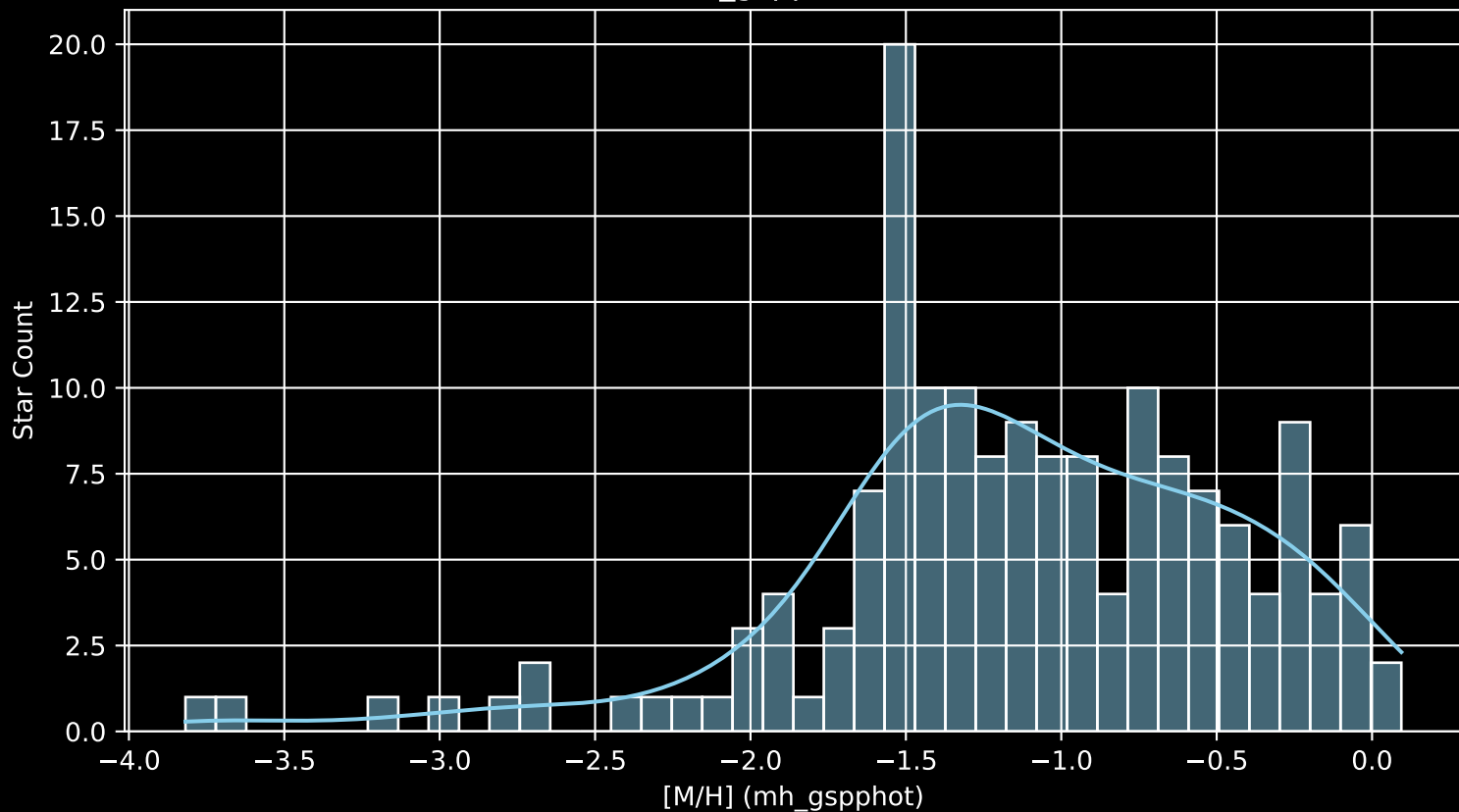
Gaia Cluster: [NGC_433 [M/H] (mh_gspphot) (n= 162)
