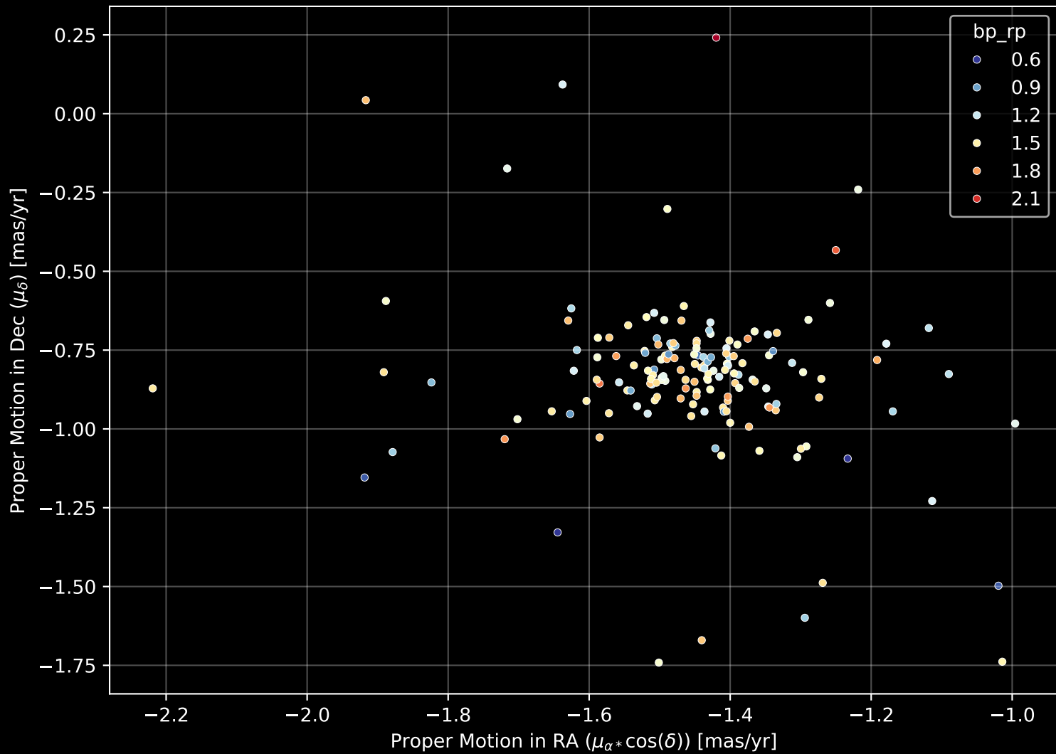
Gaia Cluster: [NGC_433] Proper Motion Diagram (n= 162)
