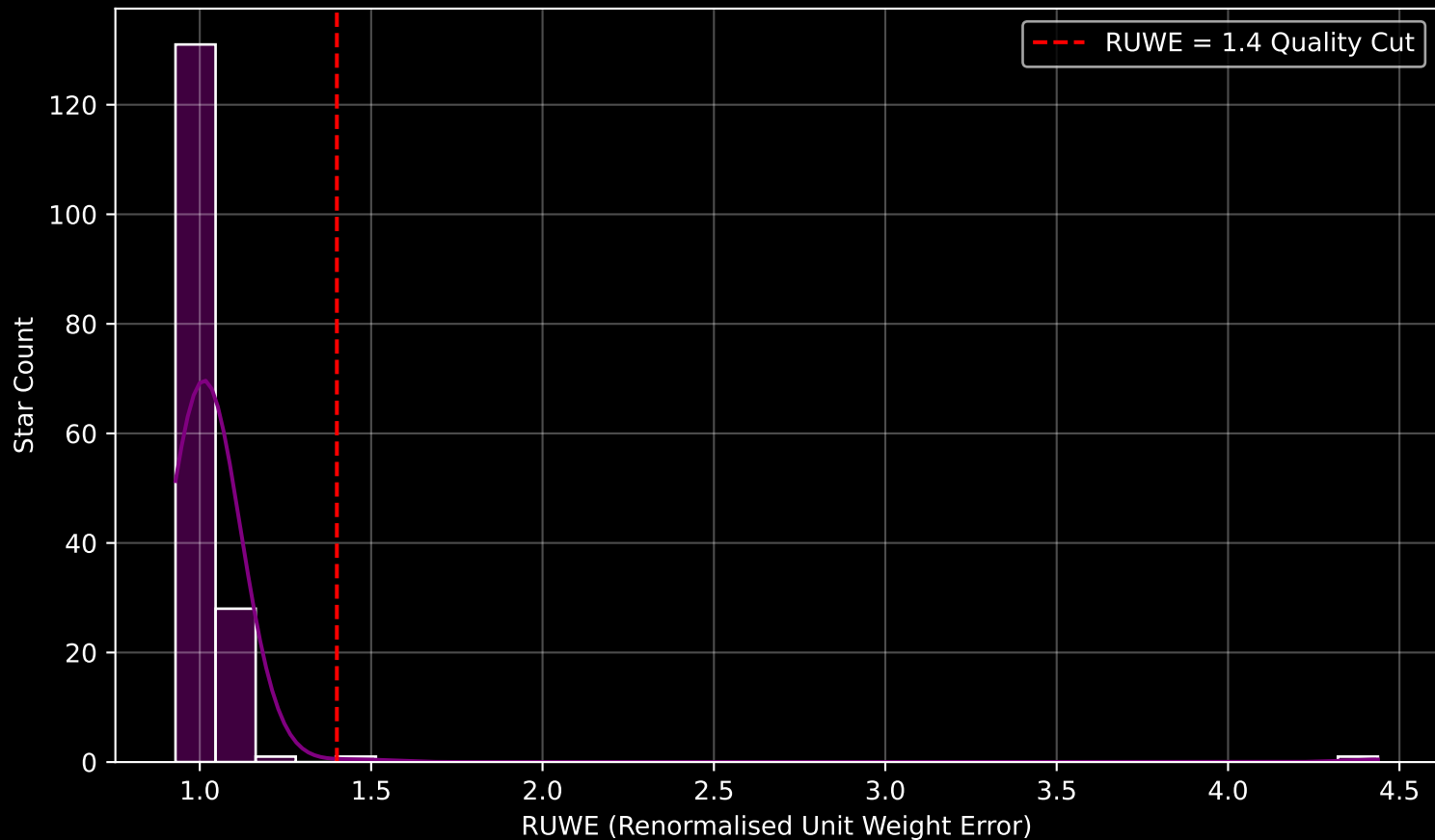
Gaia Cluster: [NGC_433] RUWE Distribution (n= 162)
