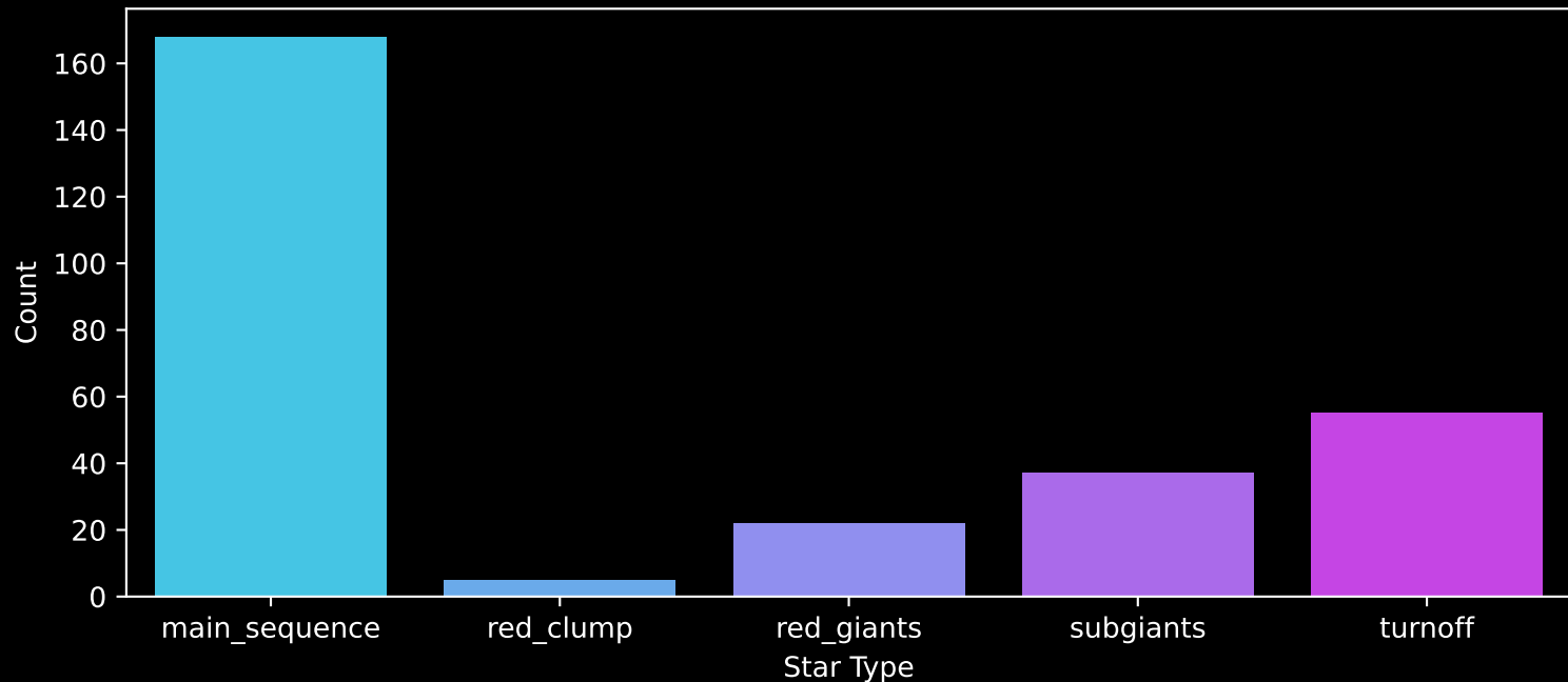
Gaia Cluster: [NGC_4337] Count plot of Star Type
