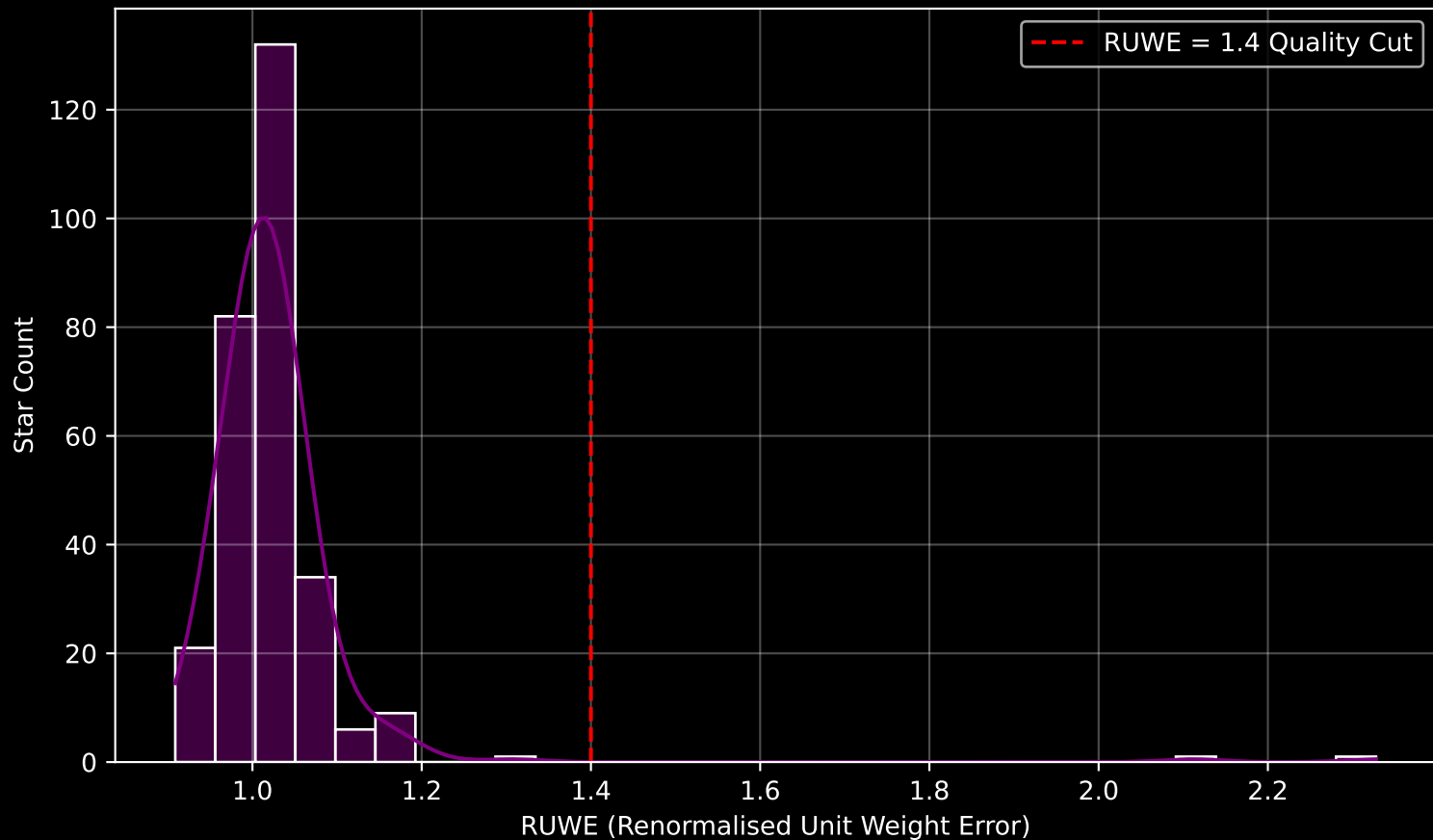
Gaia Cluster: [NGC_4337] RUWE Distribution (n= 287)
