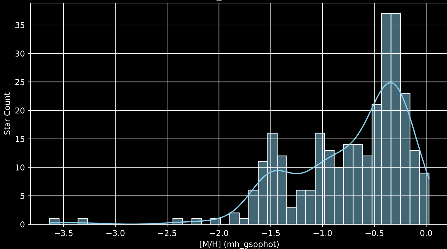
Gaia Cluster: [NGC_4337 [M/H] (mh_gspphot) (n= 287)
