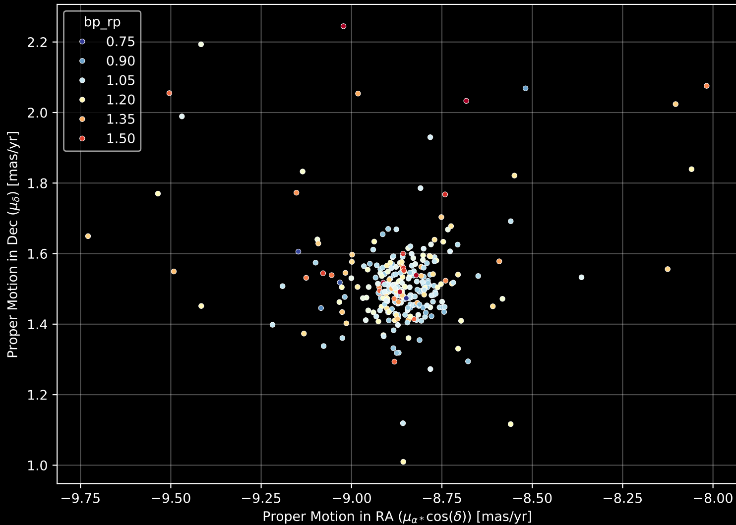
Gaia Cluster: [NGC_4337] Proper Motion Diagram (n= 287)
