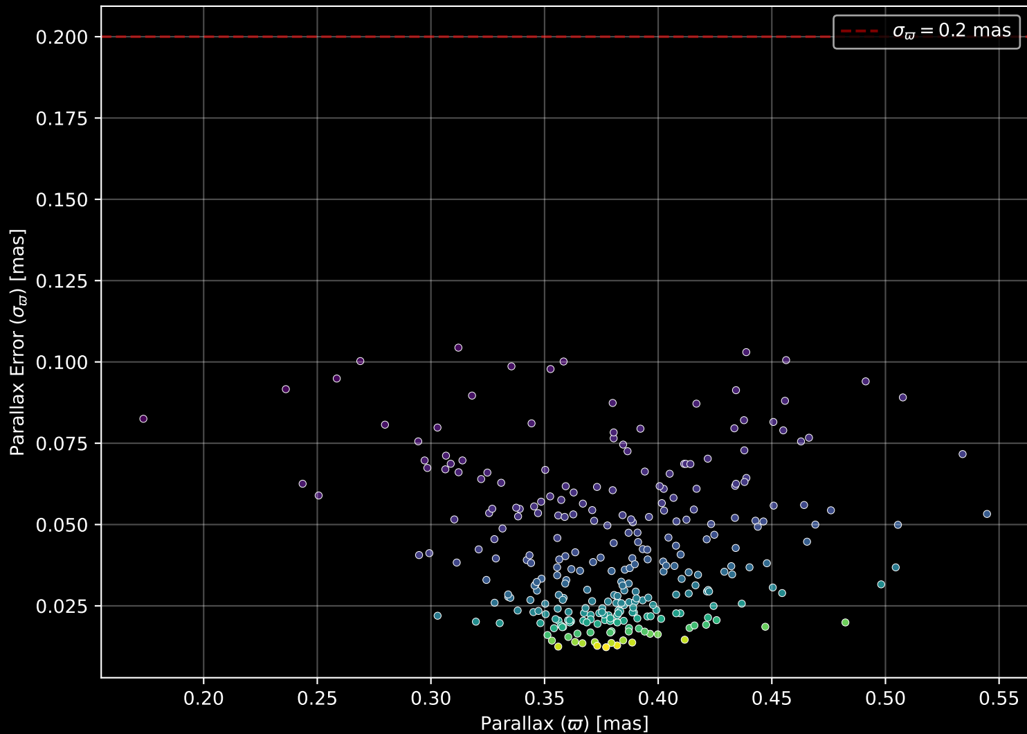
Gaia Cluster: [NGC_4337] Parallax Quality (n= 287)
