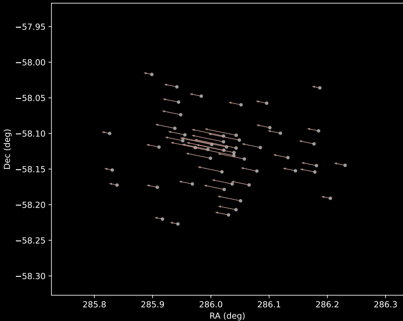
Gaia DR3 Cluster 11 Proper Motion Vectors (n=52)
