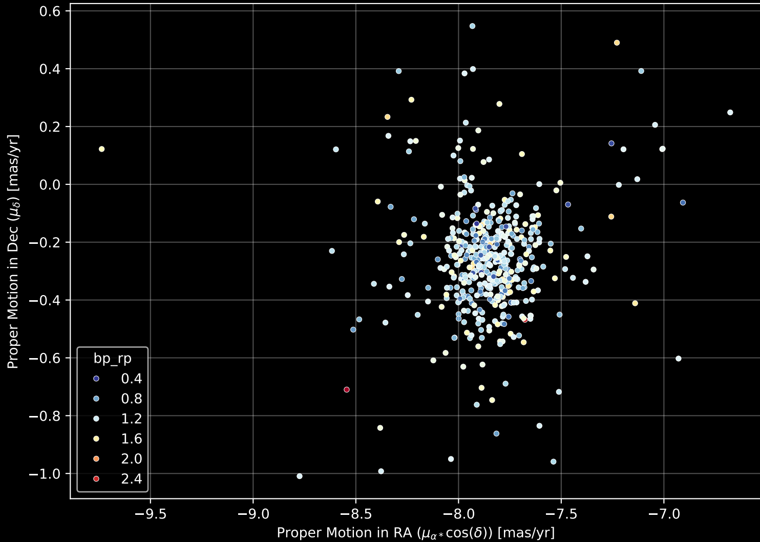
Gaia Cluster: [NGC_4349] Proper Motion Diagram (n= 482)
