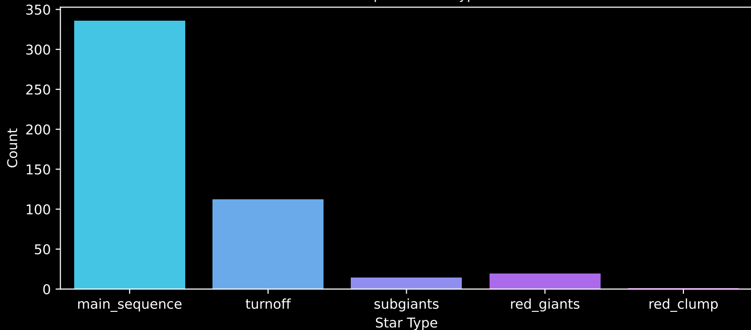
Gaia Cluster: [NGC_4349] Count plot of Star Type
