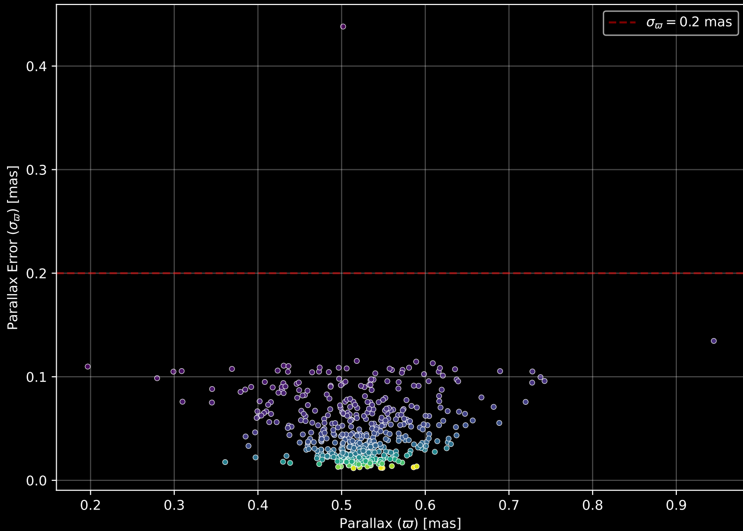
Gaia Cluster: [NGC_4349] Parallax Quality (n= 482)
