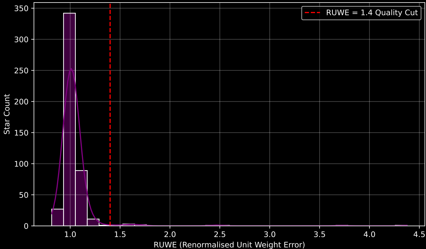
Gaia Cluster: [NGC_4349] RUWE Distribution (n= 480)
