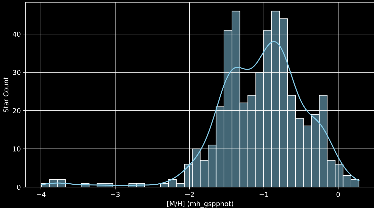
Gaia Cluster: [NGC_4349 [M/H] (mh_gspphot) (n= 482)
