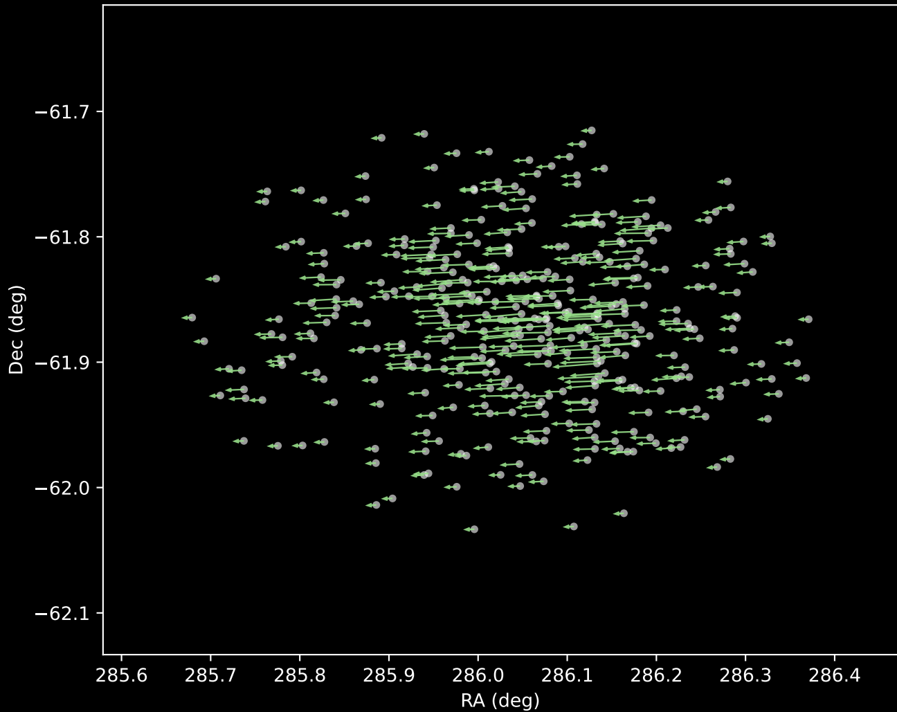
Gaia DR3 Cluster 5 Proper Motion Vectors (n=370)
