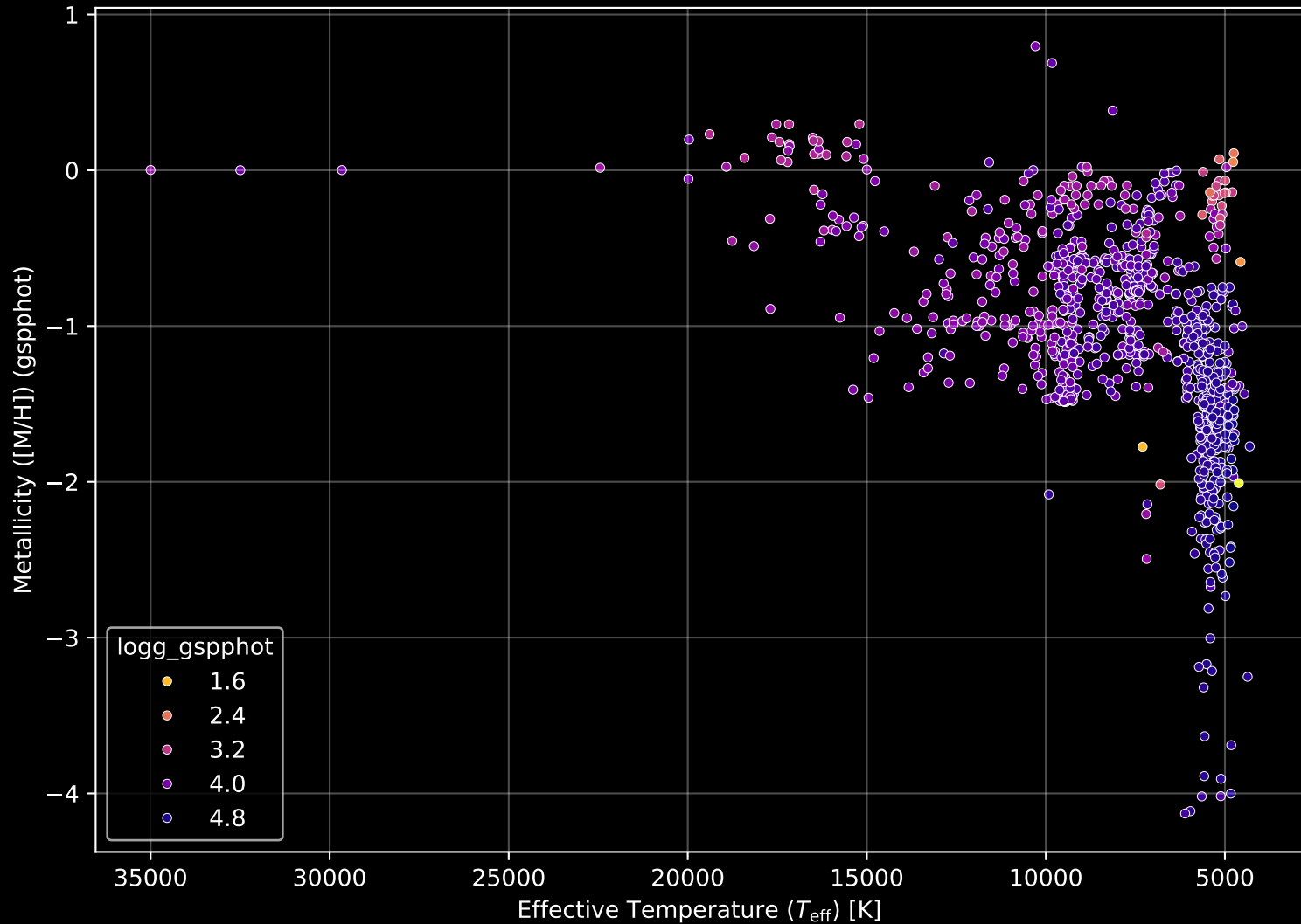
Gaia Cluster: [NGC_457] Stellar Population Parameters (n= 1017)
