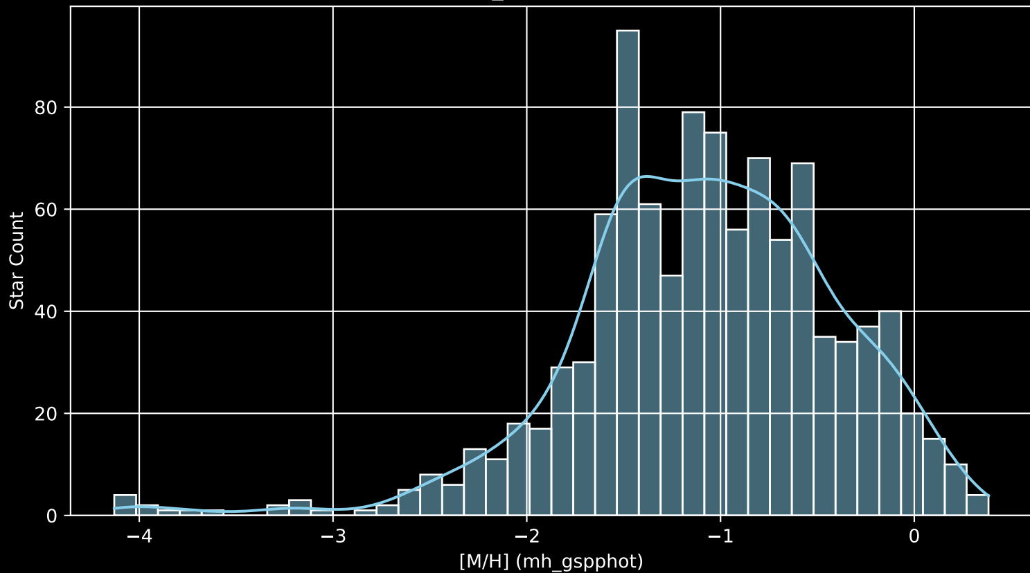
Gaia Cluster: [NGC_457 [M/H] (mh_gspphot) (n= 1015)
