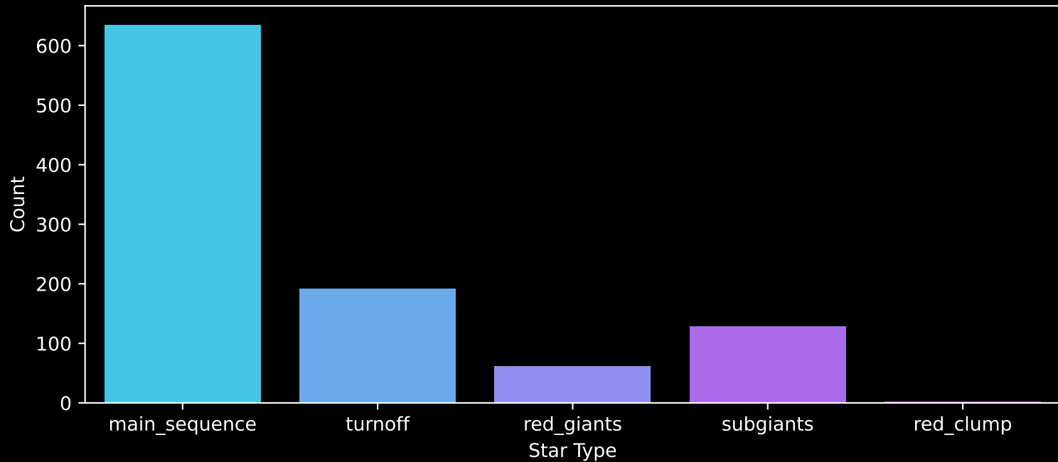
Gaia Cluster: [NGC_457] Count plot of Star Type
