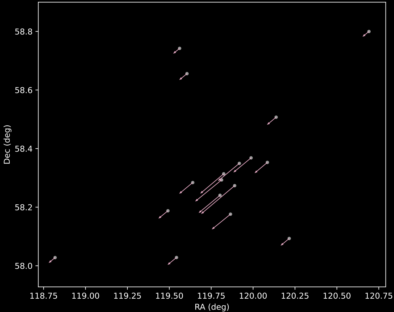
Gaia DR3 Cluster 53 Proper Motion Vectors (n=17)
