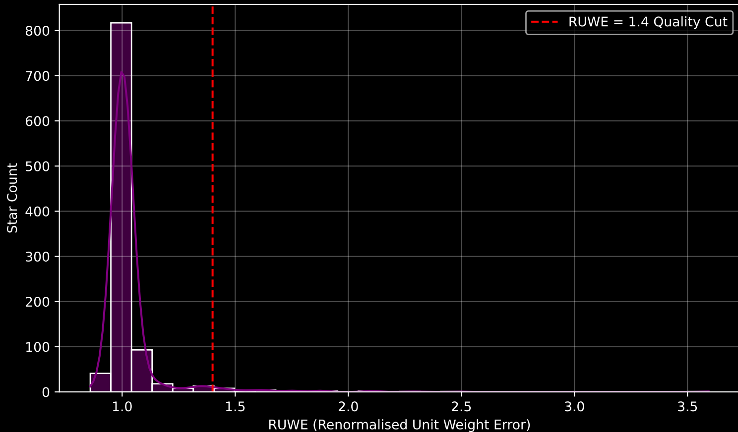
Gaia Cluster: [NGC_457] RUWE Distribution (n= 1016)
