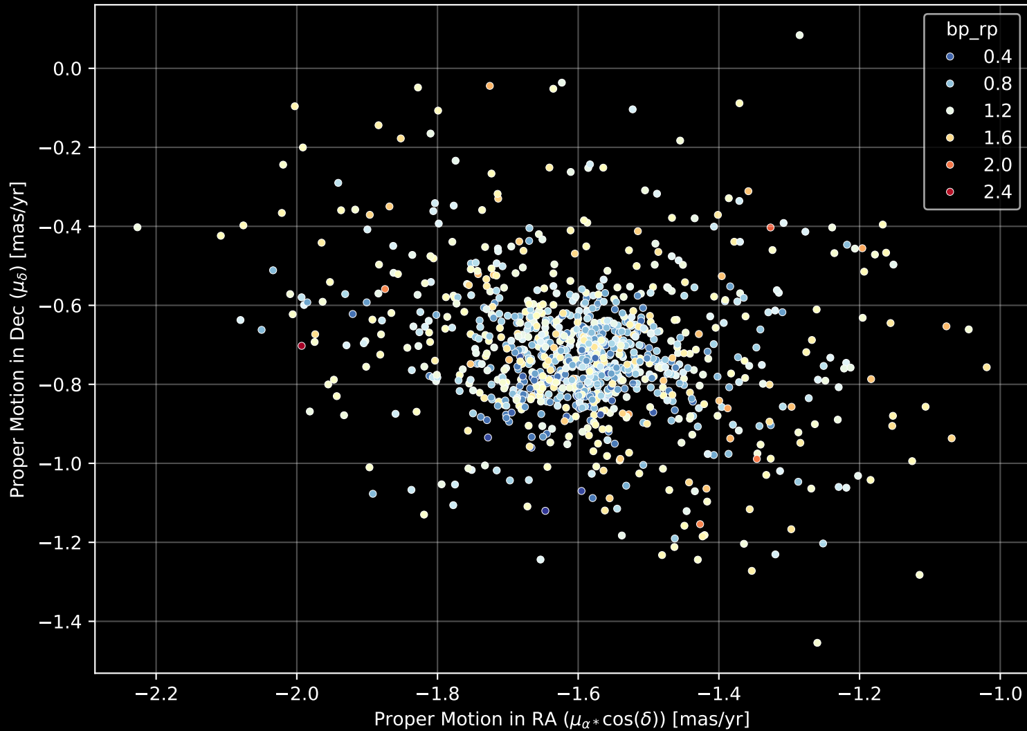
Gaia Cluster: [NGC_457] Proper Motion Diagram (n= 1017)
