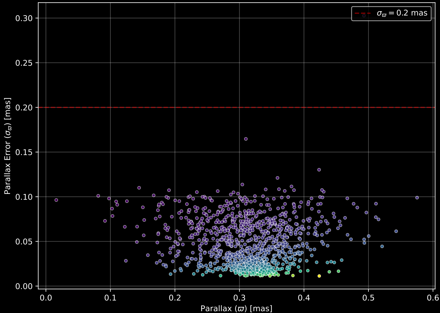
Gaia Cluster: [NGC_457] Parallax Quality (n= 1017)
