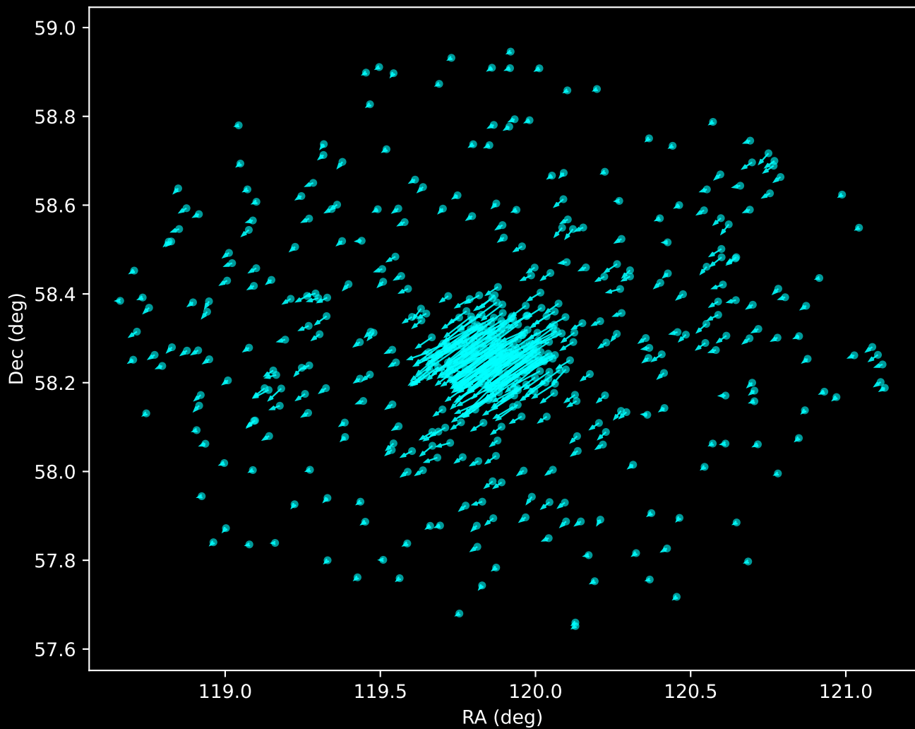
Gaia DR3 Noise Stream Proper Motion Vectors (n=504)
