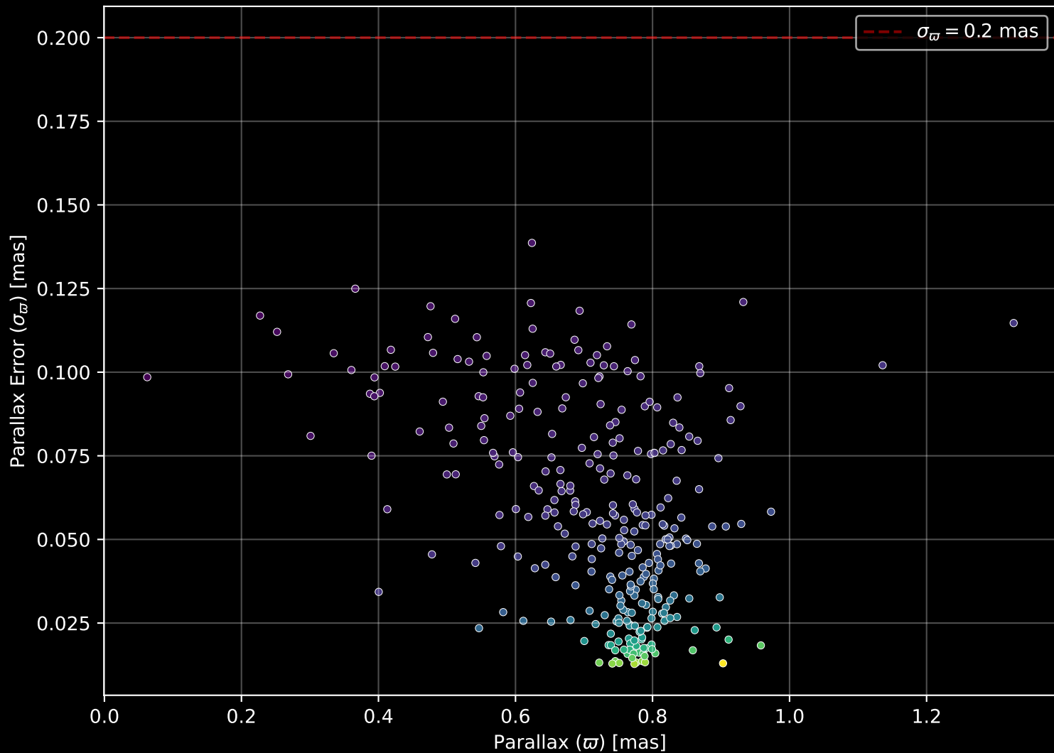
Gaia Cluster: [NGC_4852] Parallax Quality (n= 308)
