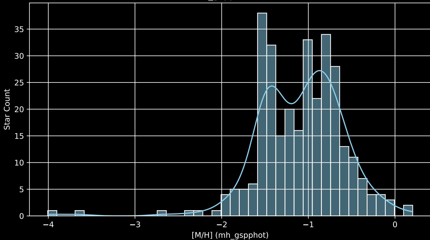
Gaia Cluster: [NGC_4852 [M/H] (mh_gspphot) (n= 308)
