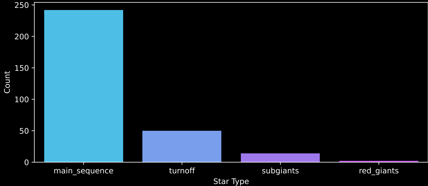
Gaia Cluster: [NGC_4852] Count plot of Star Type
