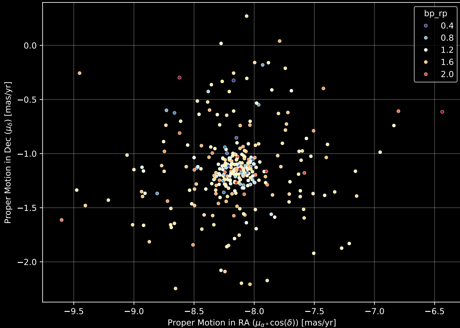
Gaia Cluster: [NGC_4852] Proper Motion Diagram (n= 308)
