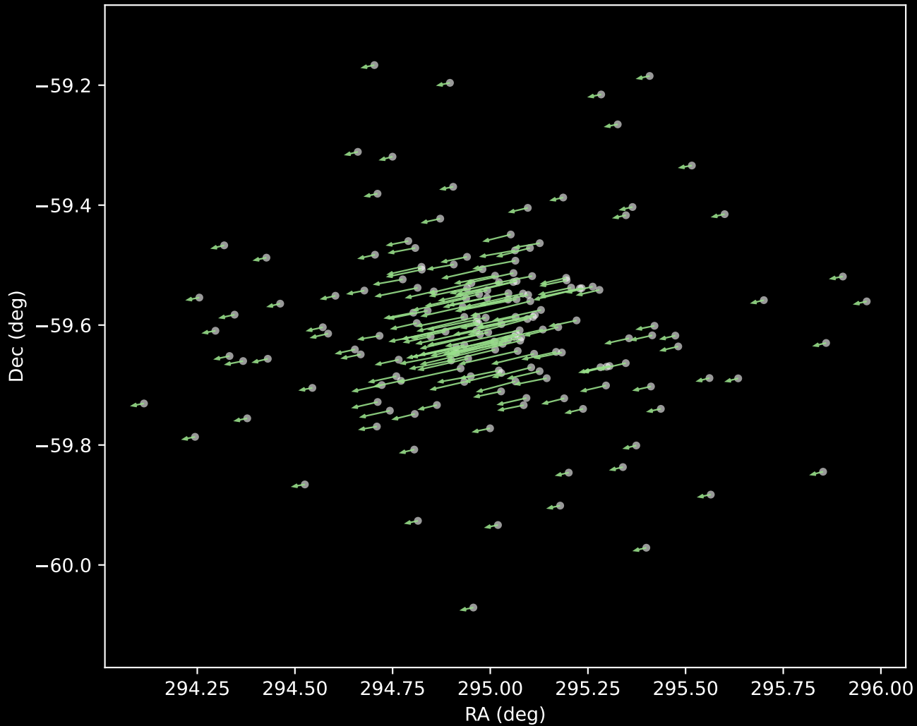
Gaia DR3 Cluster 5 Proper Motion Vectors (n=172)
