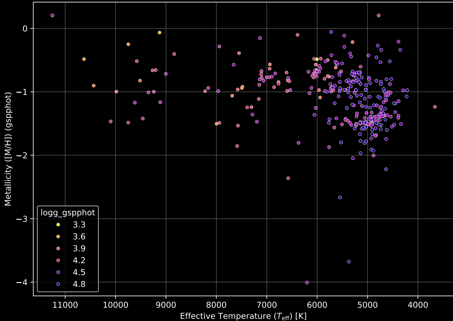
Gaia Cluster: [NGC_4852] Stellar Population Parameters (n= 308)
