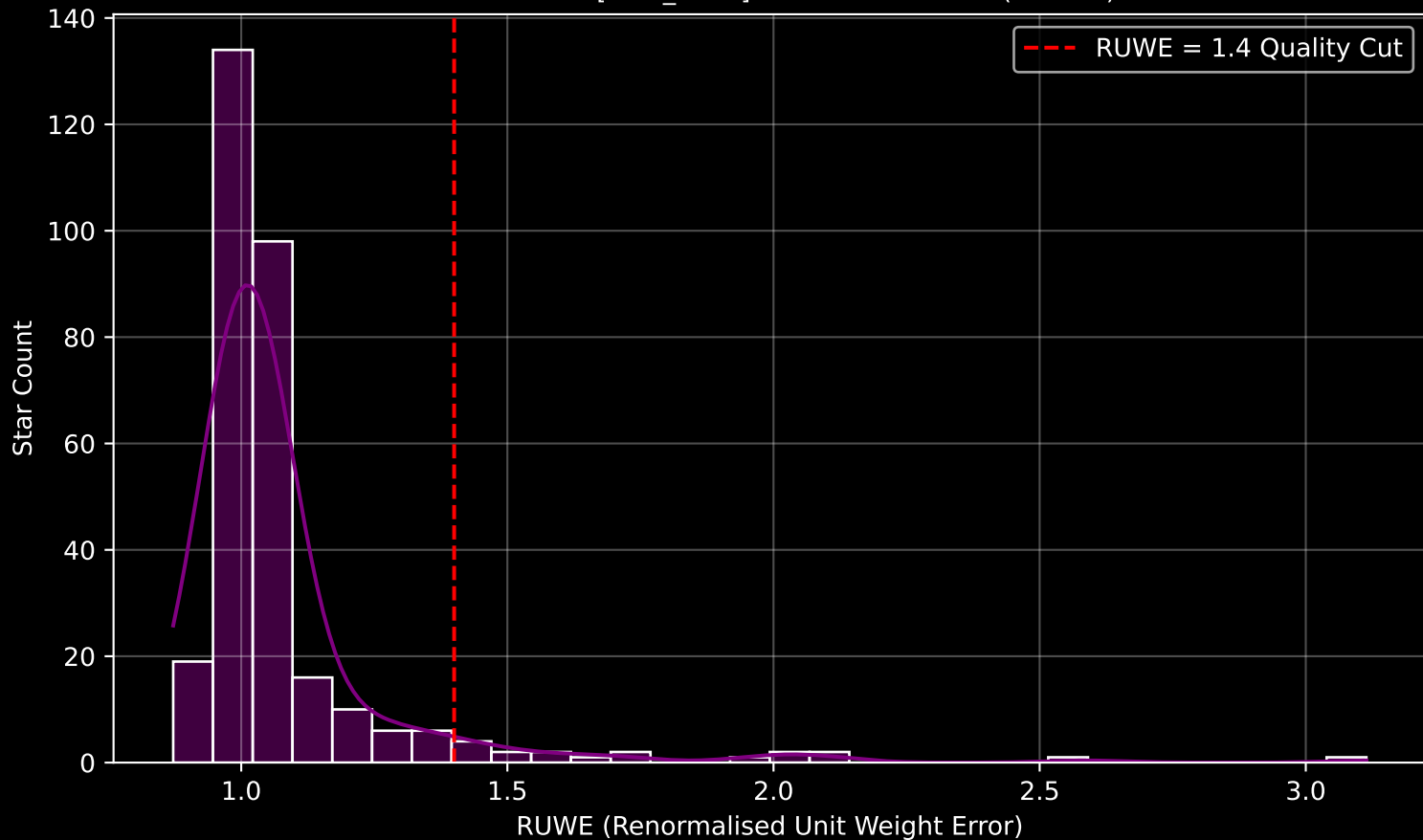
Gaia Cluster: [NGC_4852] RUWE Distribution (n= 307)
