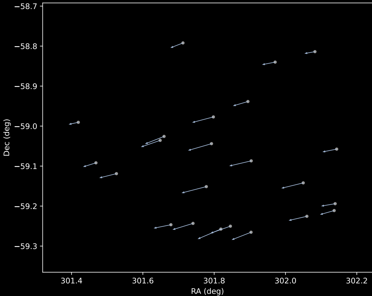
Gaia DR3 Cluster 1 Proper Motion Vectors (n=23)
