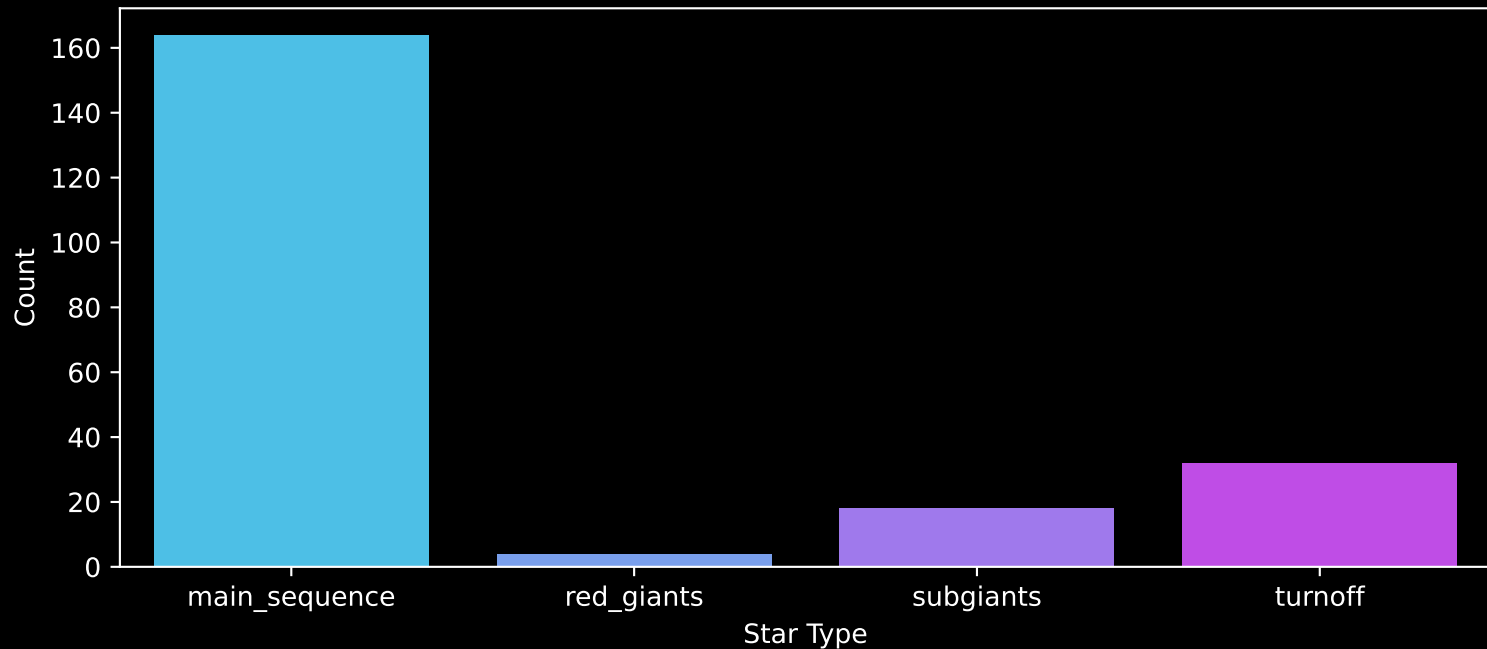
Gaia Cluster: [NGC_5138] Count plot of Star Type
