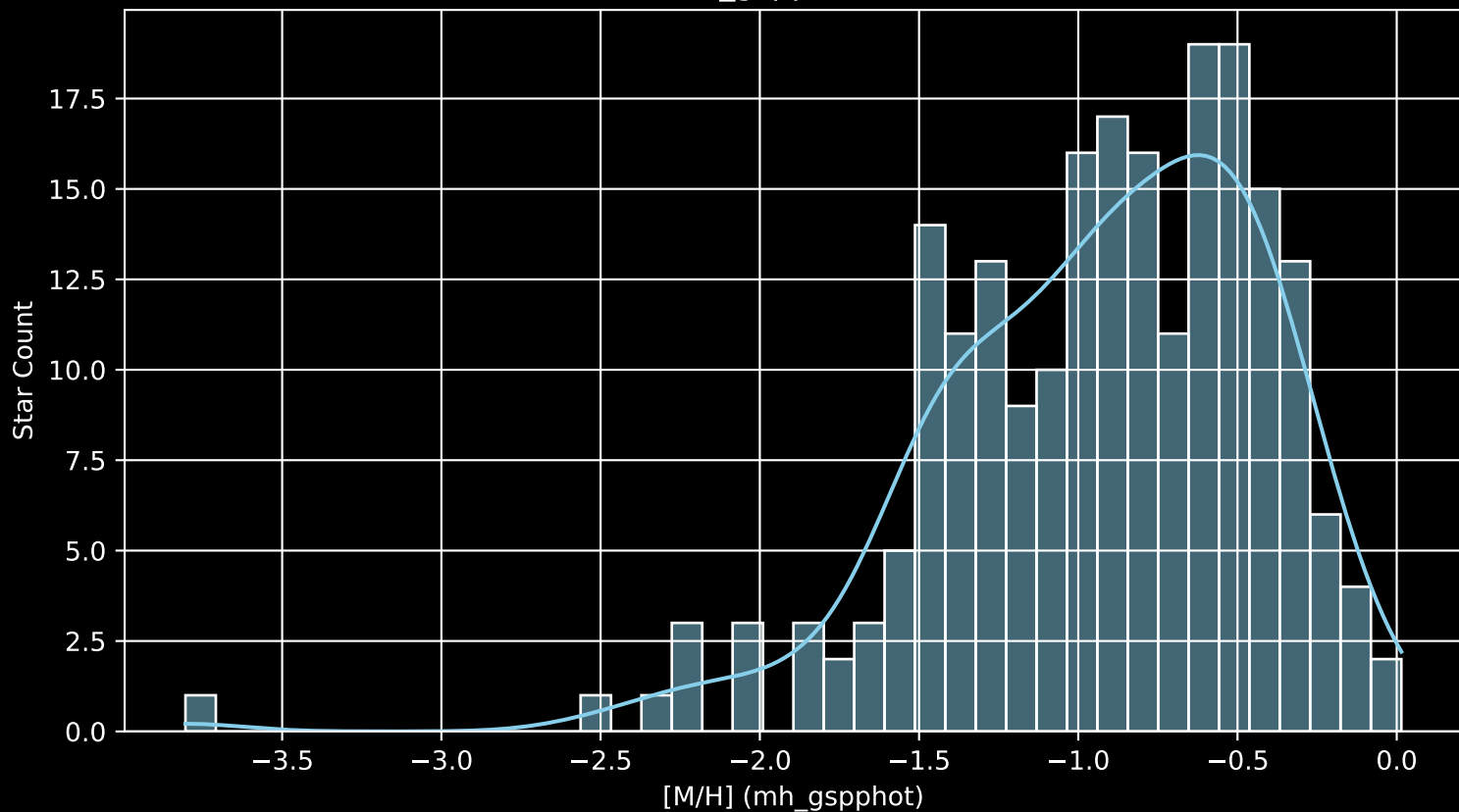
Gaia Cluster: [NGC_5138 [M/H] (mh_gspphot) (n= 217)
