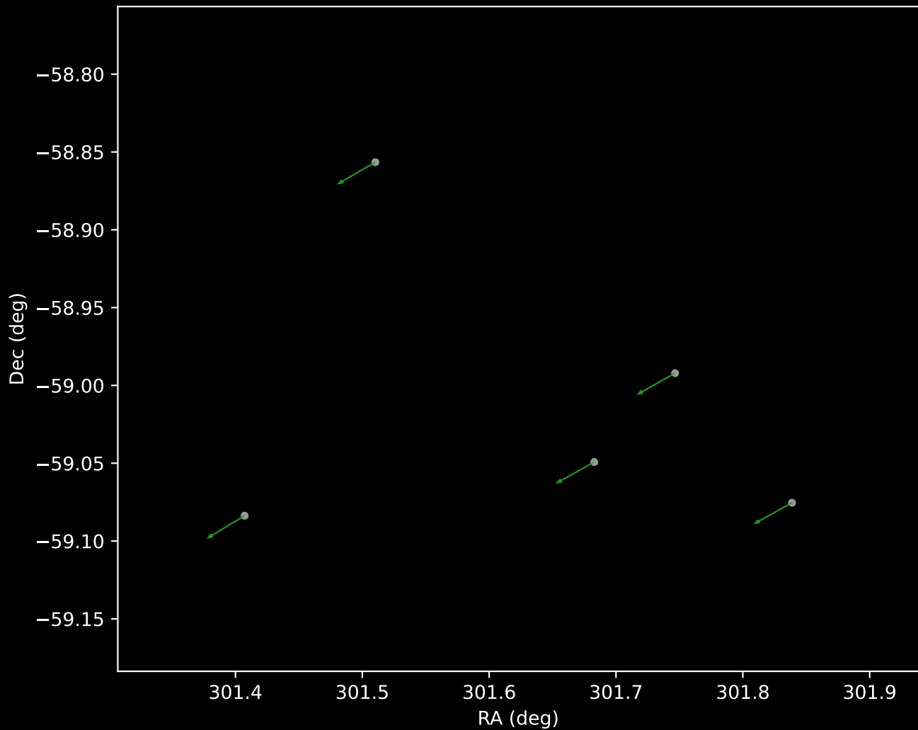
Gaia DR3 Cluster 4 Proper Motion Vectors (n=5)
