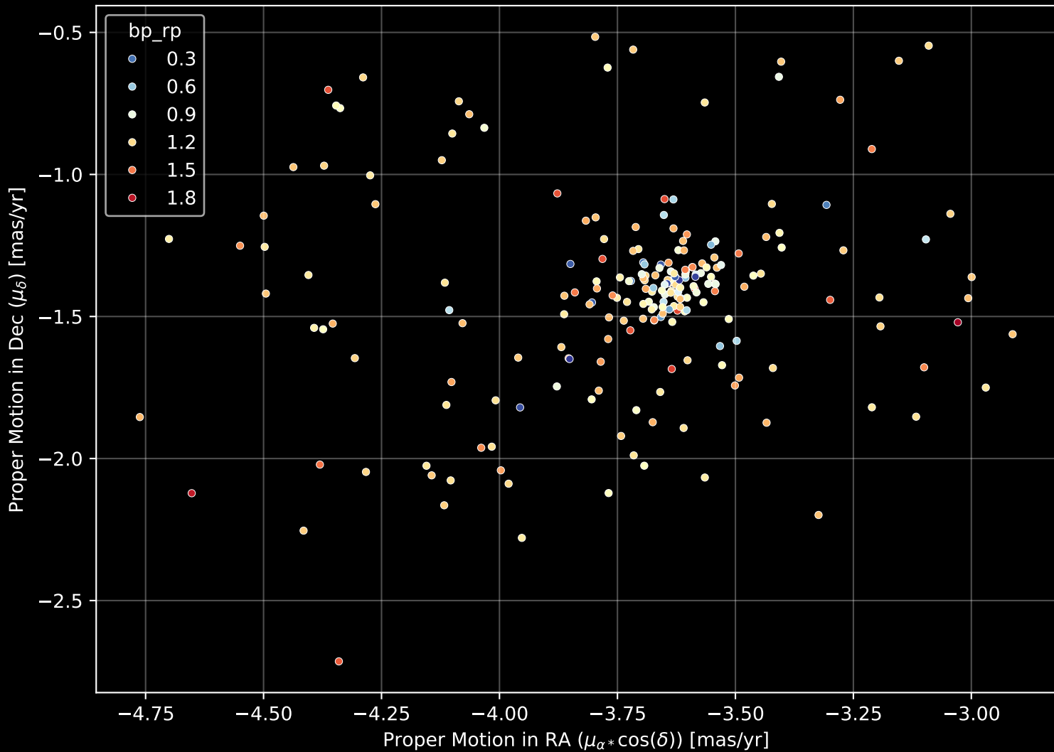
Gaia Cluster: [NGC_5138] Proper Motion Diagram (n= 218)
