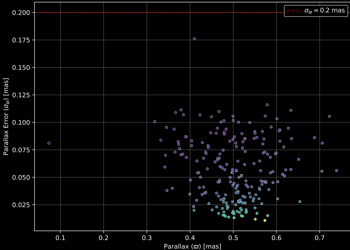
Gaia Cluster: [NGC_5138] Parallax Quality (n= 218)
