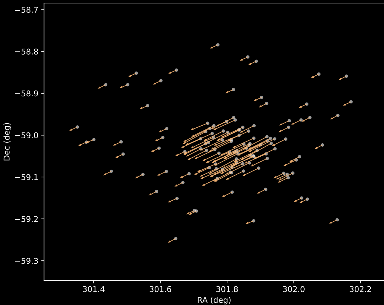
Gaia DR3 Cluster 3 Proper Motion Vectors (n=117)
