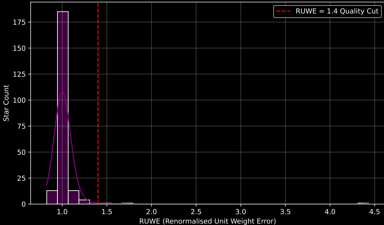
Gaia Cluster: [NGC_5138] RUWE Distribution (n= 218)
