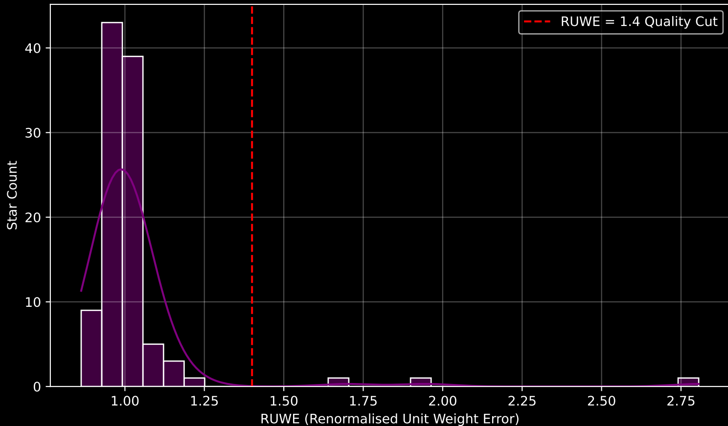
Gaia Cluster: [NGC_5269] RUWE Distribution (n= 103)
