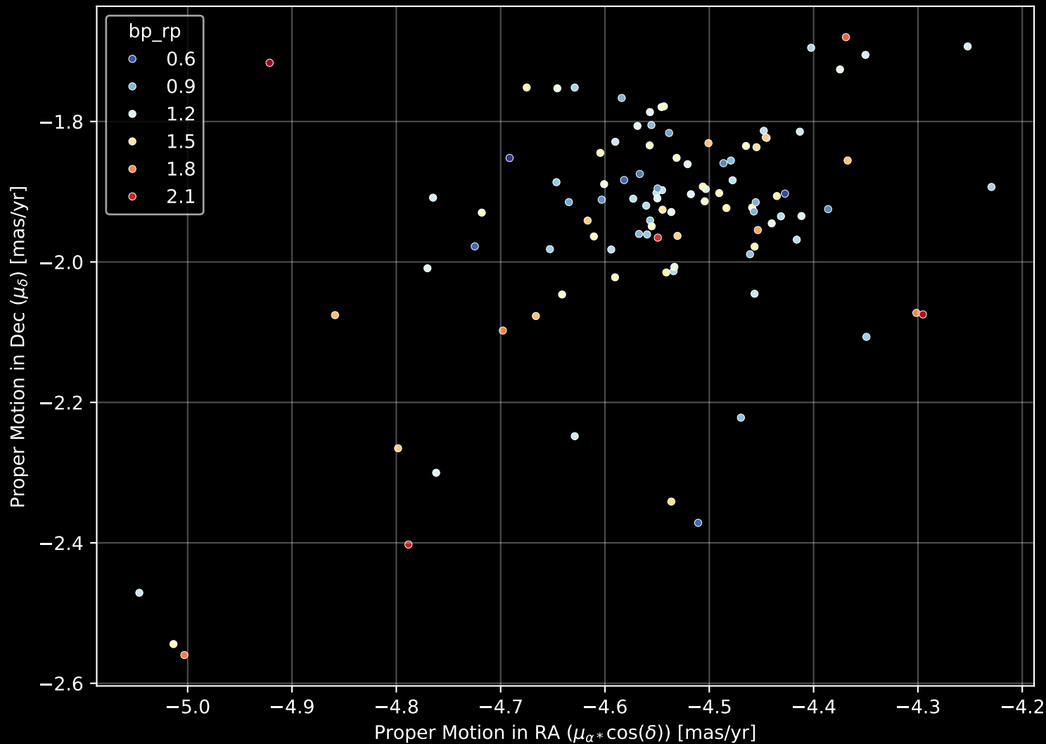
Gaia Cluster: [NGC_5269] Proper Motion Diagram (n= 103)
