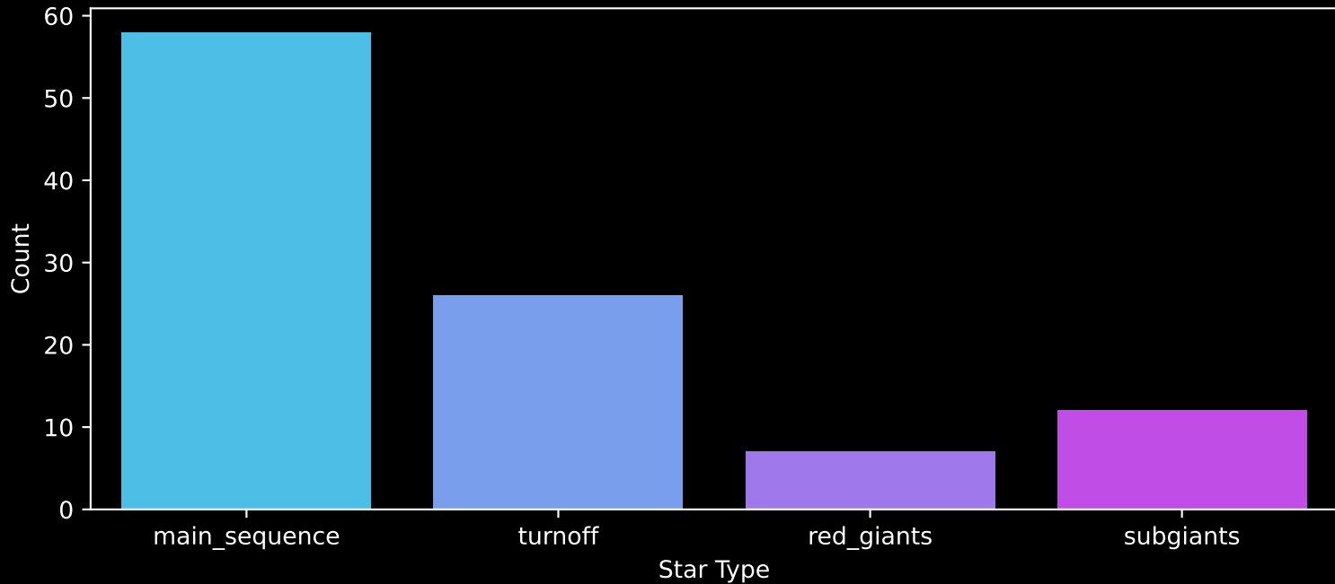
Gaia Cluster: [NGC_5269] Count plot of Star Type
