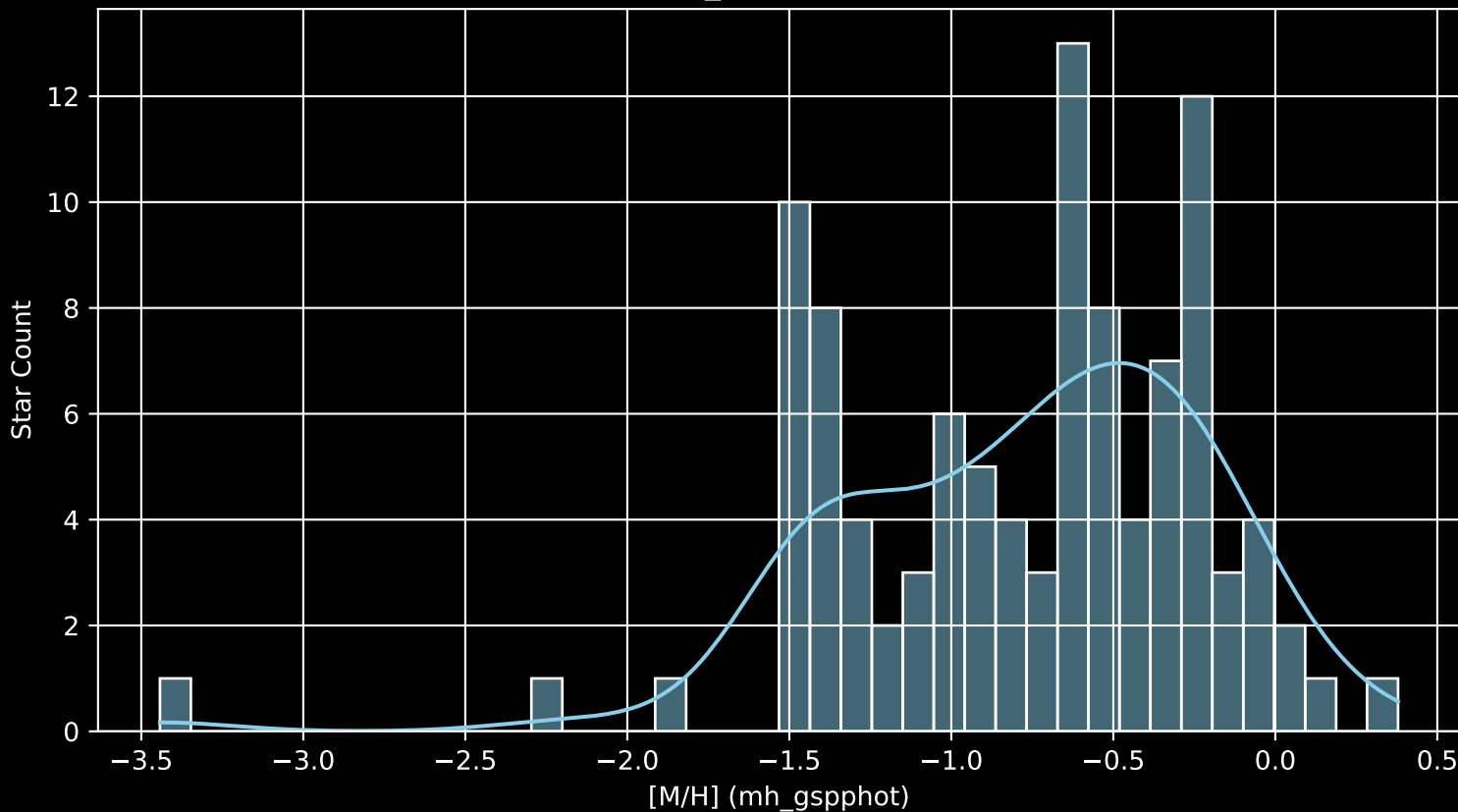
Gaia Cluster: [NGC_5269 [M/H] (mh_gspphot) (n= 103)
