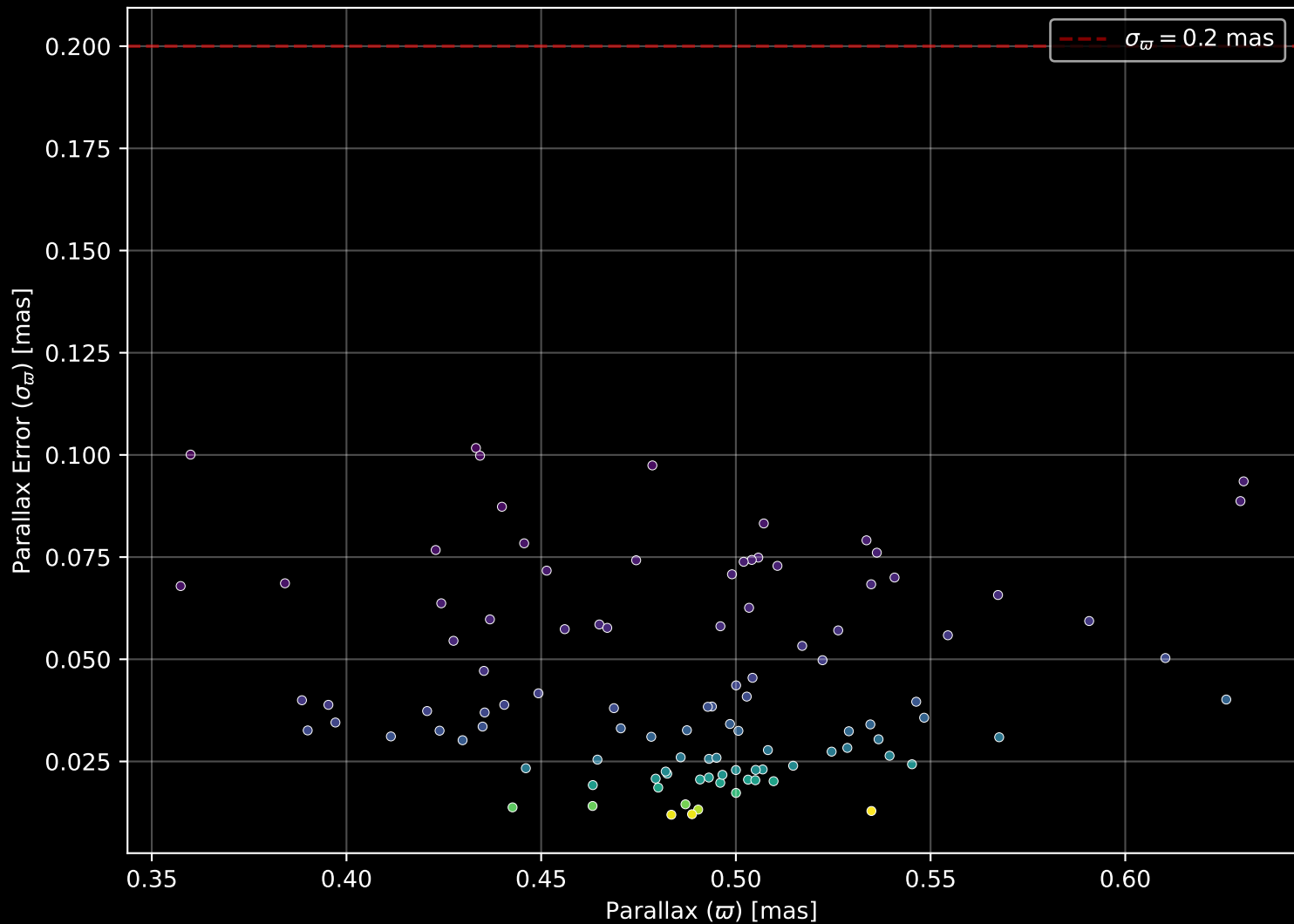
Gaia Cluster: [NGC_5269] Parallax Quality (n= 103)
