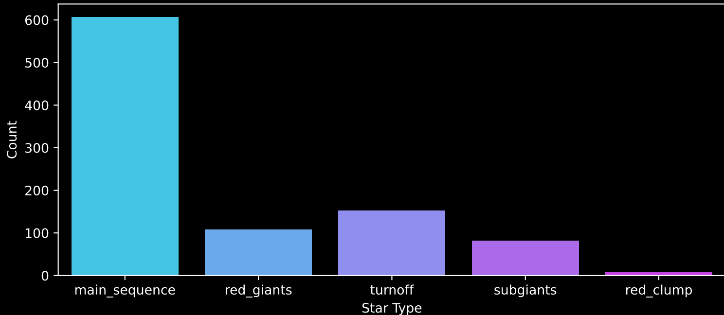
Gaia Cluster: [NGC_5381] Count plot of Star Type
