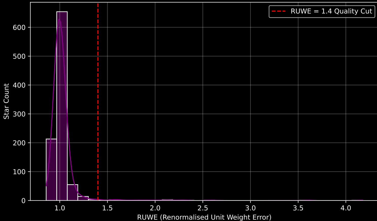
Gaia Cluster: [NGC_5381] RUWE Distribution (n= 957)
