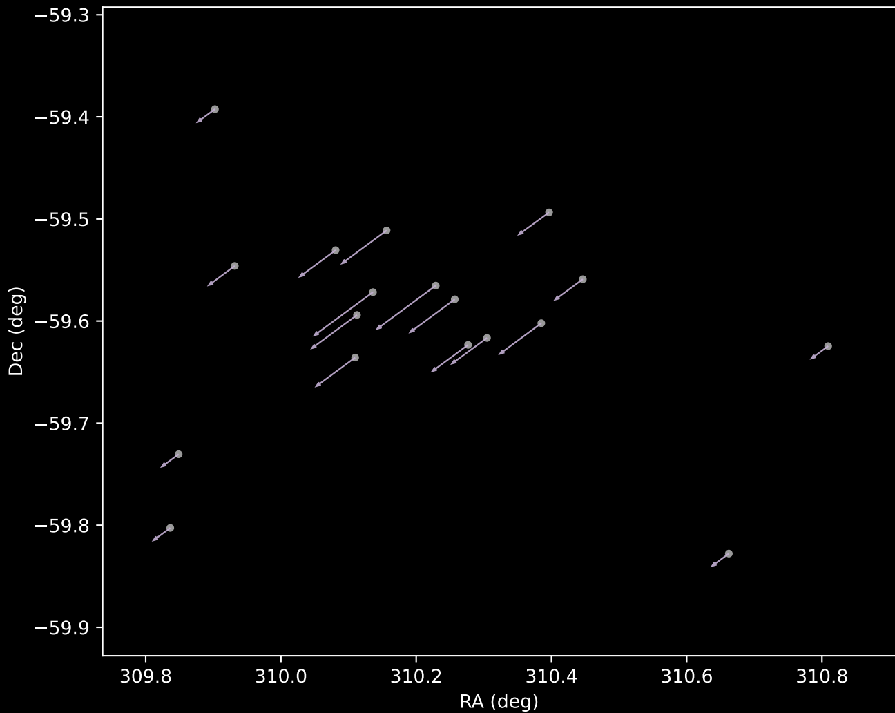
Gaia DR3 Cluster 49 Proper Motion Vectors (n=18)
