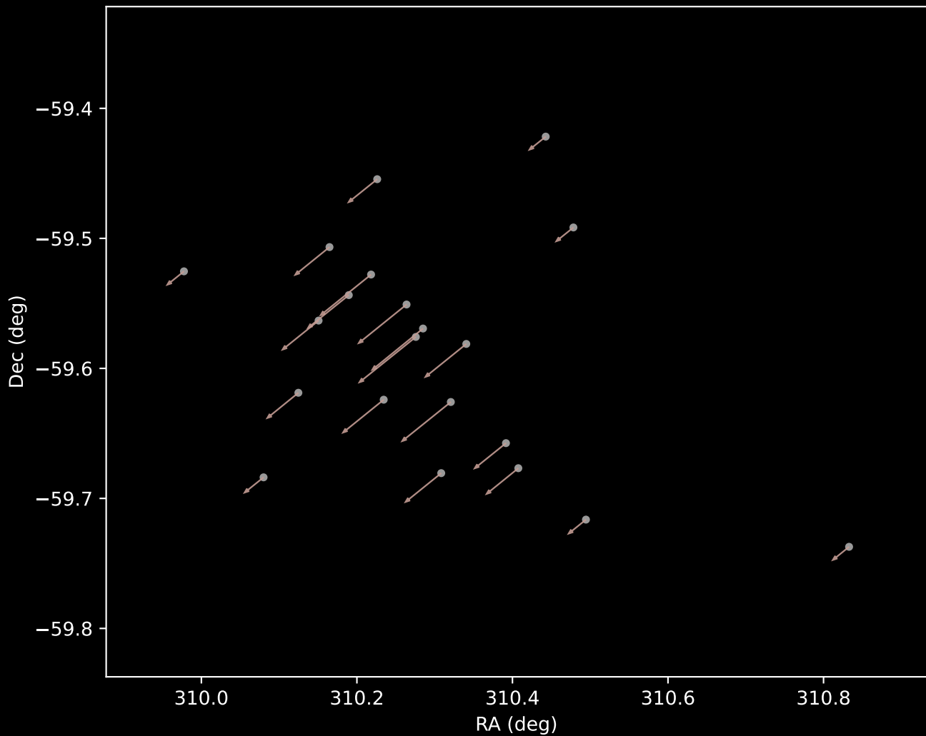
Gaia DR3 Cluster 51 Proper Motion Vectors (n=21)
