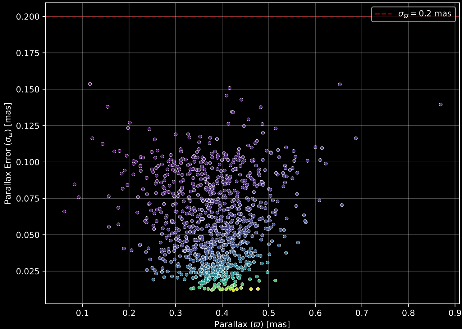
Gaia Cluster: [NGC_5381] Parallax Quality (n= 957)
