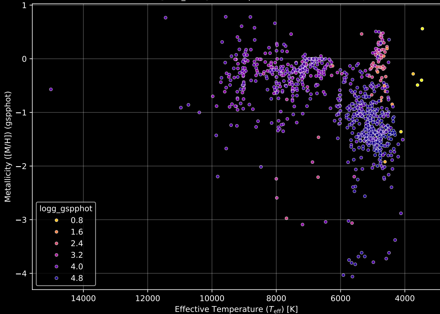
Gaia Cluster: [NGC_5381] Stellar Population Parameters (n= 957)
