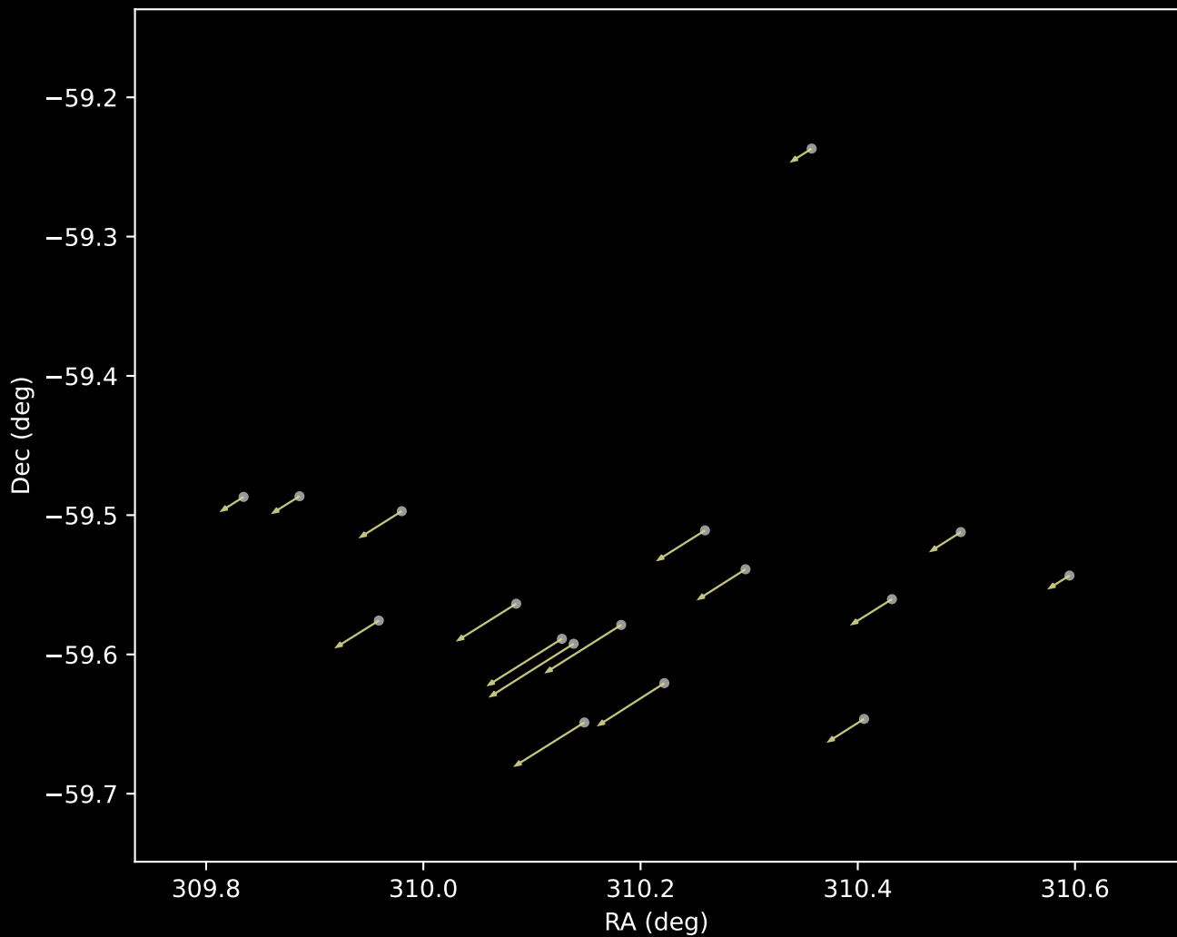
Gaia DR3 Cluster 37 Proper Motion Vectors (n=17)
