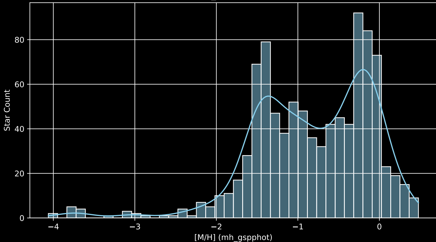
Gaia Cluster: [NGC_5381 [M/H] (mh_gspphot) (n= 948)
