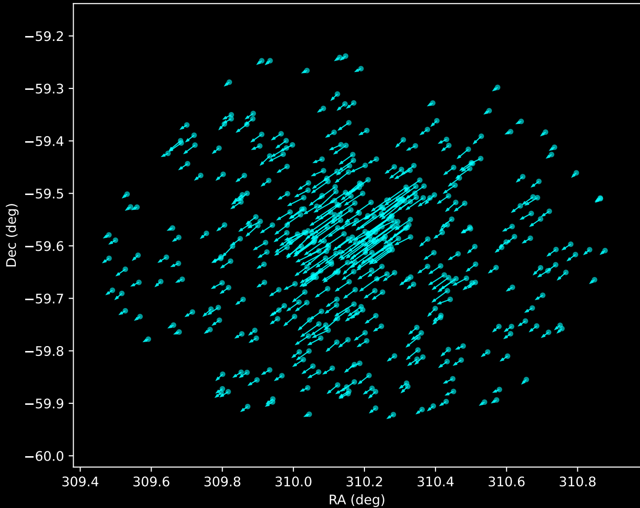
Gaia DR3 Noise Stream Proper Motion Vectors (n=423)
