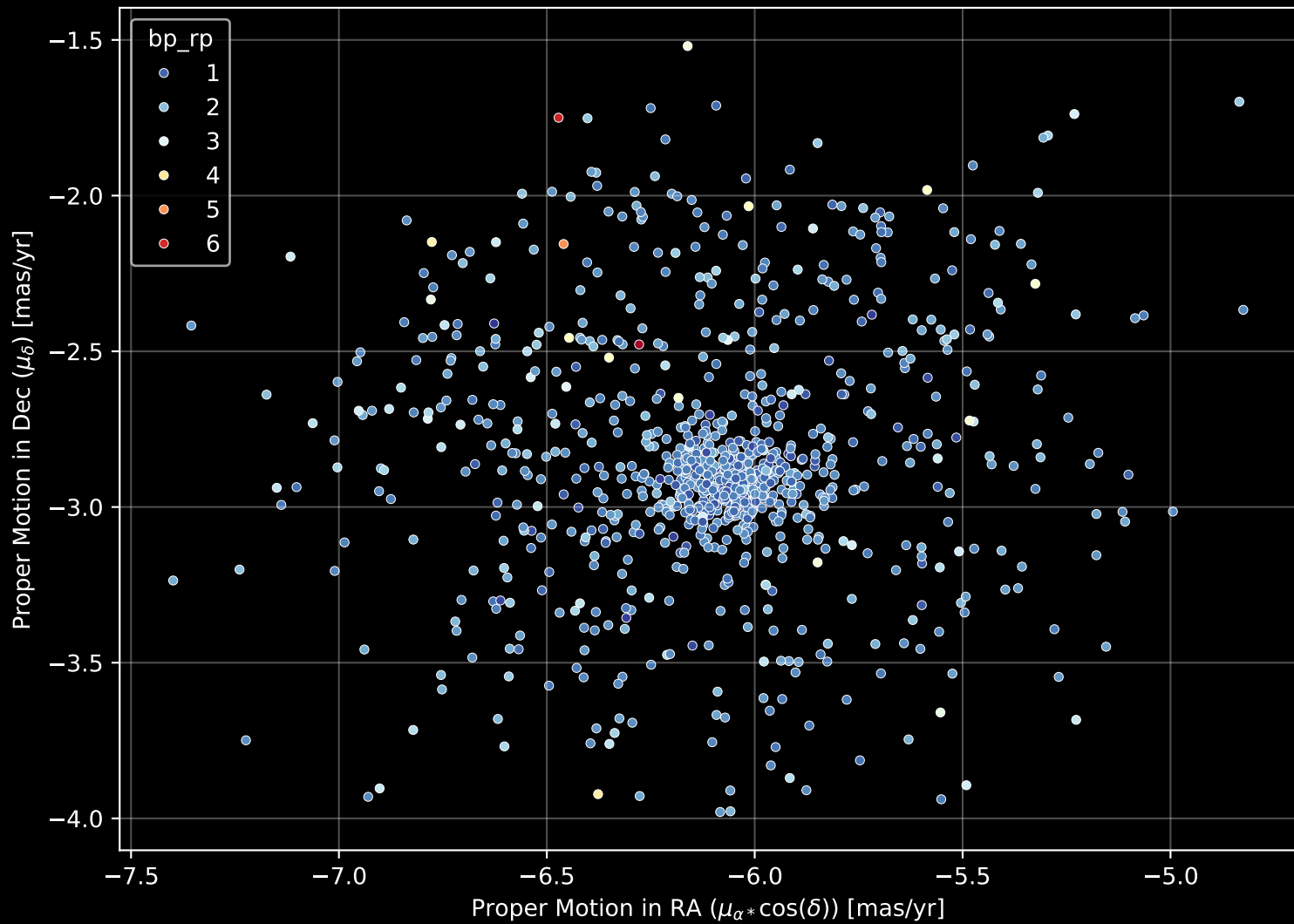
Gaia Cluster: [NGC_5381] Proper Motion Diagram (n= 957)
