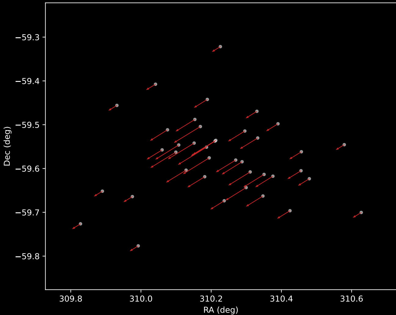
Gaia DR3 Cluster 46 Proper Motion Vectors (n=39)
