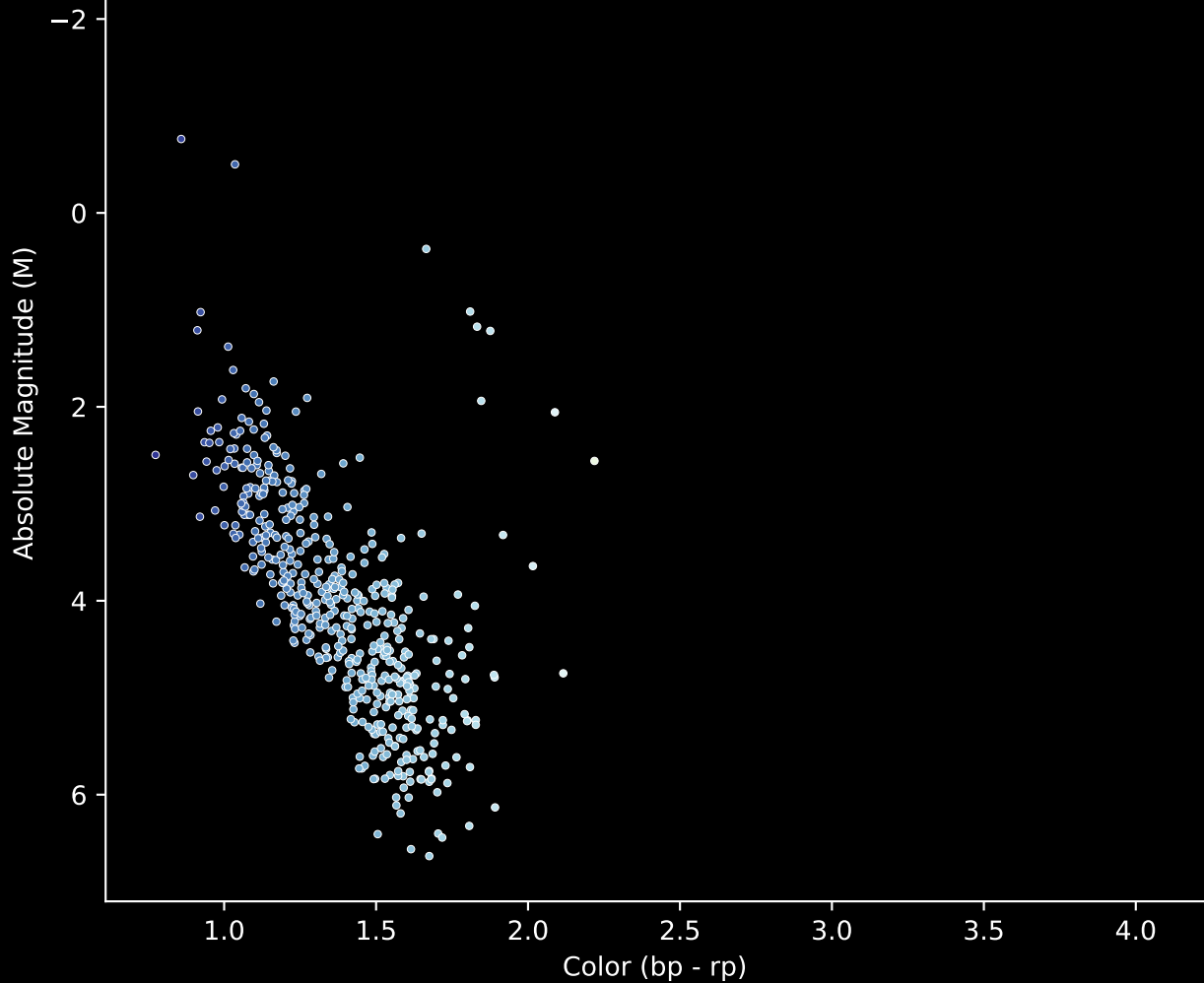
Gaia Cluster: [NGC_559] Stars (n= 492) Hertzsprung-Russel Diagram
