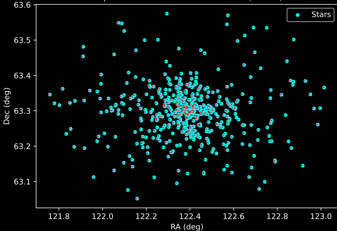
Gaia Cluster: [NGC_559] Proper Motion Vectors for Gaia Star Field (n= 492)
