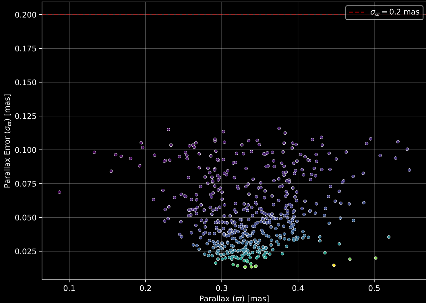
Gaia Cluster: [NGC_559] Parallax Quality (n= 492)
