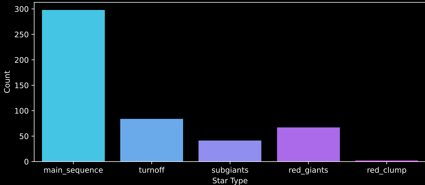
Gaia Cluster: [NGC_559] Count plot of Star Type
