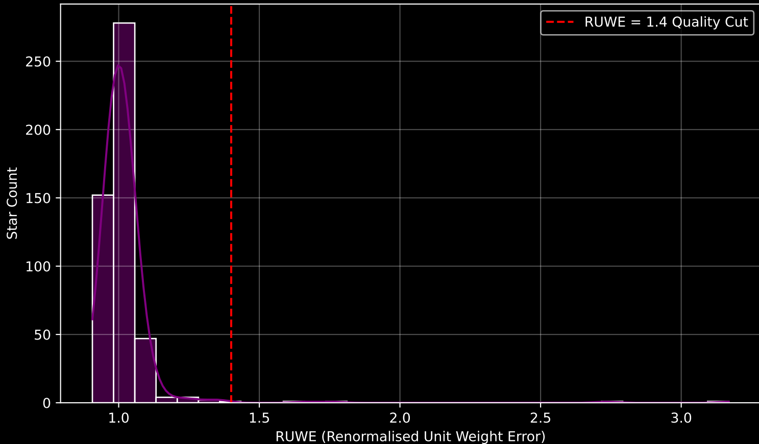
Gaia Cluster: [NGC_559] RUWE Distribution (n= 492)
