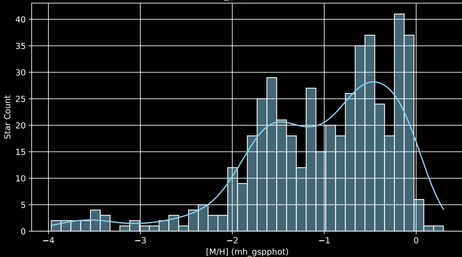
Gaia Cluster: [NGC_559 [M/H] (mh_gspphot) (n= 491)
