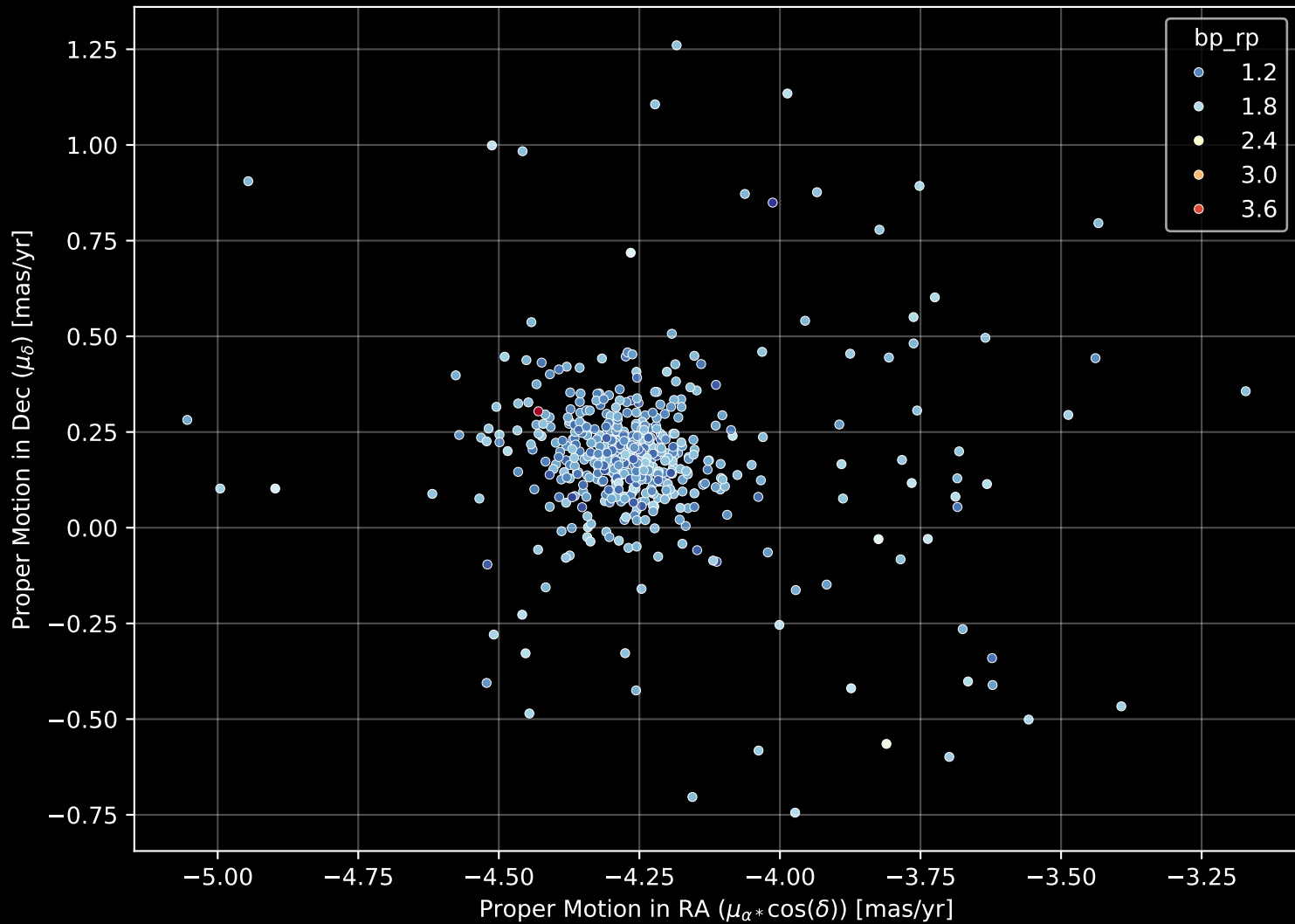
Gaia Cluster: [NGC_559] Proper Motion Diagram (n= 492)
