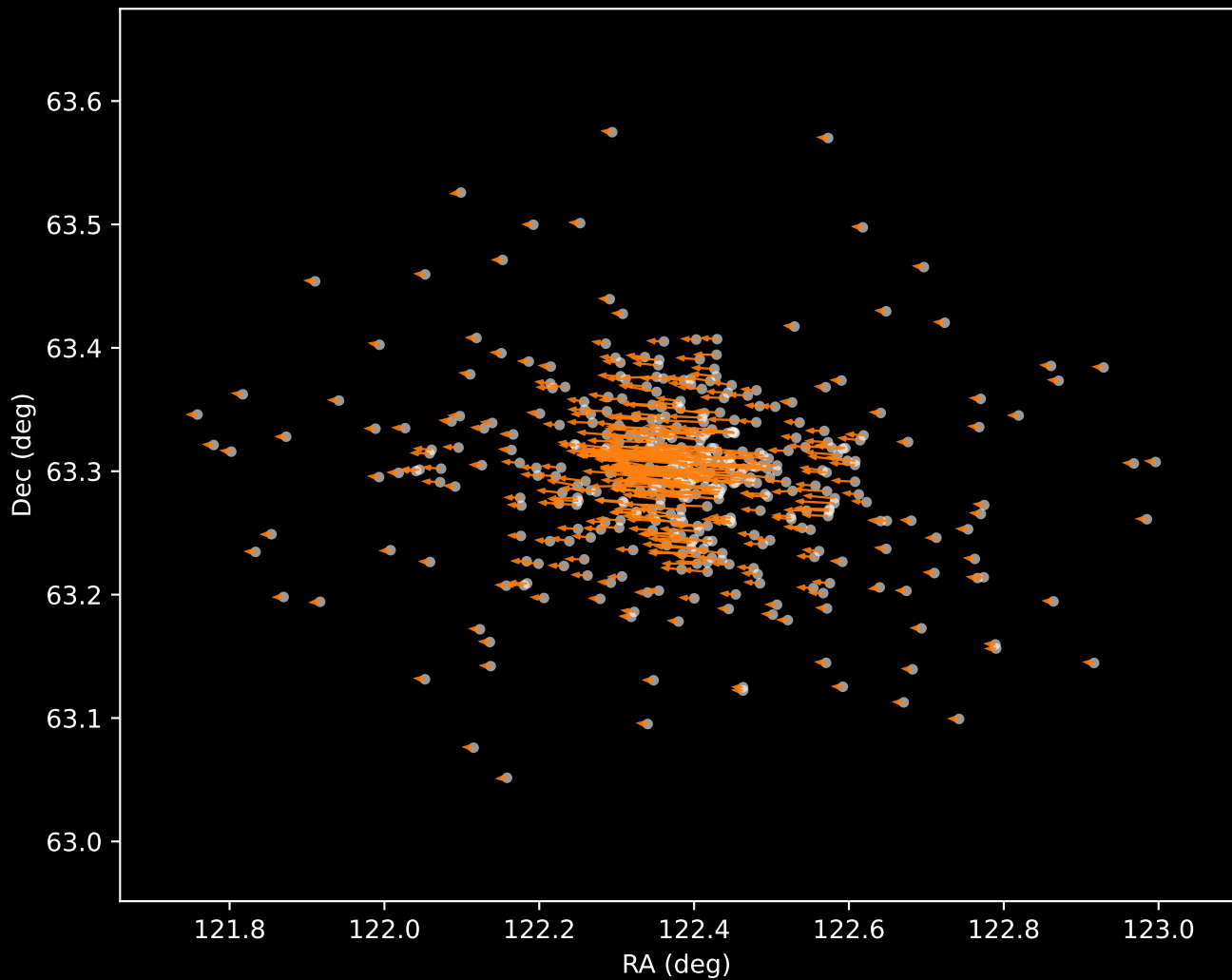
Gaia DR3 Cluster 2 Proper Motion Vectors (n=436)
