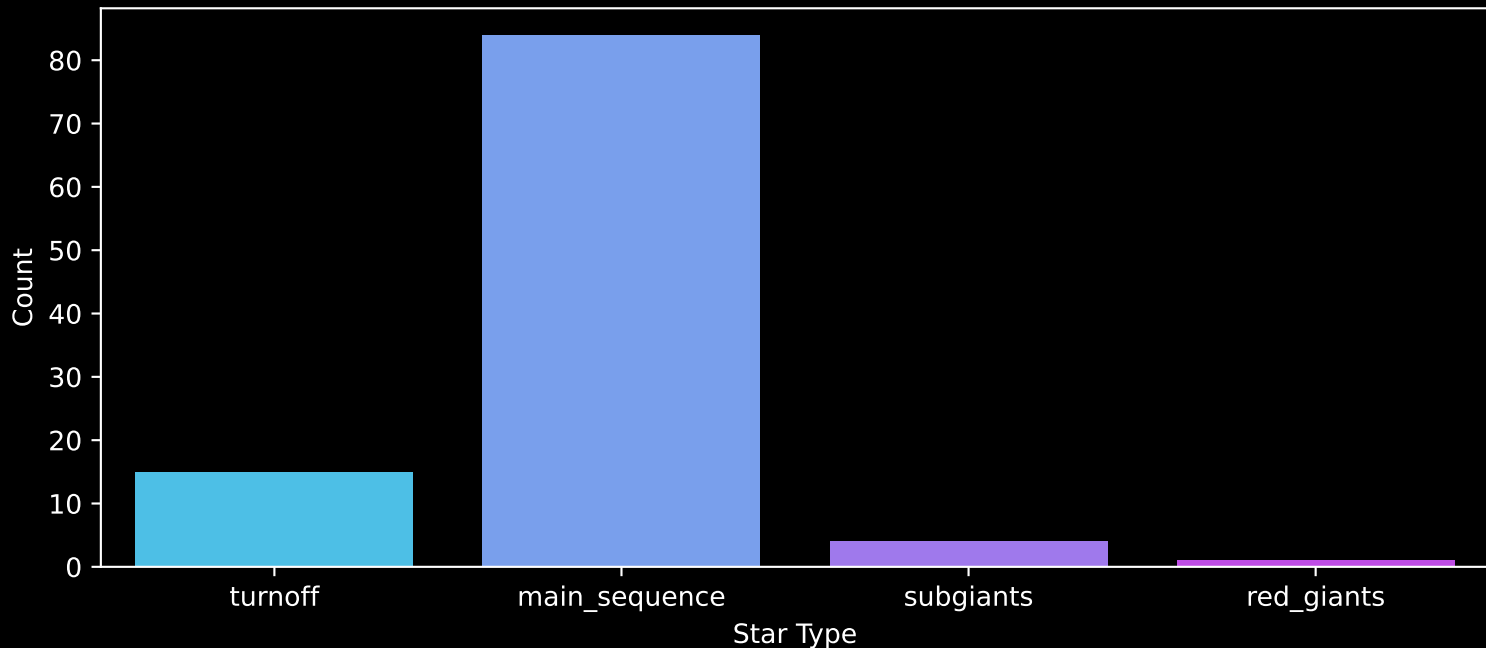
Gaia Cluster: [NGC_5749] Count plot of Star Type
