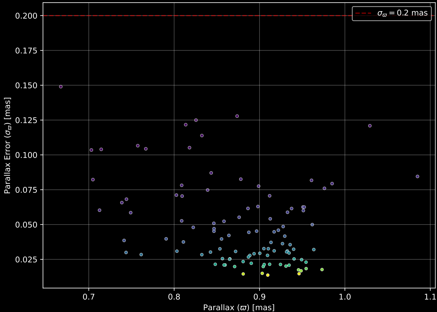
Gaia Cluster: [NGC_5749] Parallax Quality (n= 104)
