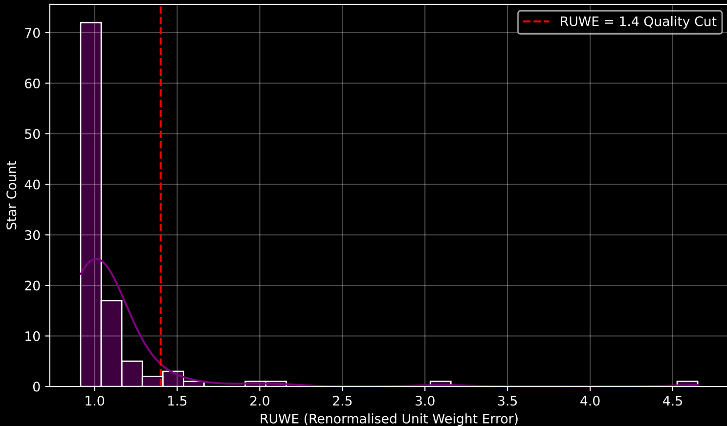
Gaia Cluster: [NGC_5749] RUWE Distribution (n= 104)
