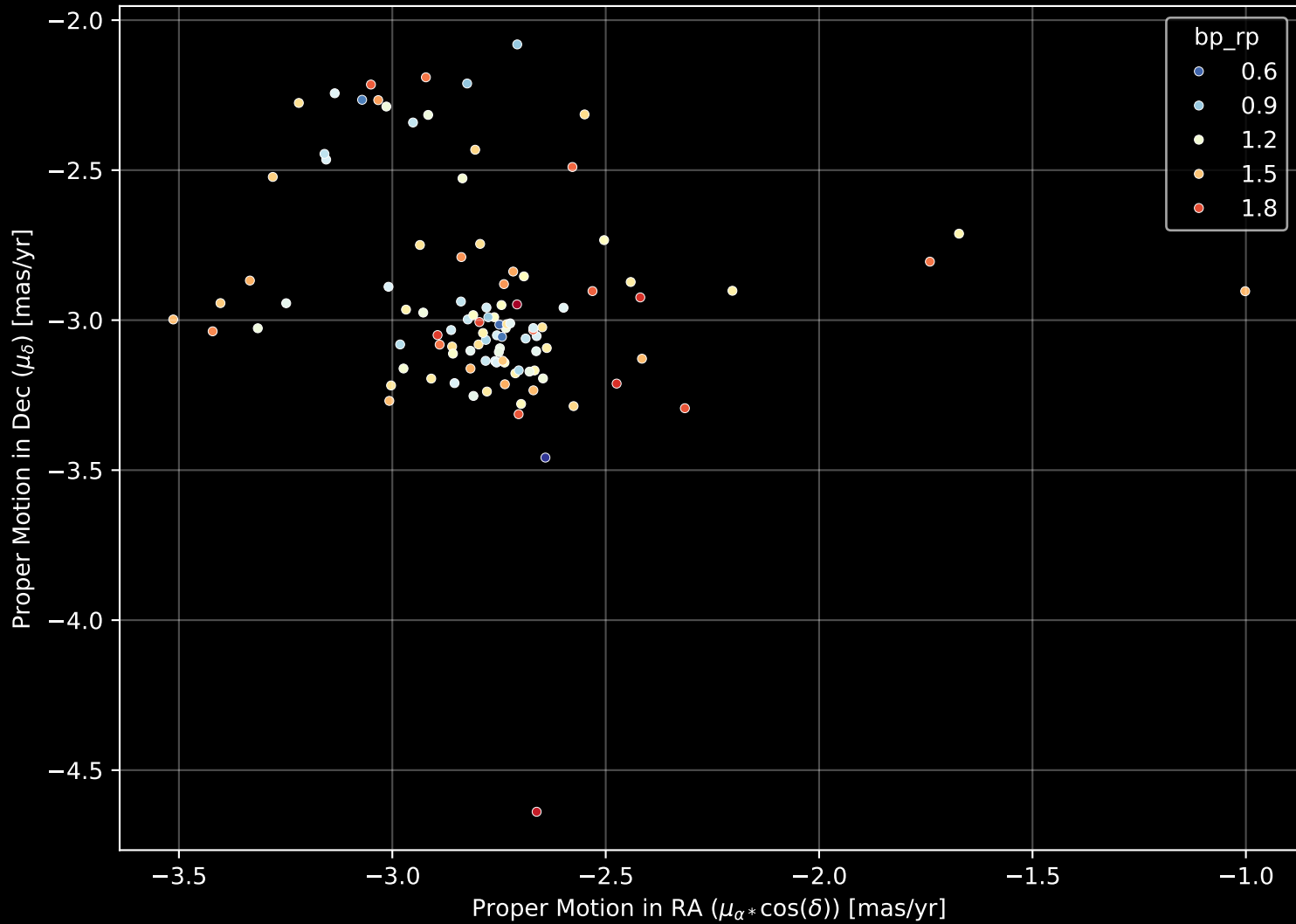
Gaia Cluster: [NGC_5749] Proper Motion Diagram (n= 104)
