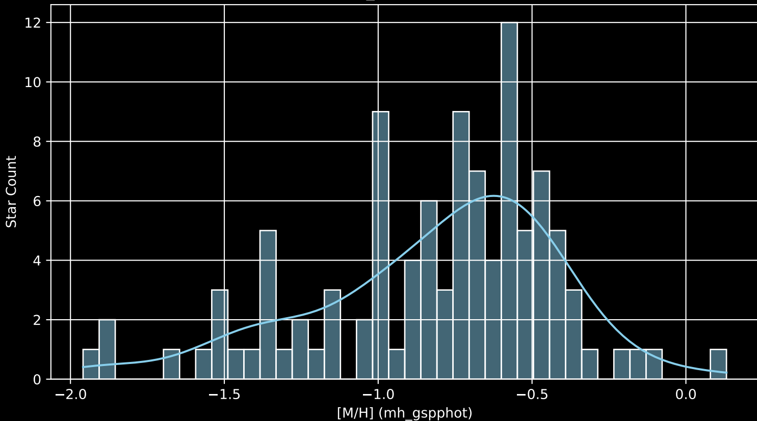
Gaia Cluster: [NGC_5749 [M/H] (mh_gspphot) (n= 104)
