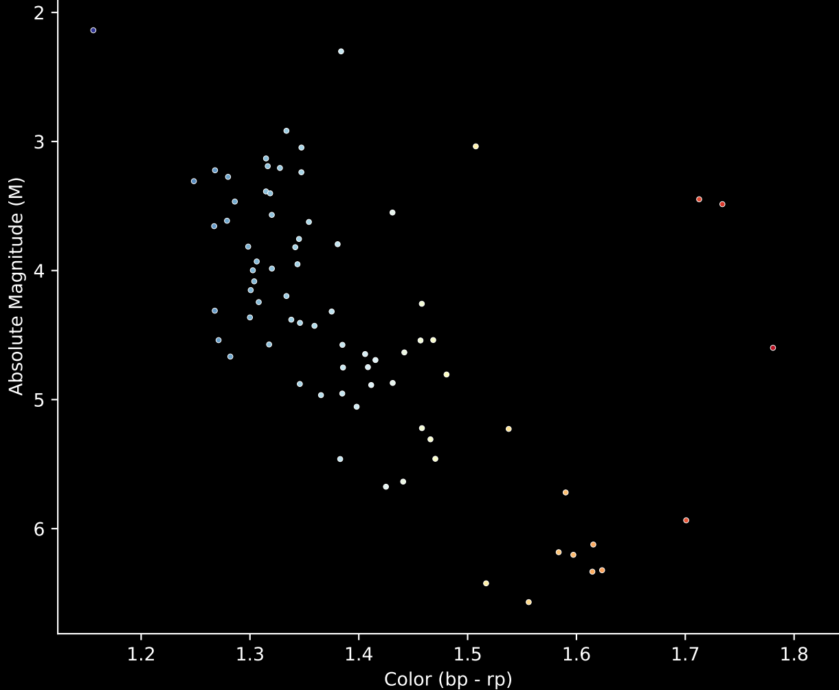
Gaia Cluster: [NGC_5764] Stars (n= 77) Hertzsprung-Russel Diagram
