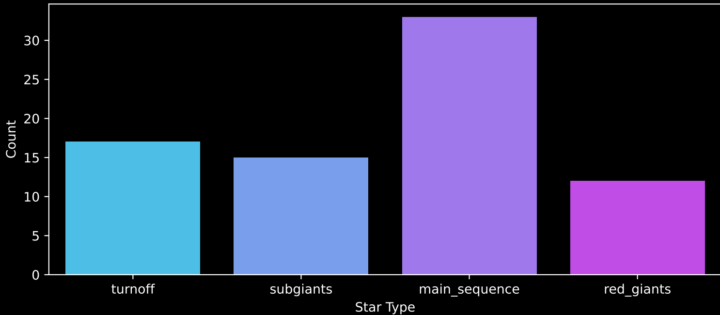
Gaia Cluster: [NGC_5764] Count plot of Star Type
