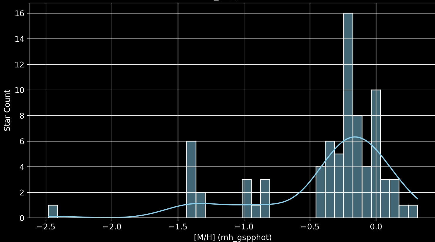
Gaia Cluster: [NGC_5764 [M/H] (mh_gspphot) (n= 77)
