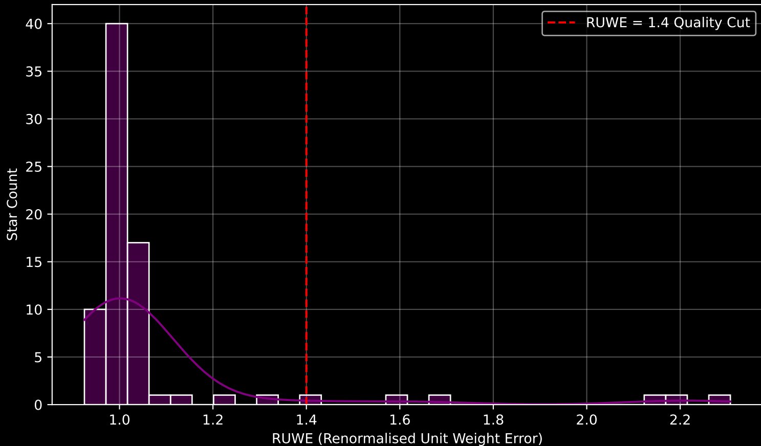
Gaia Cluster: [NGC_5764] RUWE Distribution (n= 77)
