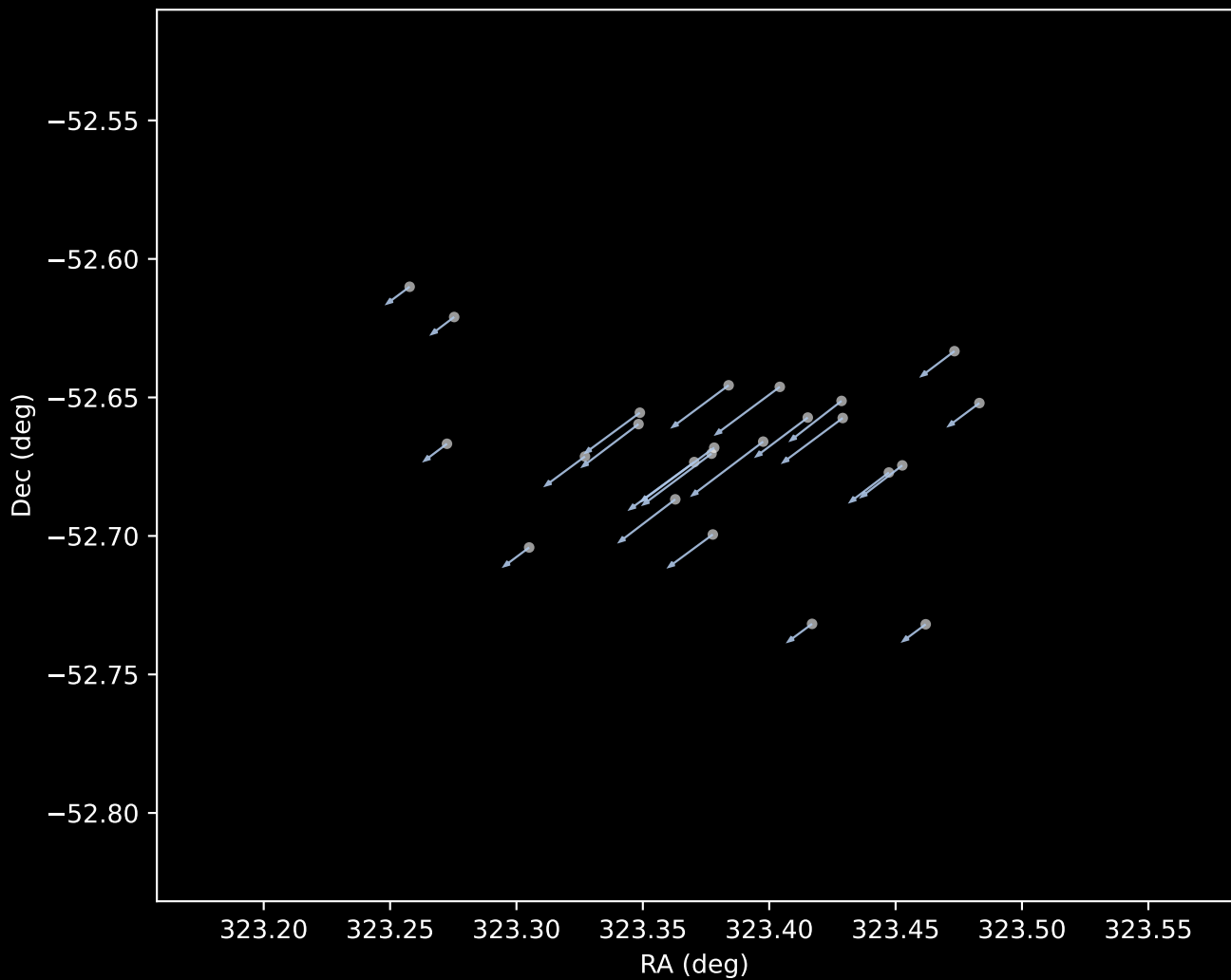
Gaia DR3 Cluster 1 Proper Motion Vectors (n=24)
