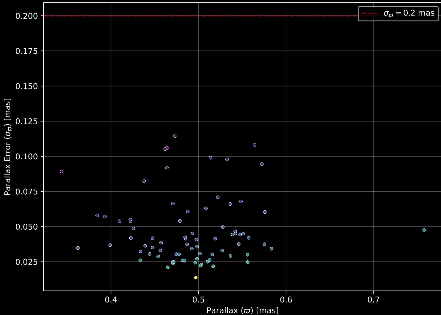
Gaia Cluster: [NGC_5764] Parallax Quality (n= 77)
