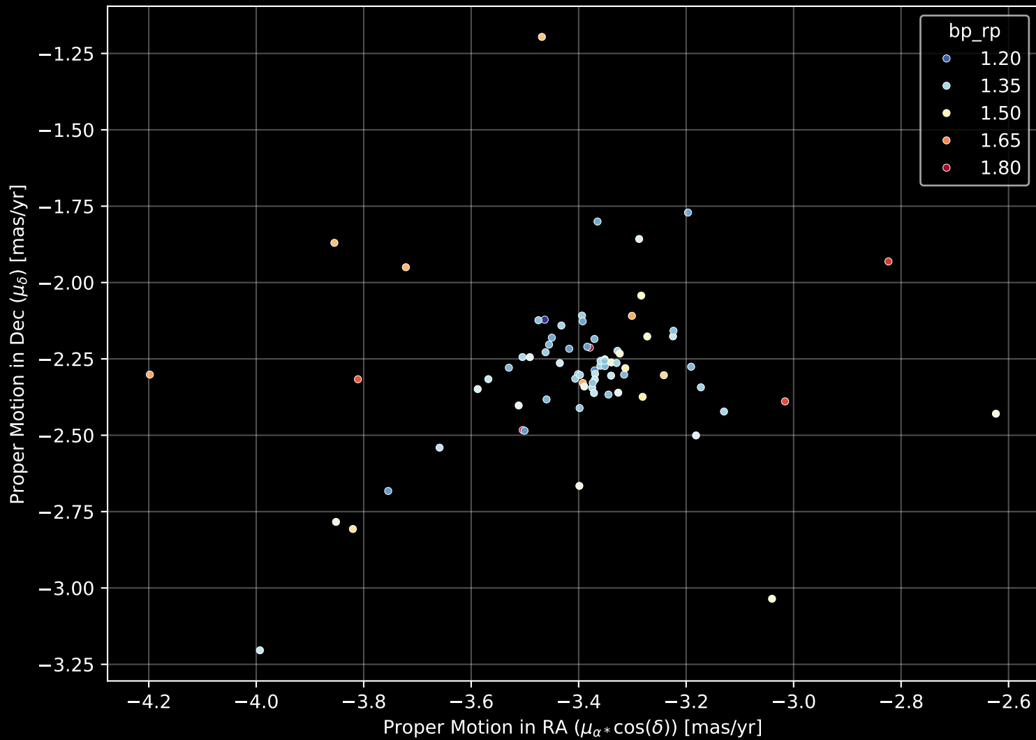
Gaia Cluster: [NGC_5764] Proper Motion Diagram (n= 77)
