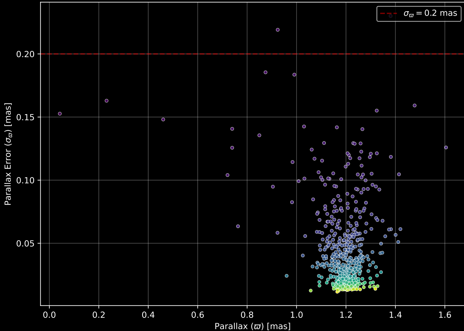
Gaia Cluster: [NGC_5822] Parallax Quality (n= 609)
