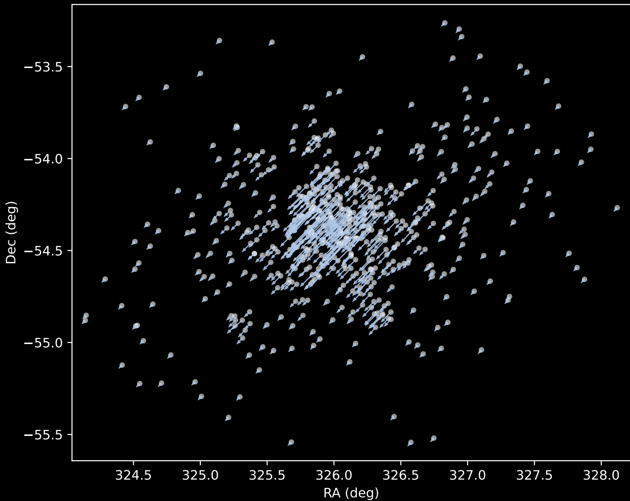
Gaia DR3 Cluster 1 Proper Motion Vectors (n=556)
