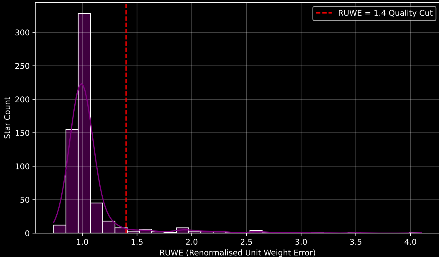
Gaia Cluster: [NGC_5822] RUWE Distribution (n= 604)
