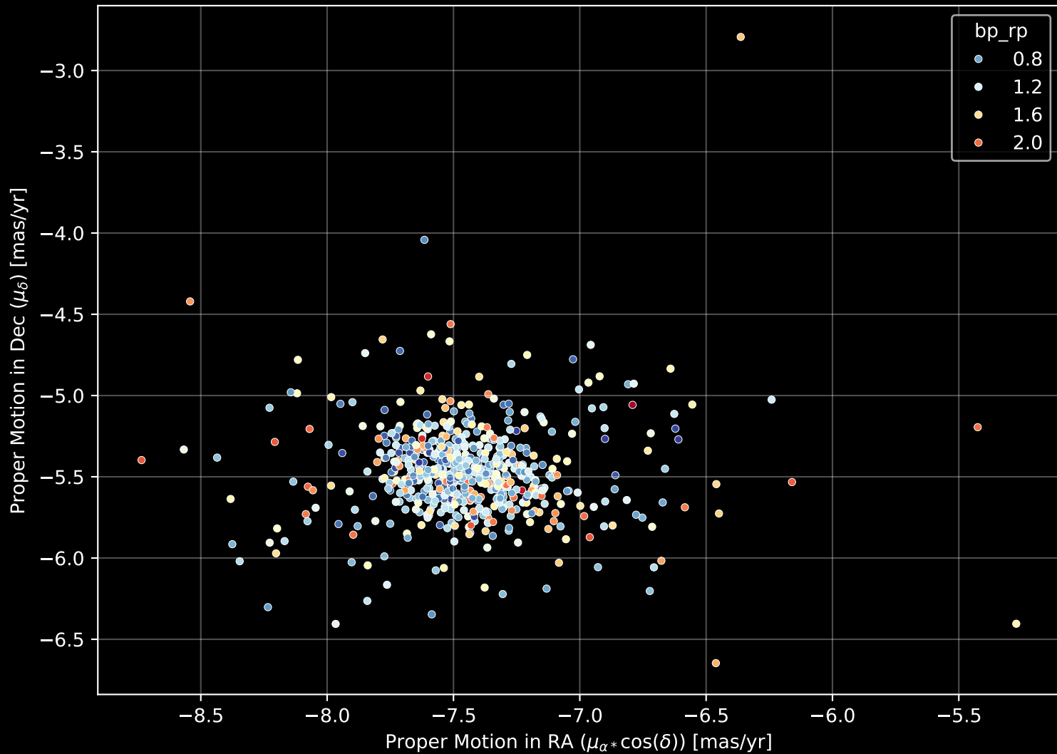
Gaia Cluster: [NGC_5822] Proper Motion Diagram (n= 609)
