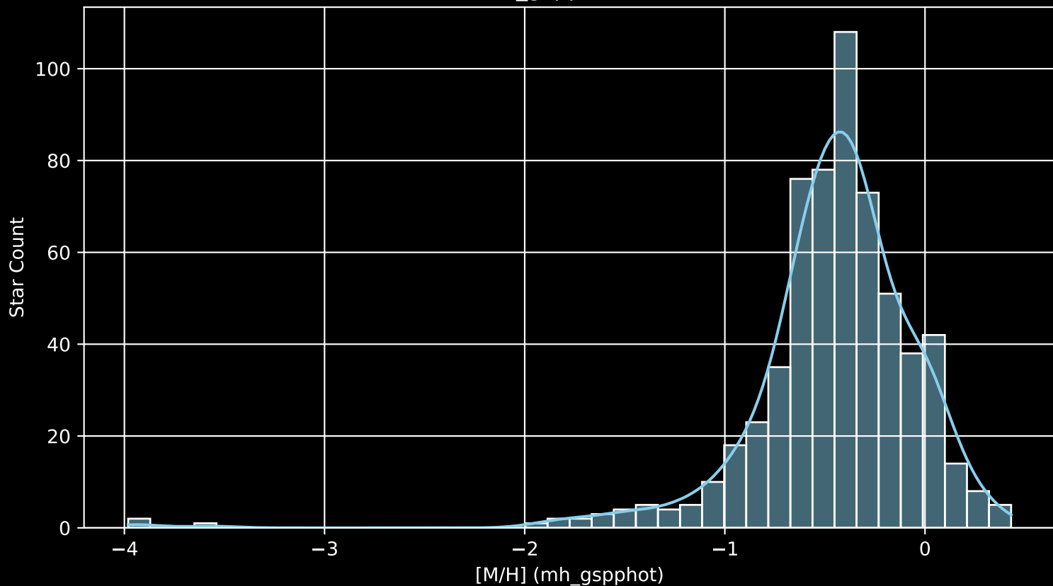
Gaia Cluster: [NGC_5822 [M/H] (mh_gspphot) (n= 608)
