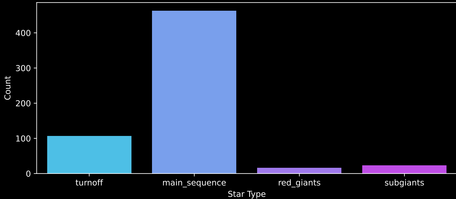
Gaia Cluster: [NGC_5822] Count plot of Star Type
