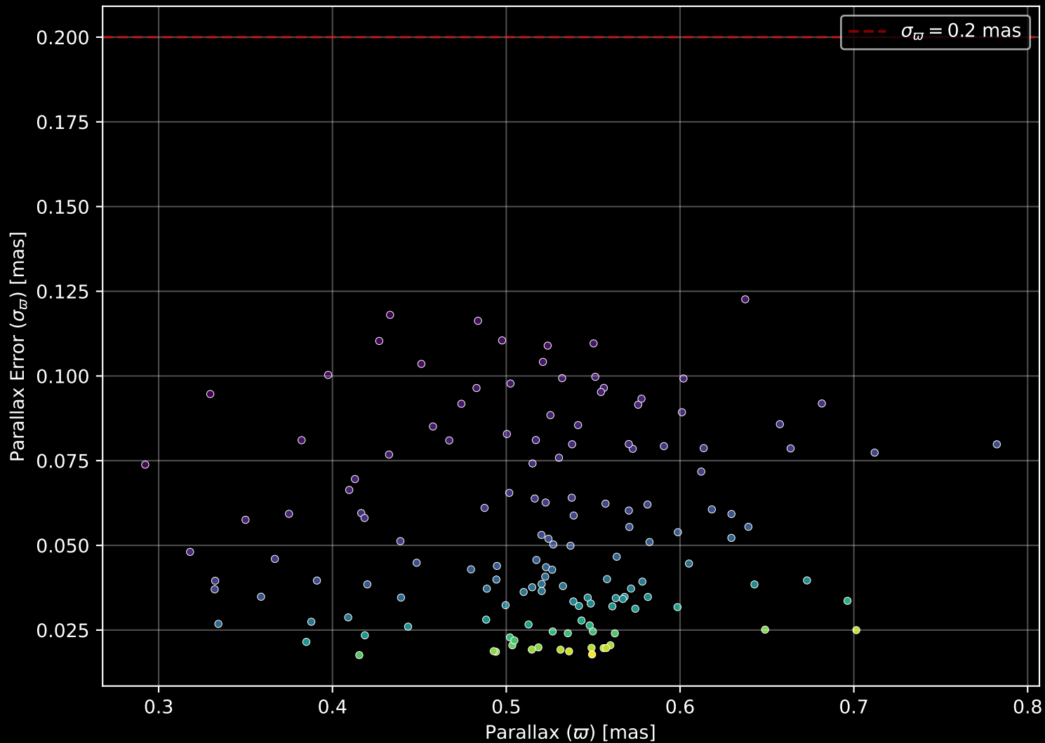
Gaia Cluster: [NGC_6031] Parallax Quality (n= 144)
