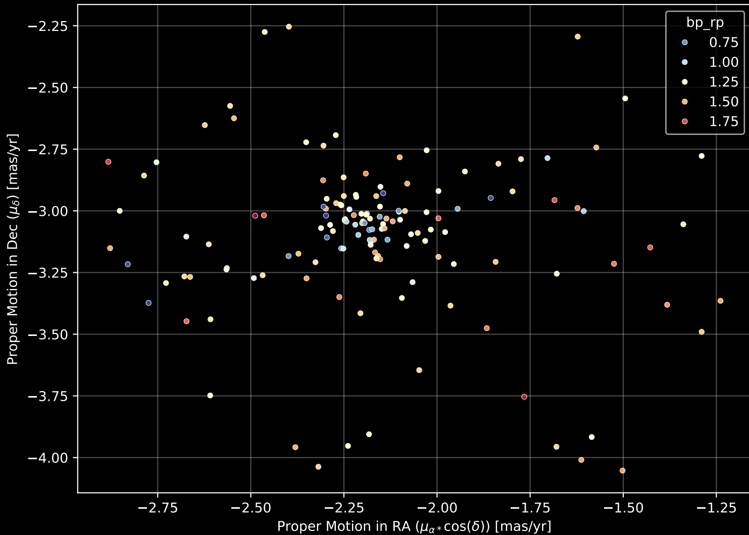
Gaia Cluster: [NGC_6031] Proper Motion Diagram (n= 144)
