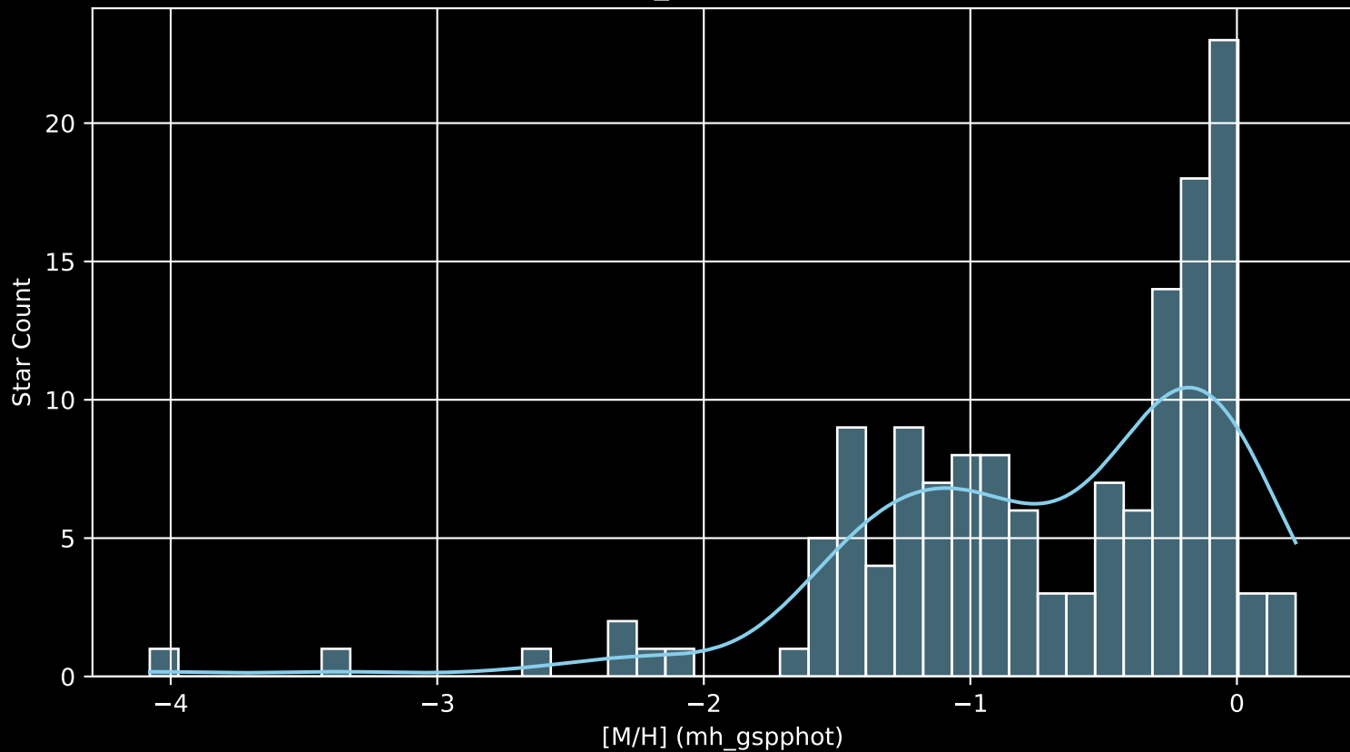
Gaia Cluster: [NGC_6031 [M/H] (mh_gspphot) (n= 144)
