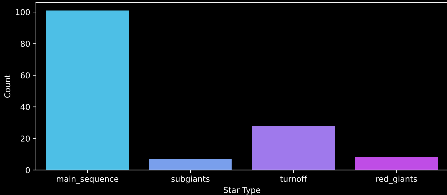
Gaia Cluster: [NGC_6031] Count plot of Star Type
