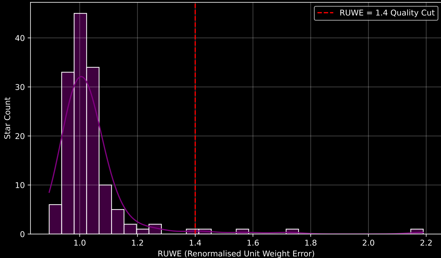
Gaia Cluster: [NGC_6031] RUWE Distribution (n= 143)
