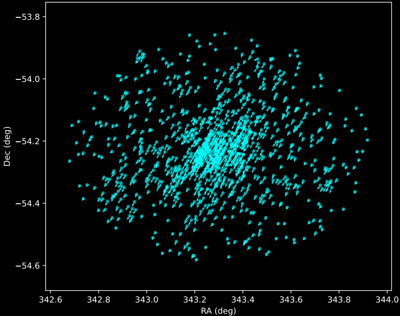
Gaia DR3 Noise Stream Proper Motion Vectors (n=901)
