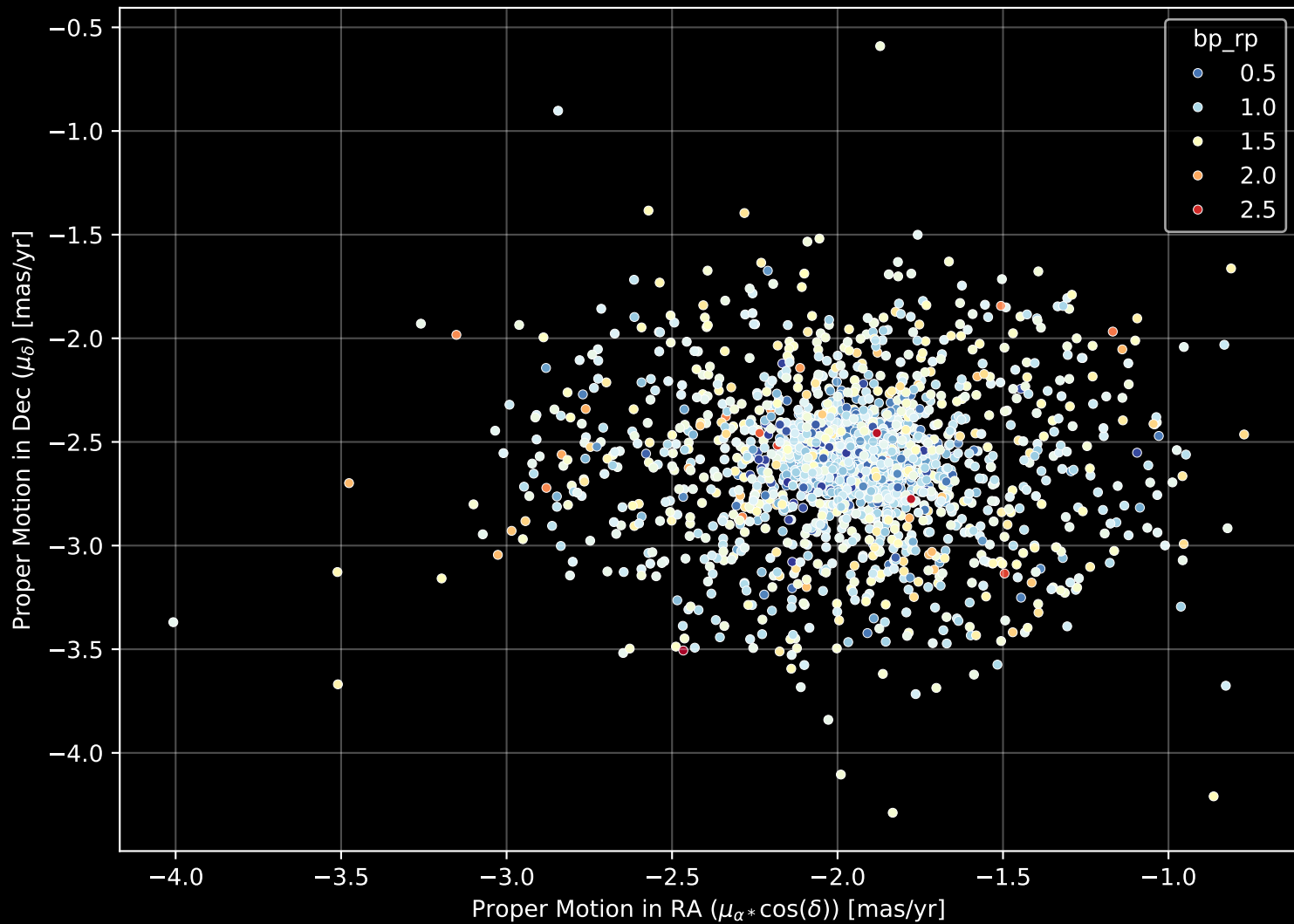
Gaia Cluster: [NGC_6067] Proper Motion Diagram (n= 2021)
