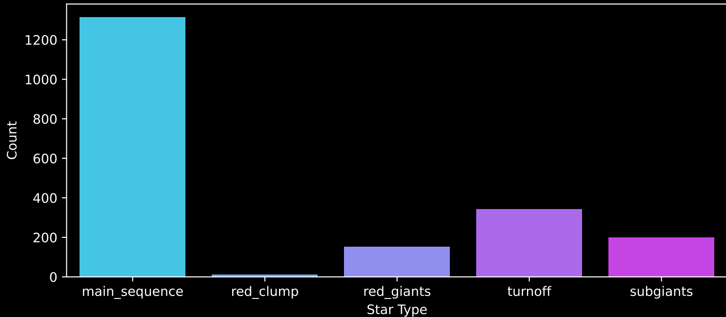
Gaia Cluster: [NGC_6067] Count plot of Star Type
