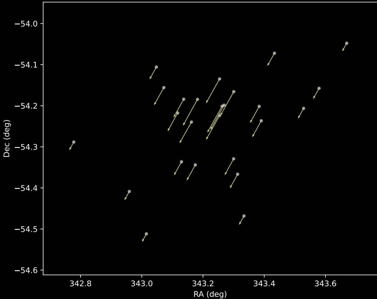
Gaia DR3 Cluster 117 Proper Motion Vectors (n=25)
