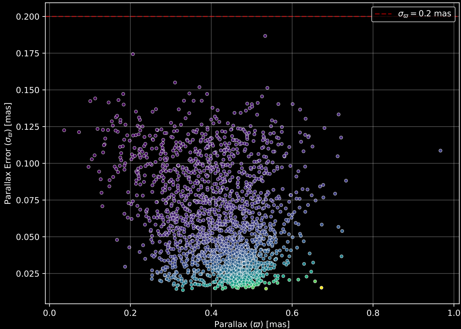
Gaia Cluster: [NGC_6067] Parallax Quality (n= 2021)
