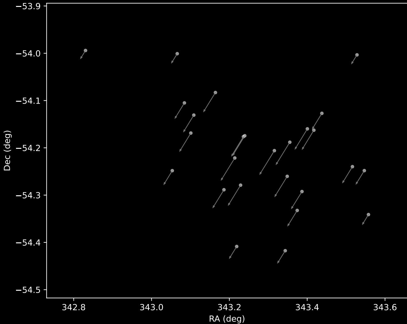
Gaia DR3 Cluster 114 Proper Motion Vectors (n=26)
