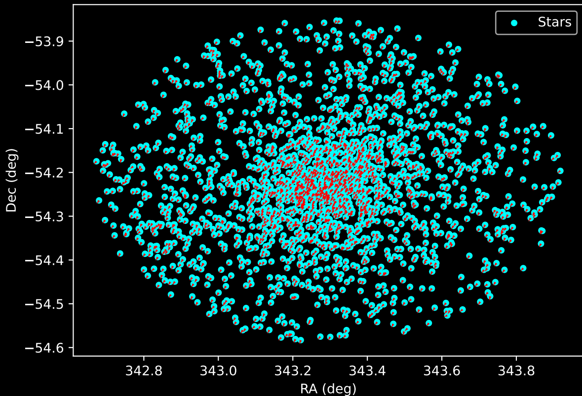
Gaia Cluster: [NGC_6067] Proper Motion Vectors for Gaia Star Field (n= 2021)
