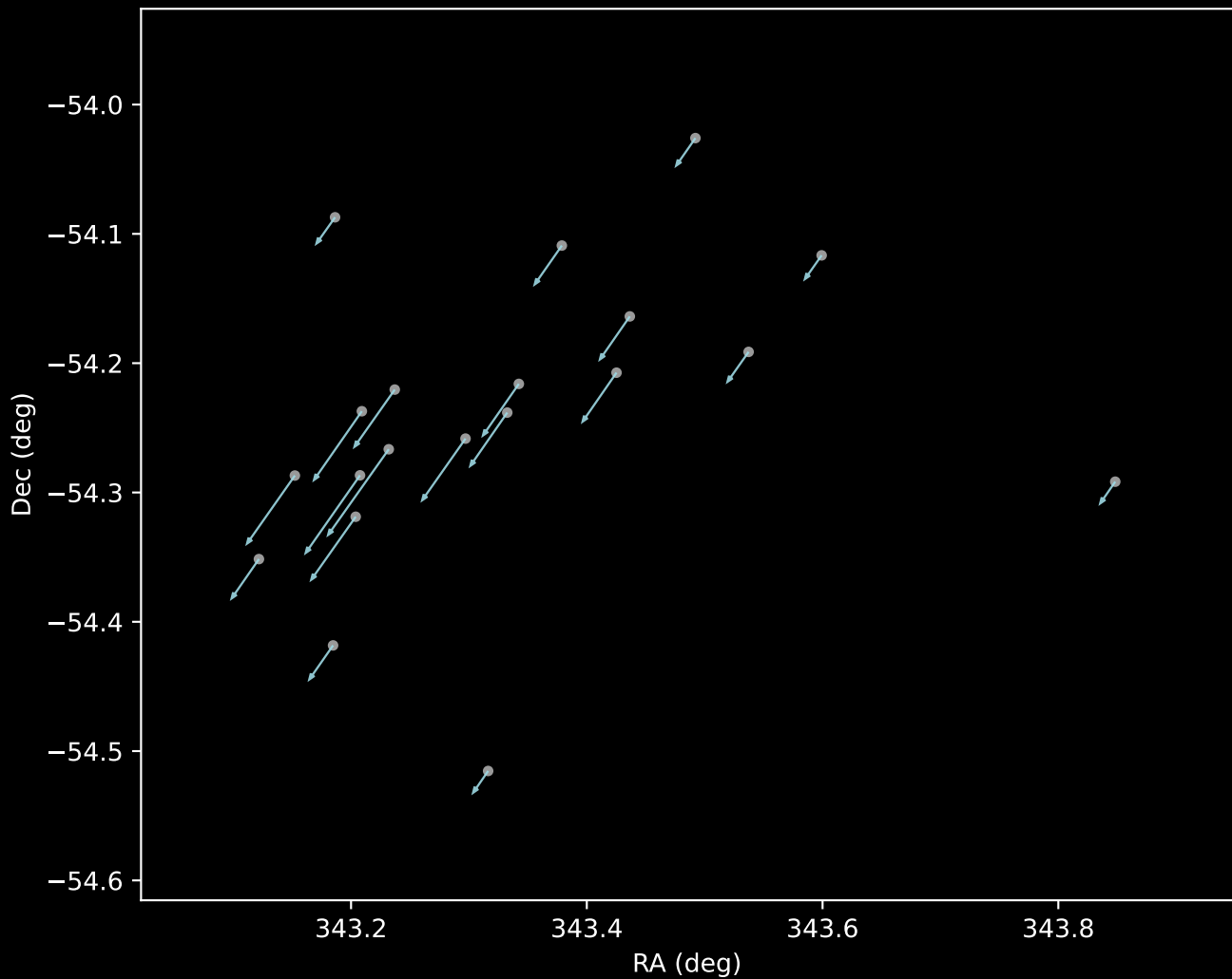
Gaia DR3 Cluster 99 Proper Motion Vectors (n=20)
