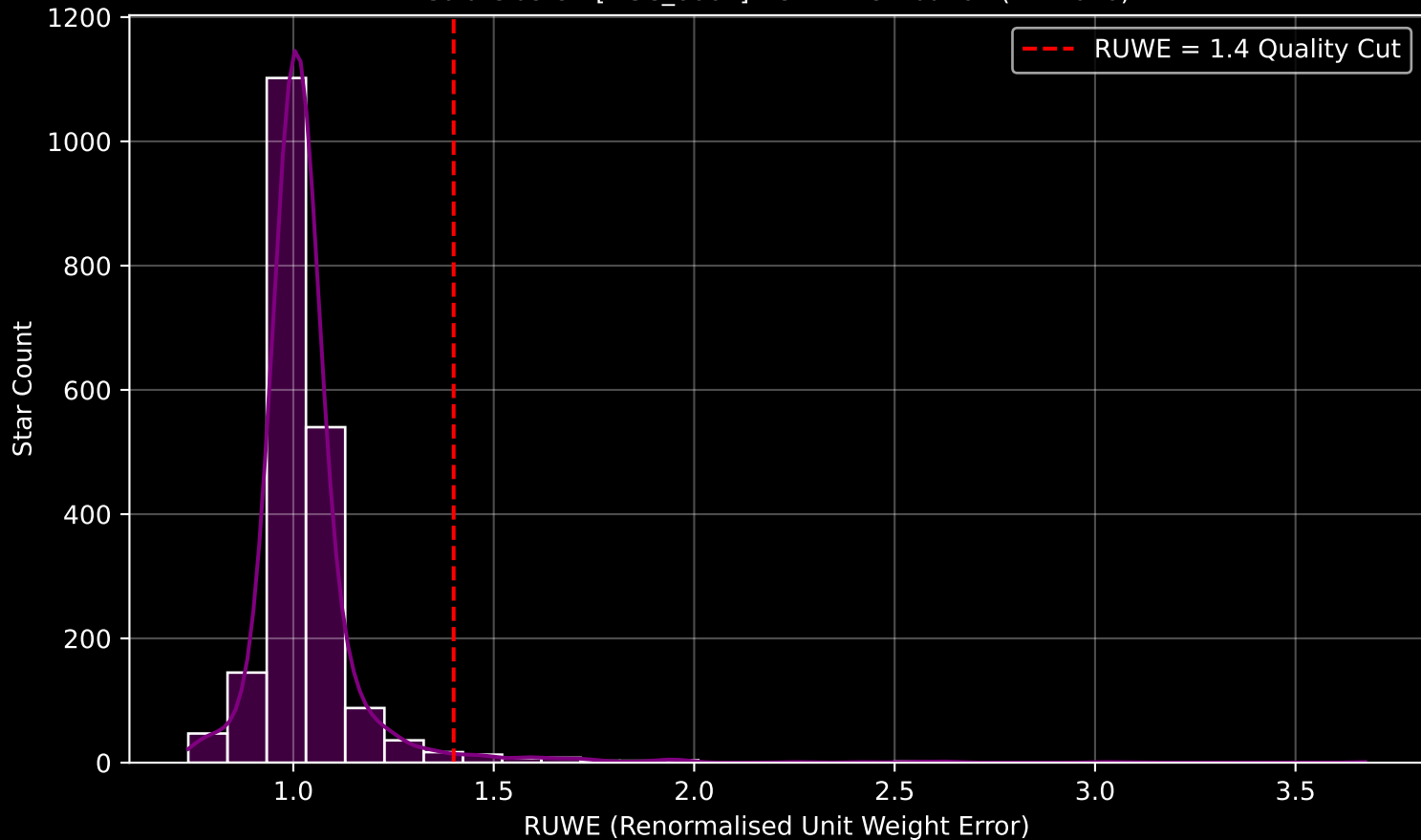
Gaia Cluster: [NGC_6067] RUWE Distribution (n= 2020)
