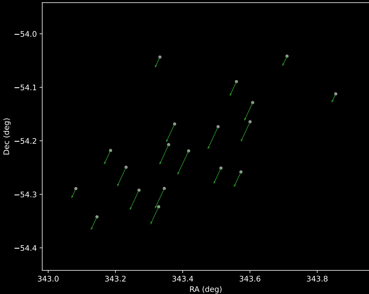
Gaia DR3 Cluster 104 Proper Motion Vectors (n=19)
