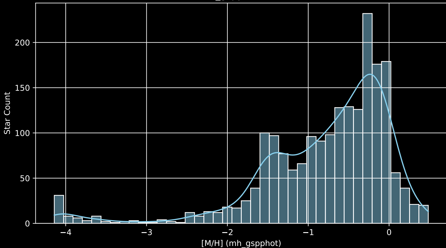
Gaia Cluster: [NGC_6067 [M/H] (mh_gspphot) (n= 2007)
