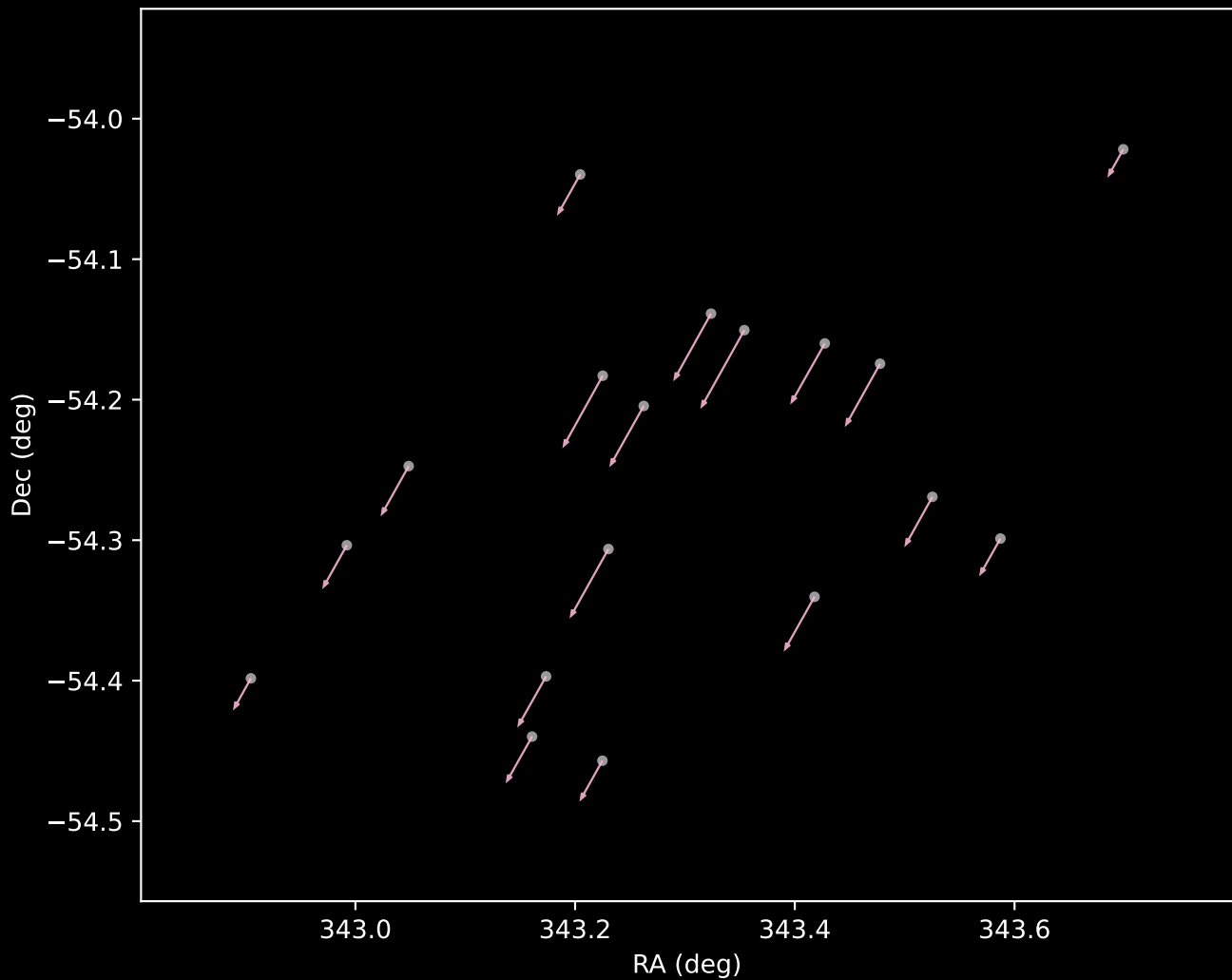
Gaia DR3 Cluster 113 Proper Motion Vectors (n=18)
