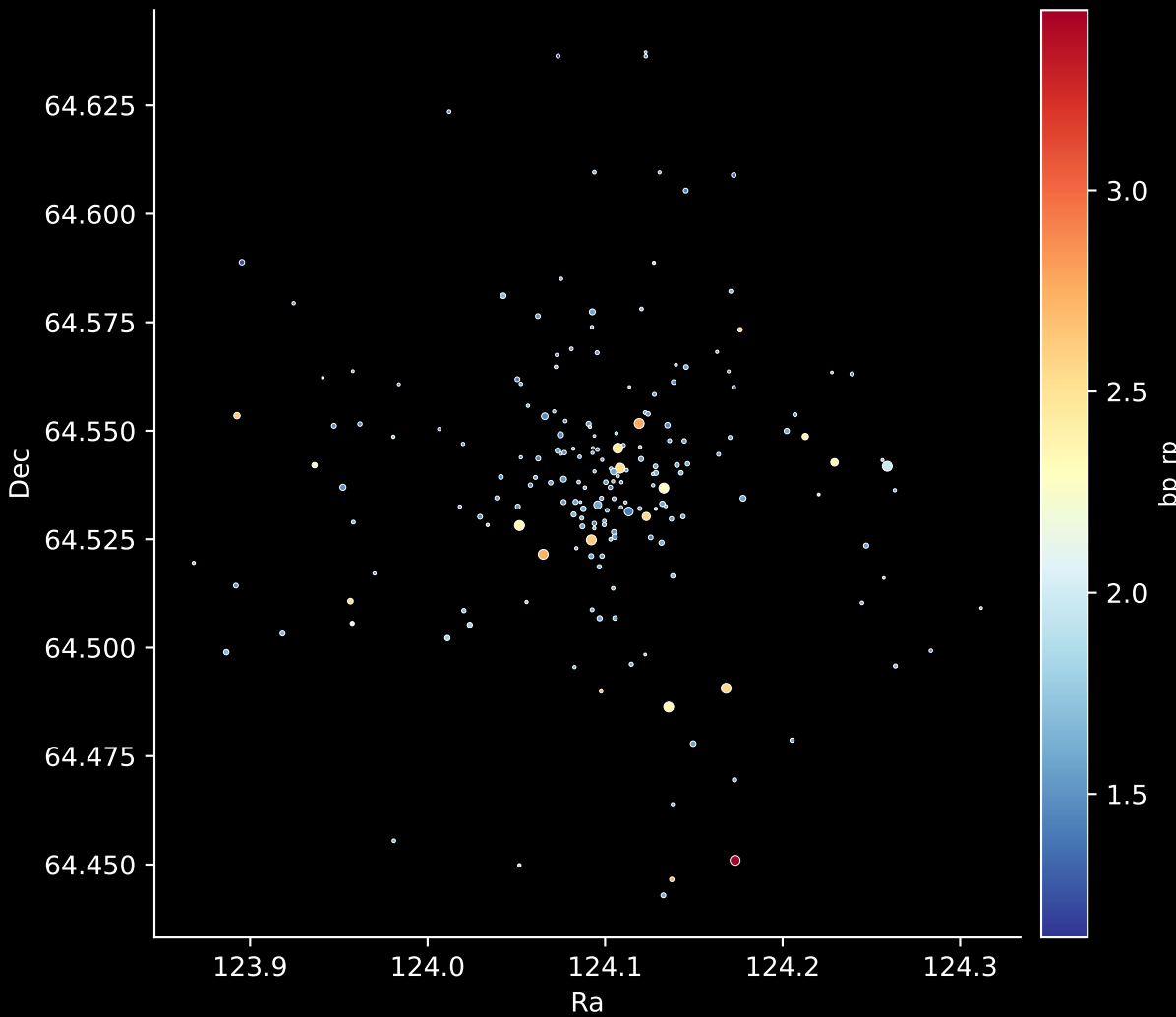
Gaia Cluster: [NGC_609] Stars: 192
