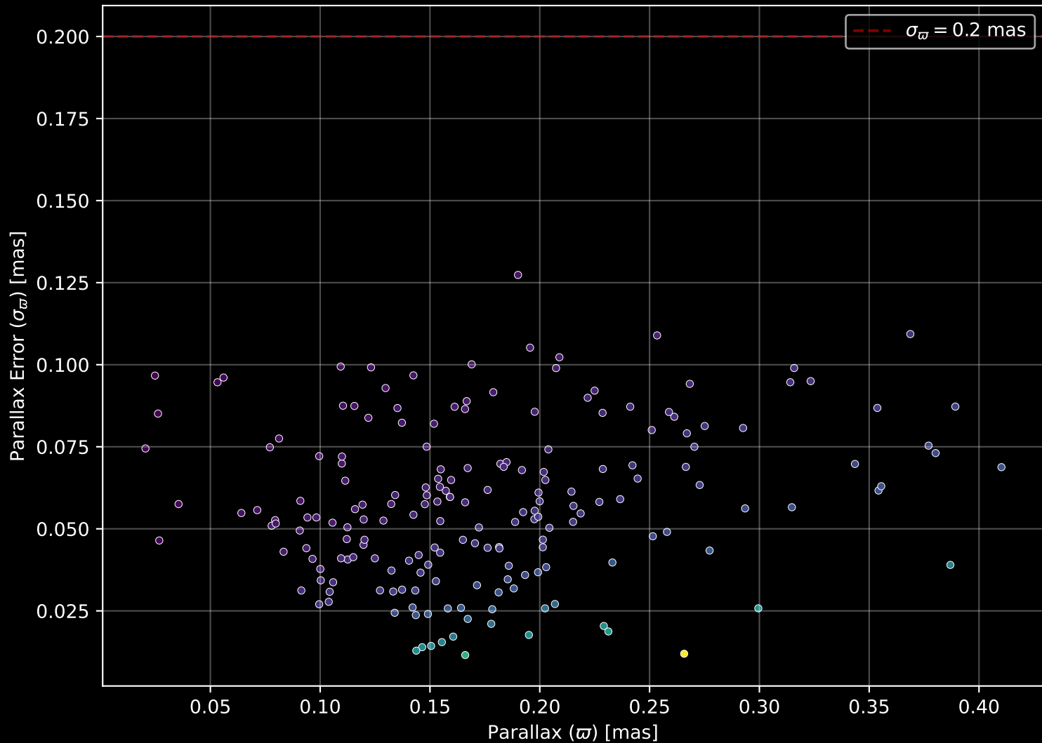
Gaia Cluster: [NGC_609] Parallax Quality (n= 192)
