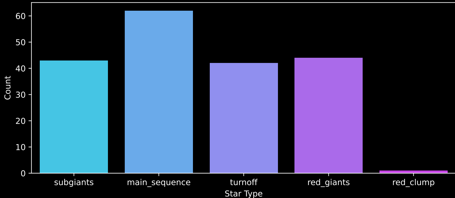
Gaia Cluster: [NGC_609] Count plot of Star Type
