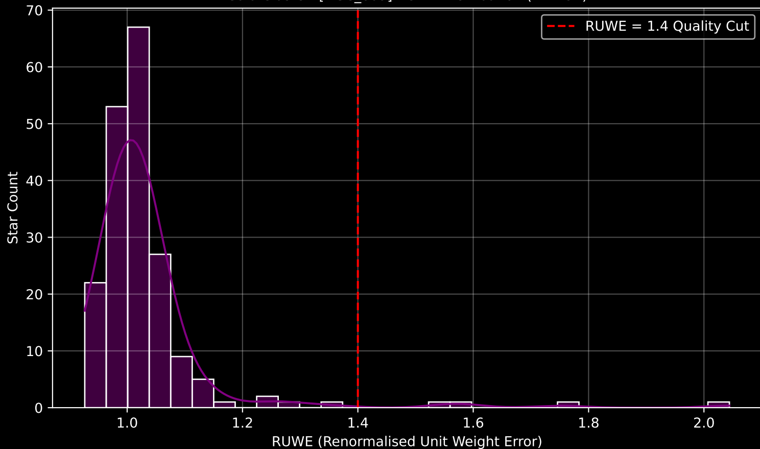
Gaia Cluster: [NGC_609] RUWE Distribution (n= 192)
