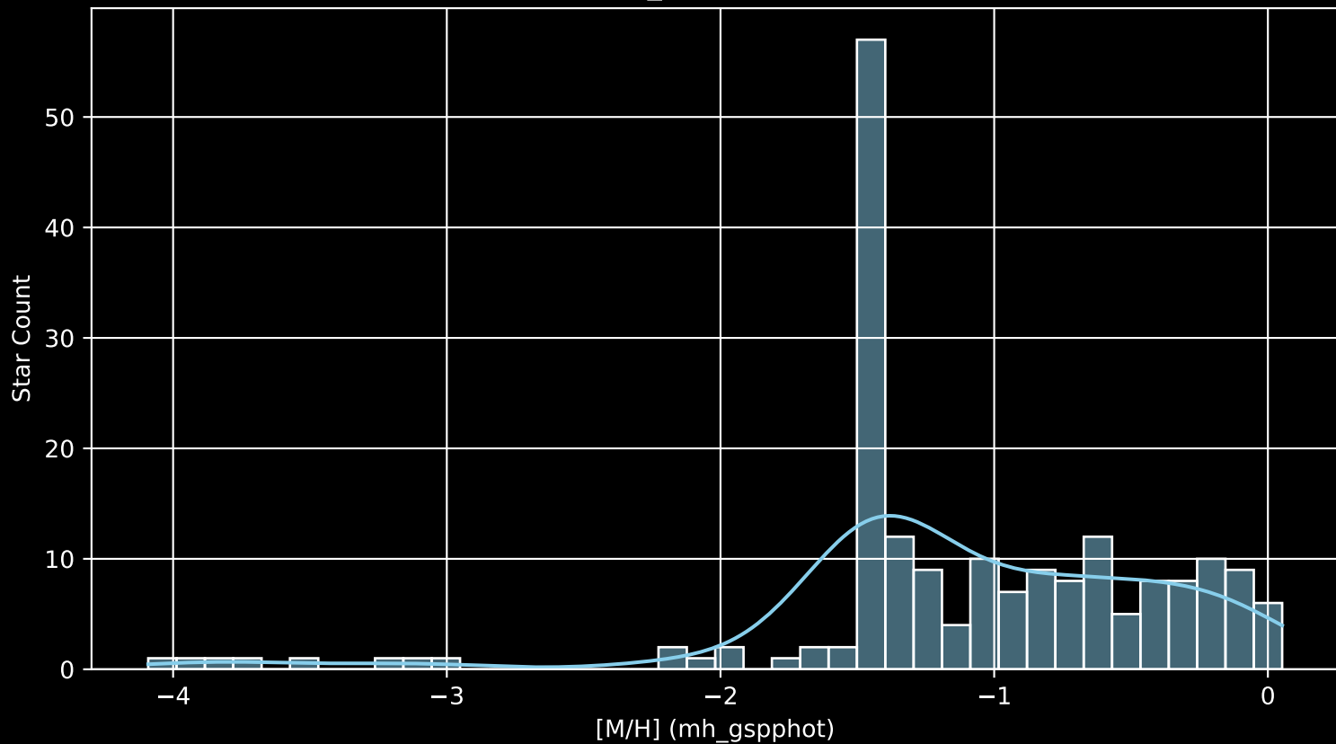
Gaia Cluster: [NGC_609 [M/H] (mh_gspphot) (n= 192)
