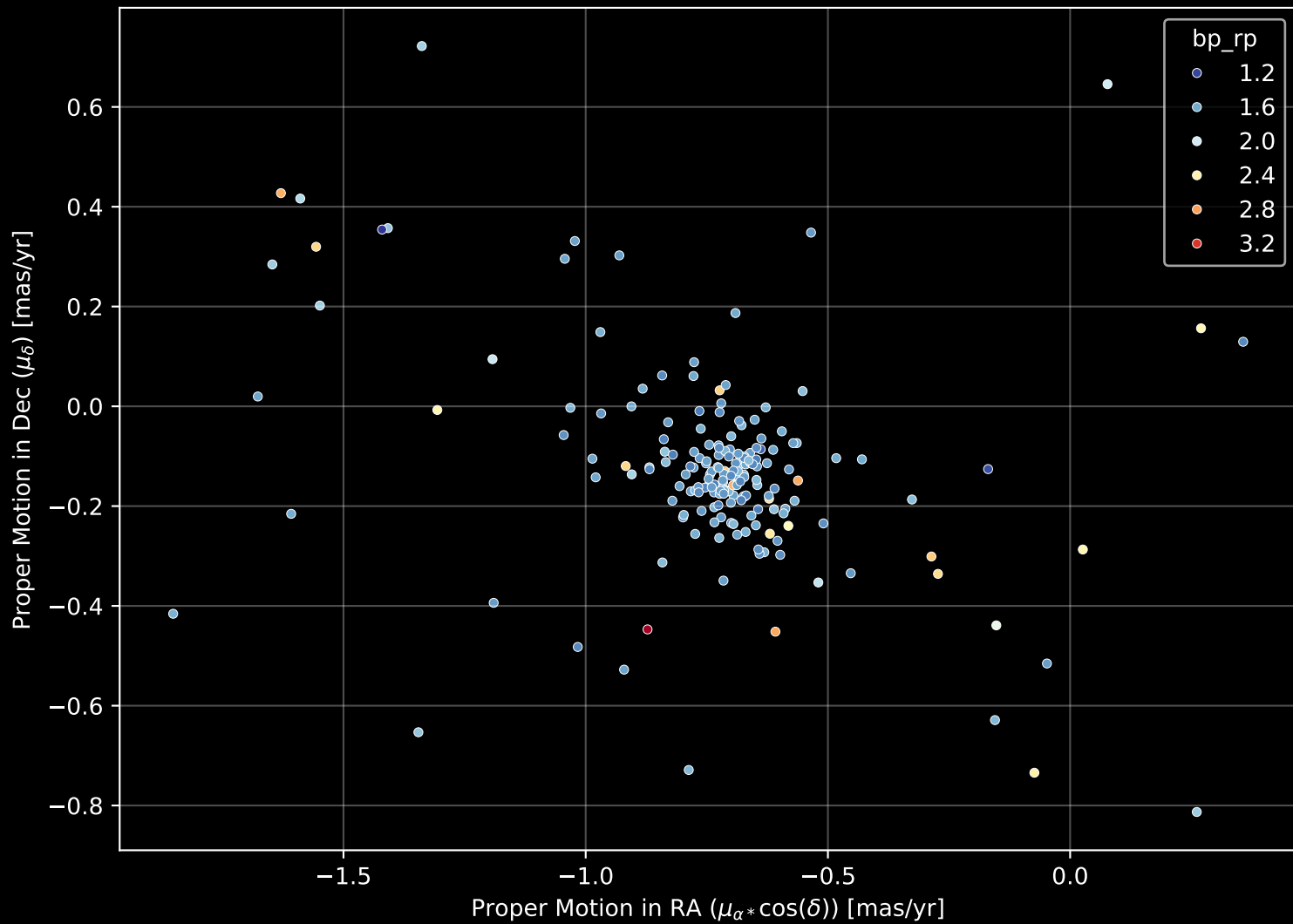
Gaia Cluster: [NGC_609] Proper Motion Diagram (n= 192)
