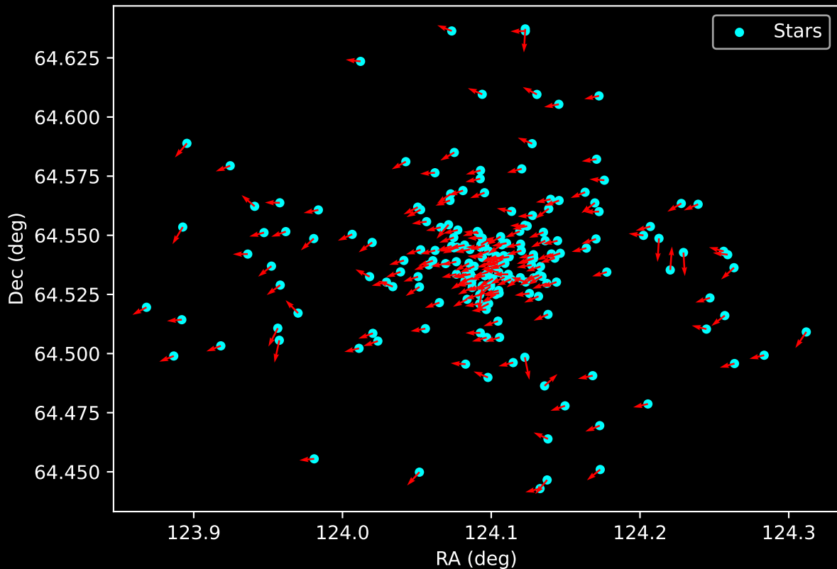
Gaia Cluster: [NGC_609] Proper Motion Vectors for Gaia Star Field (n= 192)
