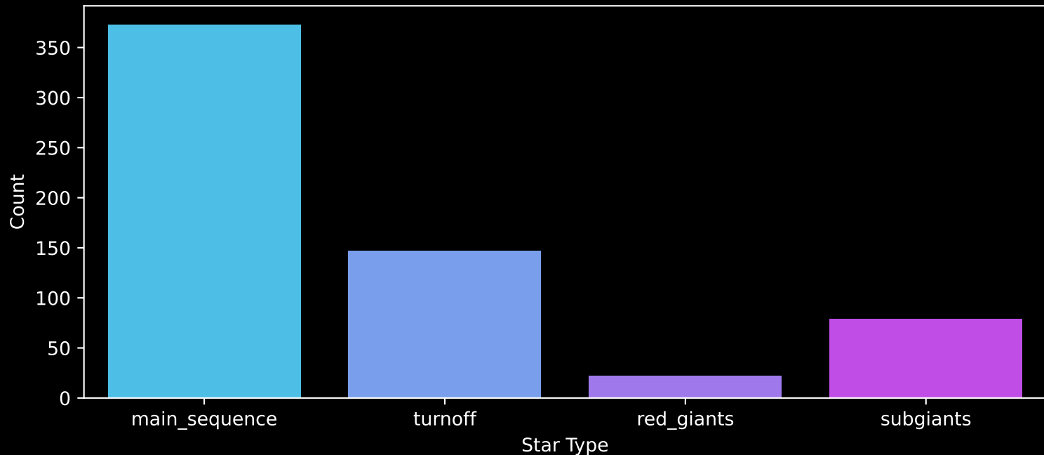
Gaia Cluster: [NGC_6167] Count plot of Star Type
