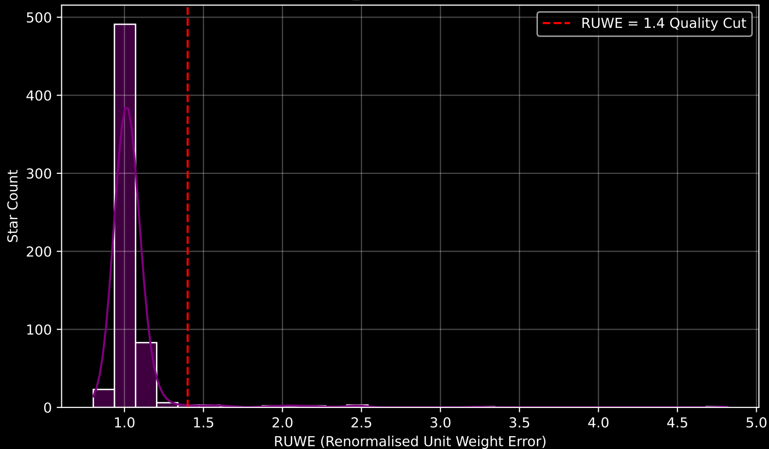
Gaia Cluster: [NGC_6167] RUWE Distribution (n= 621)
