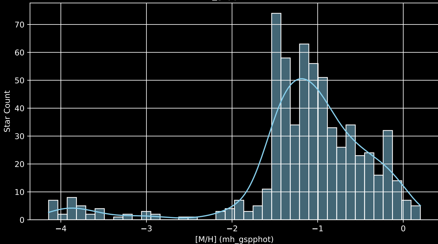
Gaia Cluster: [NGC_6167 [M/H] (mh_gspphot) (n= 621)
