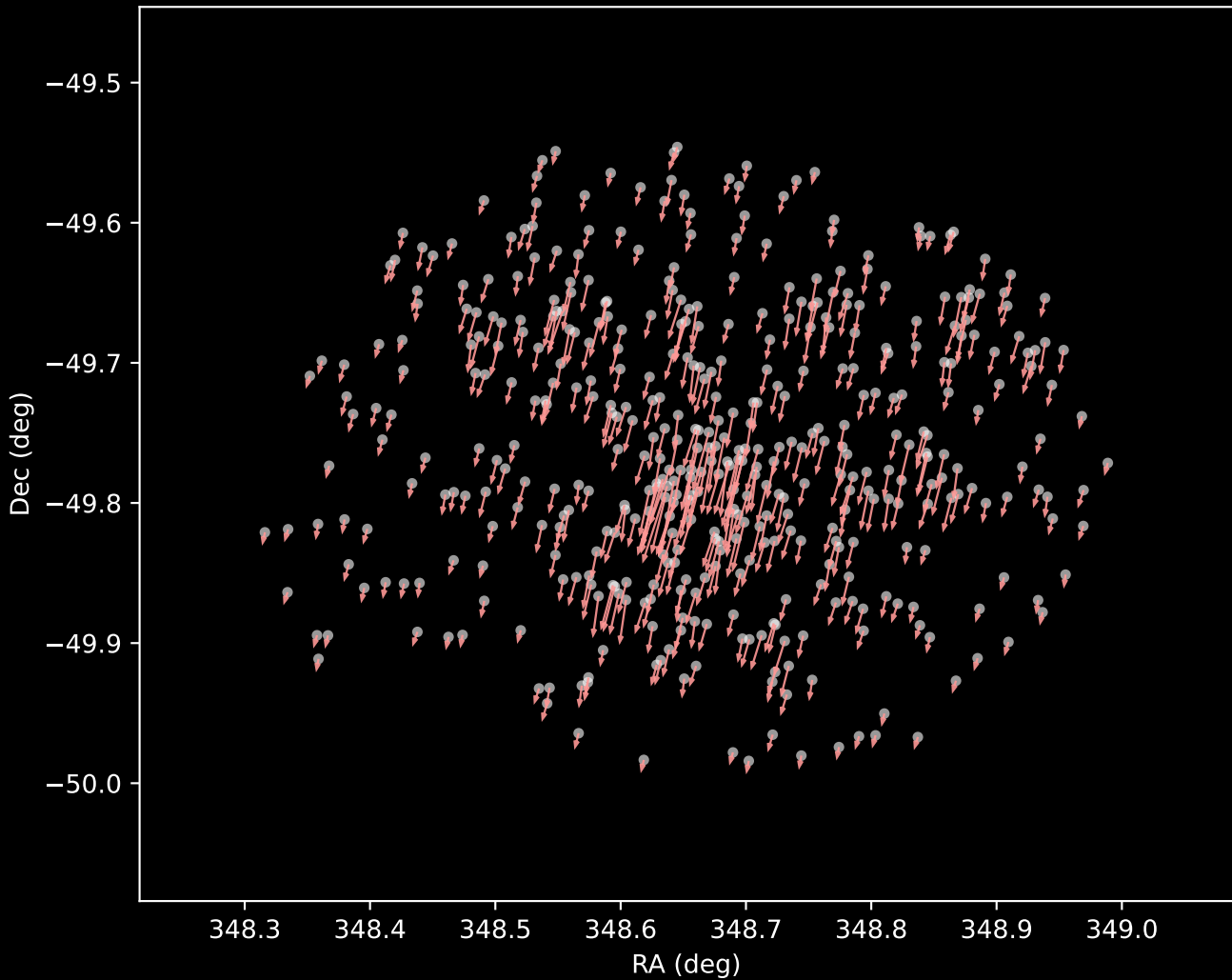
Gaia DR3 Cluster 7 Proper Motion Vectors (n=449)
