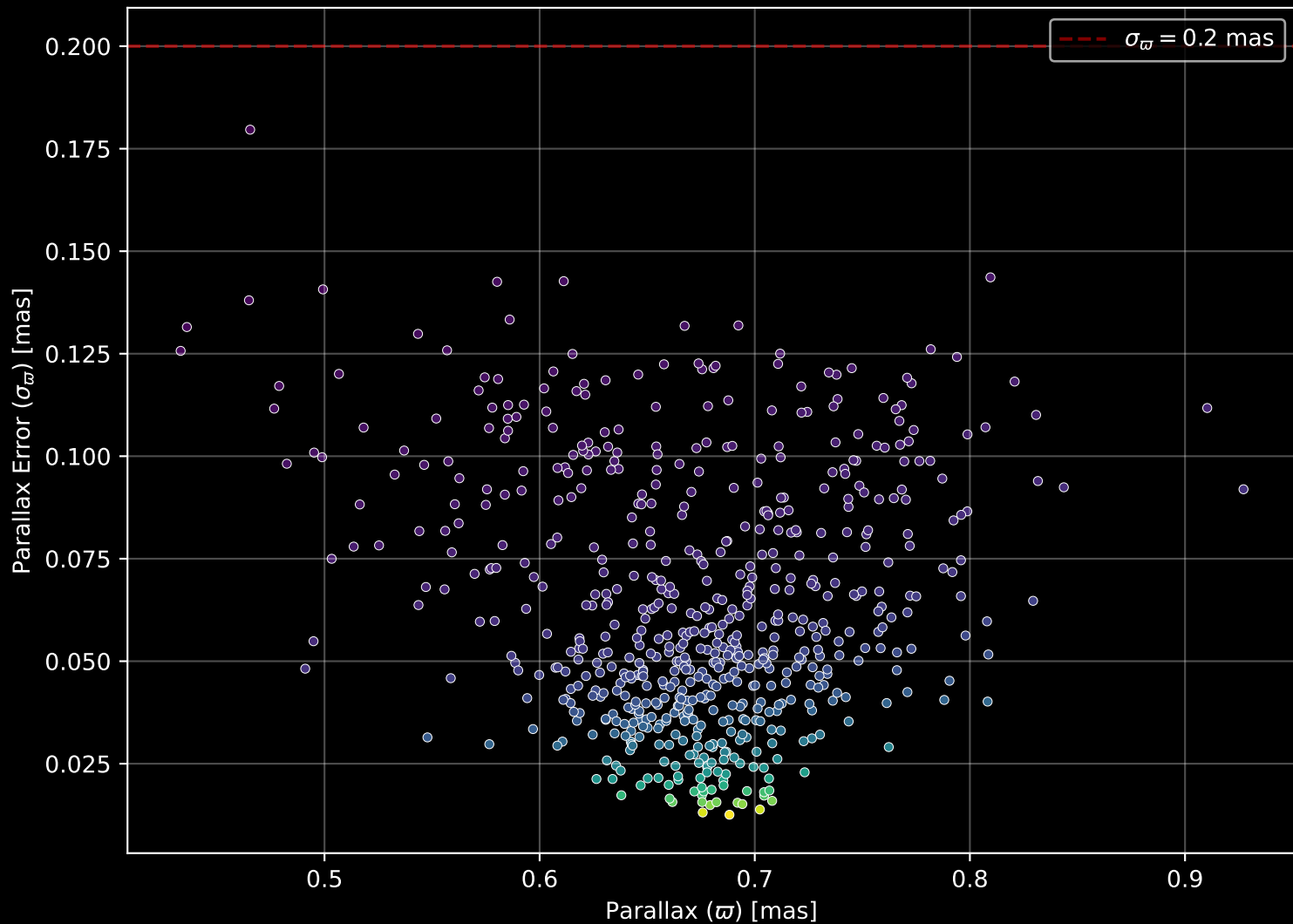
Gaia Cluster: [NGC_6167] Parallax Quality (n= 621)
