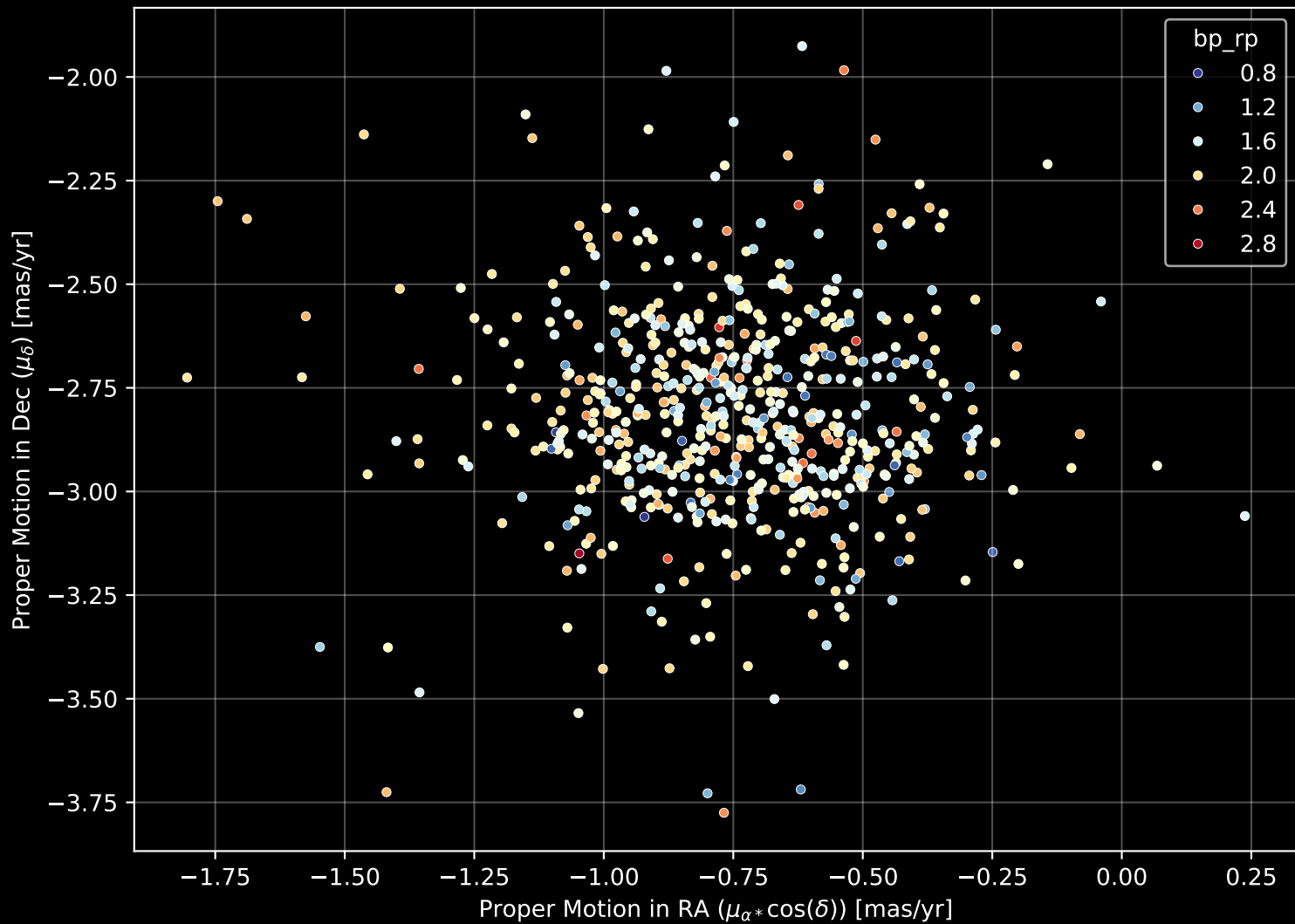
Gaia Cluster: [NGC_6167] Proper Motion Diagram (n= 621)
