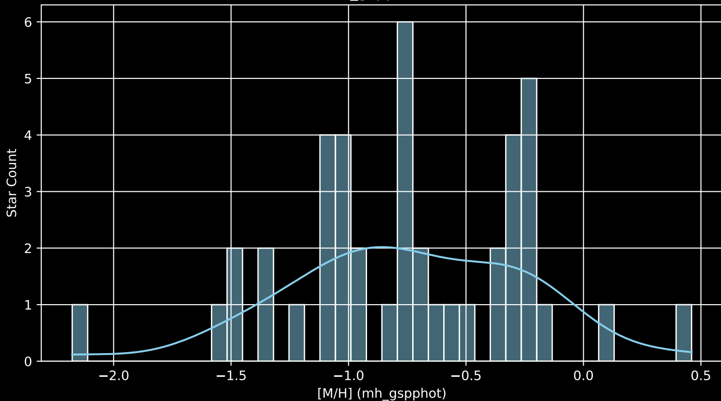
Gaia Cluster: [NGC_6178 [M/H] (mh_gspphot) (n= 43)
