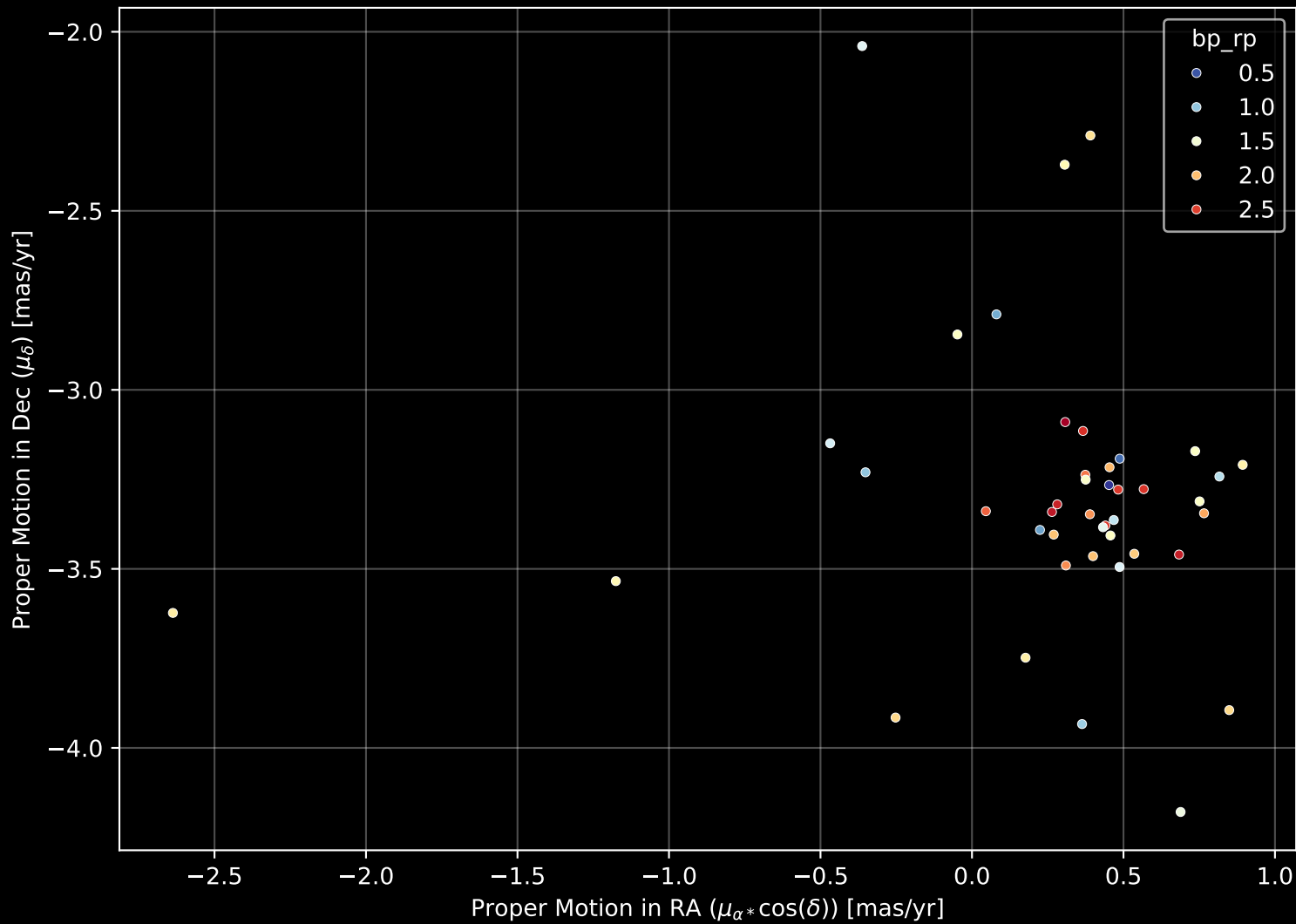
Gaia Cluster: [NGC_6178] Proper Motion Diagram (n= 43)
