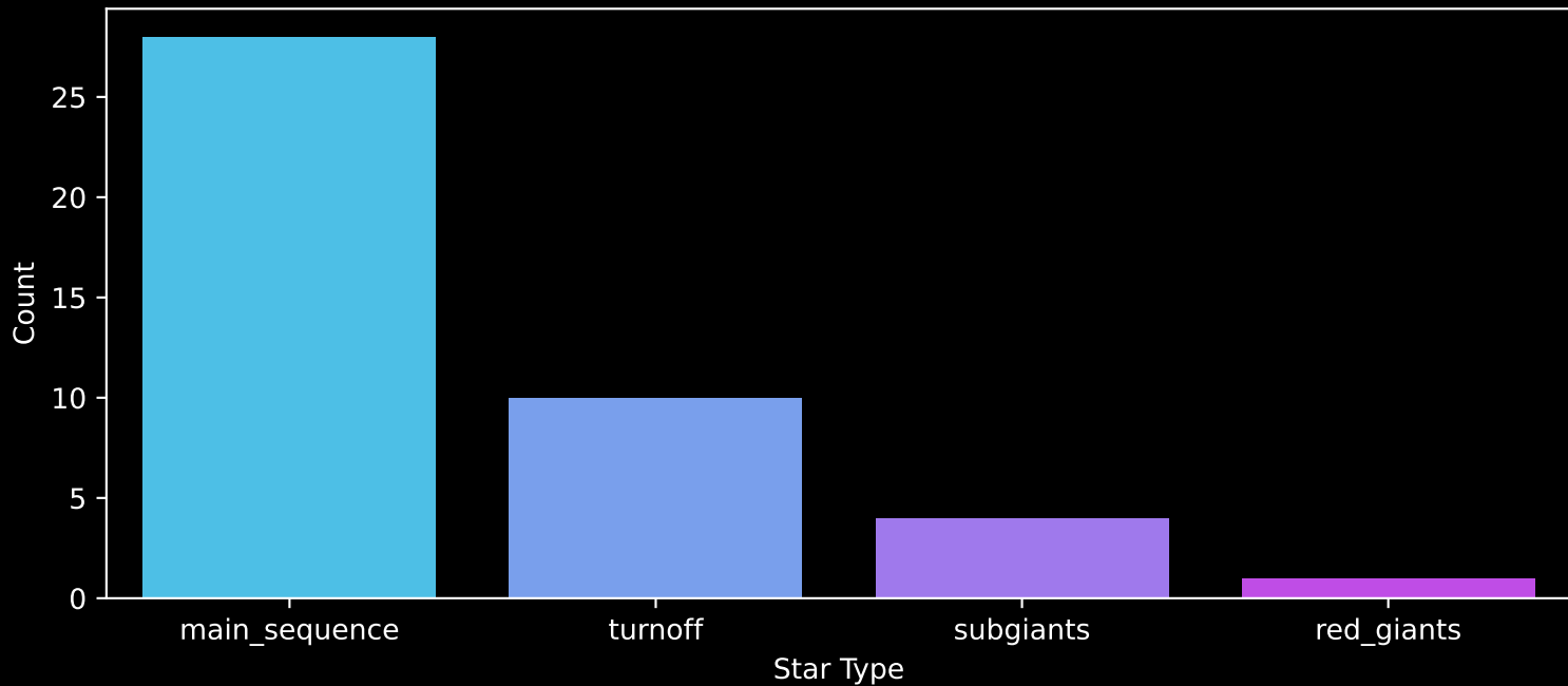
Gaia Cluster: [NGC_6178] Count plot of Star Type
