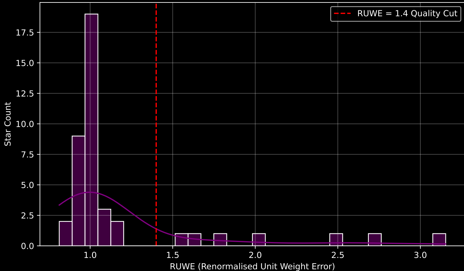
Gaia Cluster: [NGC_6178] RUWE Distribution (n= 42)
