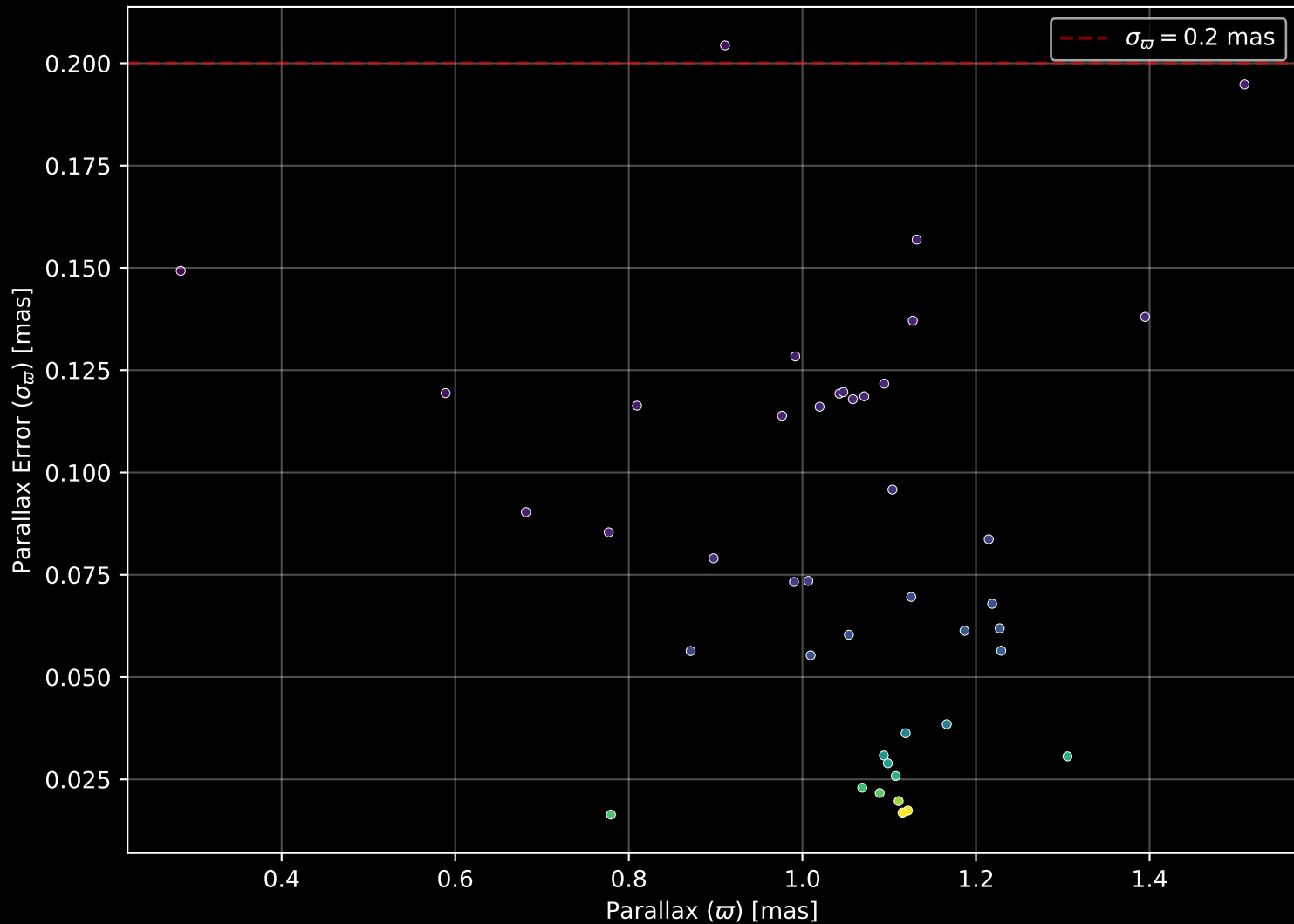
Gaia Cluster: [NGC_6178] Parallax Quality (n= 43)
