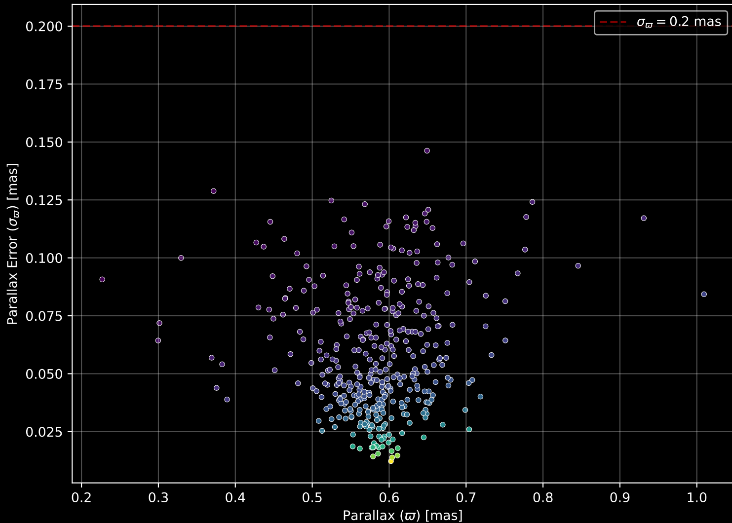
Gaia Cluster: [NGC_6192] Parallax Quality (n= 373)
