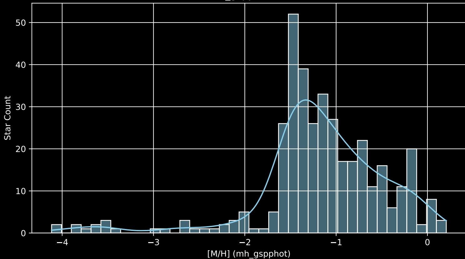
Gaia Cluster: [NGC_6192 [M/H] (mh_gspphot) (n= 372)
