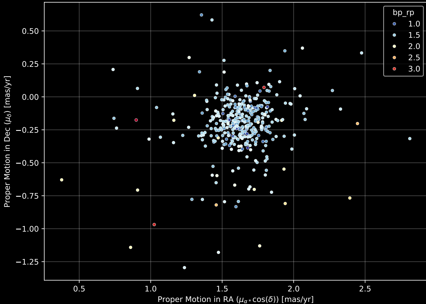
Gaia Cluster: [NGC_6192] Proper Motion Diagram (n= 373)
