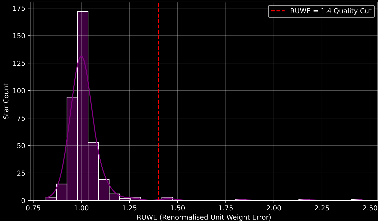
Gaia Cluster: [NGC_6192] RUWE Distribution (n= 373)
