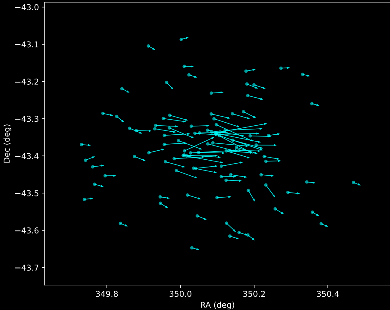
Gaia DR3 Noise Stream Proper Motion Vectors (n=96)
