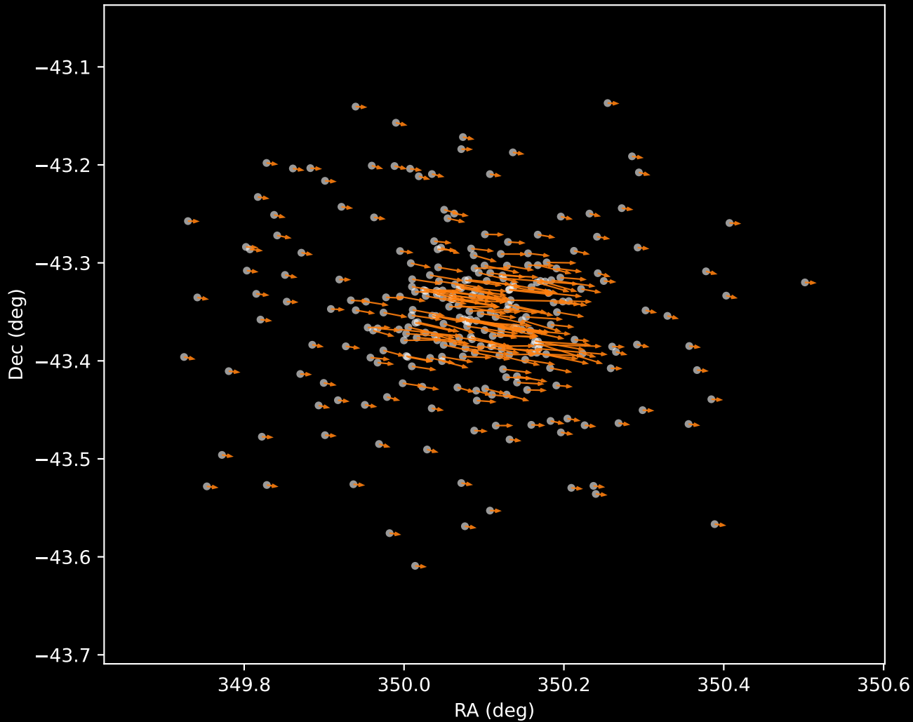
Gaia DR3 Cluster 2 Proper Motion Vectors (n=264)
