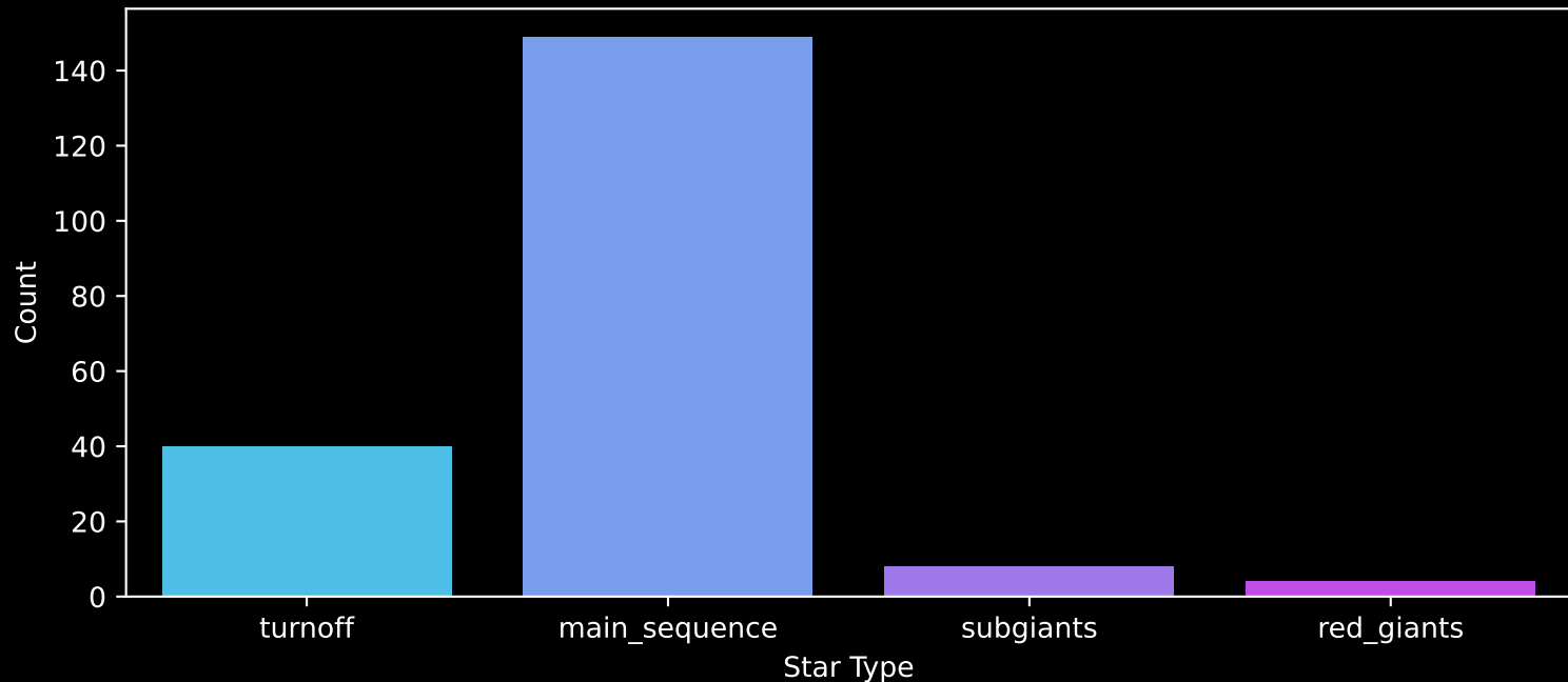
Gaia Cluster: [NGC_6204] Count plot of Star Type
