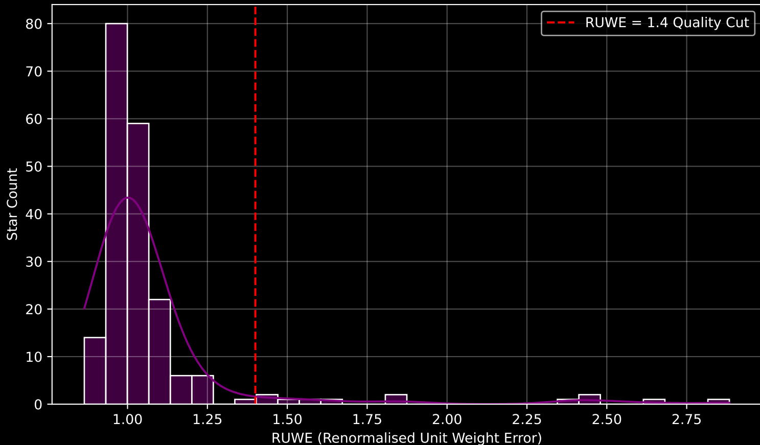
Gaia Cluster: [NGC_6204] RUWE Distribution (n= 200)
