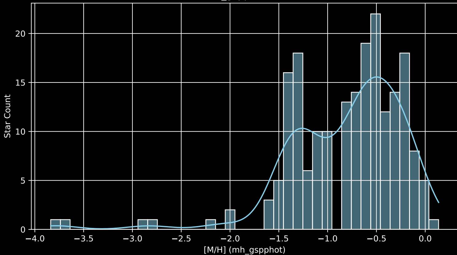
Gaia Cluster: [NGC_6204 [M/H] (mh_gspphot) (n= 201)
