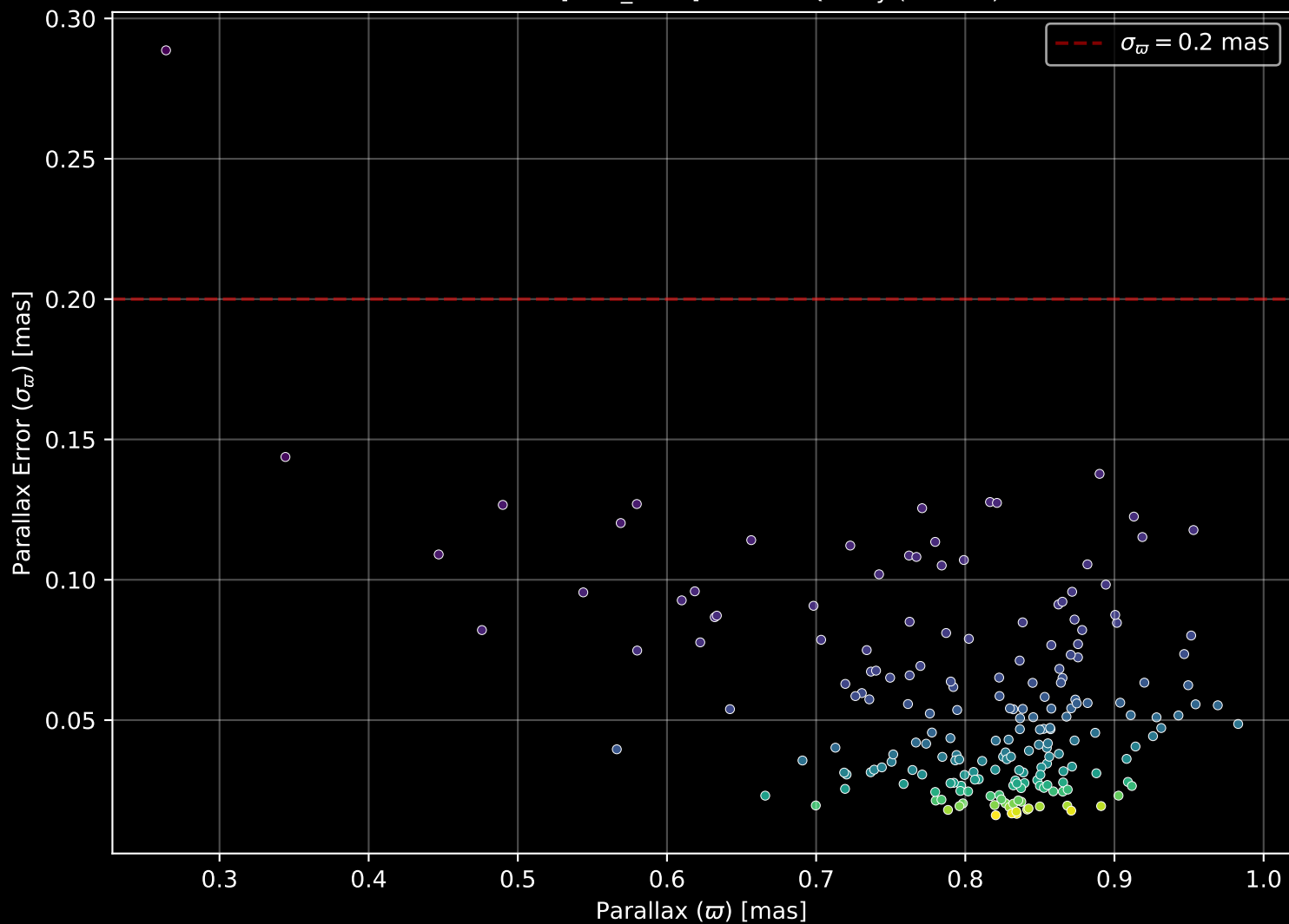
Gaia Cluster: [NGC_6204] Parallax Quality (n= 201)
