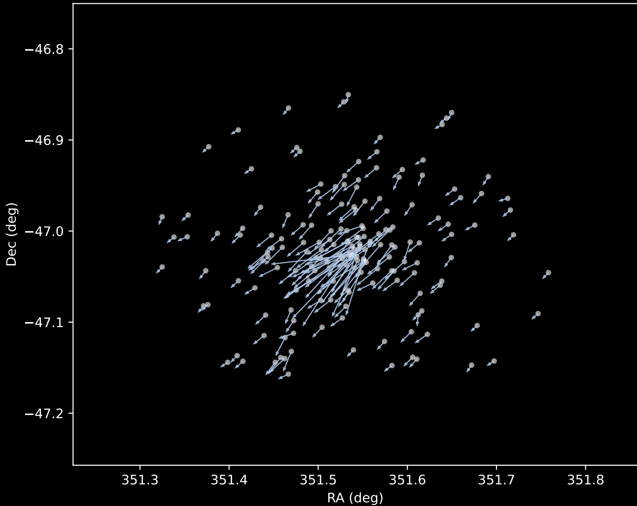
Gaia DR3 Cluster 1 Proper Motion Vectors (n=177)
