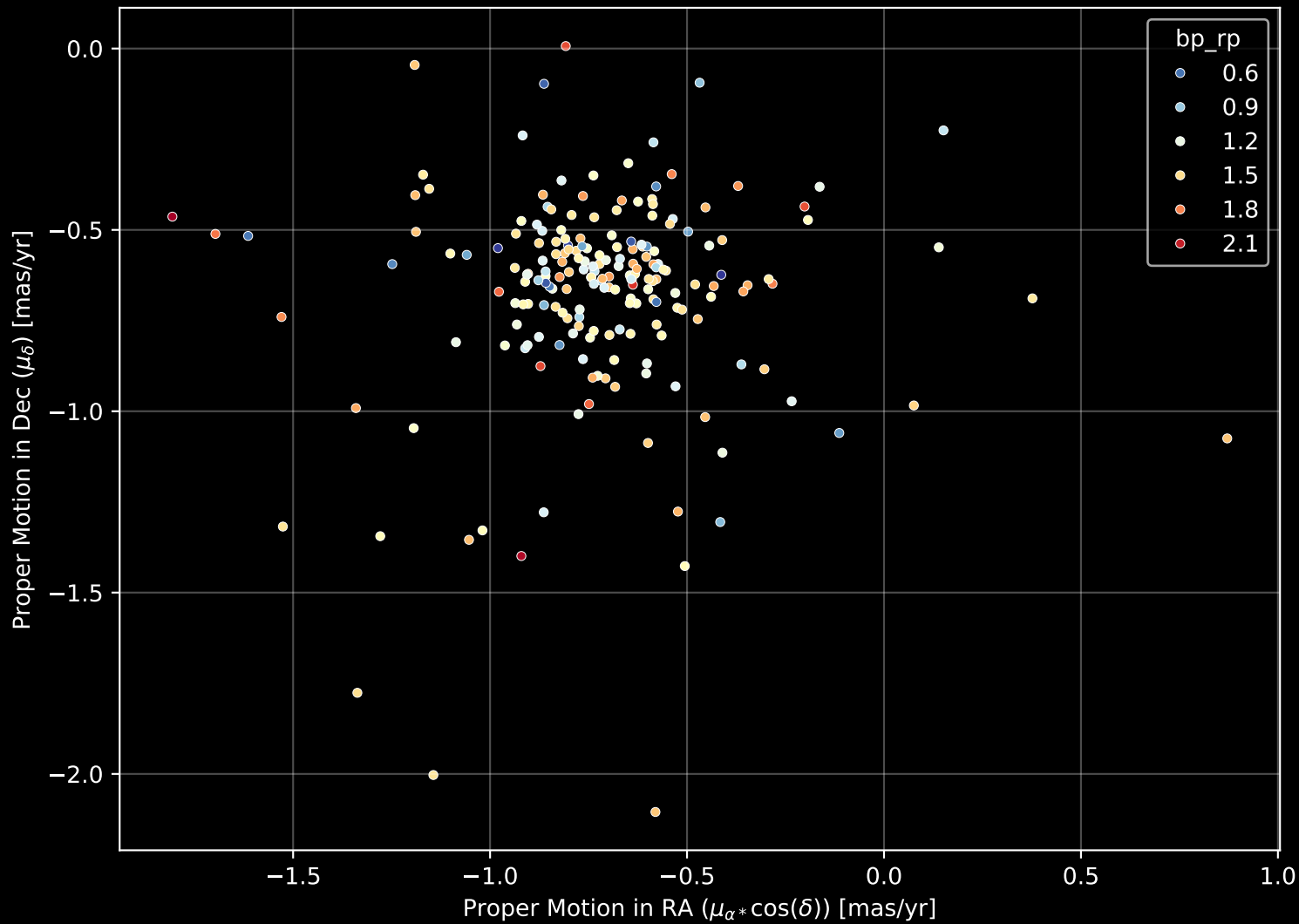
Gaia Cluster: [NGC_6204] Proper Motion Diagram (n= 201)
