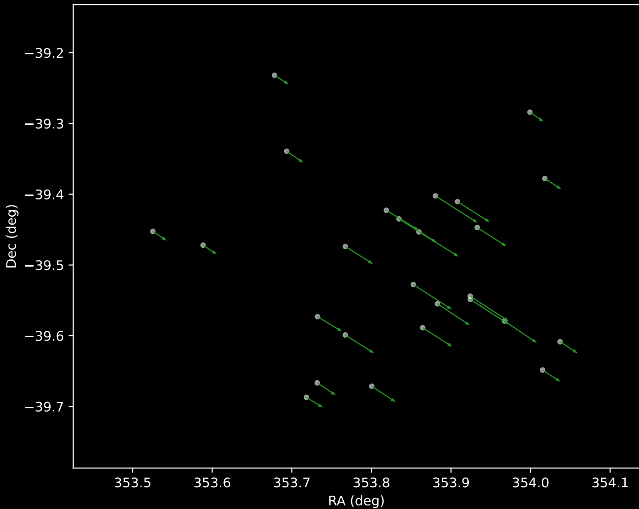
Gaia DR3 Cluster 24 Proper Motion Vectors (n=26)
