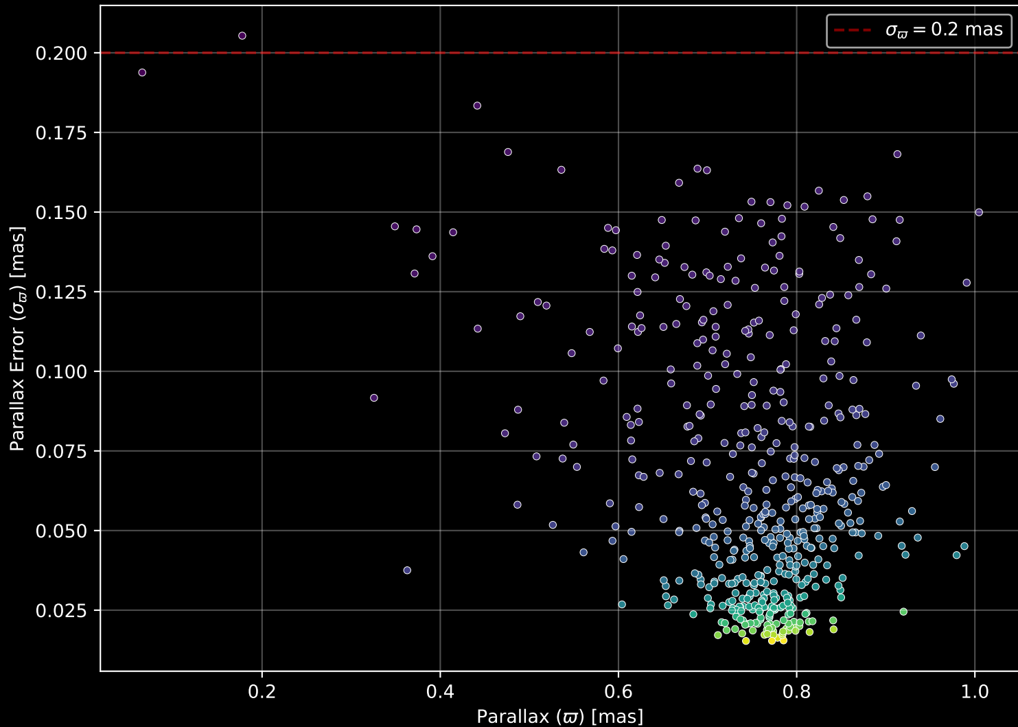
Gaia Cluster: [NGC_6242] Parallax Quality (n= 523)
