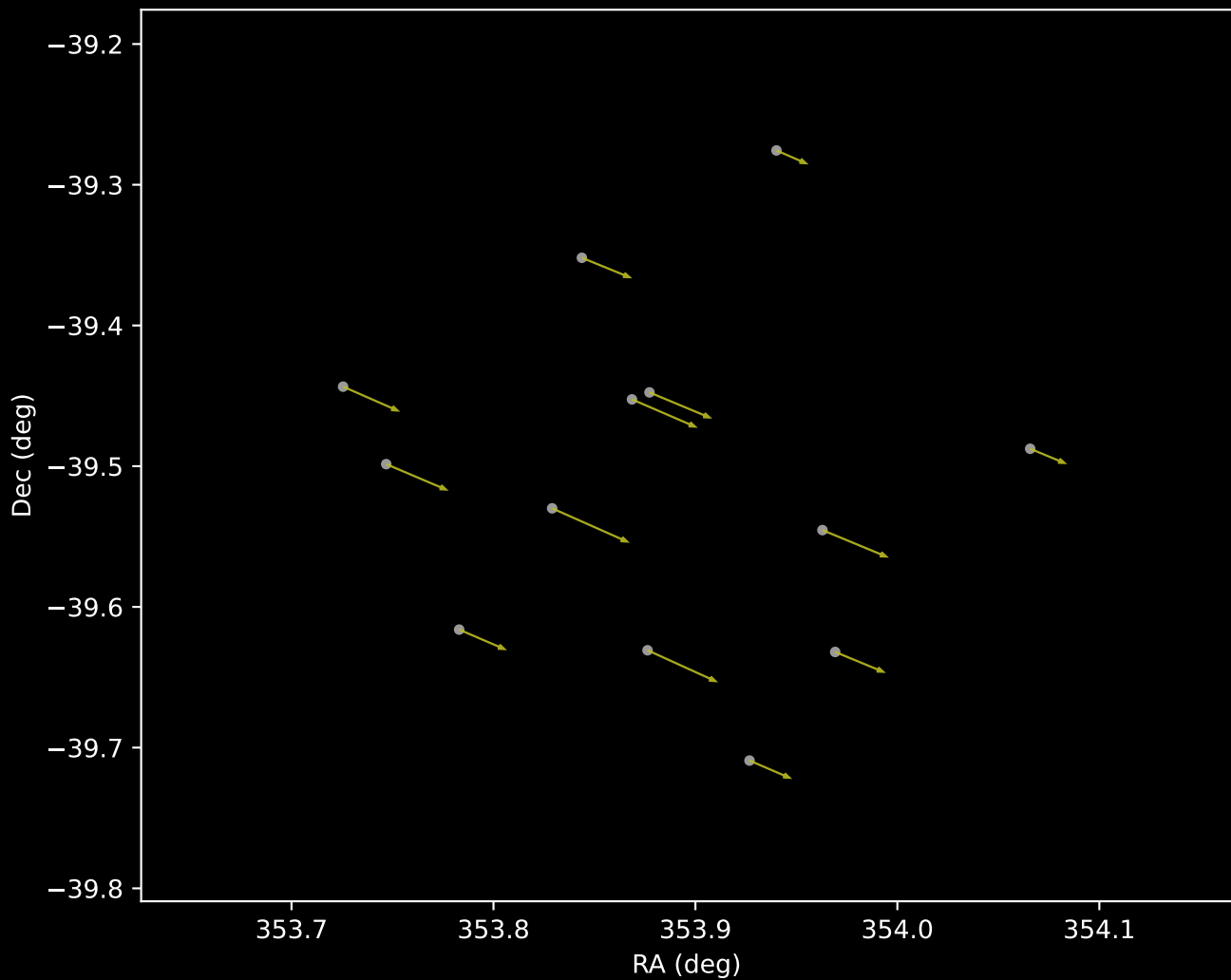
Gaia DR3 Cluster 16 Proper Motion Vectors (n=13)
