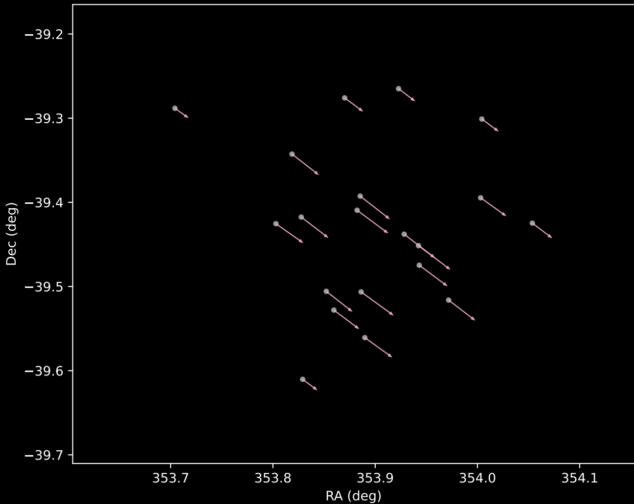
Gaia DR3 Cluster 13 Proper Motion Vectors (n=20)
