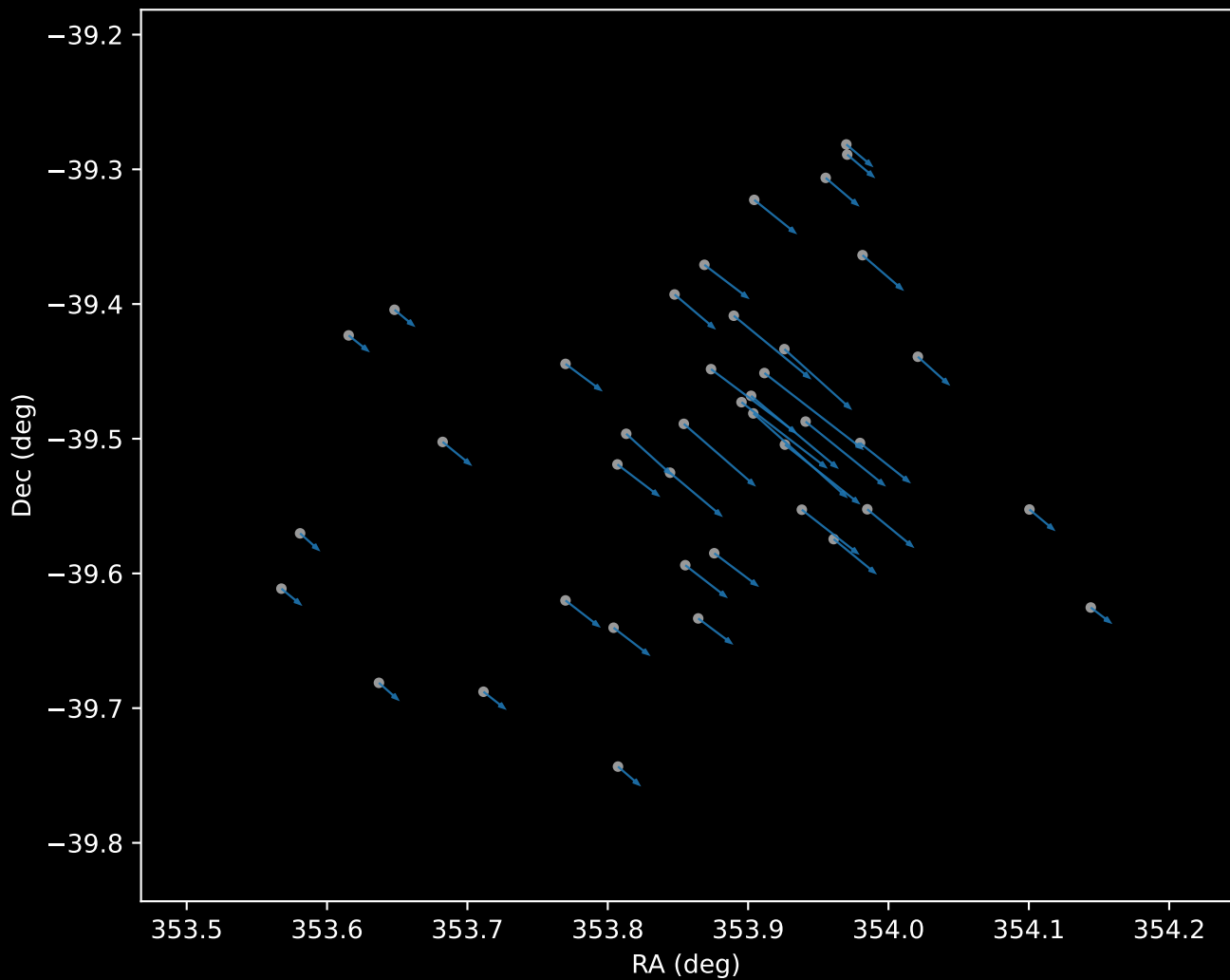
Gaia DR3 Cluster 20 Proper Motion Vectors (n=41)
