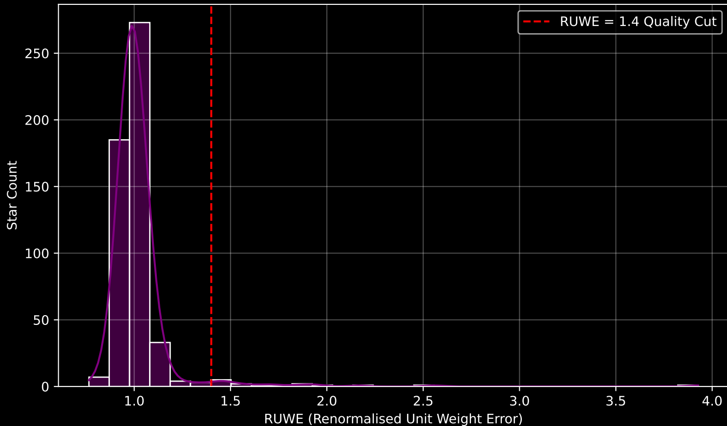
Gaia Cluster: [NGC_6242] RUWE Distribution (n= 520)
