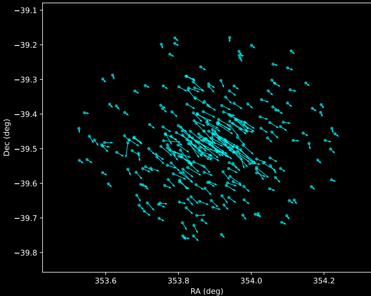
Gaia DR3 Noise Stream Proper Motion Vectors (n=260)
