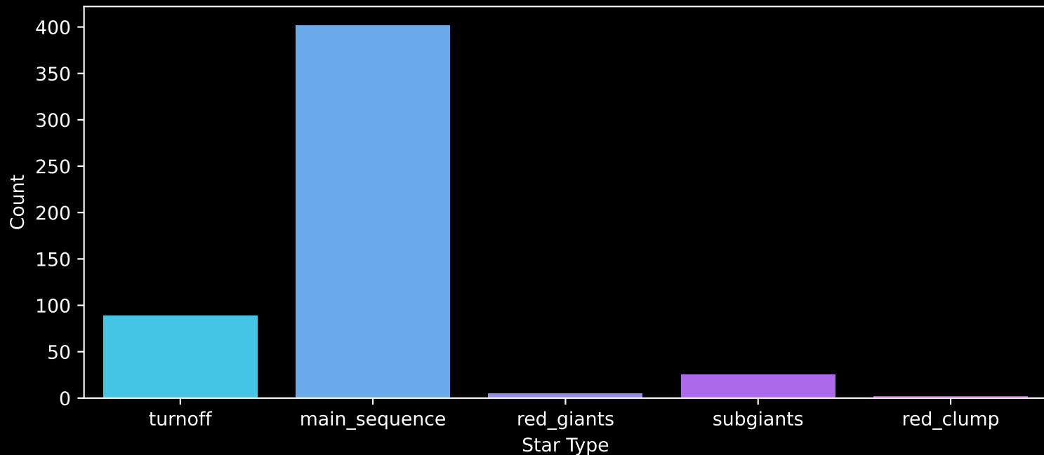
Gaia Cluster: [NGC_6242] Count plot of Star Type
