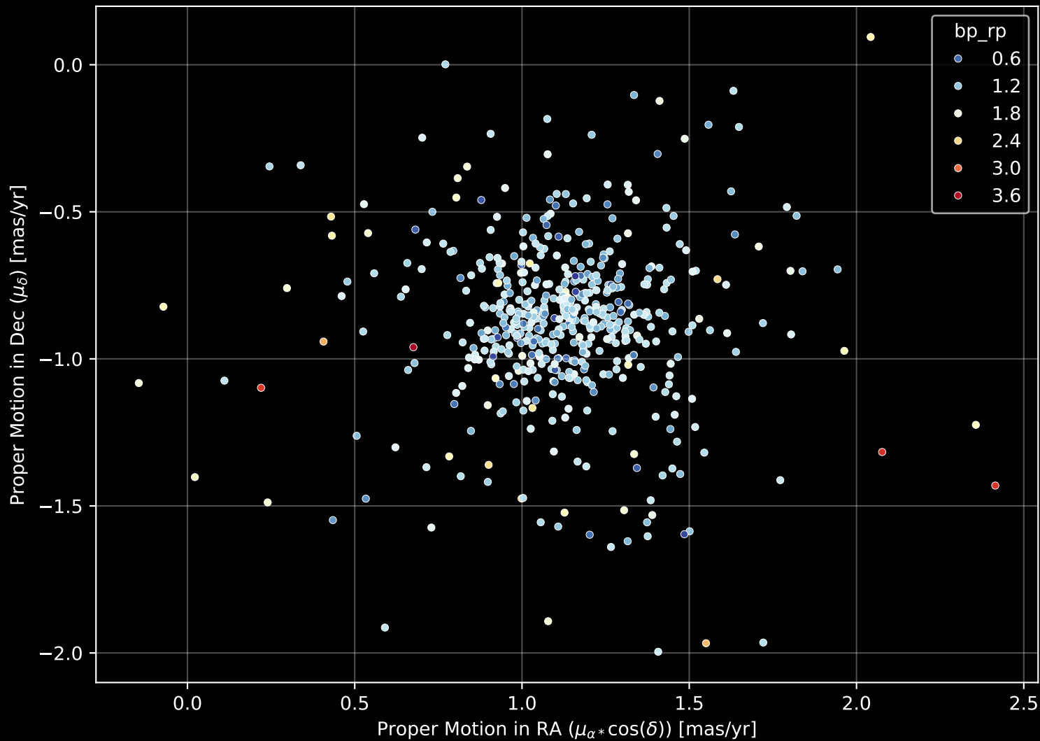
Gaia Cluster: [NGC_6242] Proper Motion Diagram (n= 523)
