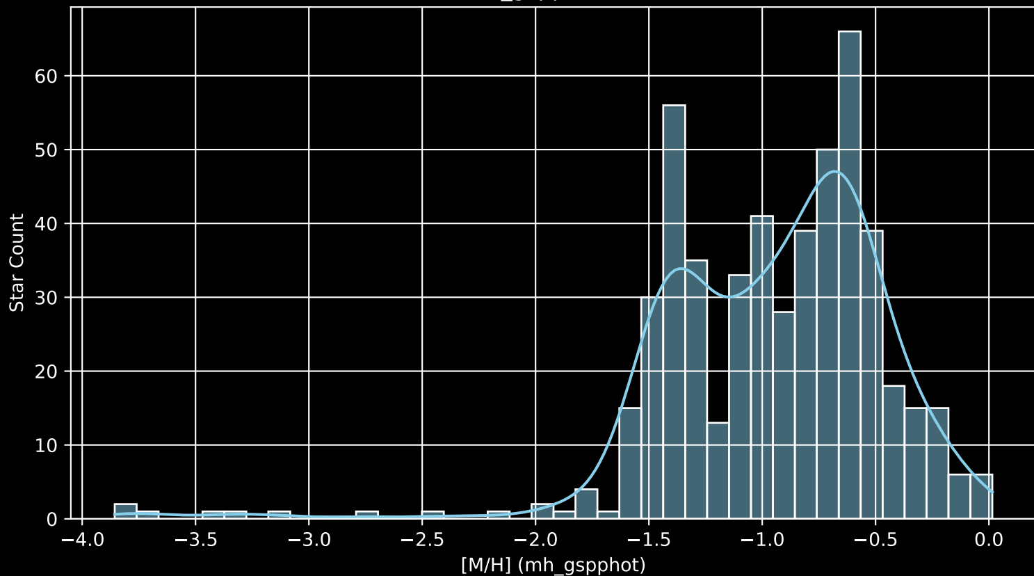
Gaia Cluster: [NGC_6242 [M/H] (mh_gspphot) (n= 522)
