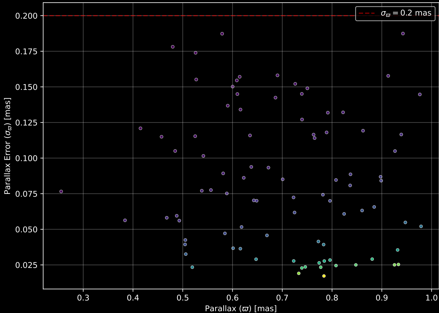
Gaia Cluster: [NGC_6322] Parallax Quality (n= 89)
