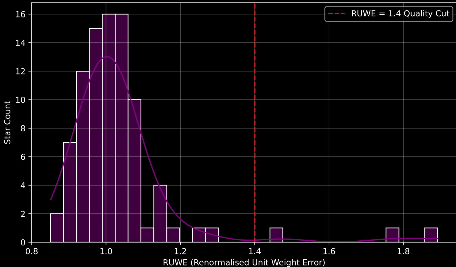
Gaia Cluster: [NGC_6322] RUWE Distribution (n= 89)
