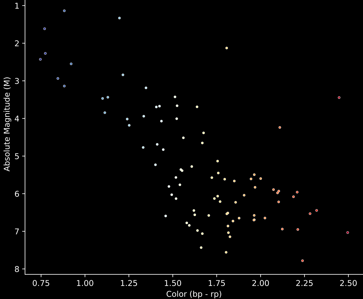
Gaia Cluster: [NGC_6322] Stars (n= 89) Hertzsprung-Russel Diagram
