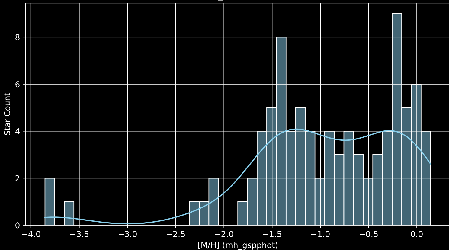
Gaia Cluster: [NGC_6322 [M/H] (mh_gspphot) (n= 89)
