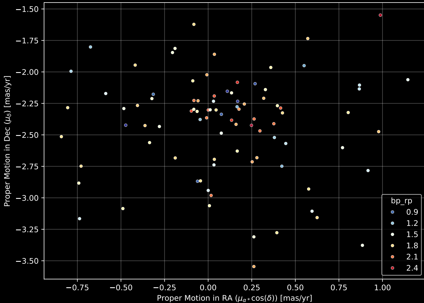
Gaia Cluster: [NGC_6322] Proper Motion Diagram (n= 89)
