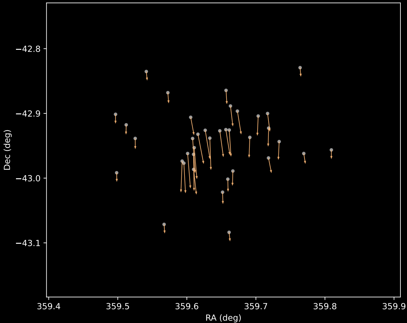
Gaia DR3 Cluster 3 Proper Motion Vectors (n=37)
