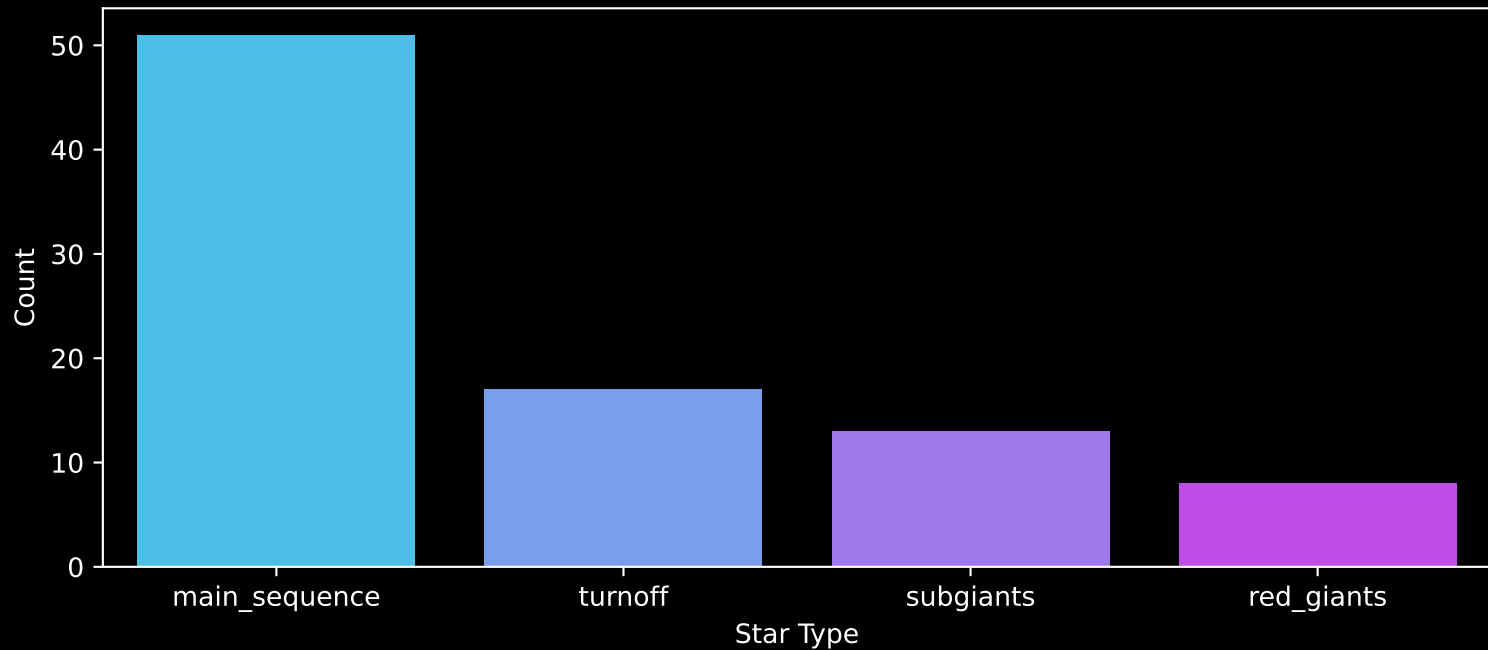
Gaia Cluster: [NGC_6322] Count plot of Star Type
