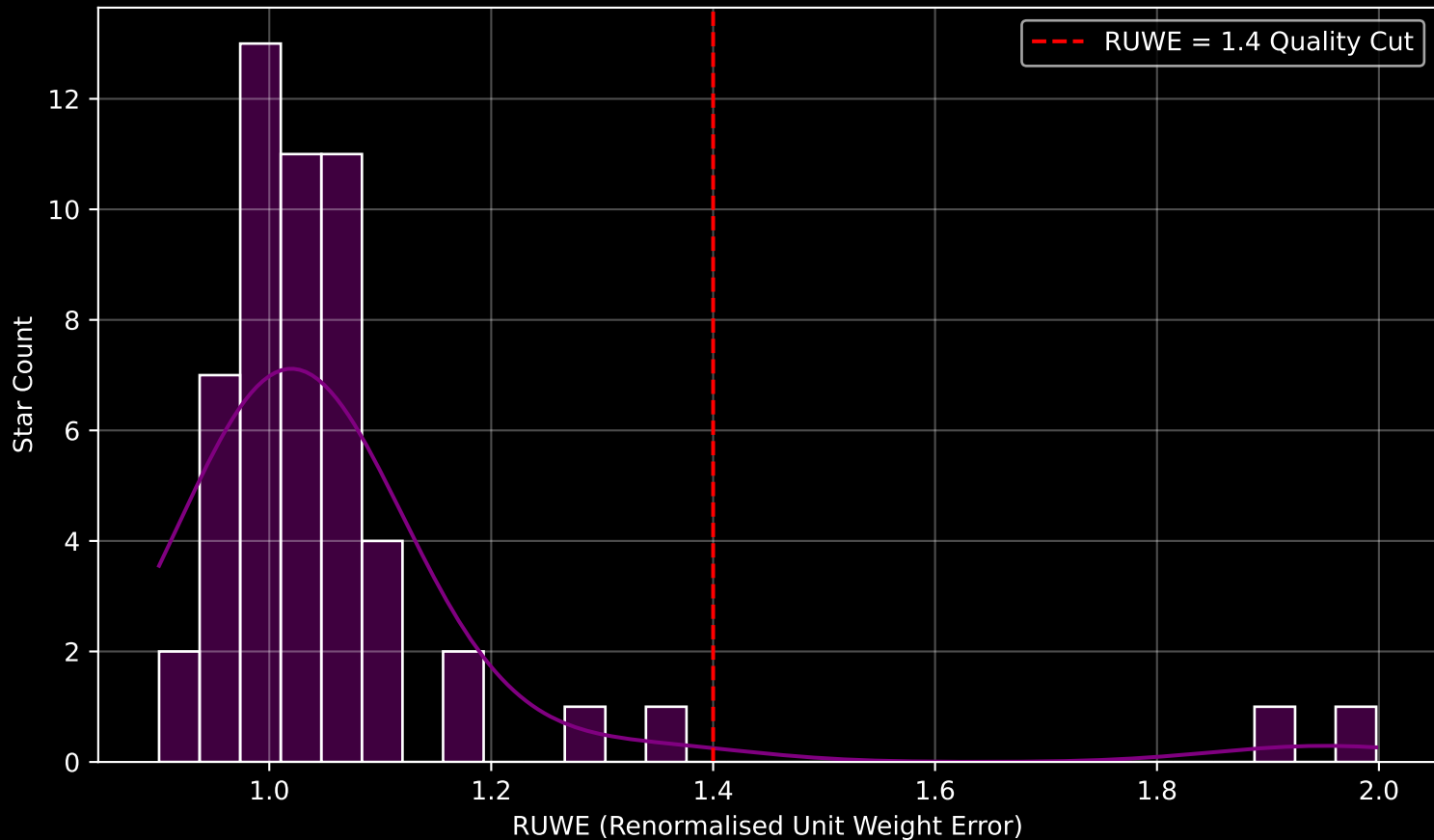
Gaia Cluster: [NGC_6357] RUWE Distribution (n= 54)
