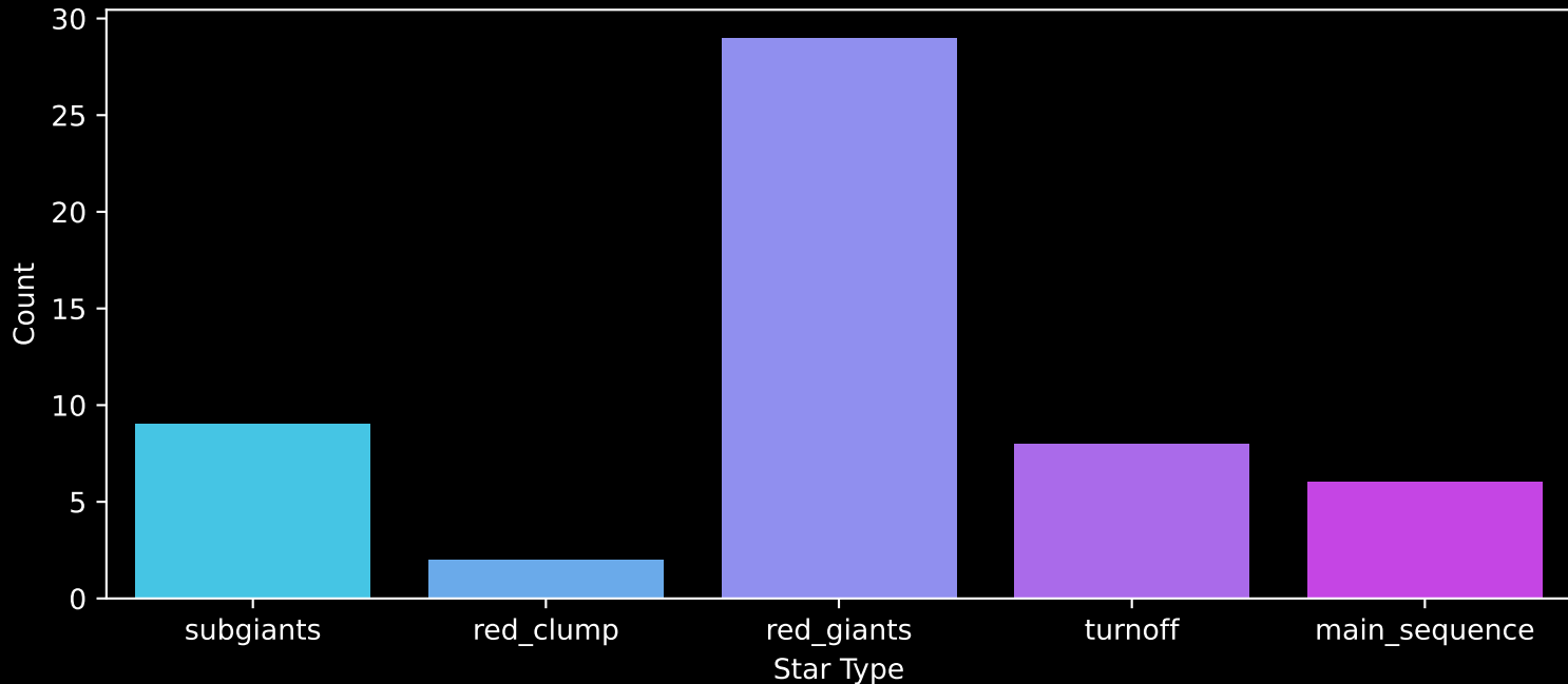
Gaia Cluster: [NGC_6357] Count plot of Star Type
