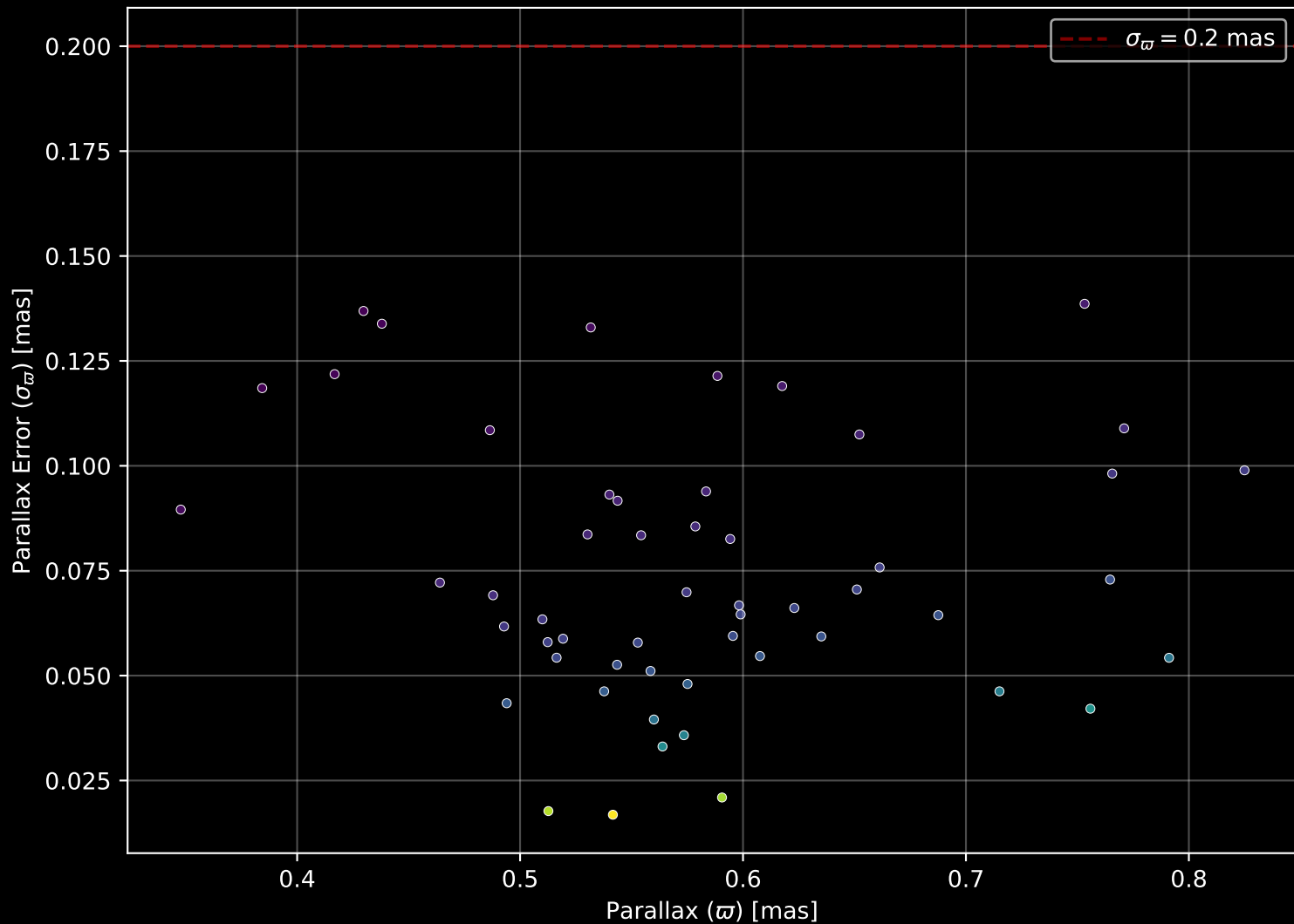
Gaia Cluster: [NGC_6357] Parallax Quality (n= 54)
