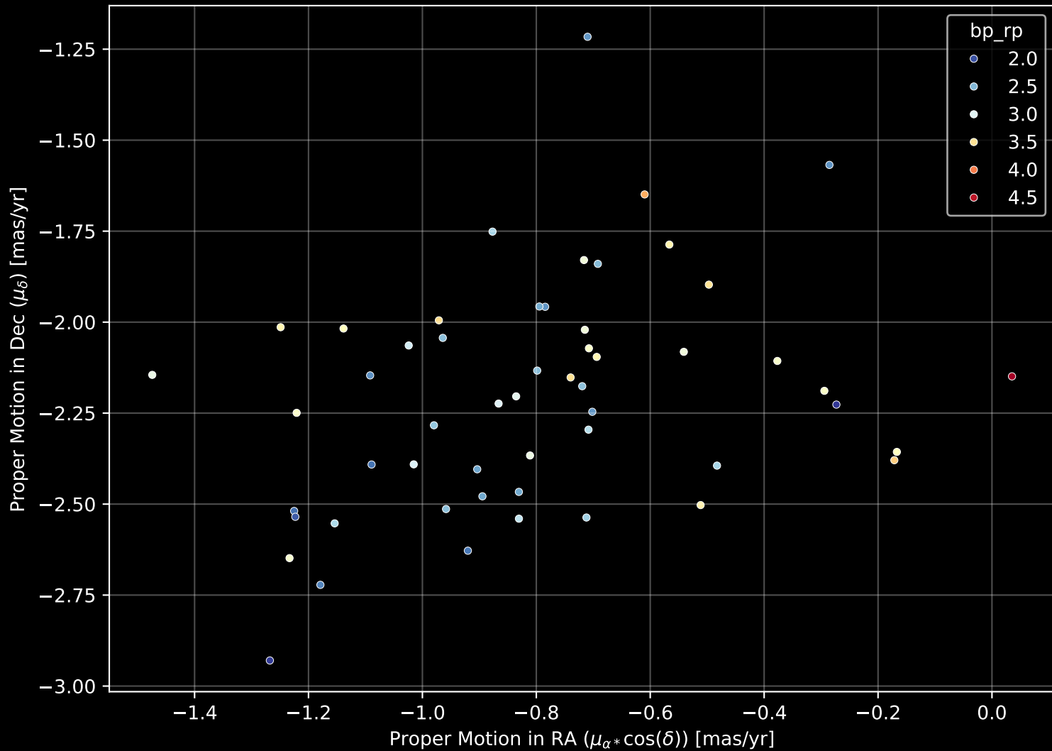
Gaia Cluster: [NGC_6357] Proper Motion Diagram (n= 54)
