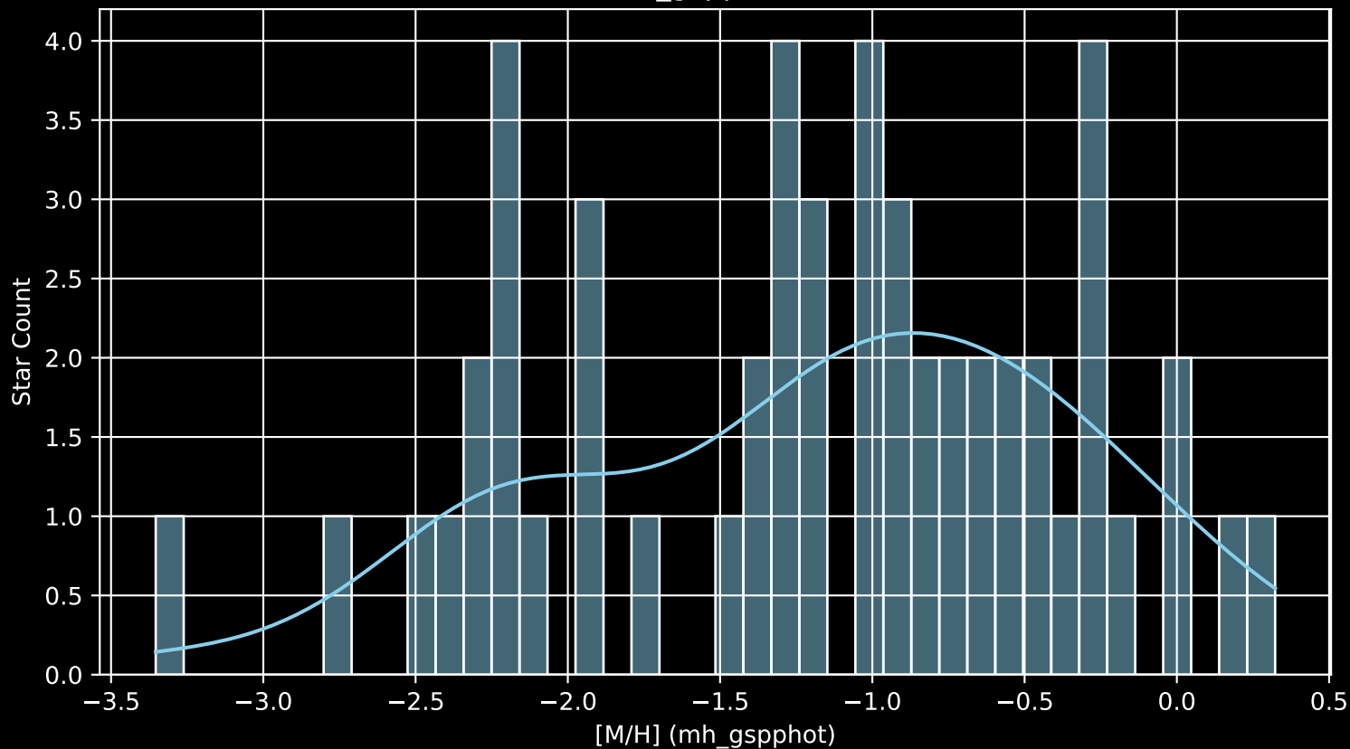
Gaia Cluster: [NGC_6357 [M/H] (mh_gspphot) (n= 52)
