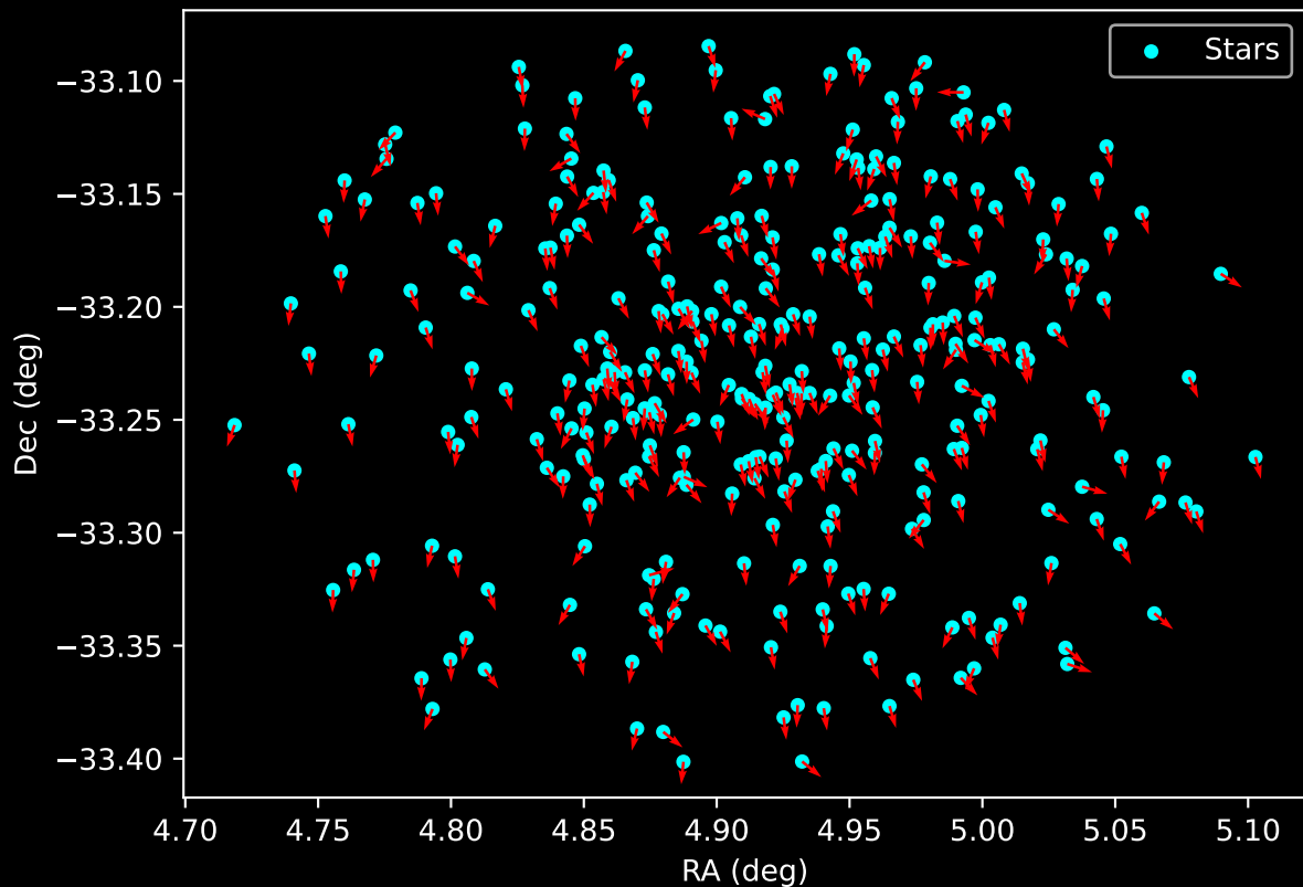
Gaia Cluster: [NGC_6404] Proper Motion Vectors for Gaia Star Field (n= 334)
