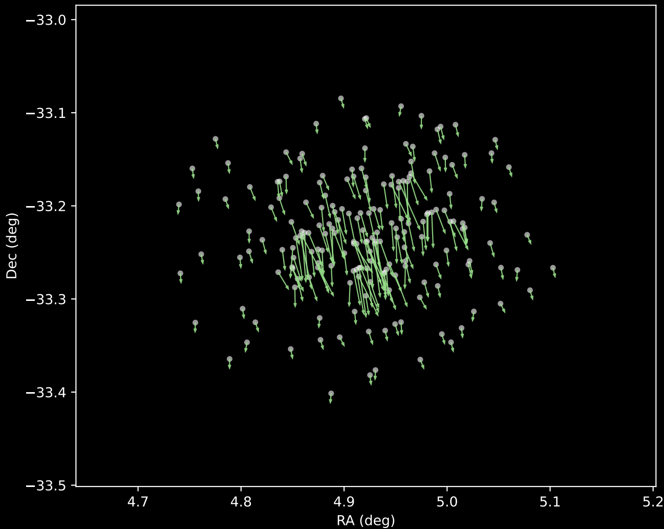
Gaia DR3 Cluster 5 Proper Motion Vectors (n=188)
