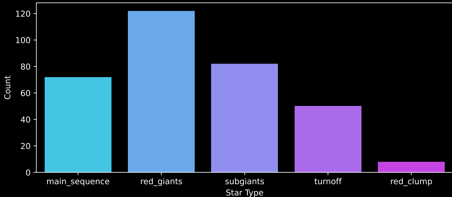
Gaia Cluster: [NGC_6404] Count plot of Star Type
