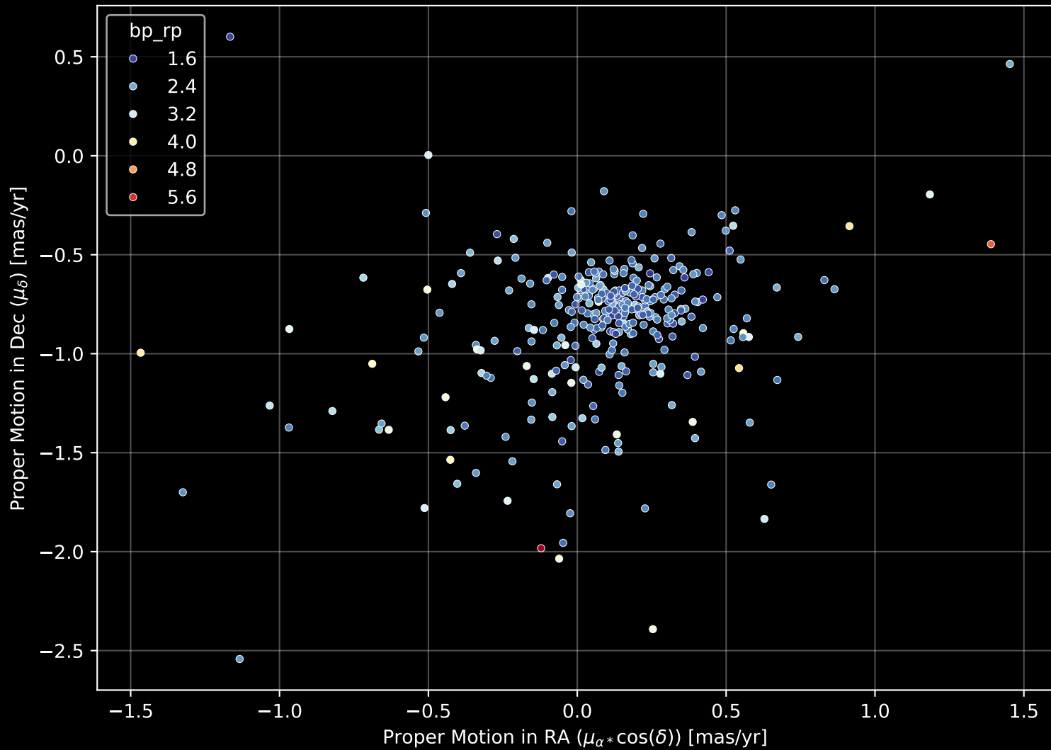
Gaia Cluster: [NGC_6404] Proper Motion Diagram (n= 334)
