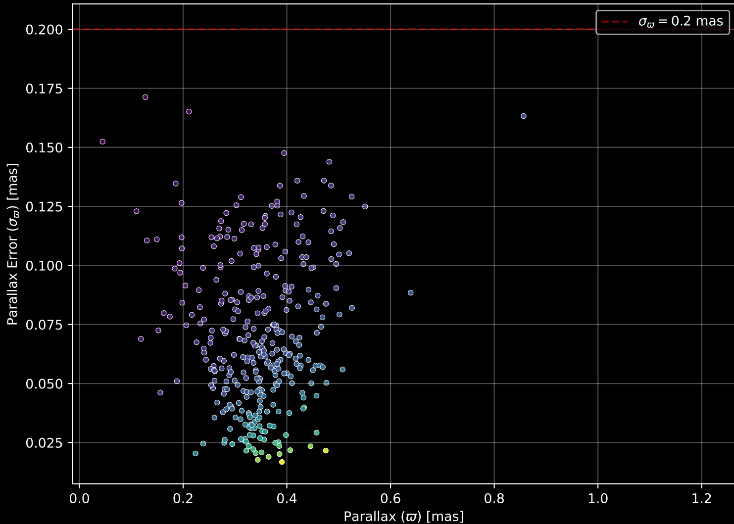
Gaia Cluster: [NGC_6404] Parallax Quality (n= 334)
