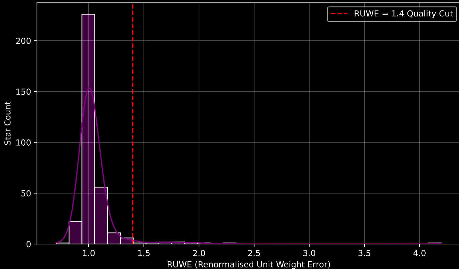
Gaia Cluster: [NGC_6404] RUWE Distribution (n= 332)
