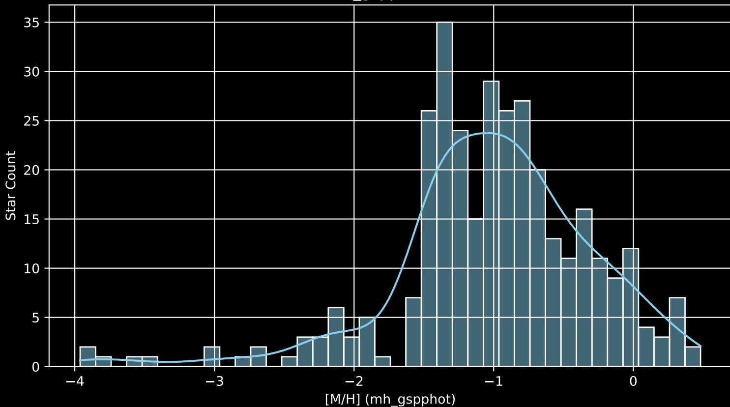
Gaia Cluster: [NGC_6404 [M/H] (mh_gspphot) (n= 329)
