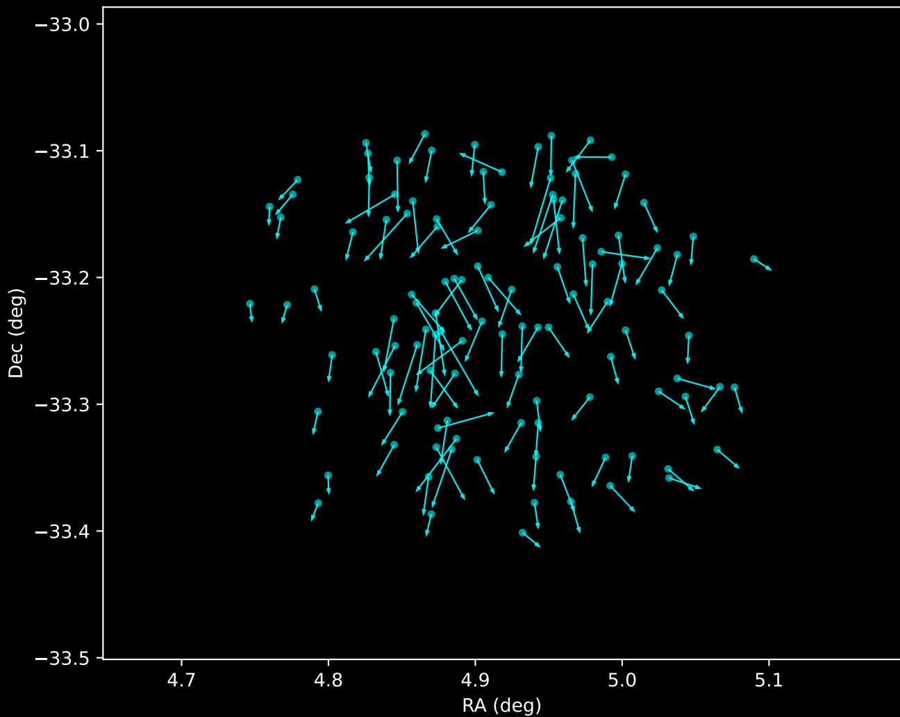
Gaia DR3 Noise Stream Proper Motion Vectors (n=114)
