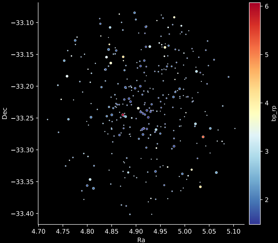
Gaia Cluster: [NGC_6404] Stars: 334
