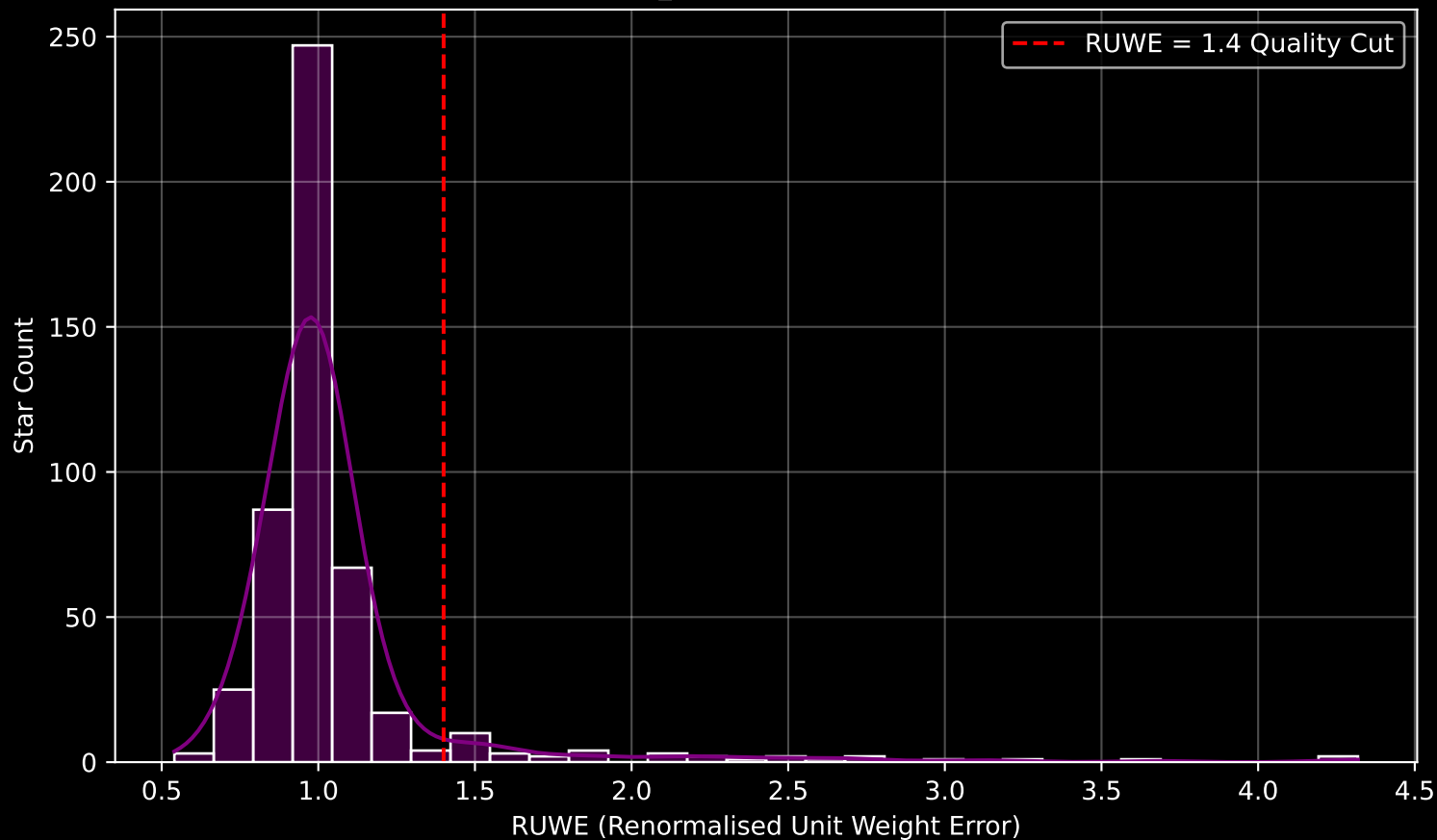
Gaia Cluster: [NGC_6405] RUWE Distribution (n= 485)
