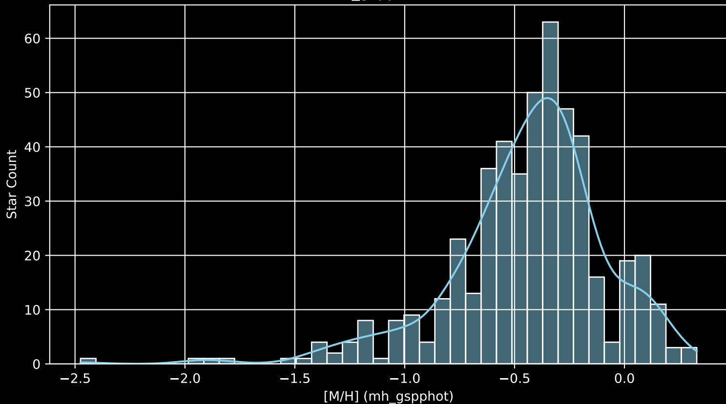
Gaia Cluster: [NGC_6405 [M/H] (mh_gspphot) (n= 484)
