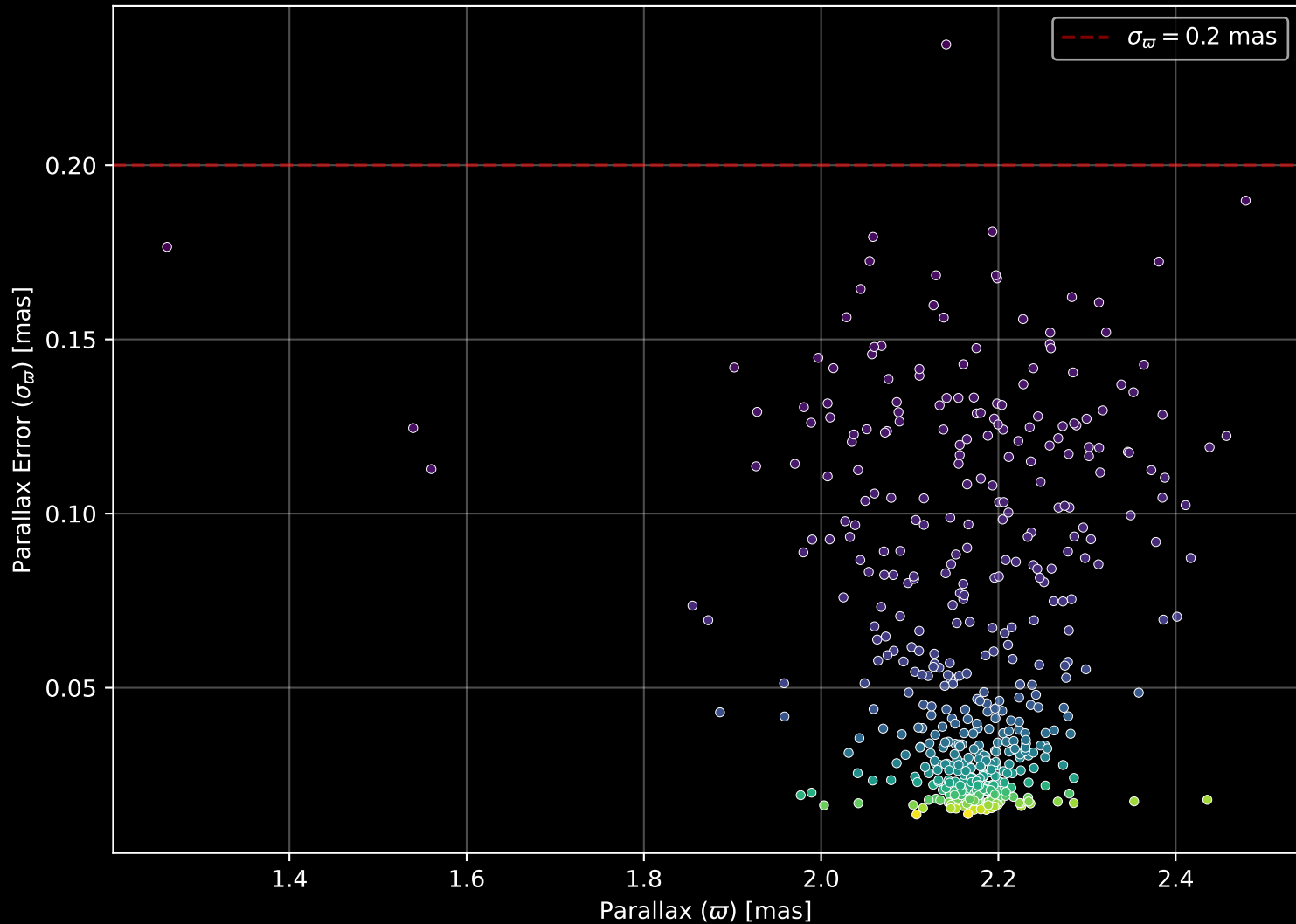
Gaia Cluster: [NGC_6405] Parallax Quality (n= 486)
