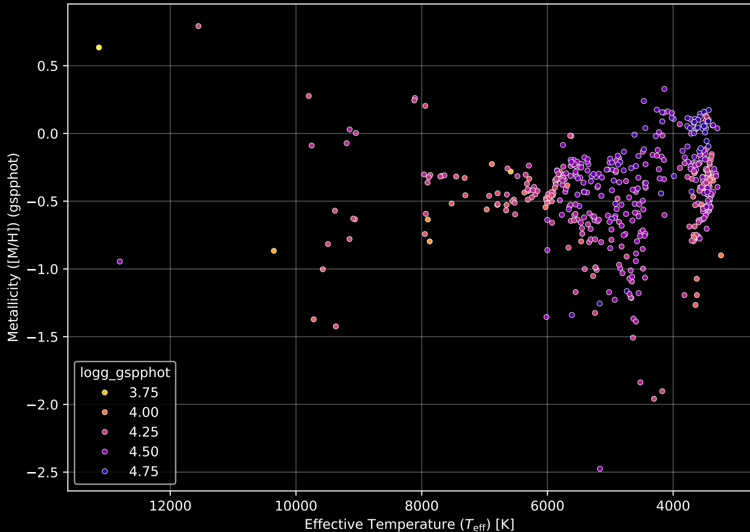
Gaia Cluster: [NGC_6405] Stellar Population Parameters (n= 486)
