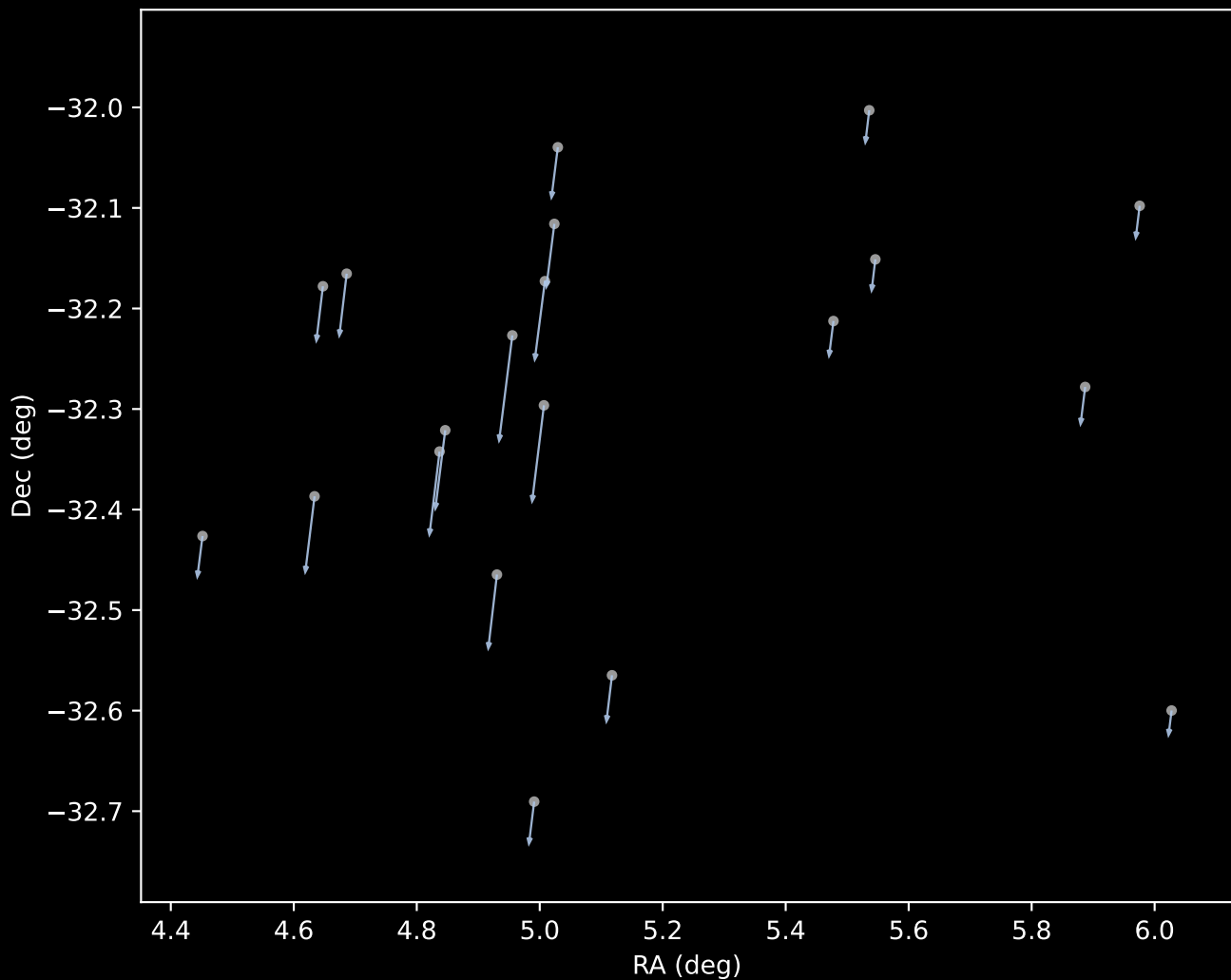
Gaia DR3 Cluster 21 Proper Motion Vectors (n=20)
