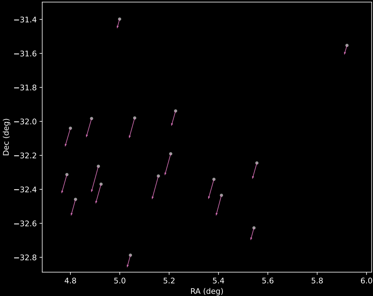
Gaia DR3 Cluster 12 Proper Motion Vectors (n=17)
