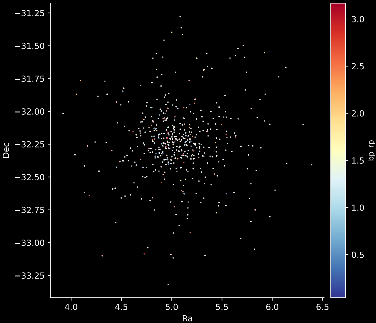
Gaia Cluster: [NGC_6405] Stars: 486
