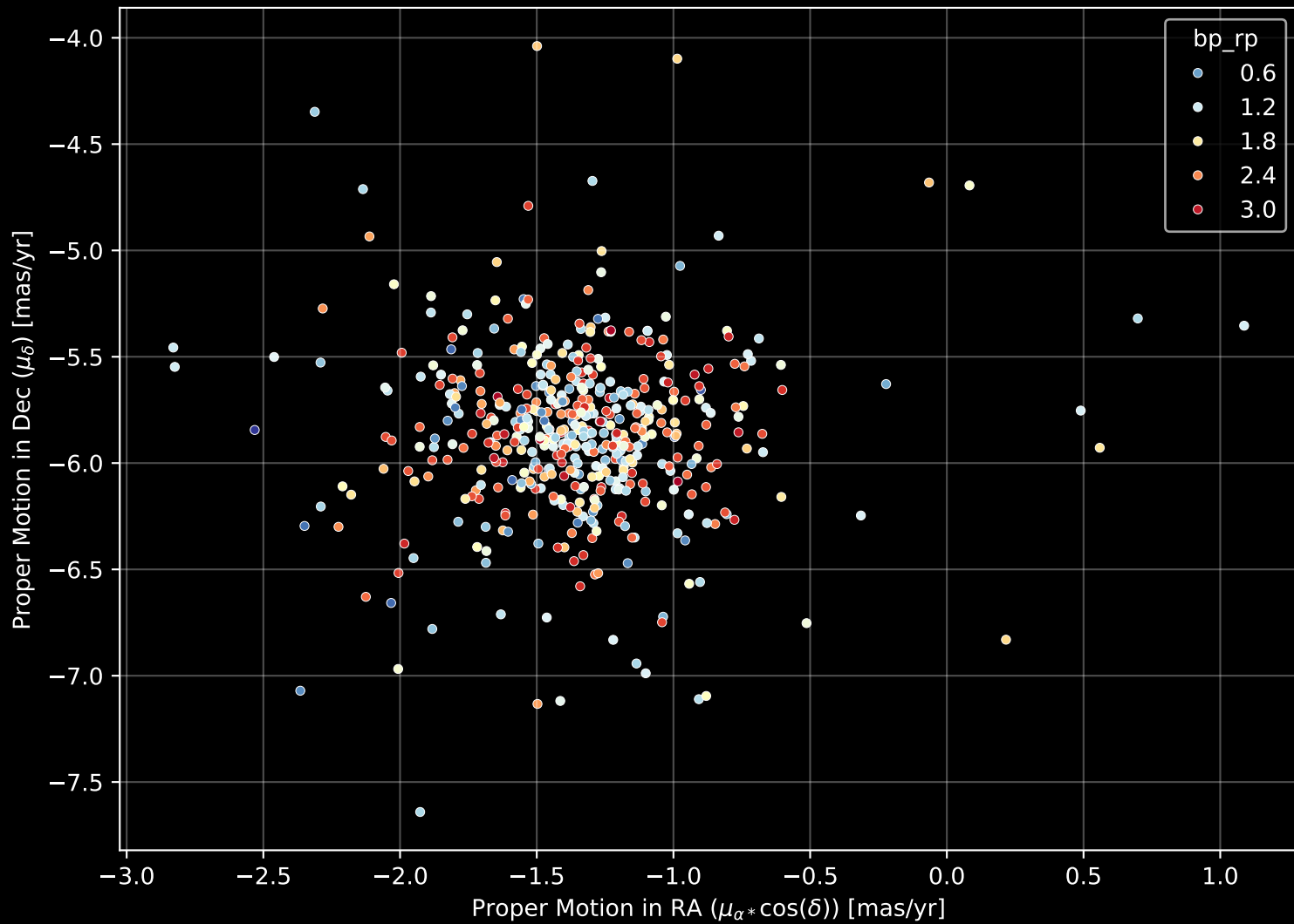
Gaia Cluster: [NGC_6405] Proper Motion Diagram (n= 486)
