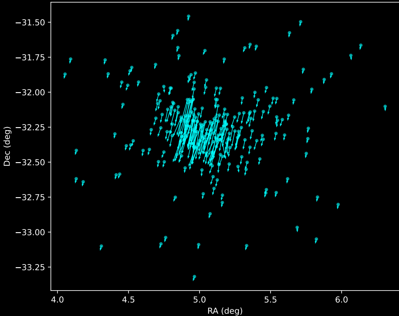
Gaia DR3 Noise Stream Proper Motion Vectors (n=247)
