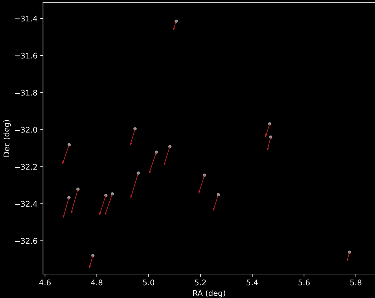
Gaia DR3 Cluster 6 Proper Motion Vectors (n=16)
