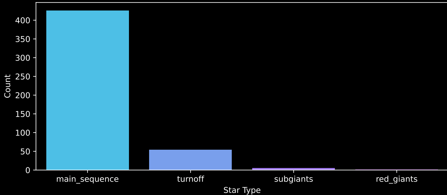
Gaia Cluster: [NGC_6405] Count plot of Star Type
