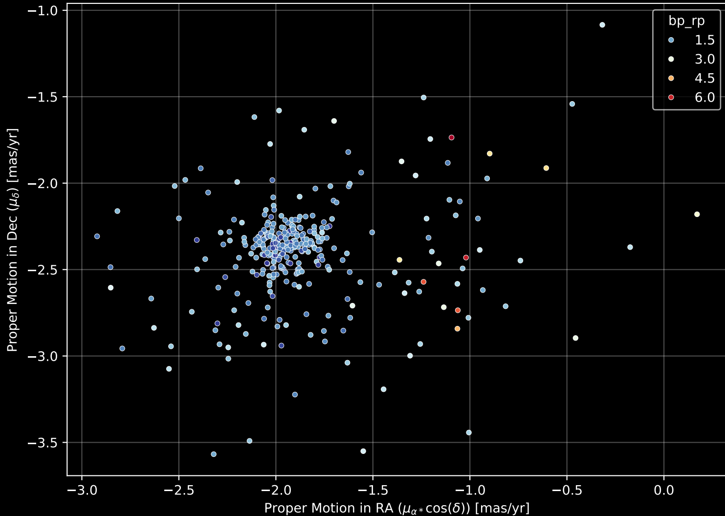
Gaia Cluster: [NGC_6416] Proper Motion Diagram (n= 333)
