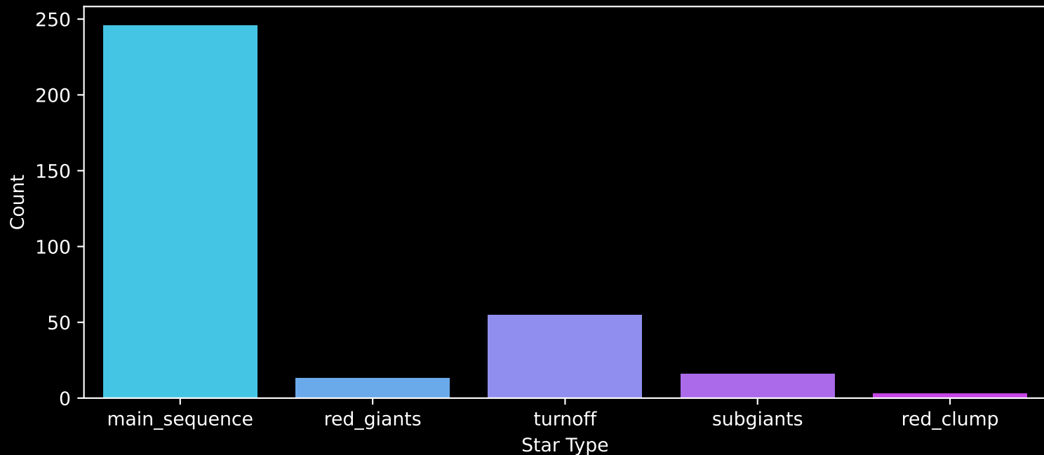
Gaia Cluster: [NGC_6416] Count plot of Star Type
