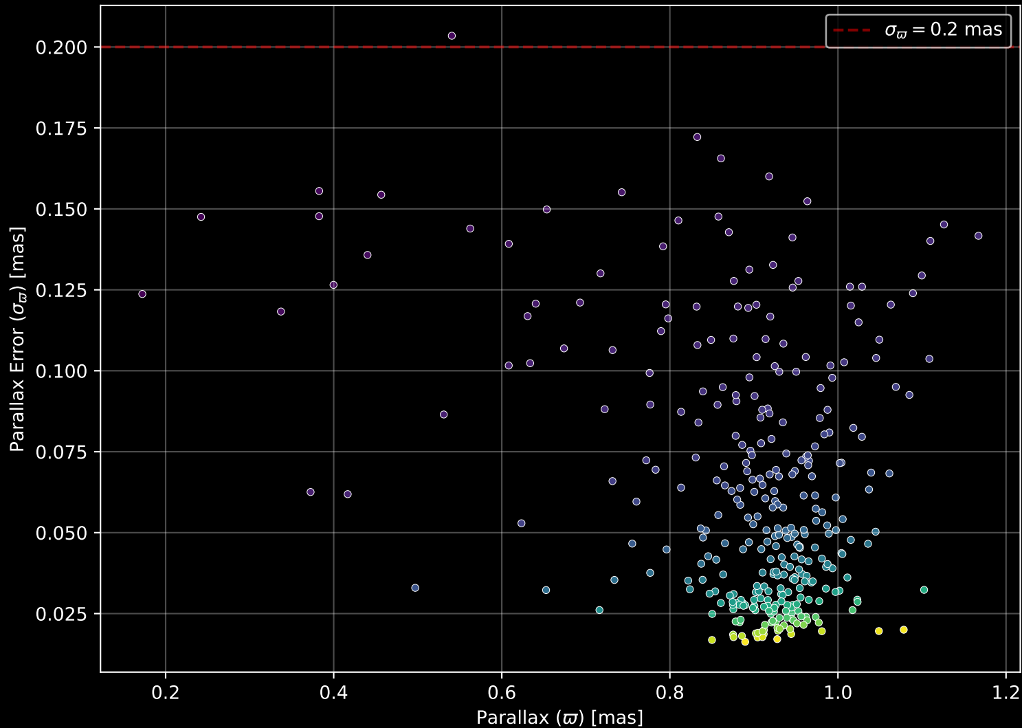
Gaia Cluster: [NGC_6416] Parallax Quality (n= 333)
