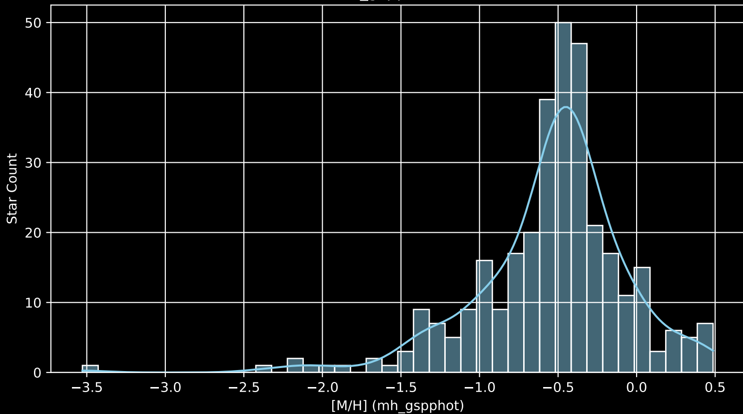
Gaia Cluster: [NGC_6416 [M/H] (mh_gspphot) (n= 326)
