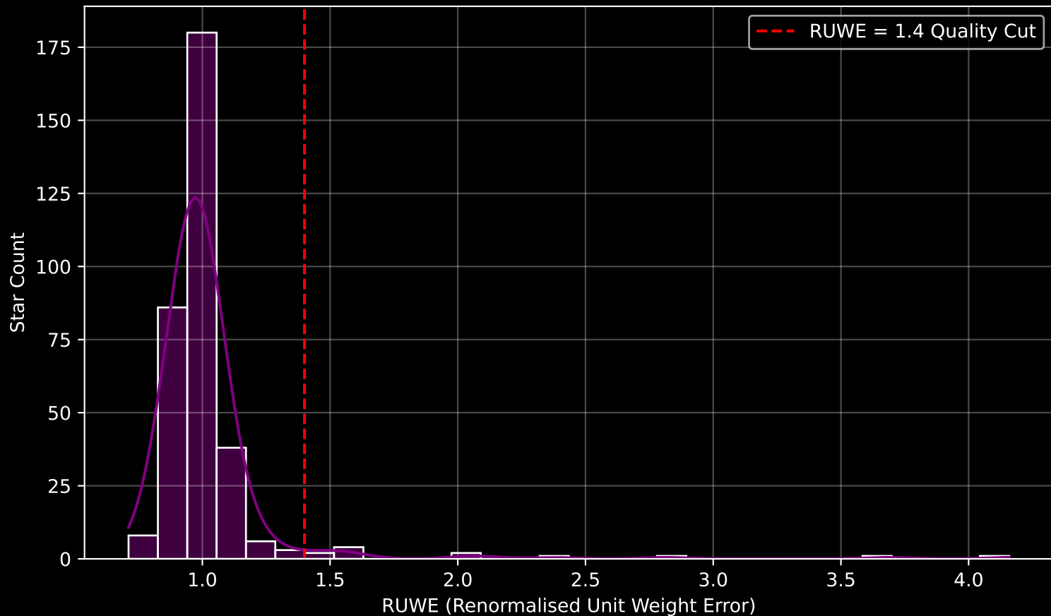
Gaia Cluster: [NGC_6416] RUWE Distribution (n= 333)
