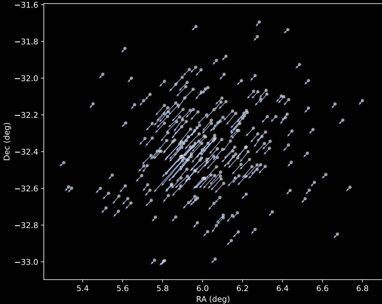
Gaia DR3 Cluster 1 Proper Motion Vectors (n=238)
